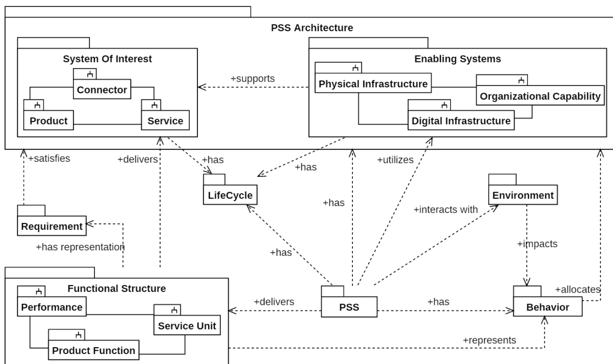
Figure 36. Package diagram
