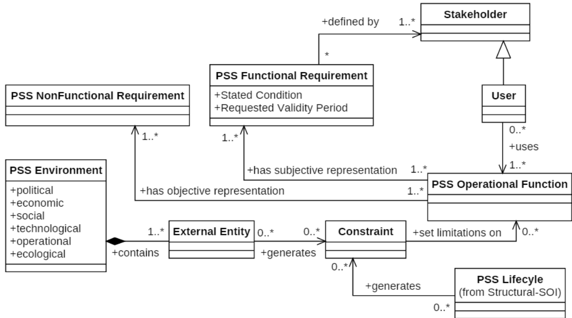
Figure 37. Requirements analysis
