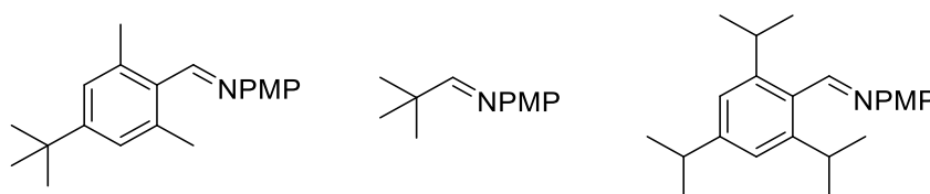
Chart 4.23 Unreactive imines
