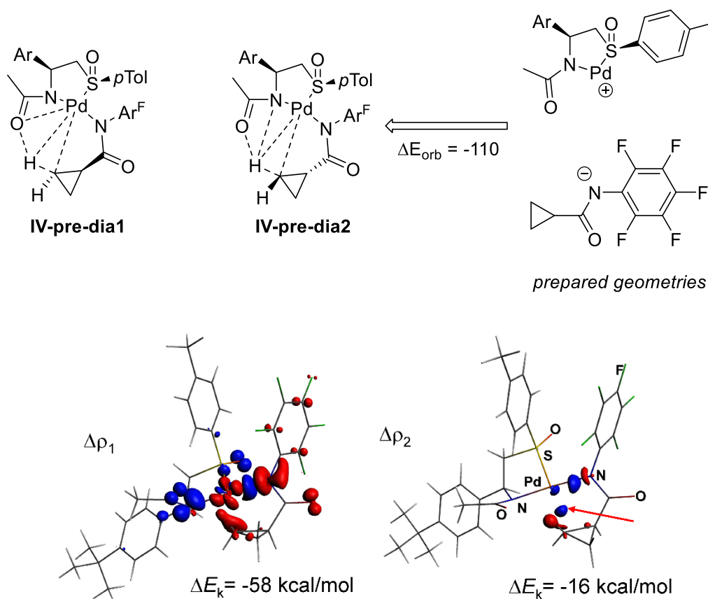
Figure 4.63 ETS-NOCV analysis of the bischelate formation
