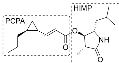
Chart 2.16 Hoshinolactam
