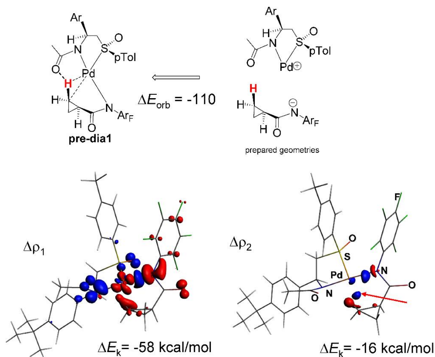
Figure 1. Plots of density deformation isosurfaces ( 0.005 \text{ e/bohr}^3 ) arising from the ETS-NOCV analysis of the interaction of the an-1b anion with the cat-Pd-L15 cation in their « prepared » geometries giving pre-dia1. Deformation density \Delta\rho_2 materialises, apart from the coordinative N-Pd interaction, the weak donor-acceptor « agostic » interaction between the vicinal \text{C}_{\text{cy}}\text{-H}_{\text{cy}} bond and the Pd(II) centre. \Delta\rho_2 contributes to about 14 % of the total interfragment orbital interaction energy. Blue and red isosurfaces are associated with density accepting and donating orbital contributors. The occurrence of a blue isosurface in an interatomic space is associated with the formation of a covalent bond. Red isosurfaces explicit the origin of the electron density contributing to the formation of this bond or to the population of the blue-colored orbital components.
