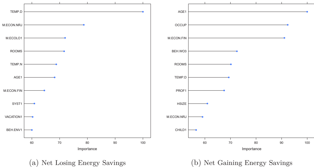
Figure 1.13: Feature Ranking using Decision Tree Classifier (Random Forest)
