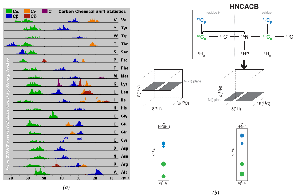
Figure 37 – Heteronuclear protein assignment. (a) Carbon chemical shift statistics for the 20 natural amino acid types in a protein, from the Biological Magnetic Resonance Bank (BMRB, http://www.bmrbl.wisc.edu/ ). They allow unambiguous recognition of certain residue types (Gly, Ala, Ser and Thr mainly). (b) Principle of the backbone sequential assignment of a [U\text{-}^{15}\text{N}; U\text{-}^{13}\text{C}] -labeled protein, with an HNCACB experiment. The intra-residue carbon chemical shift pattern of a residue can be matched to the inter-residue carbon chemical shift pattern of another residue, identifying them as sequentially linked.
