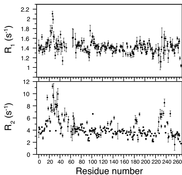
Figure 72 – ^{15}\text{N} R_1 and R_2 relaxation rates for the OY mutant of CtErbB2, measured at 22.3 T (950 MHz proton frequency).
