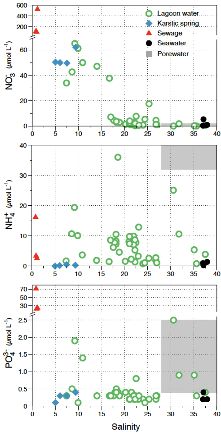
Figure 2.7| Dissolved inorganic nutrient ( \text{NO}_3^- , \text{NH}_4^+ and \text{PO}_4^{3-} ) concentrations in lagoon waters, the karstic spring, the sewage effluent and seawater endmembers, as a function of water salinity. The gray area represents the range of nutrient concentrations and salinities covering 66% of porewater samples (it extends to a salinity of 61 and to a \text{NH}_4^+ concentration of 180 \mu\text{mol L}^{-1} ).
