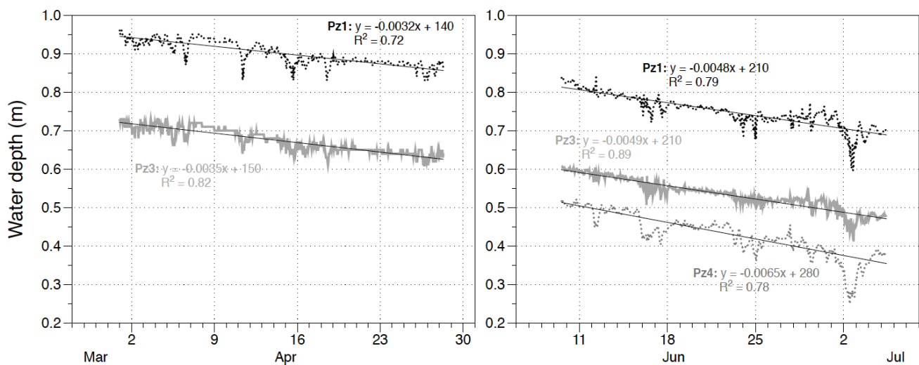
Figure 2.8| Evolution of water depths in the northern basin of La Palme lagoon in April and June 2017. Average changes in lagoon water level over time derived from linear regressions (-0.0034 and -0.0054 m d -1 for April and June 2017, respectively) were used to estimate \frac{\partial V_N}{\partial t} for April 2017 and June 2017 campaigns. The short-term variations on water depth are likely produced by rapidly changing wind conditions and are expected to have a minor influence on the water mass balance.
