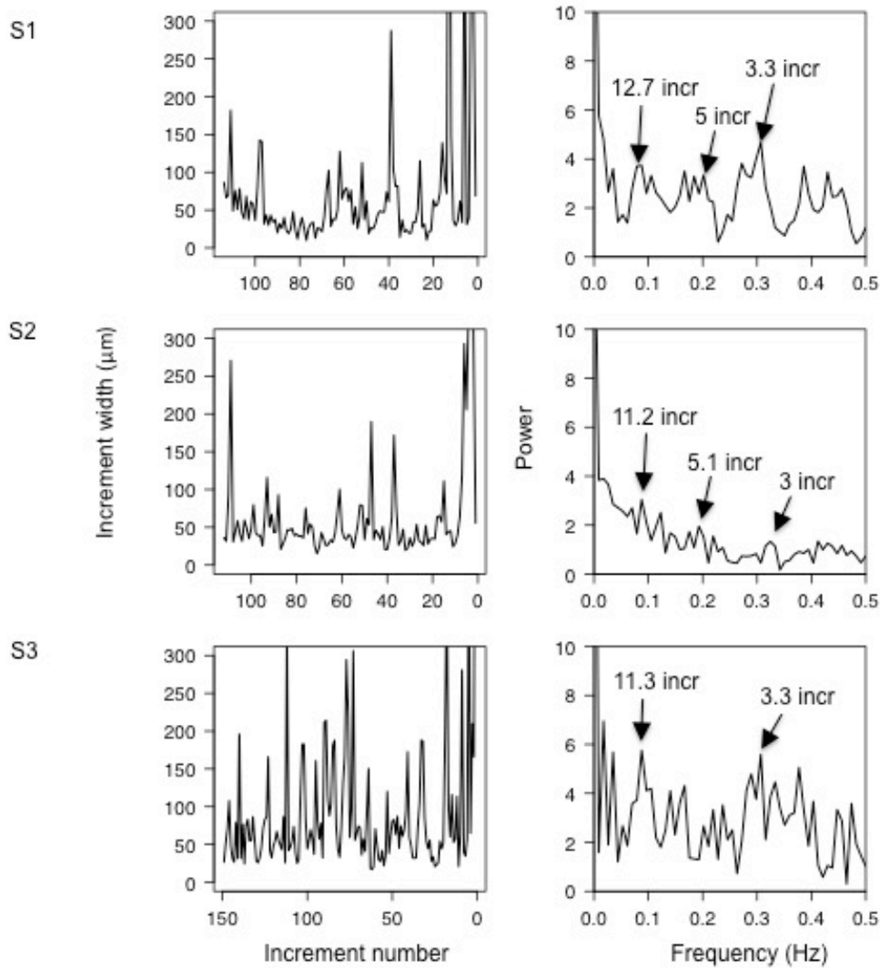
Figure 4.6 | Left panel: increment number from the calcein mark (right side) to the collection (left side) for three representative Mytilus galloprovincialis shells S1 (FDS0118-3), S2 (FDD0118-4) and S3 (PF0118-3) between June 2017 and January 2018. Right panel: Fast Fourier Transform showing the periodicities of the increment width.
