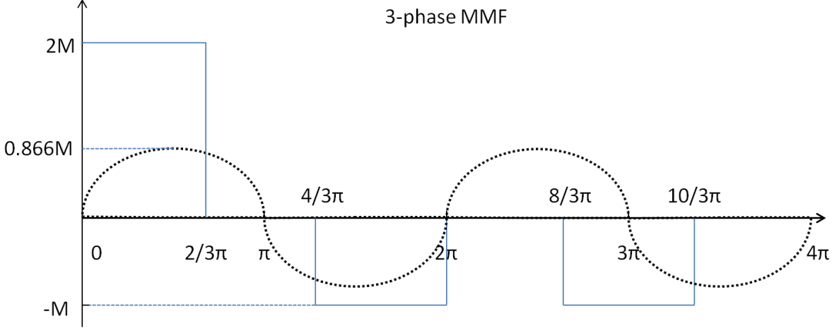
Fig. 57 3-phase MMF of 2p6s motor at the moment I_A = \hat{I}, I_B = -\hat{I}/2, I_C = -\hat{I}/2
