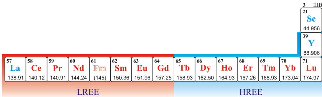
Fig. 5 Groups of light and heavy rare earth elements
