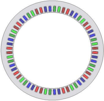
Fig. 125 Stator structure of 5p60s/f IPMSM with Delta connection
