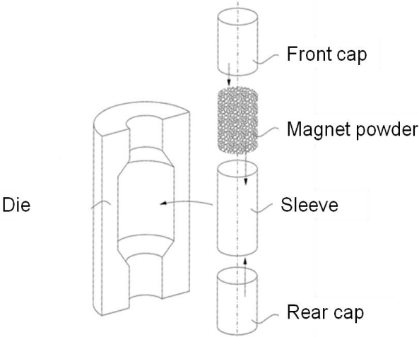
Fig. 45 IP magnet rotor production schematic diagram [72]
