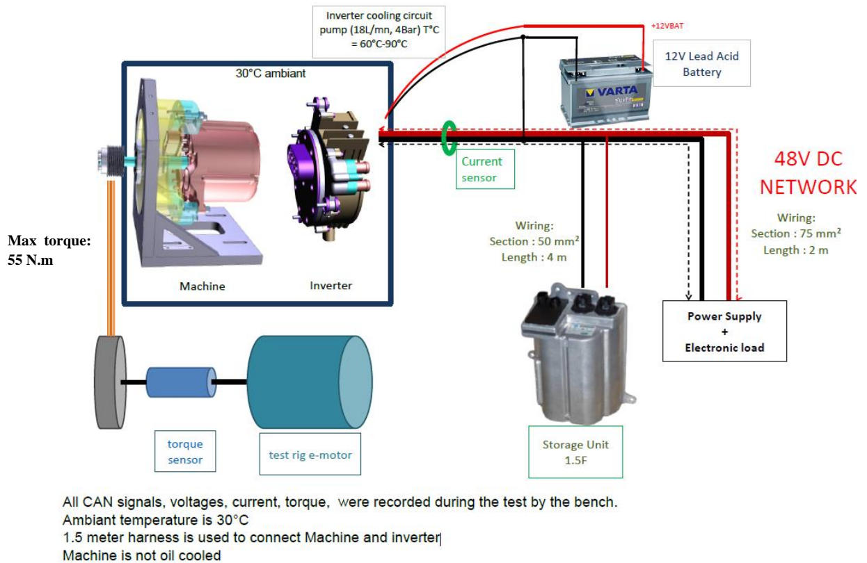
Fig. 160 Test bench configuration for the IPMSM mock-up tests
