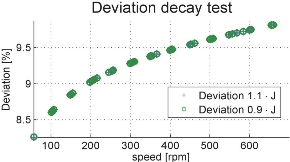
Fig. 189 Deviation of losses calculation with changing J
