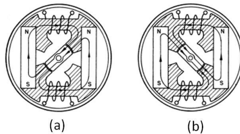
Fig. 32 schematic plot of a single phase PM flux-switch machine (a) armature with positive current magnitude; (b) armature with negative current magnitude [48].
