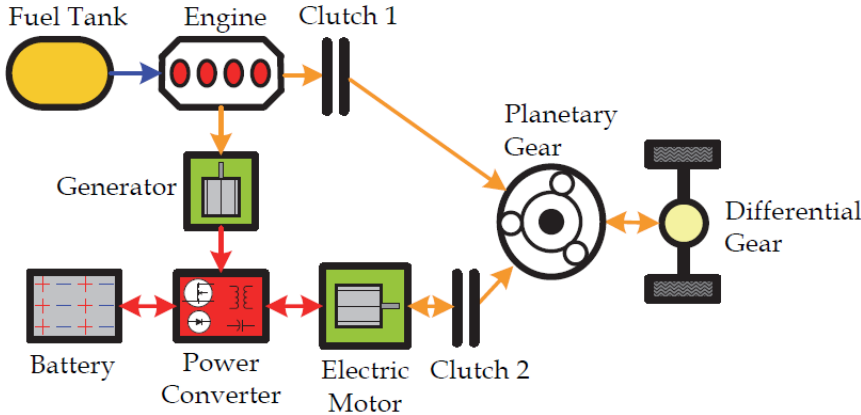
Fig. 39 Architecture of a typical series- parallel HEV [31]
