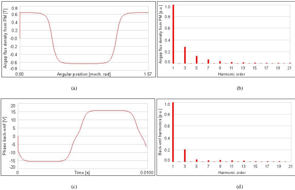
Fig. 3 EMETOR KTH results of (a)Waveform of airgap flux density during open circuit operation; (b) Spectrum of airgap flux density during open circuit operation; (c)Waveform of one phase back-EMF @1500 rpm; (b) Spectrum of one phase back-EMF @1500 rpm;
