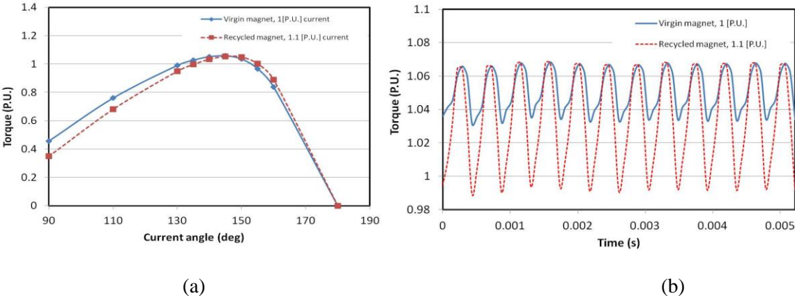
Fig. 206 Torque performances comparison between the IPMSMs with virgin magnet and recycled magnet respectively (a) Torque vs. current angle curves @ 120 °C (b) torque ripple curves @ 120 °C around 140° current angle. Torque ripple rate of the virgin magnet machine equals 3.5 %, the recycled magnet machine equals 7.6%.
