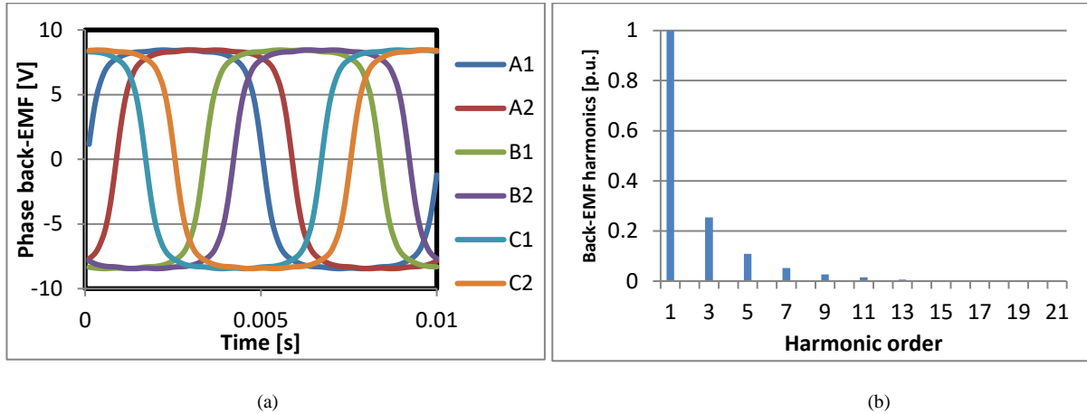
Fig. 16 (a) Waveform of six phase back-EMF @1500 rpm; (b) Spectrum of phase A1 back-EMF @1500 rpm;
