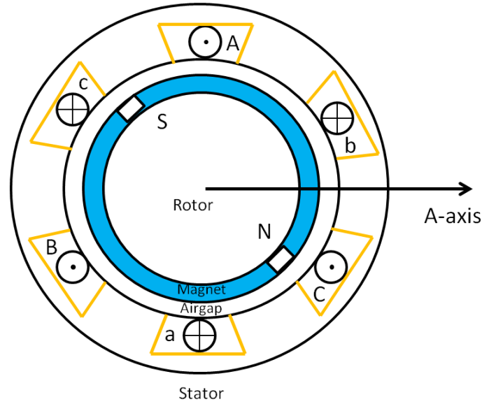
Fig. 53 A simple model that represent a 2-pole, three phases, inner rotor SPMSM
