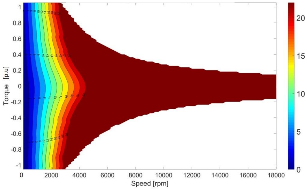
Fig. 122 Total voltage map (Vac) of 5p60s/f IPM at 80°C
