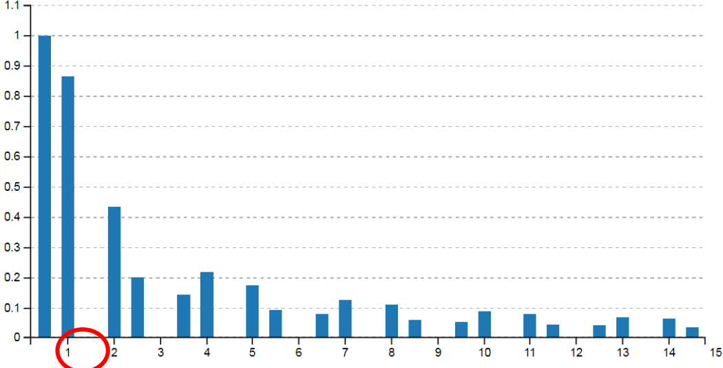
Fig. 58 Harmonics spectrum of 2p6s motor MMF by using FFT
