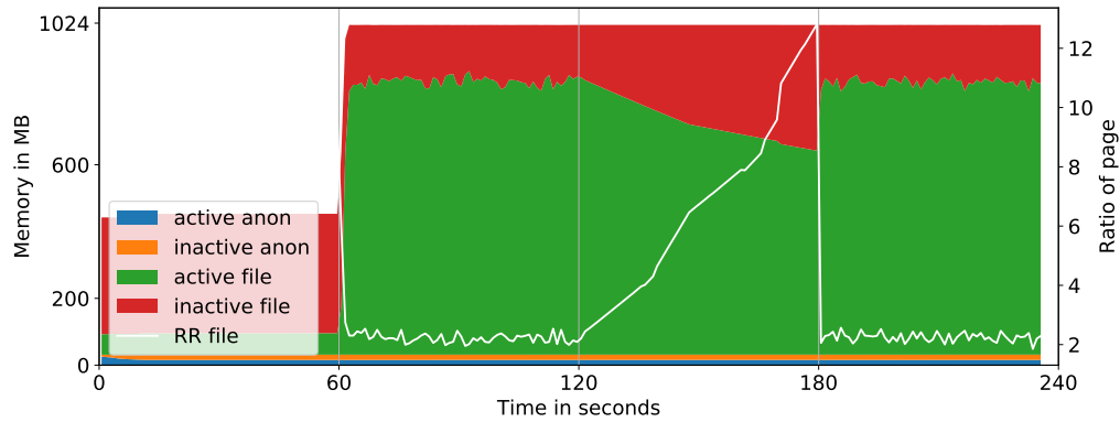
(c) The \text{lru} is artificially updated at an extra 1 MB/s rate.
