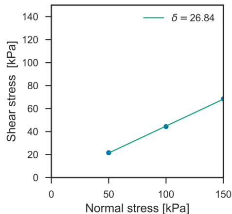
Figure 3-13: Interface friction angle of Fontainebleau sand – concrete interface at 13^{\circ}\text{C} .
