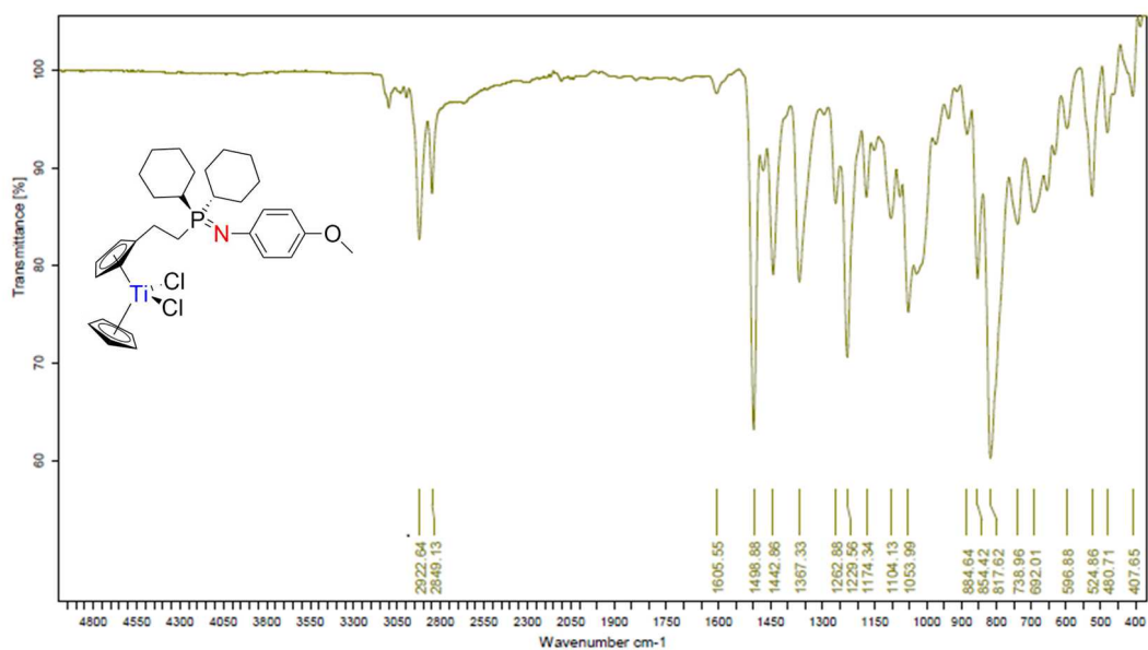
Spectrum 0-496: HRMS of 59 (Positive mode ESI, dichloromethane)
