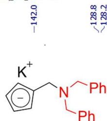
Spectrum 0-13: ^1\text{H} NMR of 3-K (500.03 MHz, 300 K, dimethylsulfoxide- d_6 )
