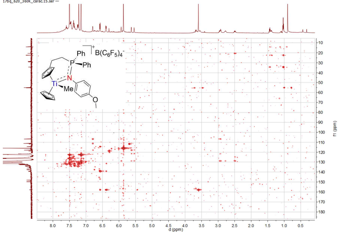
Spectrum 0-554: ^1\text{H} ^{13}\text{C} HMBC of 64 (600.23 MHz / 150.94 MHz, 360 K, bromobenzene- d_5 )
