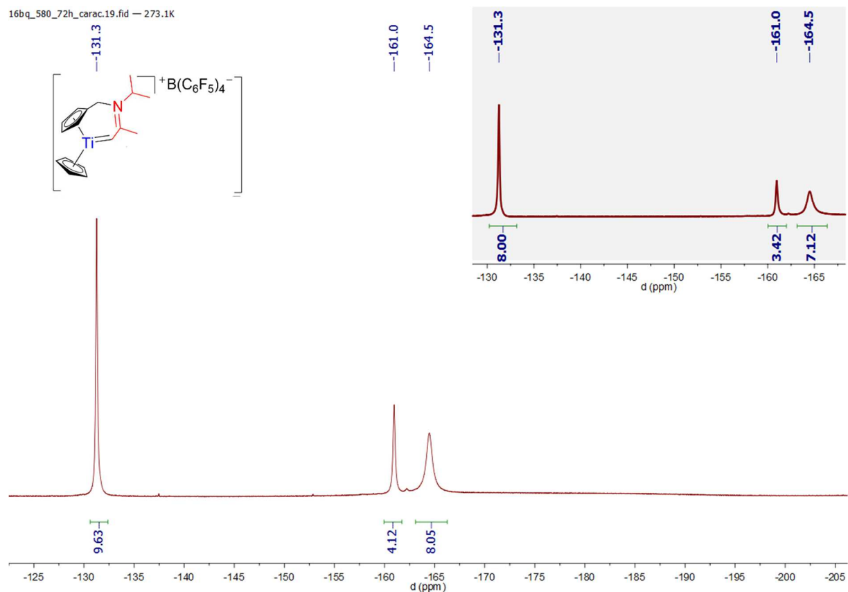
Spectrum 0-332: ^{19}\text{F}\{^1\text{H}\} and ^{19}\text{F} (opacified) NMR of 43 (470.45 MHz, 273 K, bromobenzene- d_5 )
