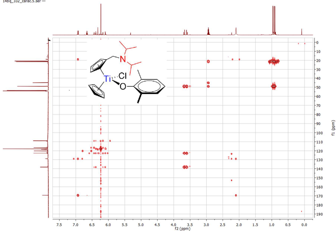
Spectrum 0-195: ^1\text{H} ^{13}\text{C} HMBC of 28 (600.23 MHz / 150.94 MHz, 300 K, dichloromethane- d_2 )
