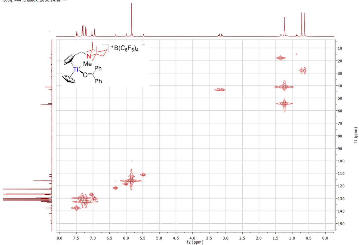
Spectrum 0-276: ^1\text{H} ^{13}\text{C} HMQC 38 (500.03 MHz / 125.03 MHz, 263 K, bromobenzene- d_5 )
