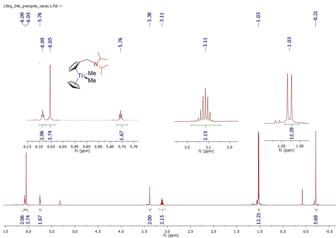
Spectrum 0-235: ^1\text{H} NMR of 34 (600.23 MHz, 300 K, dichloromethane- d_2 )
