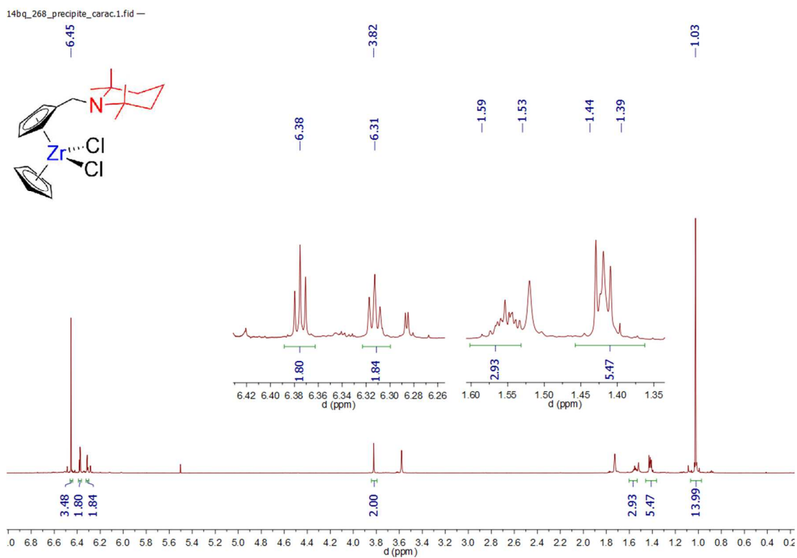
Spectrum 0-157: 1 H NMR of 24 (600.23 MHz, 300 K, tetrahydrofuran-d 8 )
