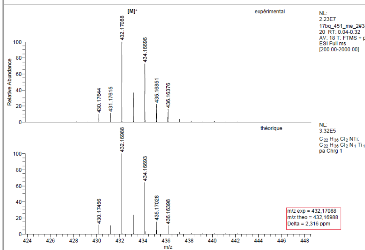
Spectrum 0-174: HRMS of 25 (Positive mode ESI, dichloromethane)
