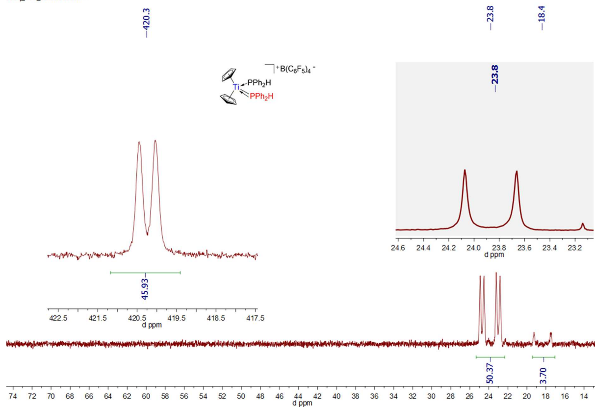
Spectrum 0-381: ^{31}P\{^1H\} and ^{31}P (opacified) NMR of 50 (202.41 MHz, 300 K, bromobenzene- d_5 )
