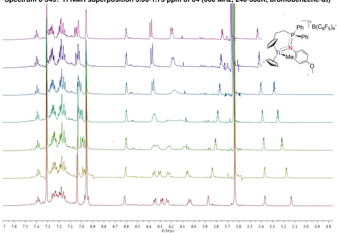
Spectrum 0-546: ^1\text{H} NMR superposition 7.6-4.8 ppm of 64 (600 MHz, 240-360K, bromobenzene- d_5 )
