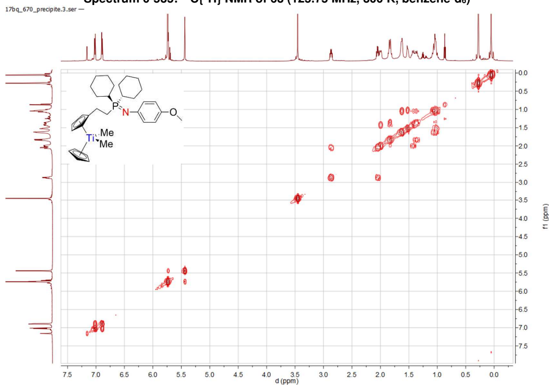
Spectrum 0-536: ^1\text{H} \ ^1\text{H} COSY of 63 (500.03 MHz, 300 K, 273 K, benzene- d_6 )
