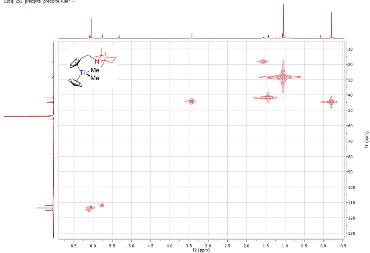
Spectrum 0-247: ^1\text{H} ^{13}\text{C} HMQC of 35 (600.23 MHz / 150.9 MHz, 300 K, dichloromethane- d_2 )
