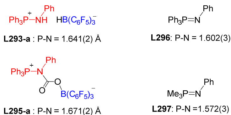
Scheme V-9: P-N bond lengths reported in the literature
