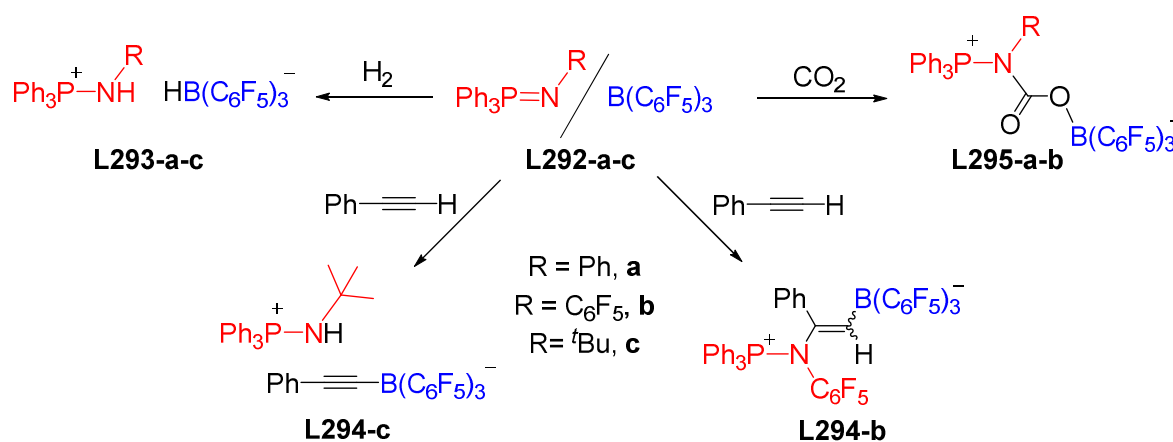
Scheme V-1: an iminophosphorane-based organic FLP
