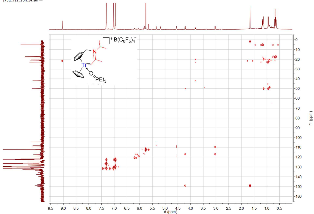
Spectrum 0-354: 1 H 13 C HMBC of 45 (600.23 MHz / 150.86 MHz, 300 K, bromobenzene-d 5 )
