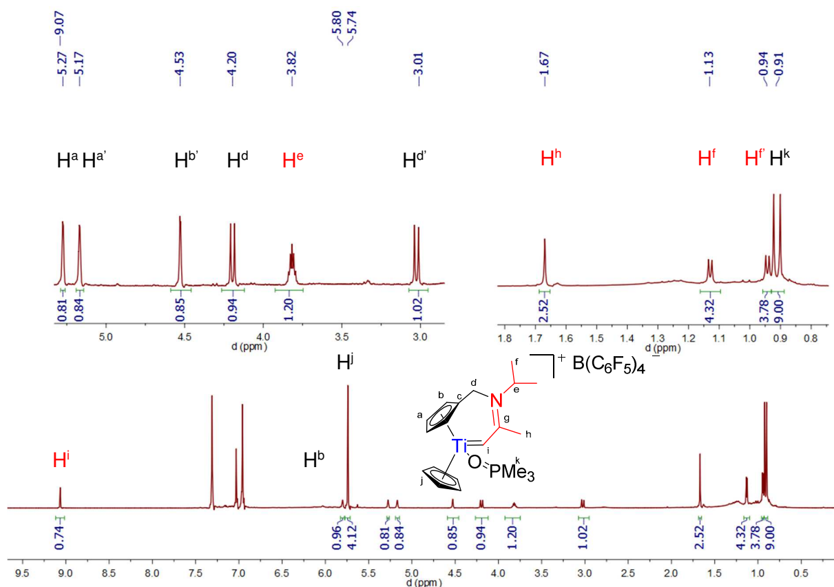
Spectrum III-12: ^1\text{H} NMR of 44 (600.23 MHz, 300 K, bromobenzene- d_5 )
