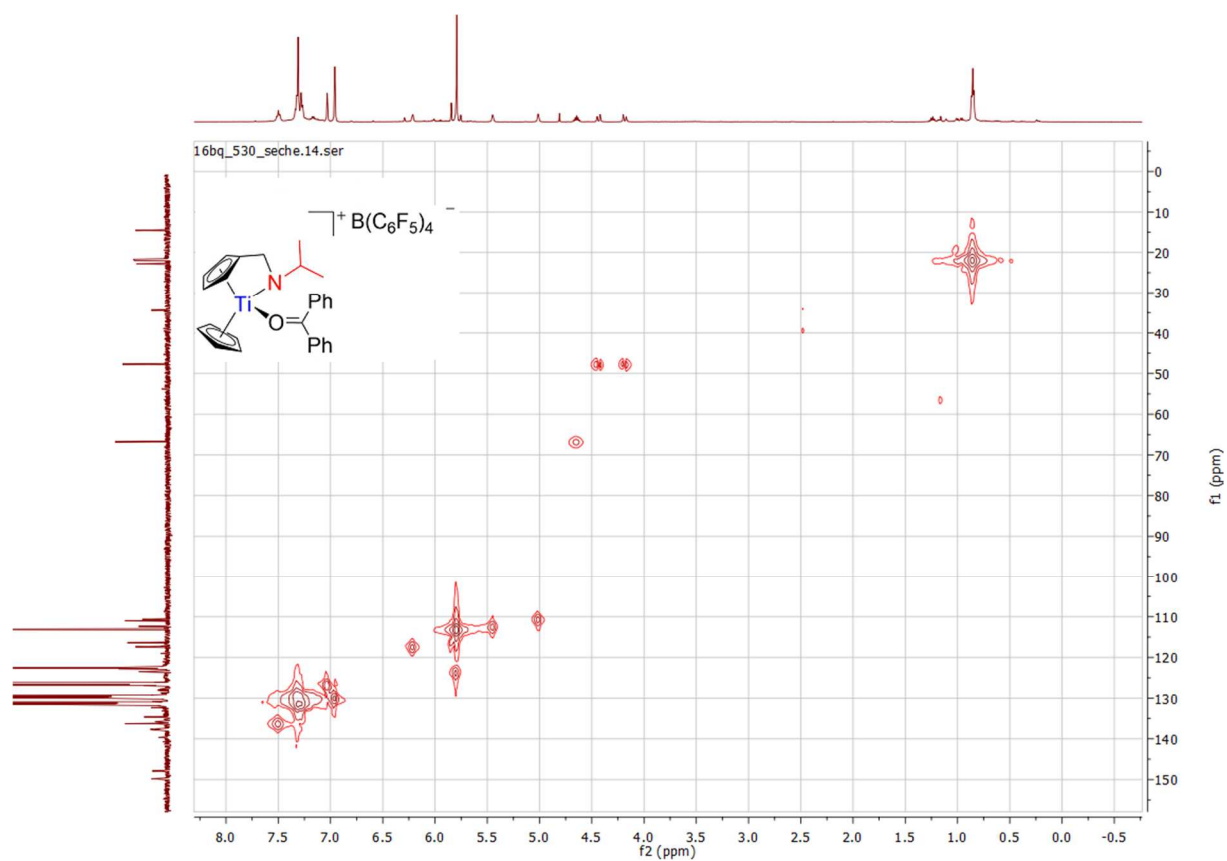
Spectrum 0-305: ^1\text{H} ^{13}\text{C} HMQC of 41 (500.03 MHz / 125.03 MHz, 300 K, bromobenzene- d_5 )
