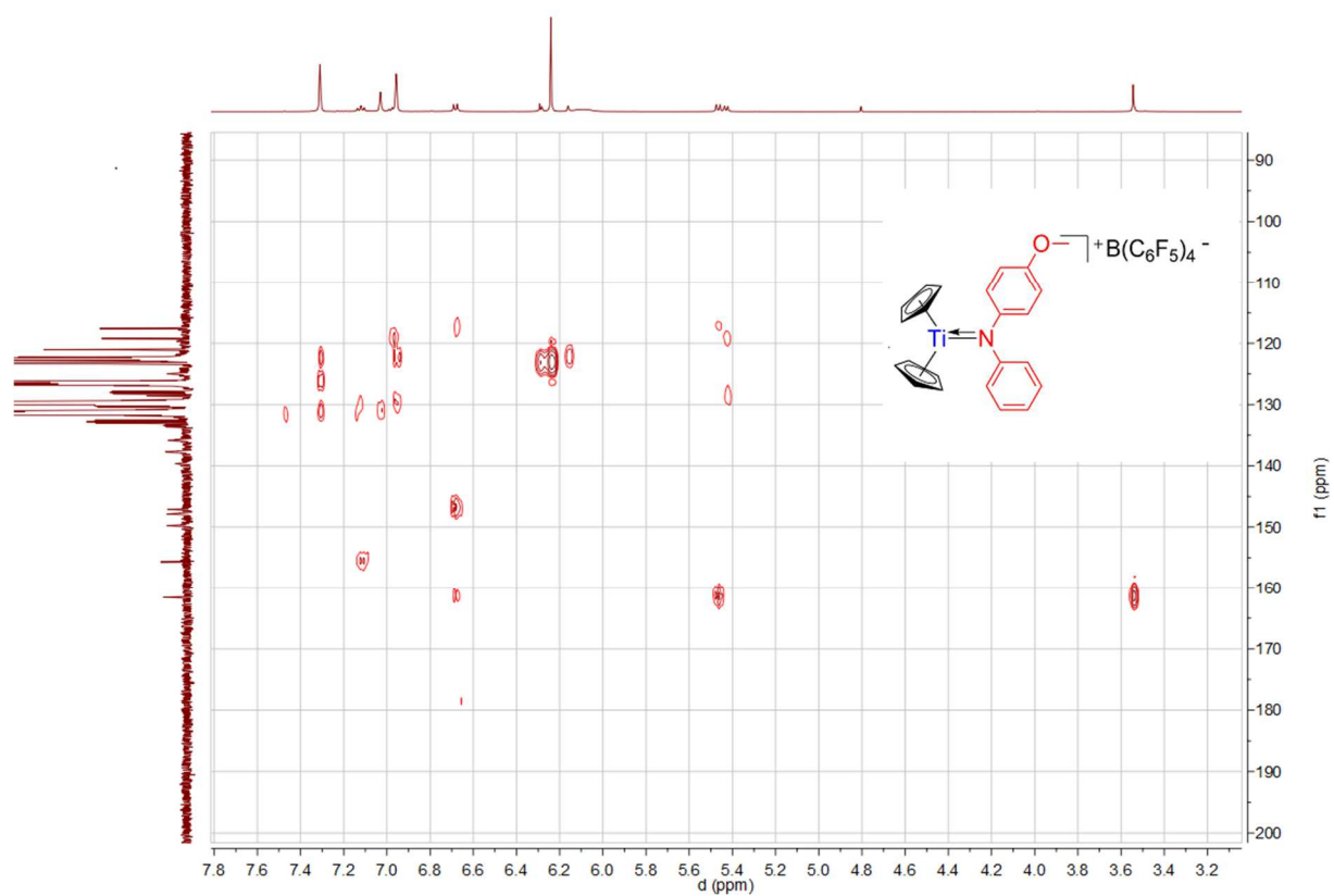
Spectrum 0-430: 1 H 13 C HMBC of 55 (500.03 MHz / 125.75 MHz, 300 K, bromobenzene-d 5 )
