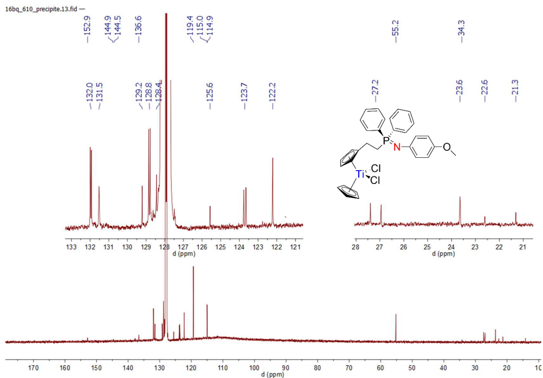
Spectrum 0-469: ^{13}\text{C}\{^1\text{H}\} NMR of 57 (125.75 MHz, 300 K, benzene- d_6 )
