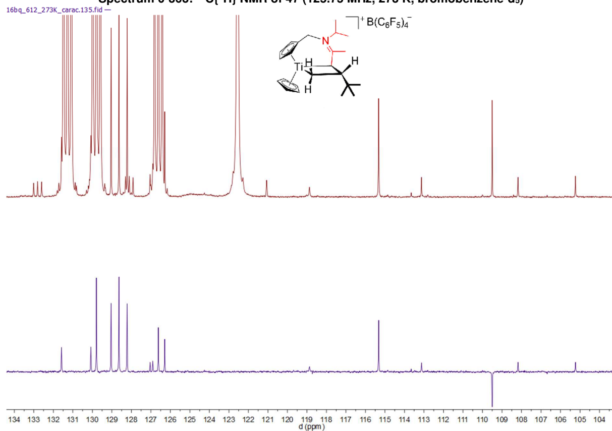
Spectrum 0-364: ^{13}C\{^1H\} NMR (top) correlated with dept135 (bottom) of 47 (125.75 MHz, 273 K, bromobenzene- d_5 )
