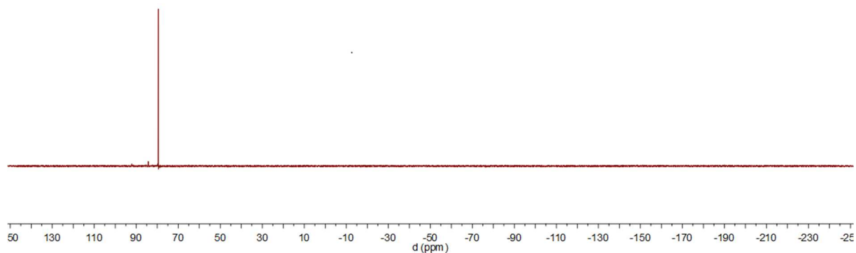
Spectrum 0-271: ^{31}\text{P}\{^1\text{H}\} NMR and ^{31}\text{P} (opacified) of 37 (202.46 MHz, 300 K, dichloromethane- d_2 )
