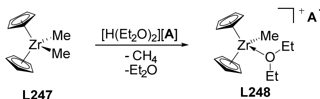
Scheme III-6: protonolysis of L247 with [\text{H}(\text{Et}_2\text{O})_2][\text{A}]
