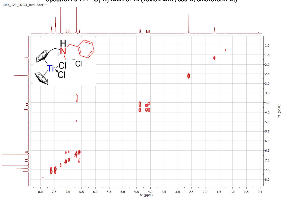
Spectrum 0-78: ^1\text{H} ^1\text{H} COSY of 14 (500.03 MHz, 300 K, chloroform- d_1 )
