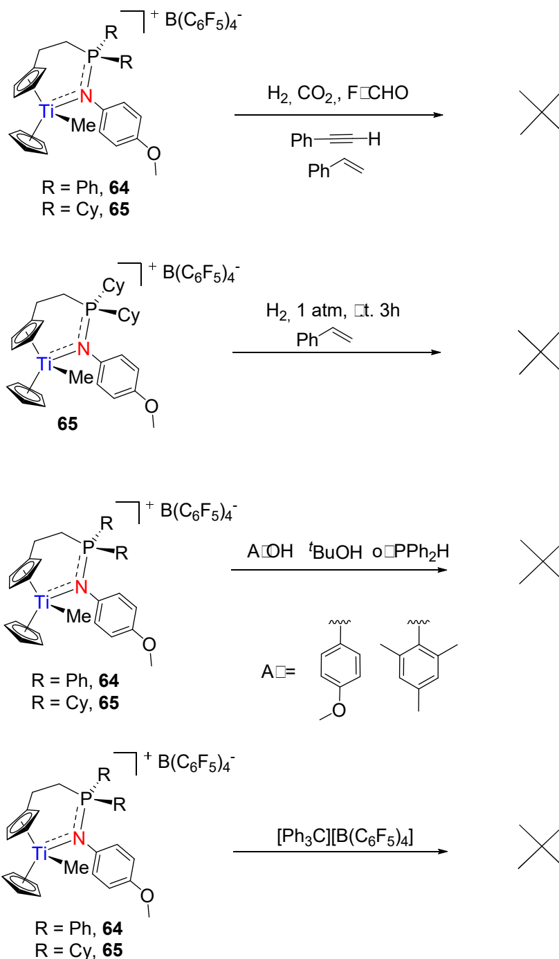
Scheme V-12: reactivity studies of 64 and 65
