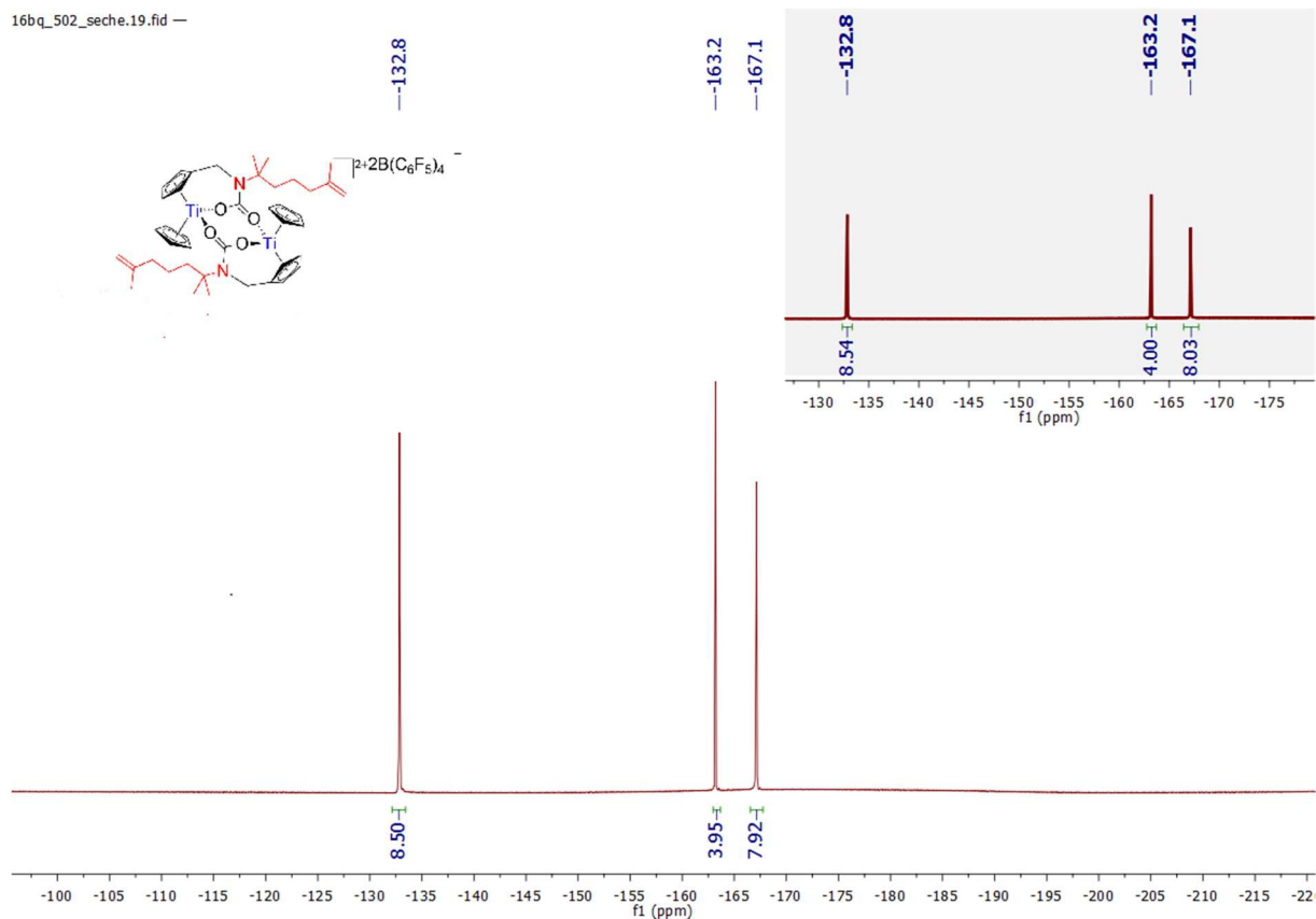
Spectrum 0-289: ^{19}\text{F}\{^1\text{H}\} and ^{19}\text{F} (opacified) NMR of 39 (470.45 MHz, 300 K, dichloromethane- d_2 )
