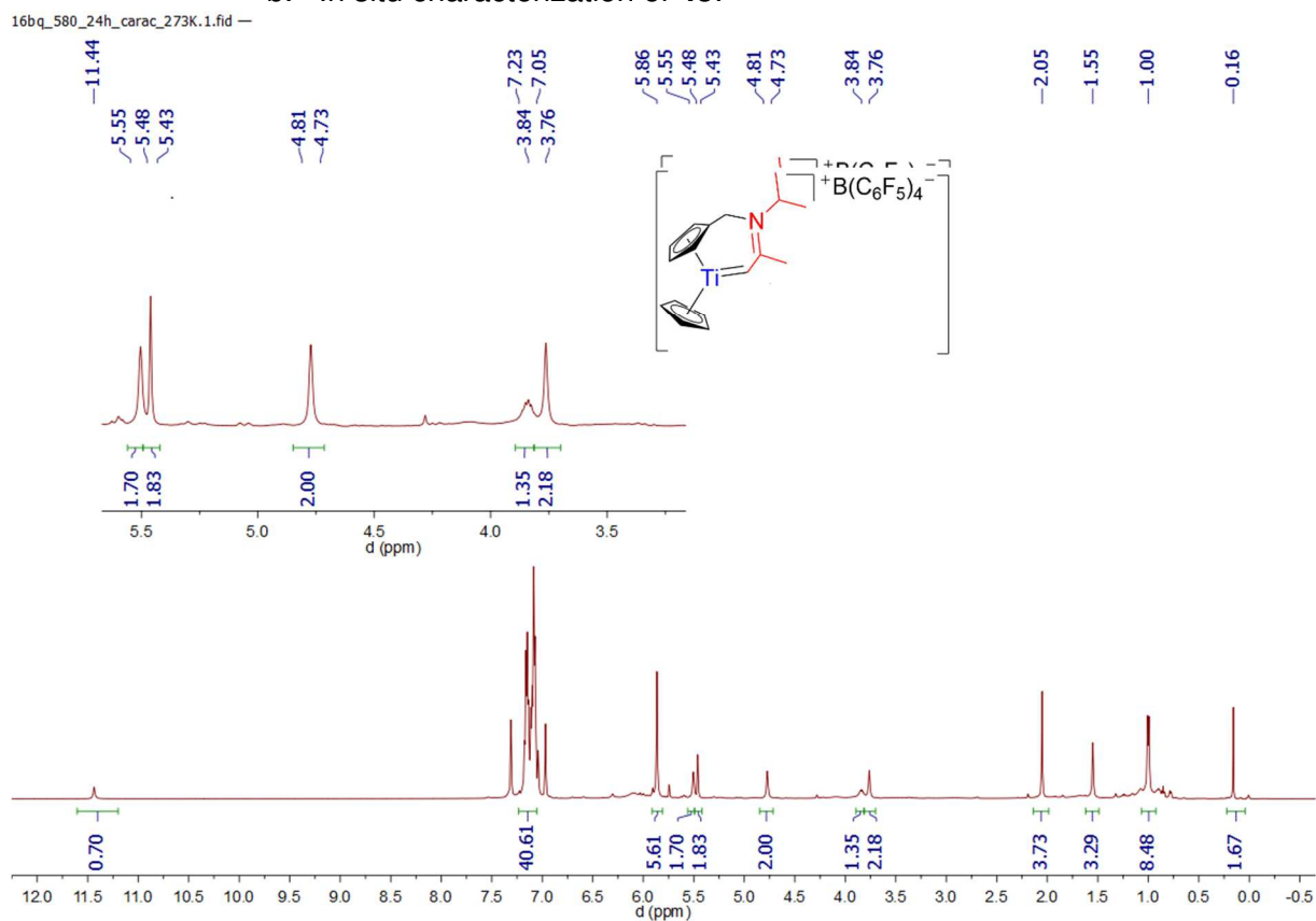
Spectrum 0-325: 1 H NMR of 43 (500.03 MHz, 273 K, bromobenzene-d 5 )
