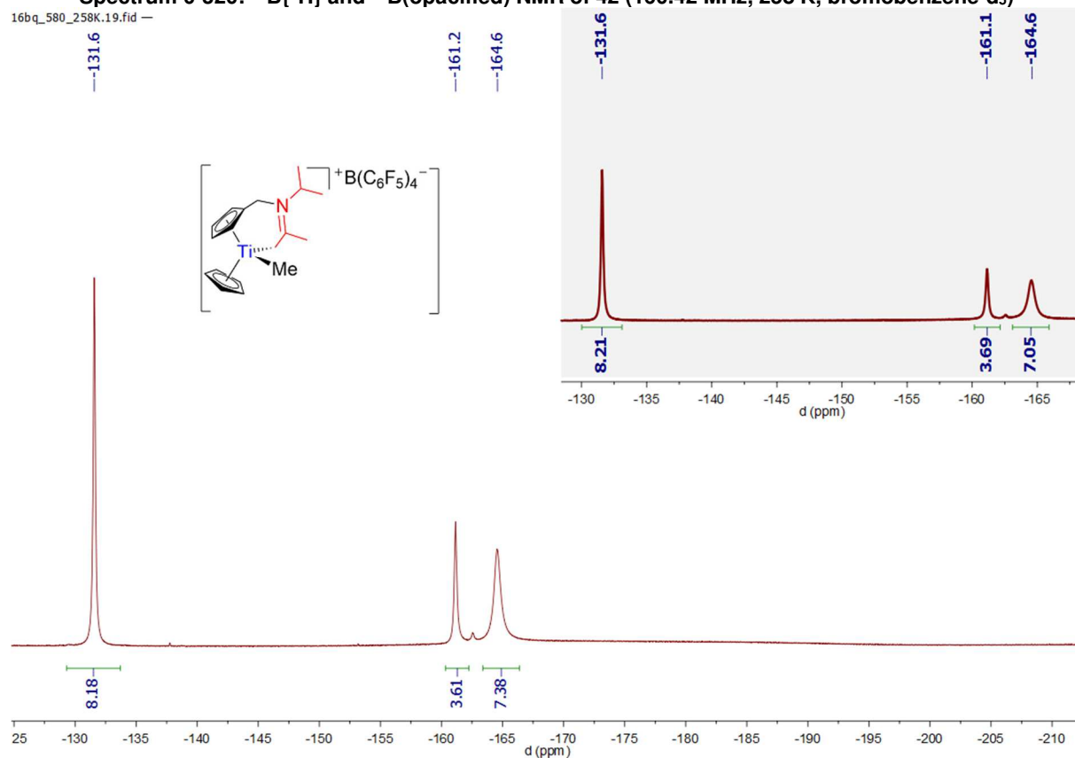
Spectrum 0-321: ^{19}\text{F}\{^1\text{H}\} and ^{19}\text{F} (opacified) NMR of 42 (470.45 MHz, 258 K, bromobenzene- \text{d}_5 )
