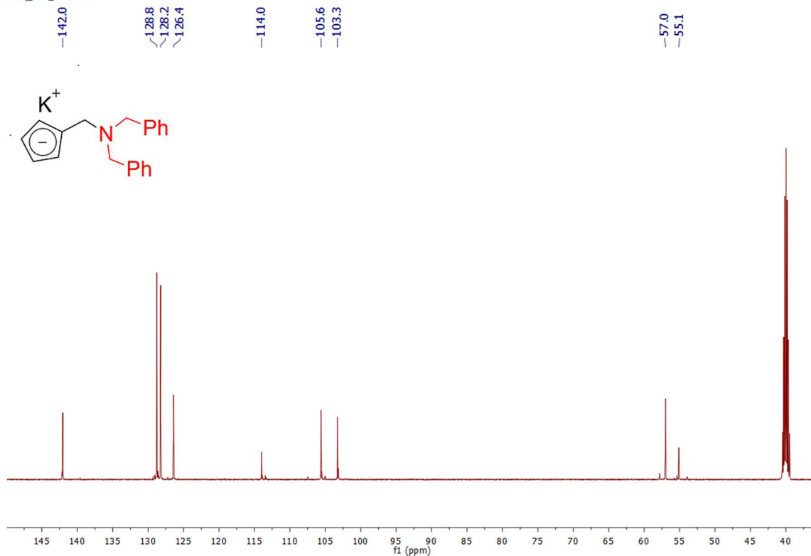
Spectrum 0-14: ^{13}\text{C}\{^1\text{H}\} NMR of 3-K (125.77 MHz, 300 K dimethylsulfoxide- d_6 )
