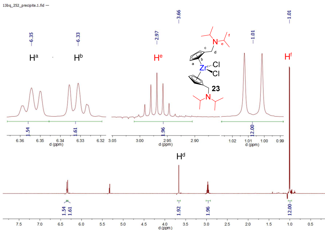
Spectrum II-6: ^1\text{H} NMR of 23 (600.23 MHz, 300 K, dichloromethane- d_2 )
