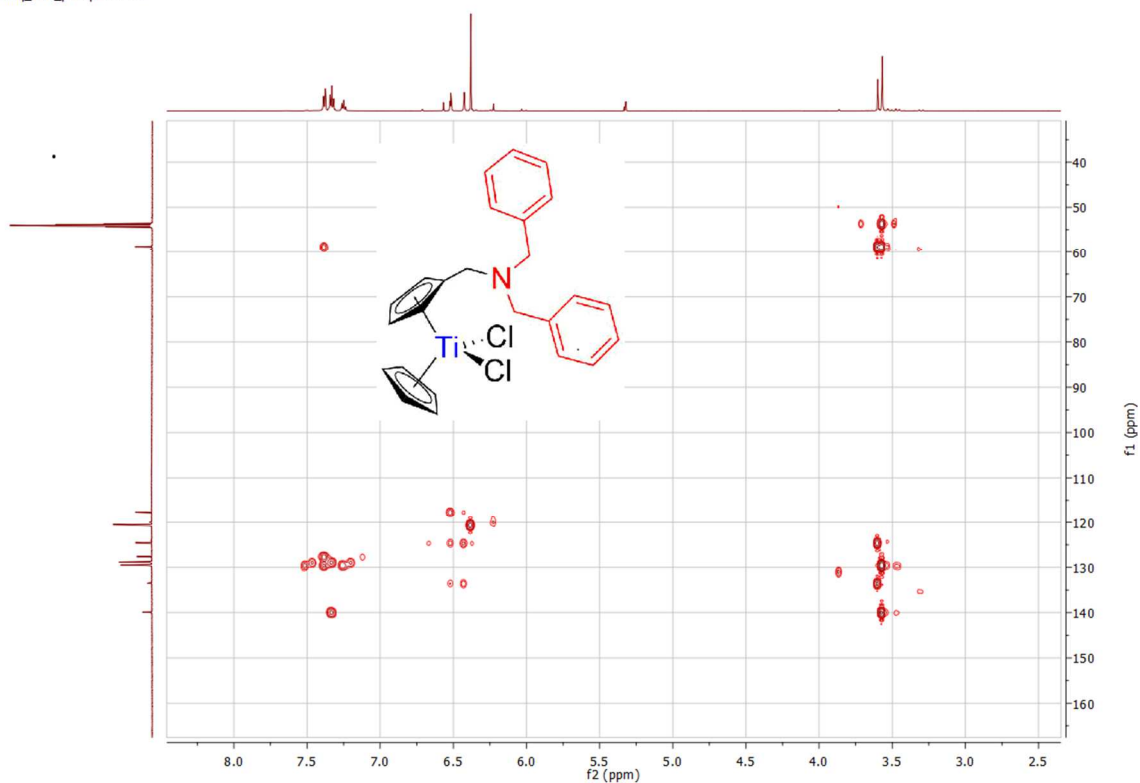
Spectrum 0-53: ^1\text{H} ^{13}\text{C} HMBC of 11 (600.23 MHz / 150.94 MHz, 300 K, dichloromethane- d_2 )
