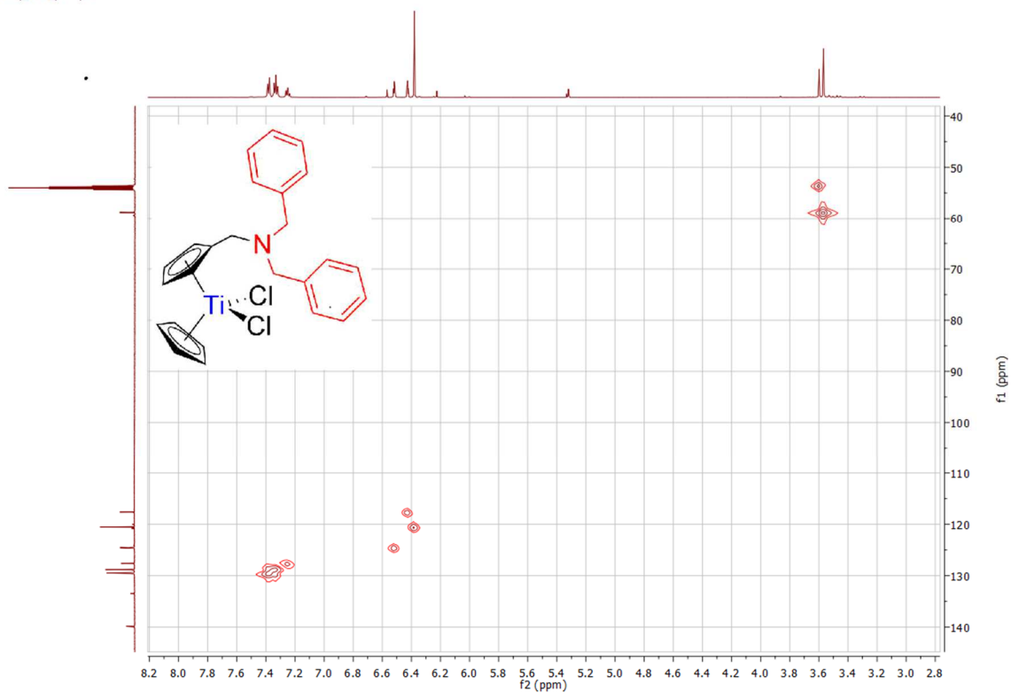
Spectrum 0-52: ^1\text{H} ^{13}\text{C} HMQC of 11 (600.23 MHz / 150.94 MHz, 300 K, dichloromethane- d_2 )
