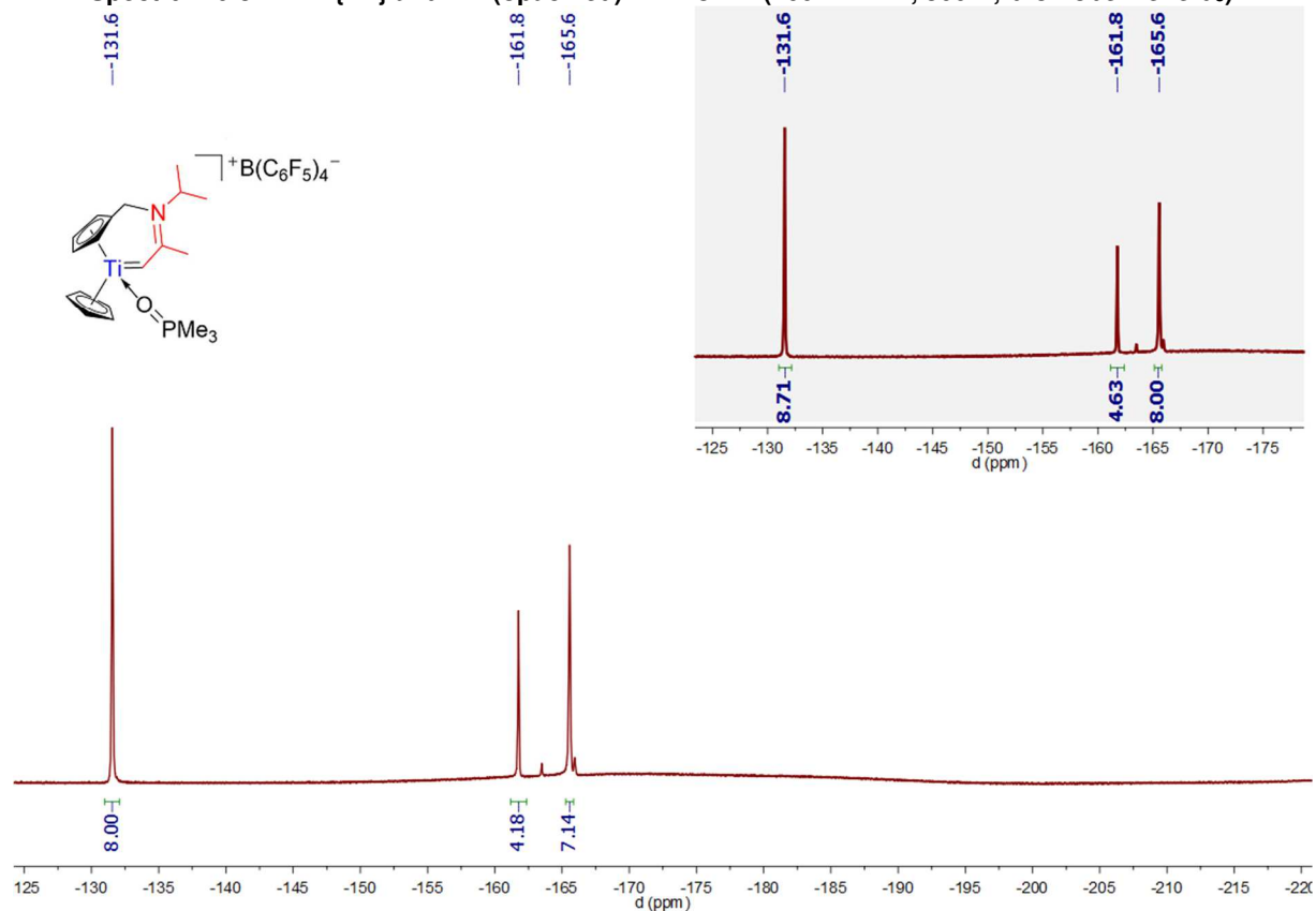
Spectrum 0-345: ^{19}\text{F}\{^1\text{H}\} and ^{19}\text{F} (opacified) NMR of 44 (470.45 MHz, 300 K, bromobenzene- d_5 )
