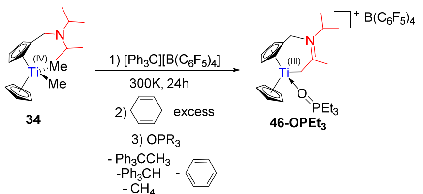
Scheme III-35: preparative scale synthesis of 46-OPEt 3
