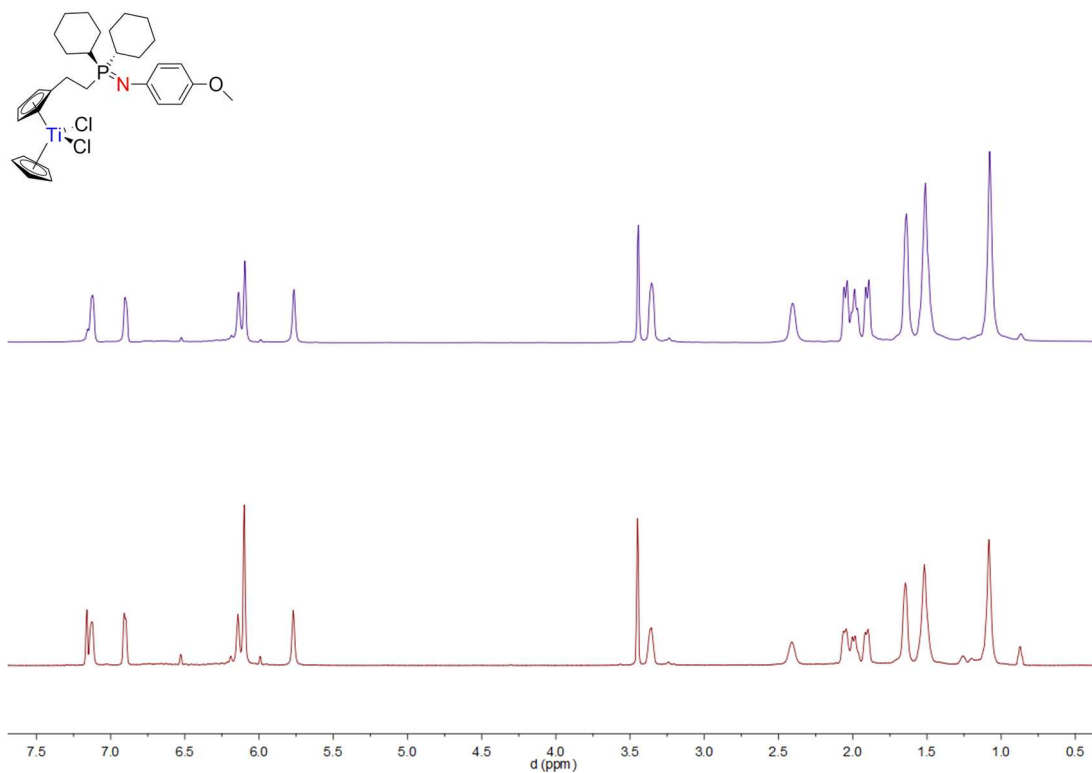
Spectrum 0-488: ^1\text{H}\{^{31}\text{P}\} NMR (top) correlated with ^1\text{H} NMR (bottom) of 59 (500.03 MHz, 300 K, benzene- d_6 )
