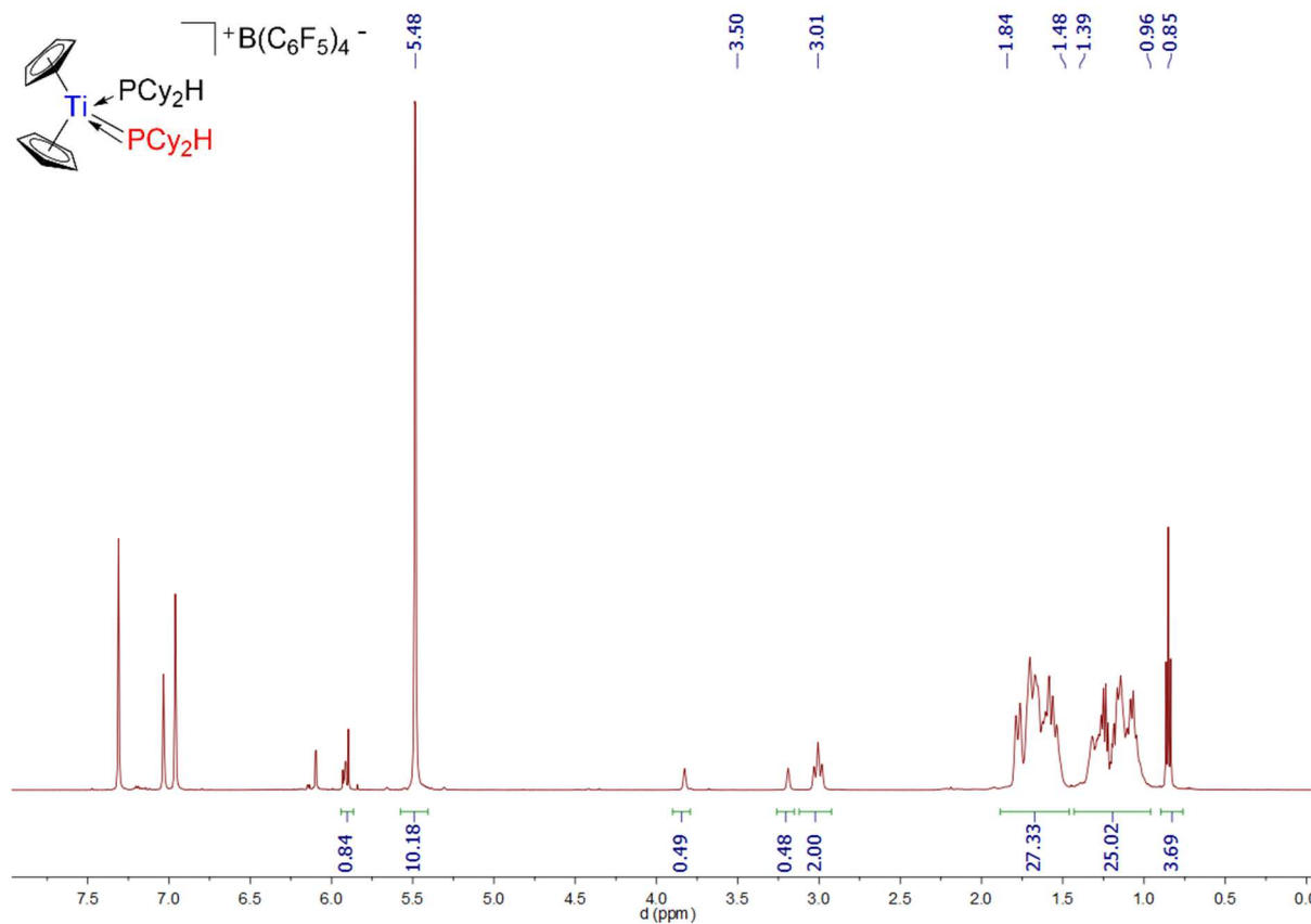
Spectrum 0-388: 1 H NMR of 51 (500.03 MHz, 300 K, bromobenzene-d 5 )
