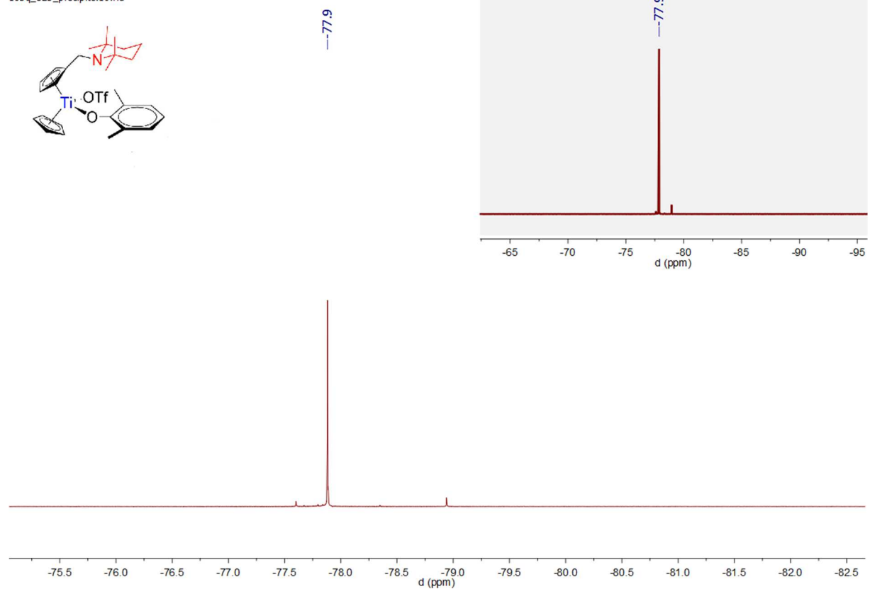
Spectrum 0-218: ^{19}\text{F}\{^1\text{H}\} and ^{19}\text{F} (σρχιφιδ) NMR of 30 (470.45 MHz, 300 K, dichloromethane- d_2 )
