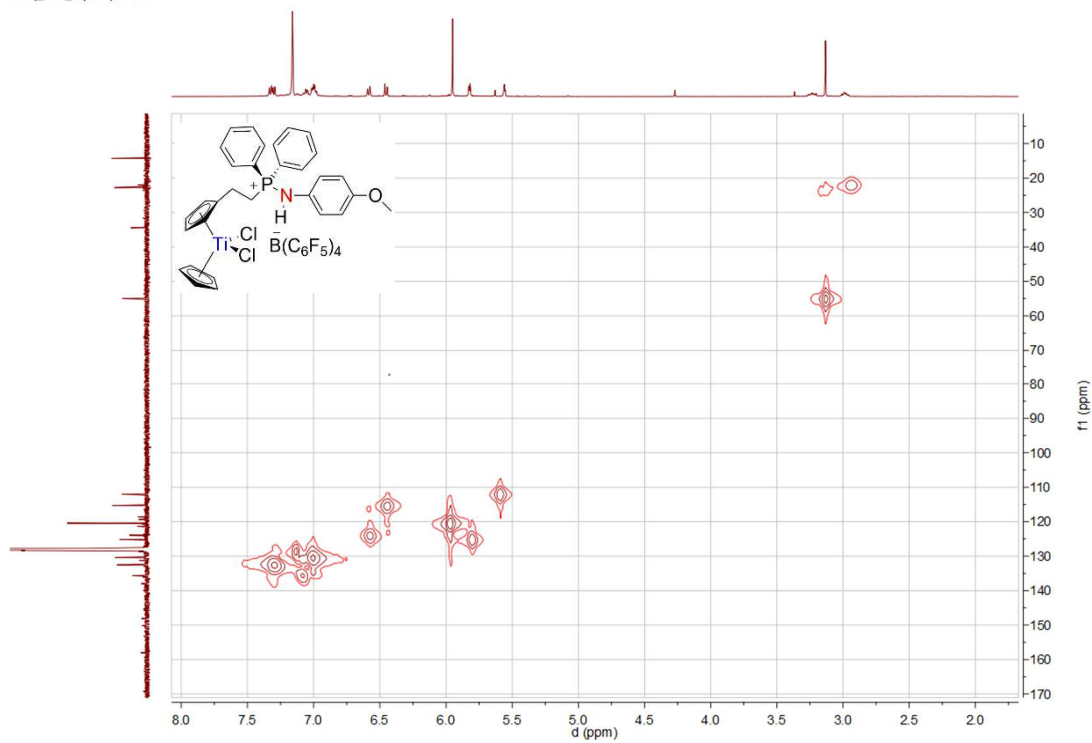
Spectrum 0-515: 1 H 13 C HMQC of 61 (500.03 MHz / 125.75 MHz, 300 K, benzene-d 6 )
