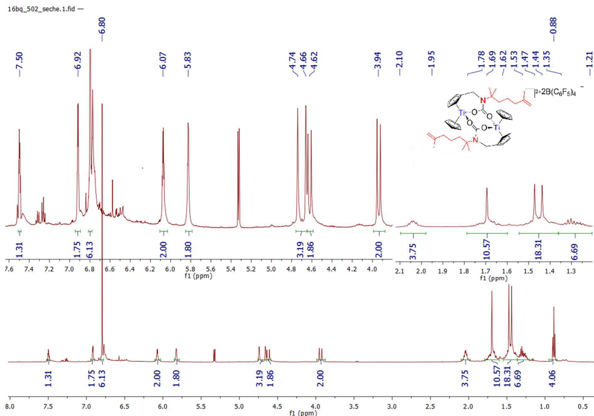
Spectrum 0-282: 1 H NMR of 39 (500.03 MHz, 300 K, dichloromethane-d 2 )
