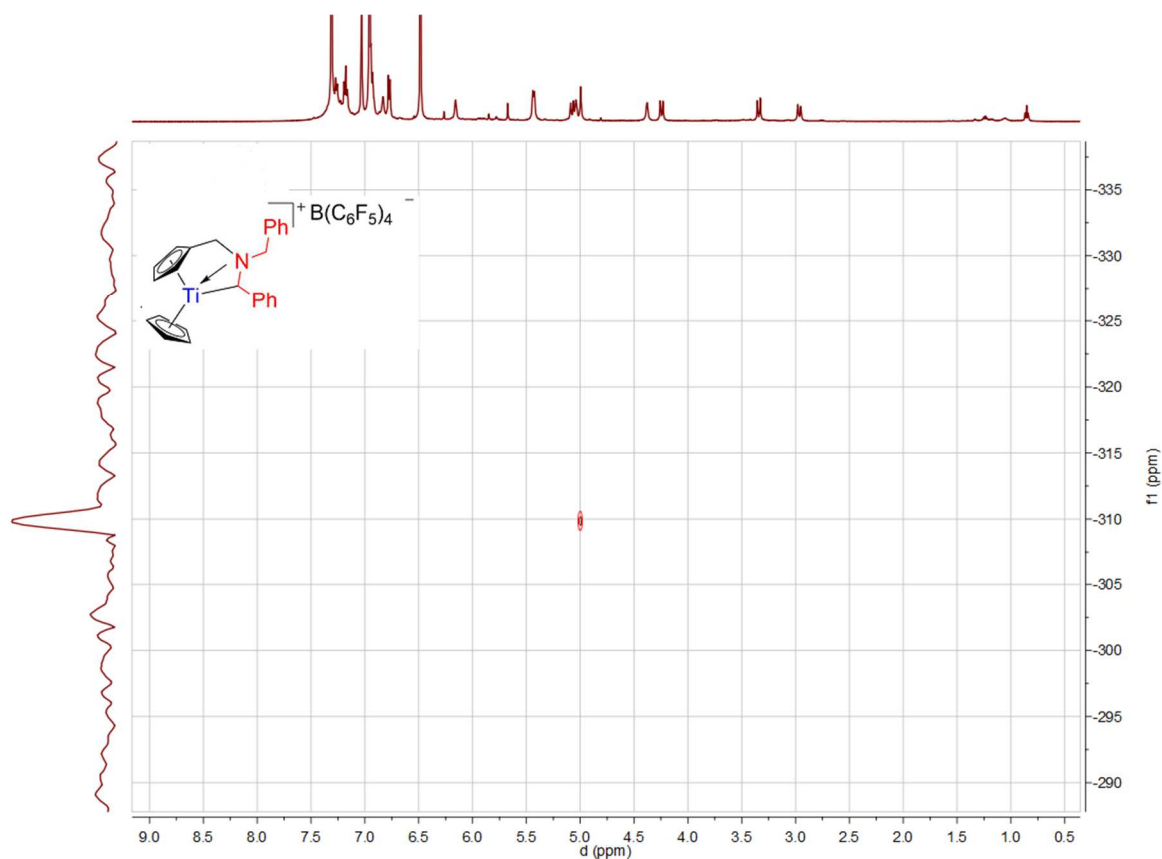
Spectrum 0-299: ^1H ^{15}N HMBC of 40 (600.23 MHz / 43.3 MHz, 300 K, bromobenzene- d_5 )
