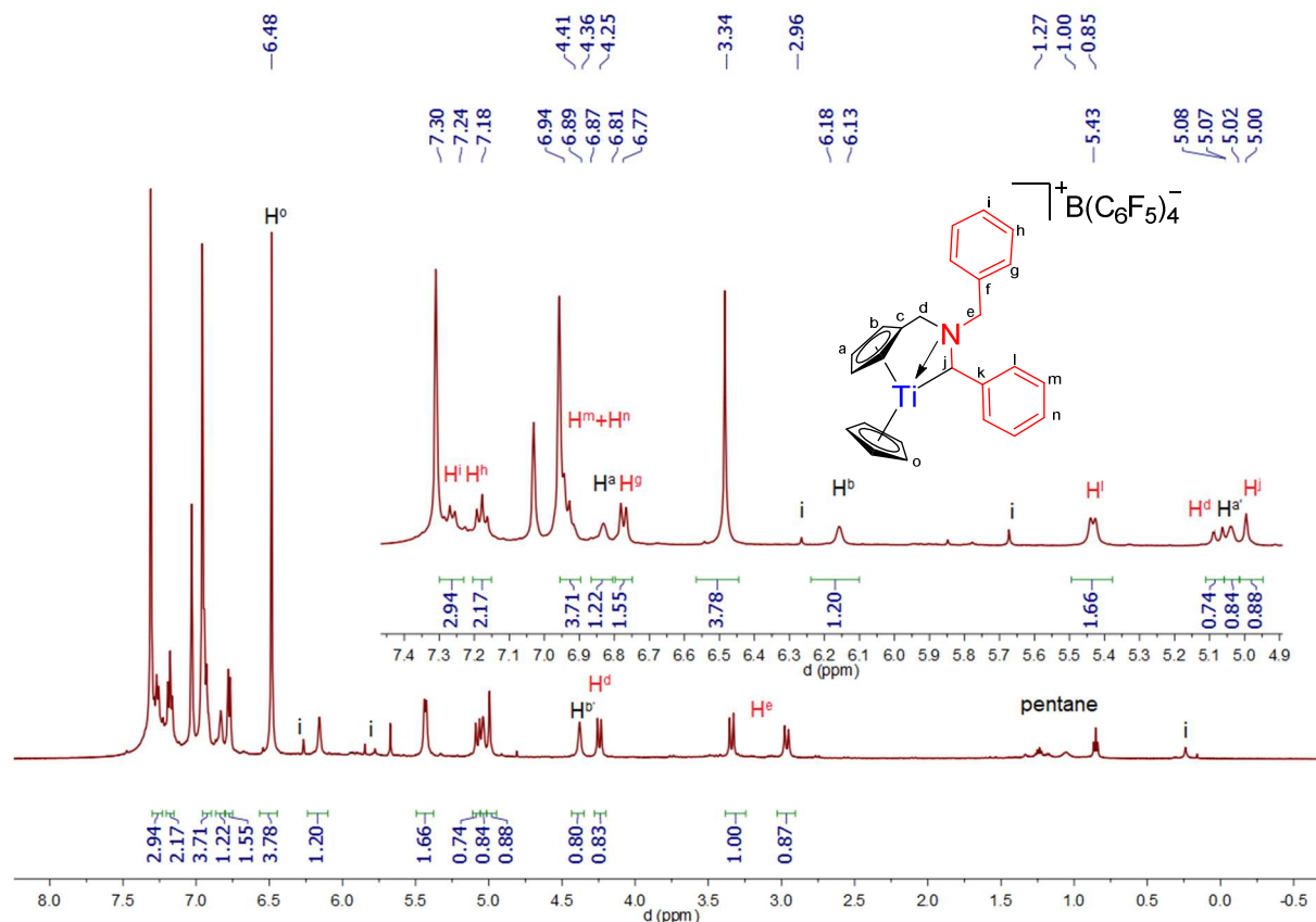
Spectrum III-9: ^1\text{H} NMR of 40 (500.03 MHz, 300 K, bromobenzene- d_5 ). ^i : unidentified impurities
