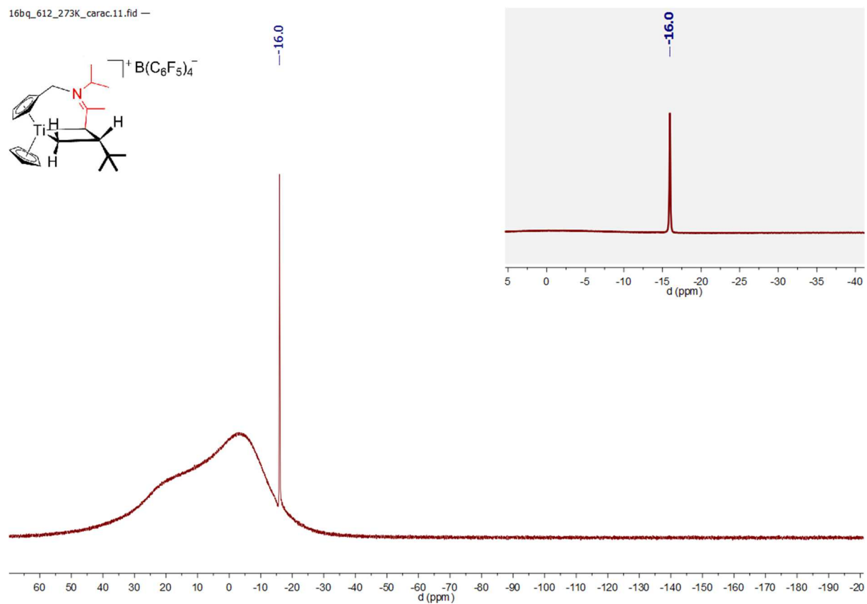
Spectrum 0-369: ^{11}\text{B}\{^1\text{H}\} and ^{11}\text{B} (opacified) NMR of 47 (160.42 MHz, 273 K, bromobenzene- d_5 )
