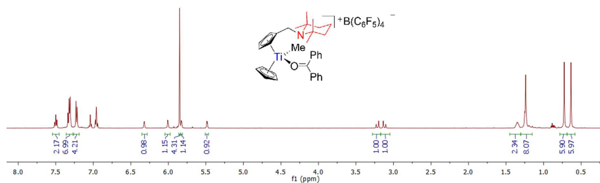
Spectrum 0-273: 1 H NMR of 38 (500.03 MHz, 263 K, bromobenzene-d 5 )
