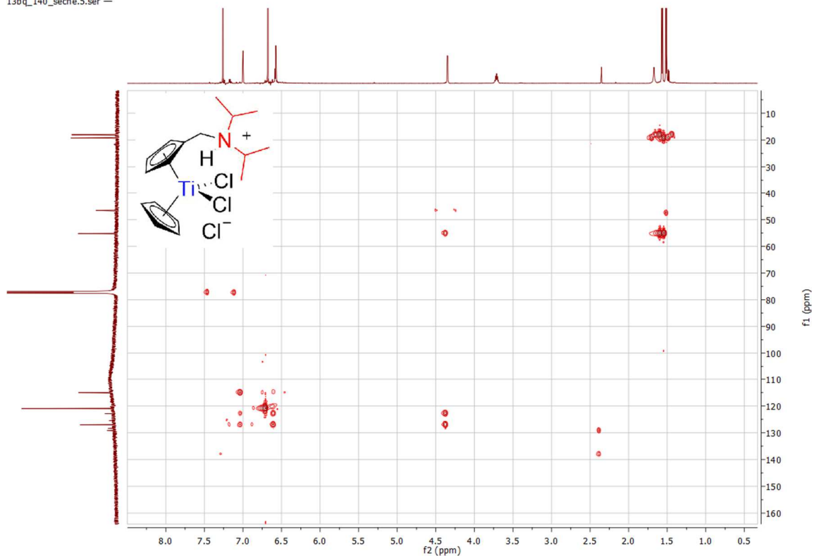
Spectrum 0-104: 1 H 13 C HMBC of 17 (600.23 MHz / 150.94 MHz, 300 K, chloroform-d 1 )
