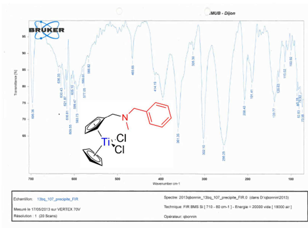
Spectrum 0-39: FIR of 9
