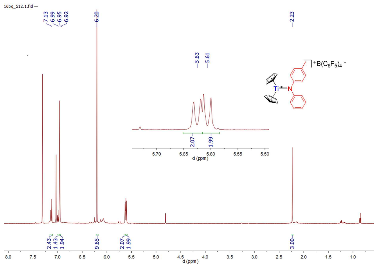
Spectrum 0-417: ^1\text{H} NMR of 54 (500.03 MHz, 300 K, bromobenzene- d_5 )
