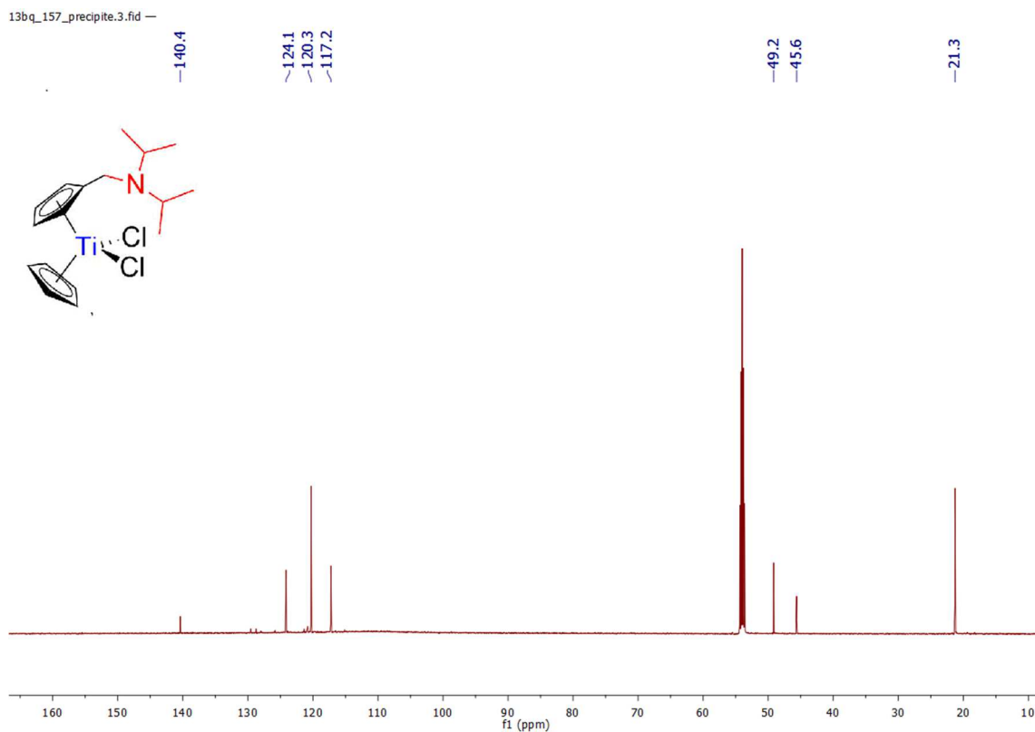
Spectrum 0-59: ^{13}\text{C}\{^1\text{H}\} NMR of 12 (150.94 MHz, 300 K, dichloromethane- d_2 )
