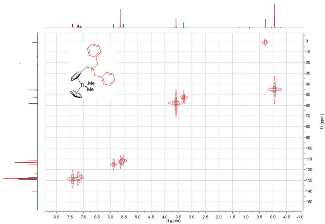
Spectrum 0-231: 1 H 13 C HMQC of 33 (500.03 MHz / 125.75 MHz, 300 K, benzene-d 6 )
