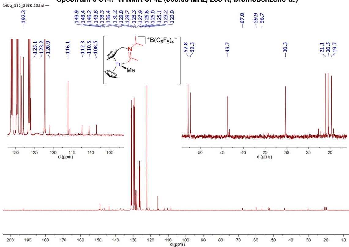
Spectrum 0-315: ^{13}\text{C}\{^1\text{H}\} NMR of 42 (125.75 MHz, 258 K, bromobenzene- d_5 )
