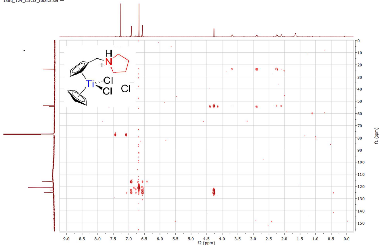
Spectrum 0-88: ^1\text{H} ^{13}\text{C} HMBC of 15 (600.23 MHz / 150.94 MHz, 300 K, chloroform- d_1 )
