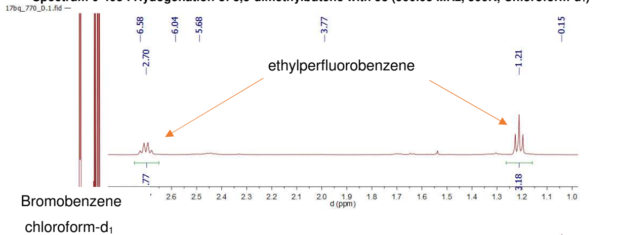
Spectrum 0-463 : Hydrogenation of 3,3-dimethylbutene with 53 (500.03 MHz, 300K, Chloroform-d 1 )
