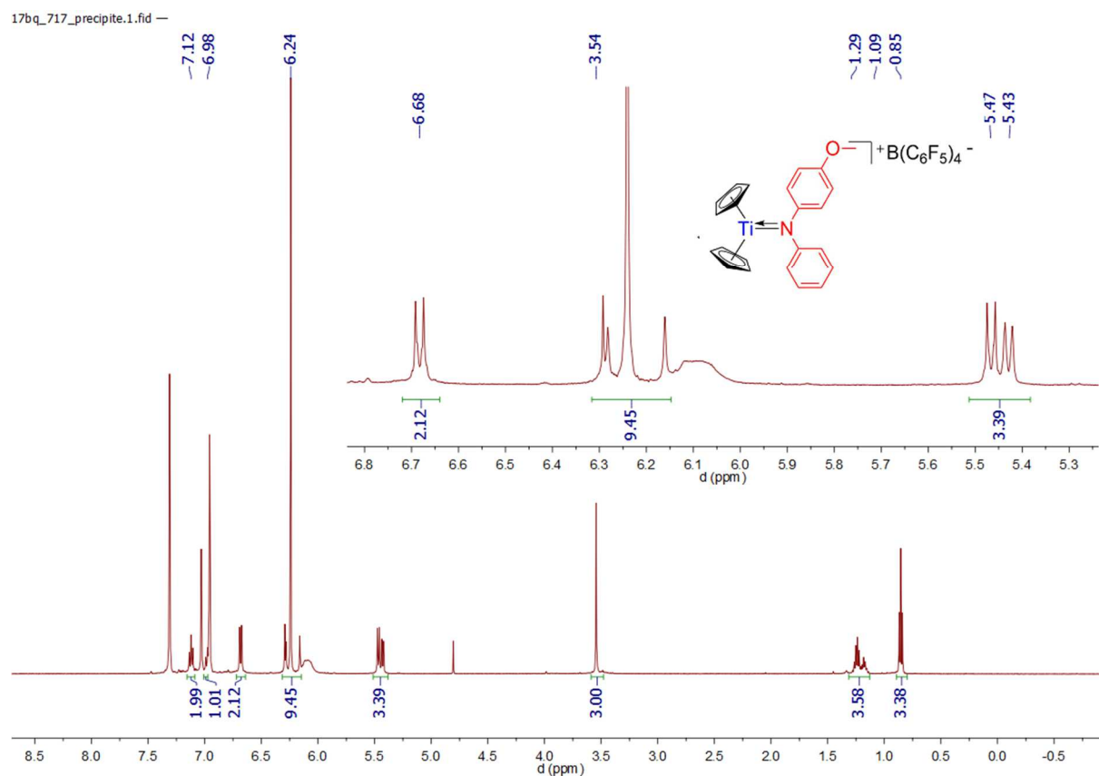
Spectrum 0-426: ^1\text{H} NMR of 55 (500.03 MHz, 300 K, bromobenzene- d_5 )
