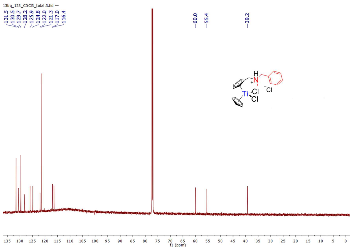
Spectrum 0-77: ^{13}\text{C}\{^1\text{H}\} NMR of 14 (150.94 MHz, 300 K, chloroform- d_1 )
