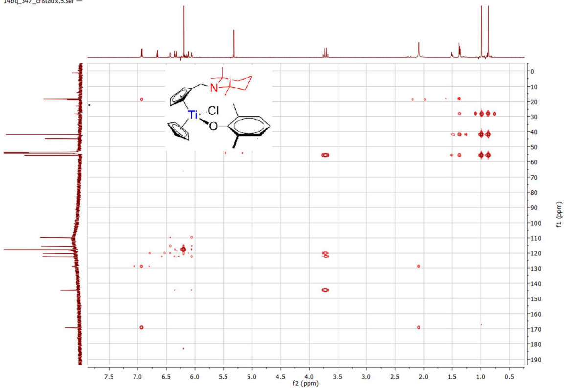
Spectrum 0-204: ^1\text{H} ^{13}\text{C} HMBC of 29 (600.23 MHz / 150.94 MHz, 300 K, dichloromethane- d_2 )
