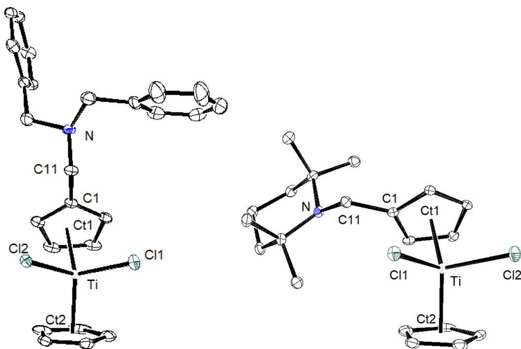
Figure II-1: ORTEP view of complex 11 (left) and 13 (right) (ellipsoids drawn at the 30% probability level, hydrogen atoms removed for clarity). Selected bond lengths (Å) and angles (°) Ct1 and Ct2 are centroids of both Cp rings as illustrated above. 11: Ct1-Ti = 2.0606(11), Ct2-Ti = 2.0598(12), Cl1-Ti = 2.3615(6), Cl2-Ti = 2.3768(6), C1-C11 = 1.494(3), C11-N = 1.481(3), Cl1-Ti-Cl2 = 93.89(2), Ct1-Ti-Ct2 = 131.12(5), C1-C11-N = 112.06(17). 13: Ct1-Ti = 2.074(2) / 2.069(2), Ct2-Ti = 2.061(2) / 2.064(2), Cl1-Ti = 2.3613(14) / 2.3539(14), Cl2-Ti = 2.3790(13) / 2.3718(13), C1-C11 = 1.509(6) / 1.508(6), C11-N = 1.468(5) / 1.470(5), Cl1-Ti-Cl2 = 94.05(5) / 94.26(5), Ct1-Ti-Ct2 = 131.39(9) / 131.73 (10), C1-C11-N = 113.9(4) / 112.3(4).
