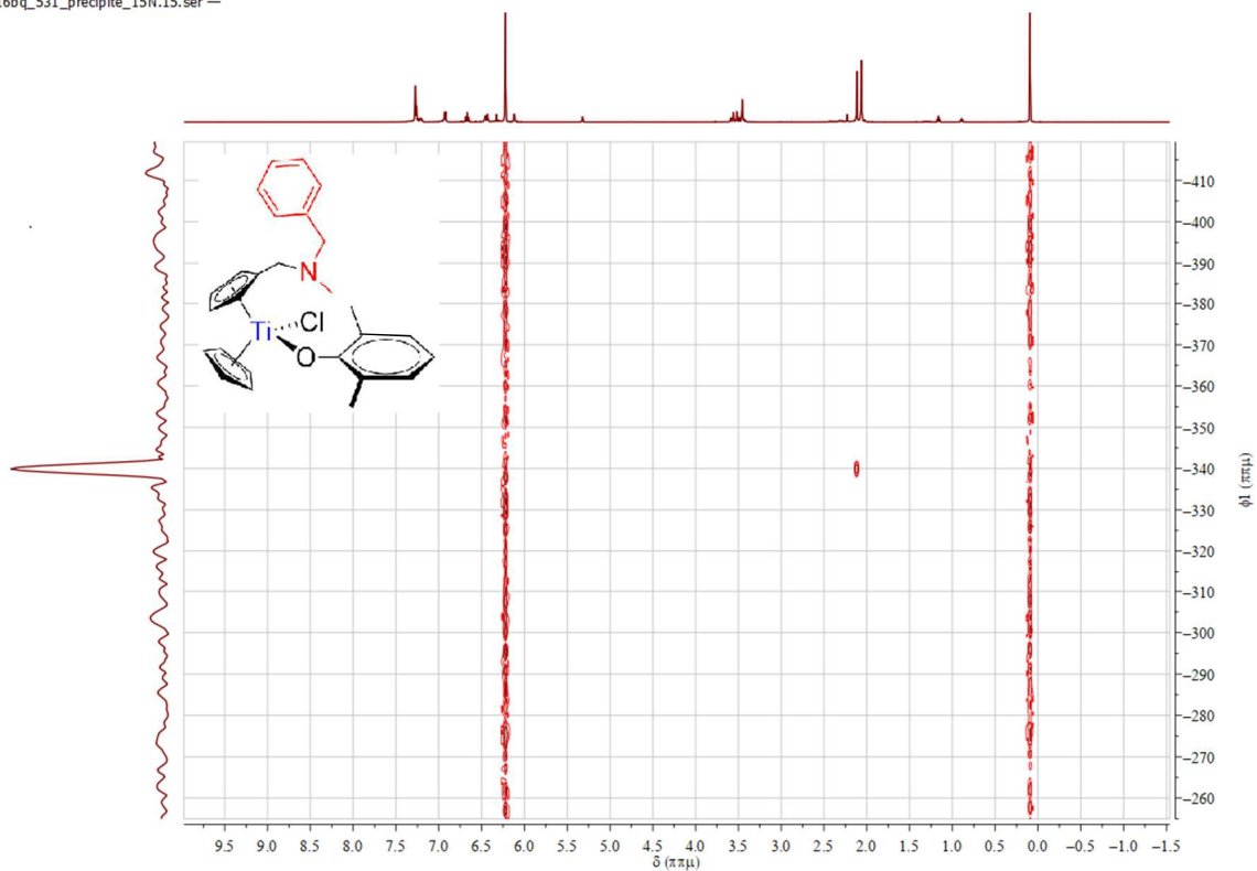
Spectrum 0-180: 1 H 15 N HMBC of 26 (600.23 MHz / 43.3 MHz, 300 K, dichloromethane-d 2 )
