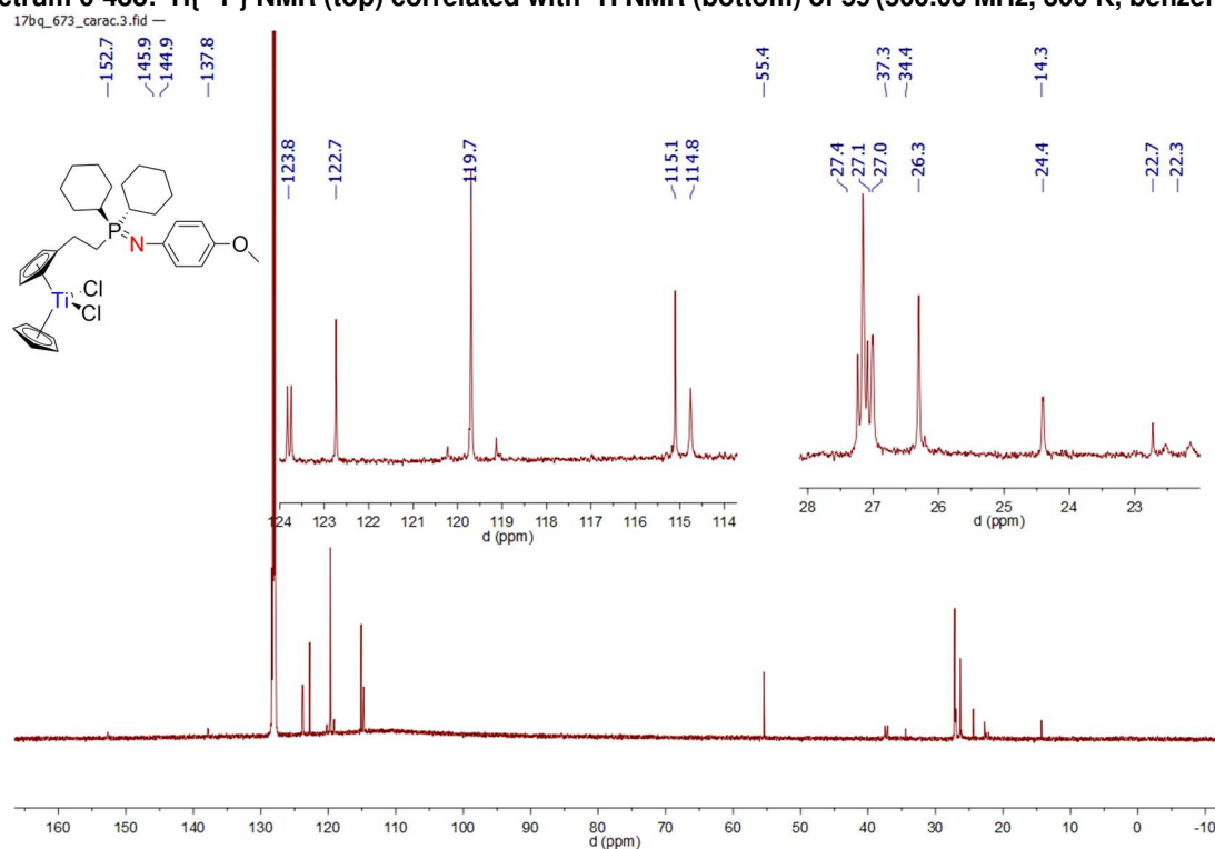
Spectrum 0-489: ^{13}\text{C}\{^1\text{H}\} NMR of 59 (125.75 MHz, 300 K, benzene- d_6 )
