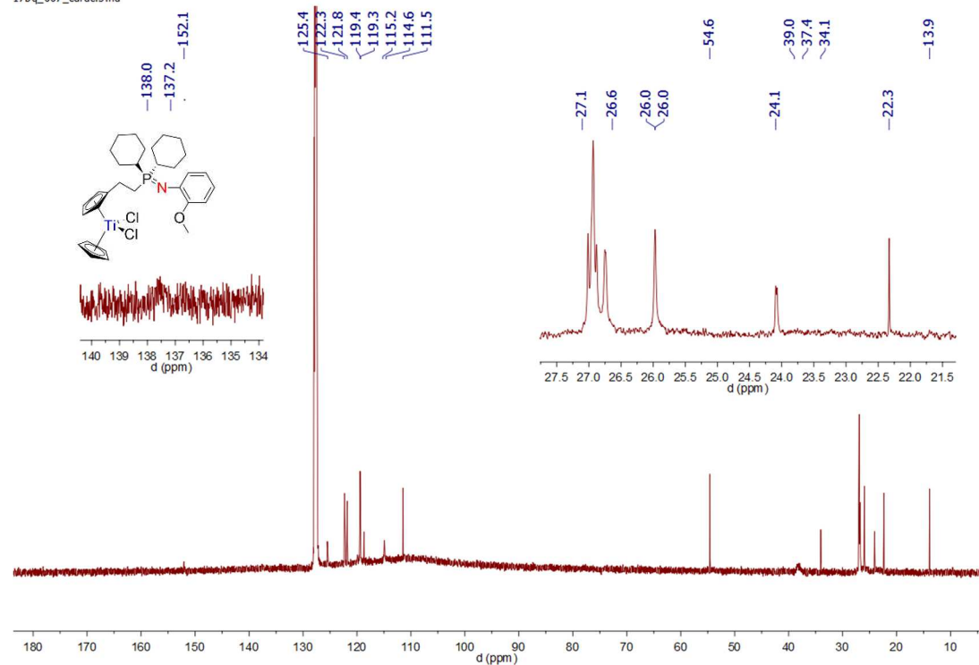
Spectrum 0-501: ^{13}\text{C}\{^1\text{H}\} NMR of 60 (150.94 MHz, 300 K, benzene- d_6 )
