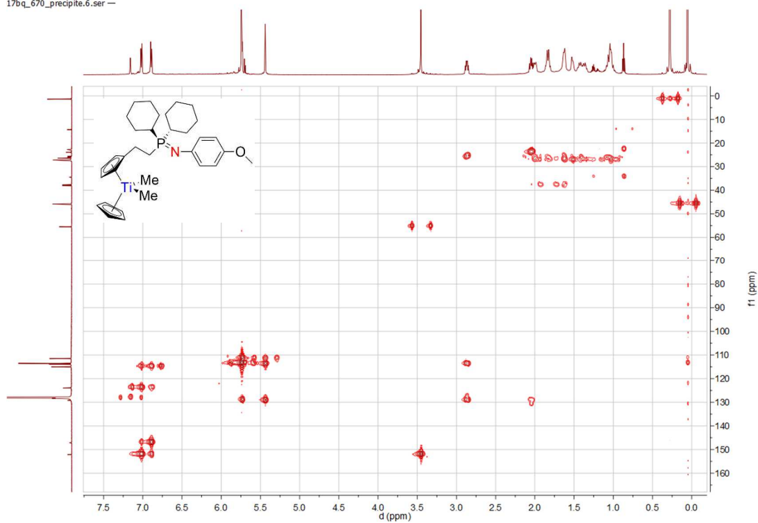
Spectrum 0-538: 1 H 13 C HMBC of 63 (600.23 MHz / 150.86 MHz, 300 K, benzene-d 6 )
