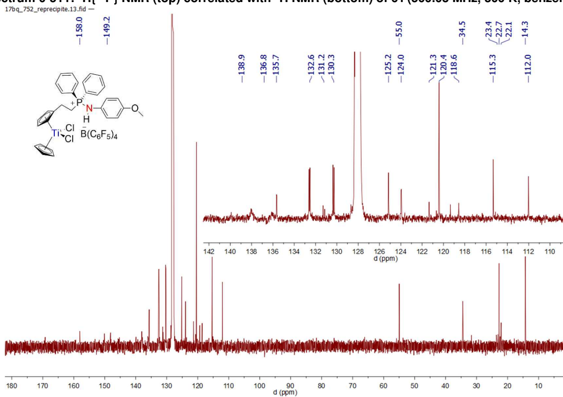
Spectrum 0-512: ^{13}\text{C}\{^1\text{H}\} NMR of 61 (125.75 MHz, 300 K, benzene- d_6 )
