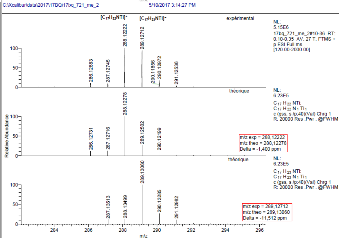
Spectrum 0-360: HRMS of 45 (Positive mode ESI, bromobenzene)
