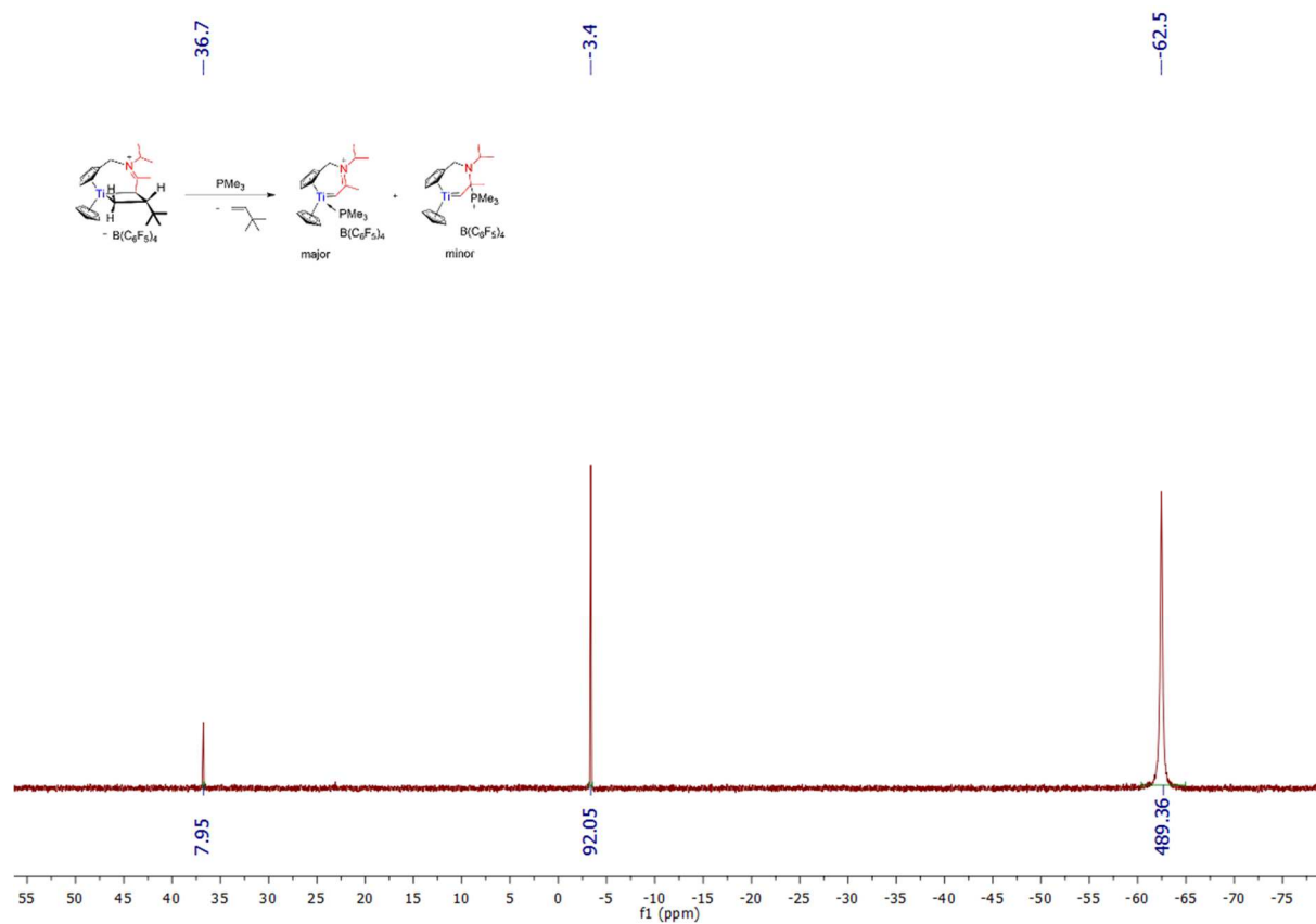
Spectrum 0-376: ^{31}\text{P}\{^1\text{H}\} NMR of 48 (243.0 MHz, 300 K, bromobenzene- d_5 )
