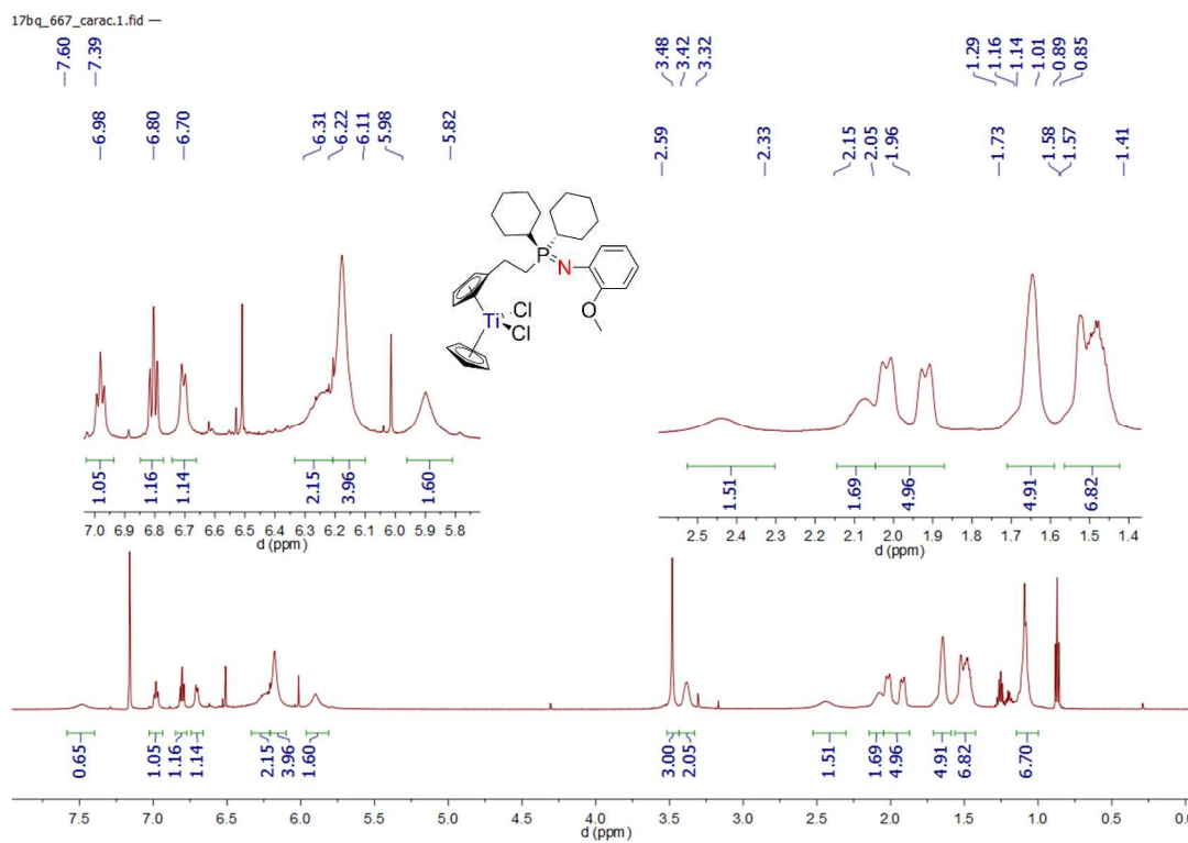
Spectrum 0-499: ^1\text{H} NMR of 60 (600.23 MHz, 300 K, benzene- d_6 )
