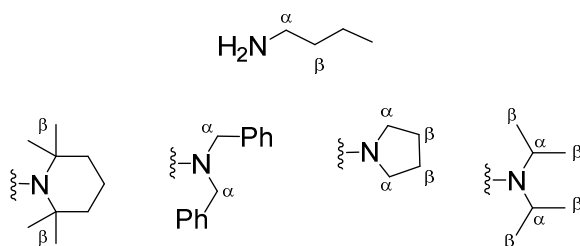
Scheme III-26: nomenclature used with amines
