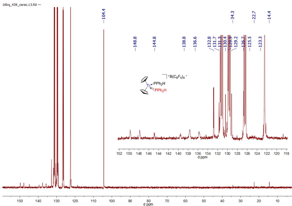
Spectrum 0-379: 13 C{ 1 H} NMR of 50 (125.75 MHz, 300 K, bromobenzene-d 5 )
