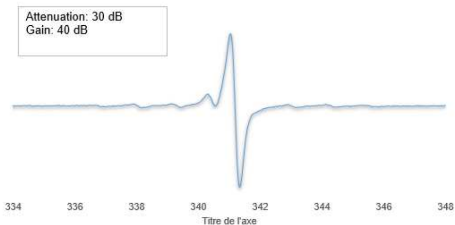
Spectrum 0-457: EPR spectrum of 54 after irradiation (9.435437, 295 K, THF)
