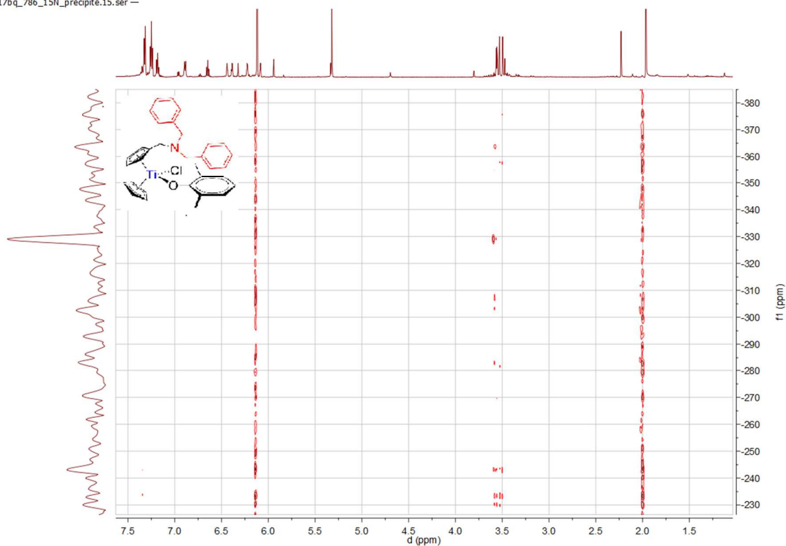
Spectrum 0-187: ^1\text{H} ^{15}\text{N} HMBC of 27 (600.23 MHz / 60.83 MHz, 300 K, dichloromethane- d_2 )
