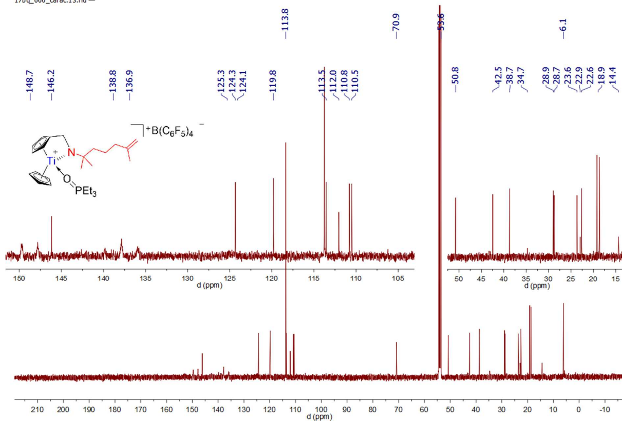
Spectrum 0-264: ^{13}\text{C}\{^1\text{H}\} NMR of 37 (125.75 MHz, 300 K, dichloromethane- d_2 )
