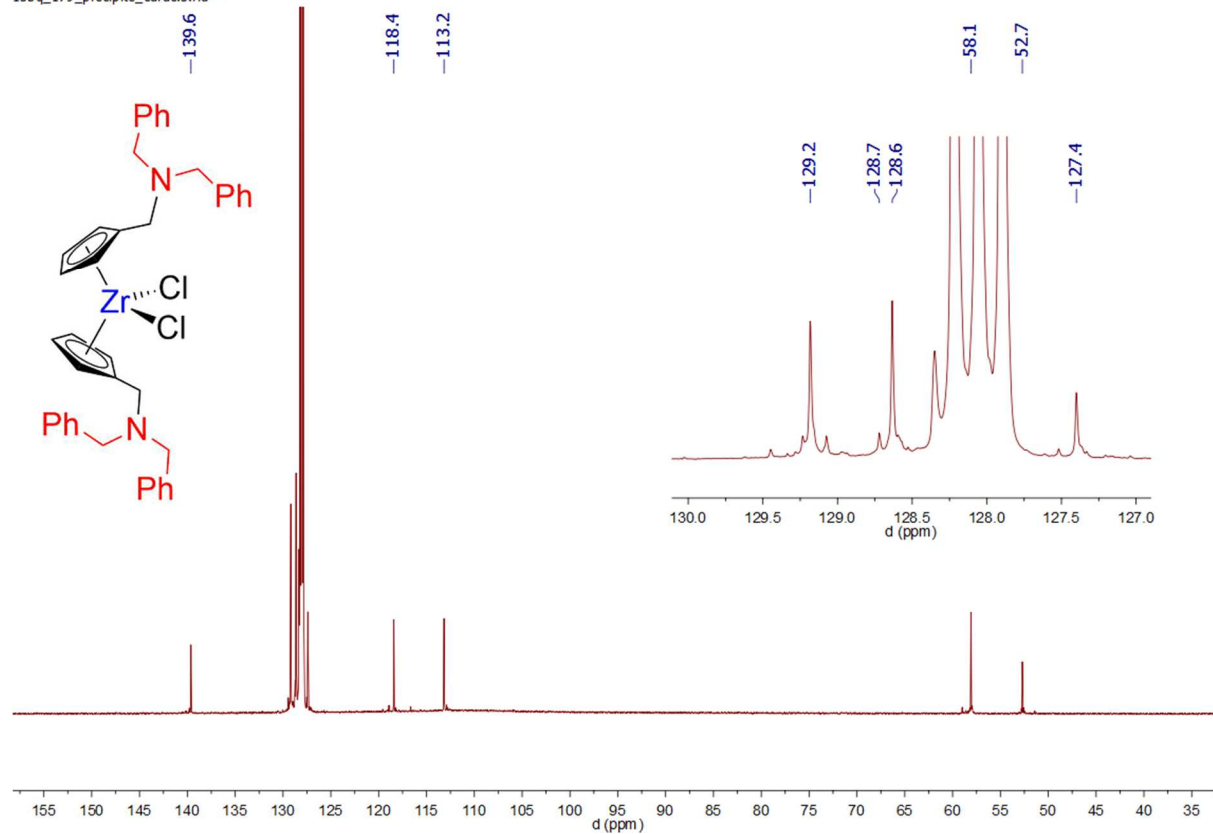
Spectrum 0-142: 13 C{ 1 H} NMR of 22 (150.94 MHz, 300 K, benzene-d 6 )
