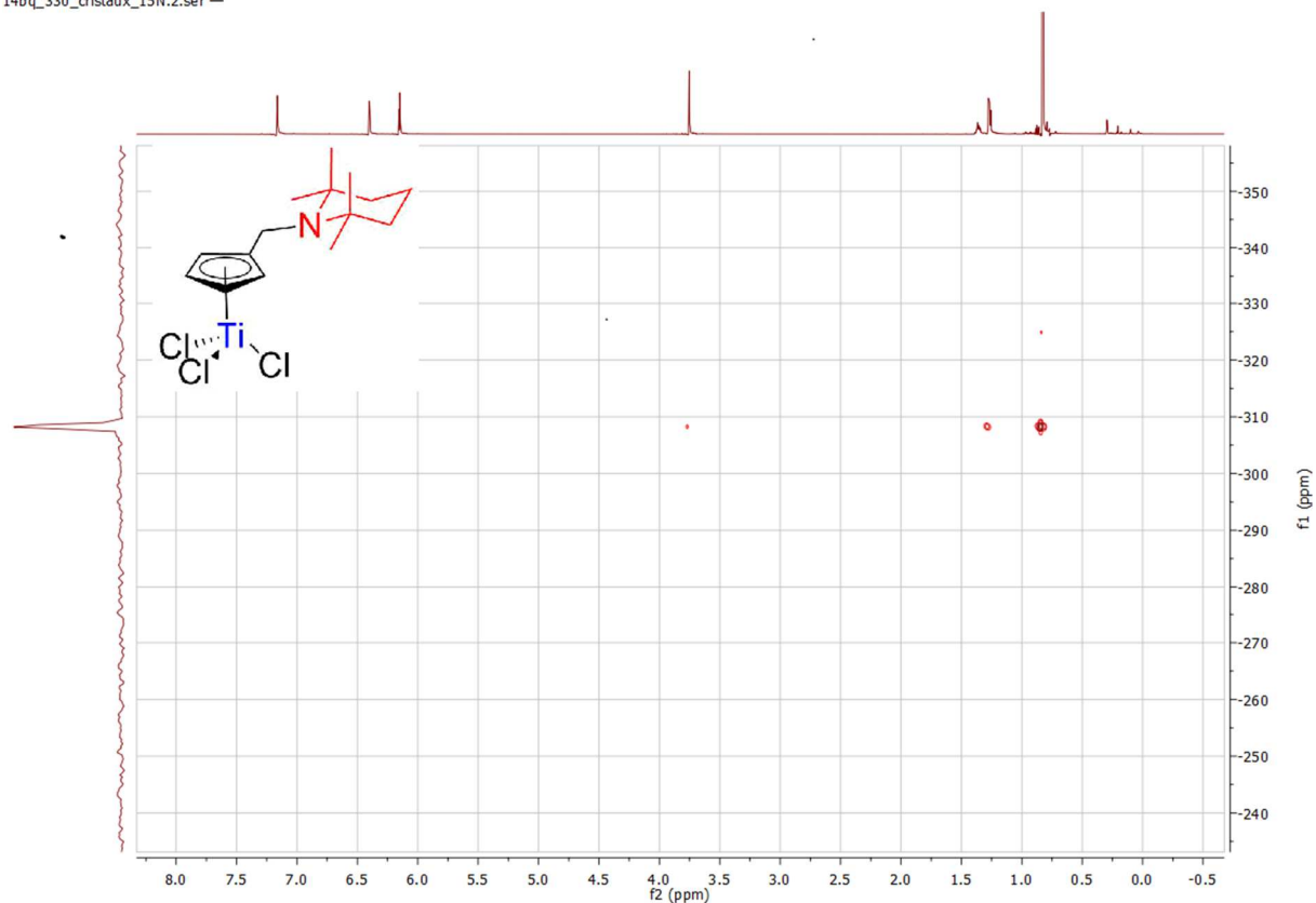
Spectrum 0-137: ^1\text{H} ^{15}\text{N} HMBC of 21 (600.23 MHz / 43.3 MHz, 300 K, benzene- d_6 )
