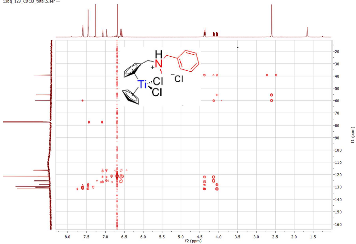
Spectrum 0-80: ^1\text{H} ^{13}\text{C} HMBC of 14 (600.23 MHz / 150.94 MHz, 300 K, chloroform- d_1 )
