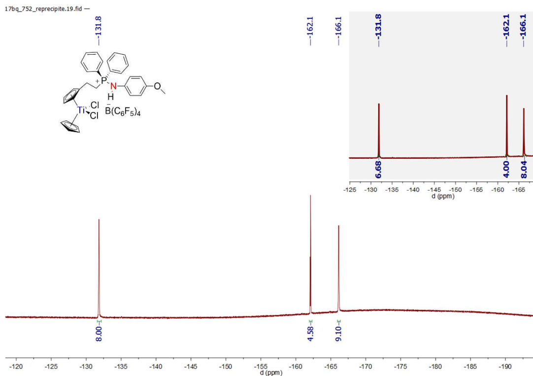
Spectrum 0-519: ^{19}\text{F}\{^1\text{H}\} and ^{19}\text{F} NMR(opacified) of 61 (470.45 MHz, 300 K, bromobenzene- d_5 )
