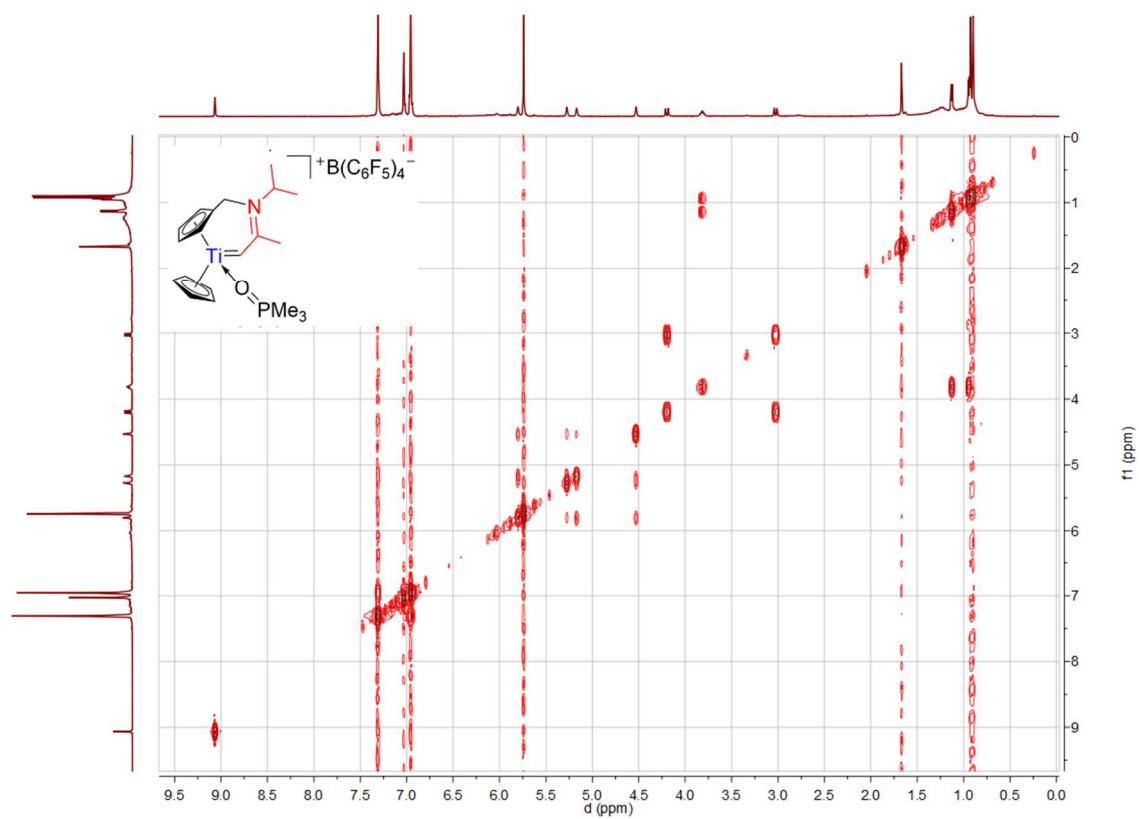
Spectrum 0-340: ^1\text{H} ^1\text{H} COSY of 44 (500.03 MHz, 300 K, bromobenzene- \text{d}_5 )
