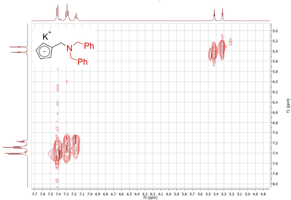
Spectrum 0-15: ^1\text{H} ^1\text{H} COSY of 3-K (500.03 MHz, 300 K, dimethylsulfoxide- \text{d}_6 )
