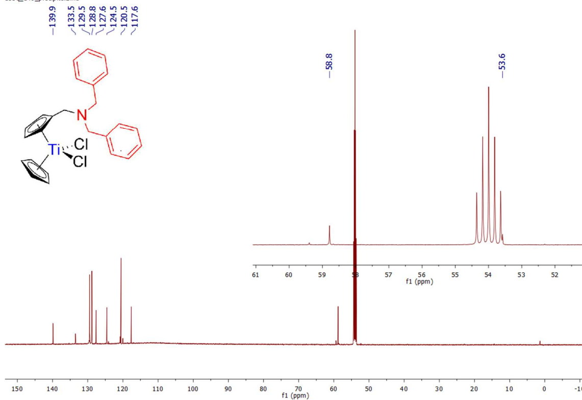
Spectrum 0-50: ^{13}\text{C}\{^1\text{H}\} NMR of 11 (150.94 MHz, 300 K, dichloromethane- d_2 )
