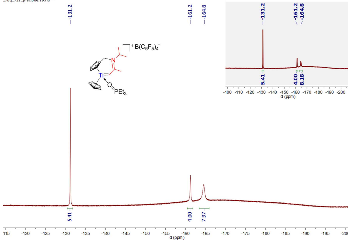
Spectrum 0-357: ^{19}\text{F}\{^1\text{H}\} and ^{19}\text{F} (opacified) NMR of 45 (470.45 MHz, 300 K, bromobenzene- d_5 )
