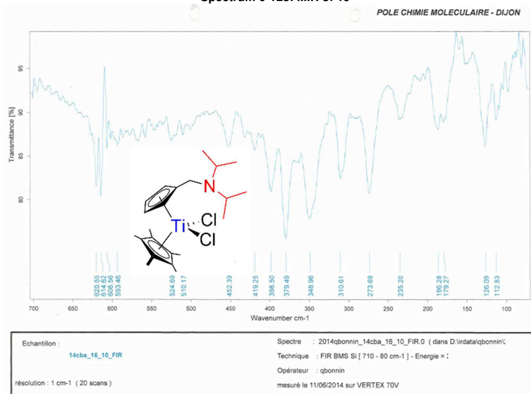
Spectrum 0-123: MIR of 19
