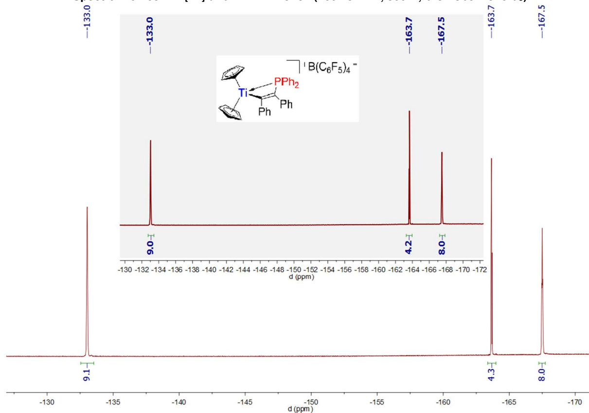
Spectrum 0-406: ^{19}\text{F}\{^1\text{H}\} and ^{19}\text{F} NMR of 52 (470.45 MHz, 300 K, bromobenzene- d_5 )
