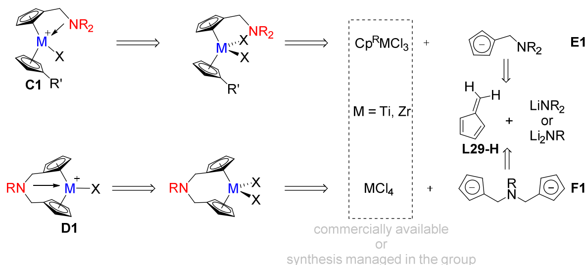
Scheme II-3: retrosynthetic scheme envisaged initially for the synthesis of aminomethyl-group 4-metallocenes
