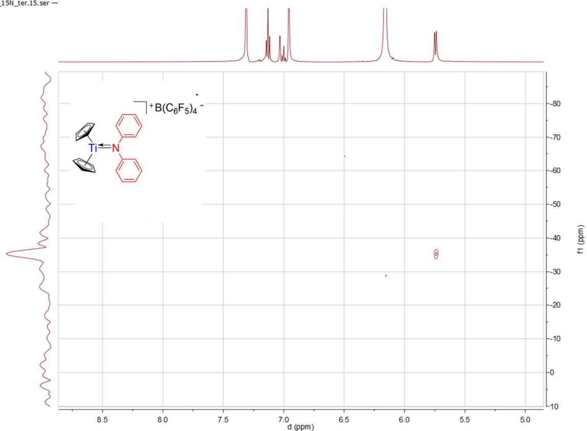
Spectrum 0-413: 1 H 15 N HMBC of 53 (500.03 MHz / 43.3 MHz, 300 K, bromobenzene-d 5 )
