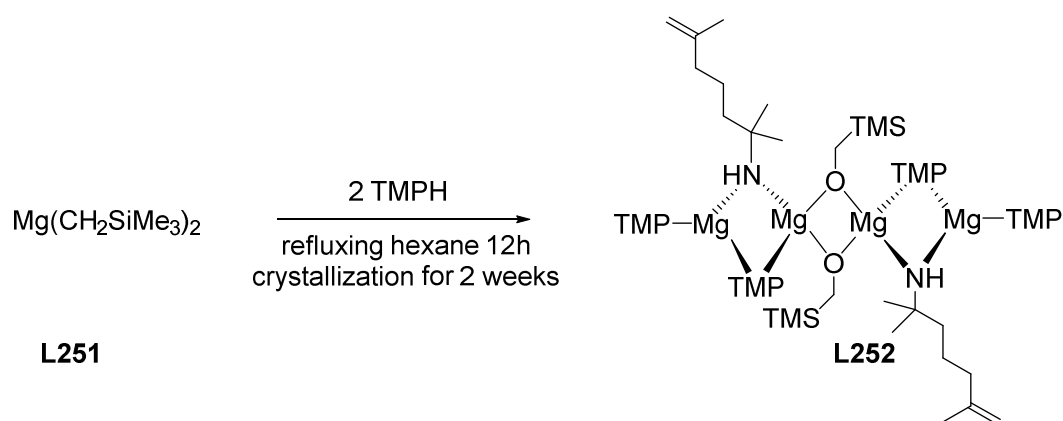
Scheme III-15: ring opening of TMP by a magnesium complex
