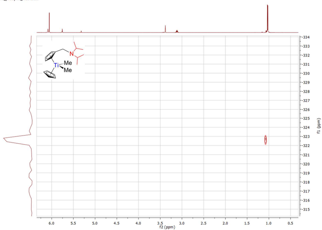
Spectrum 0-240: 1 H 15 N HMBC of 34 (600.23 MHz / 43.3 MHz, 300 K, dichloromethane-d 2 )
