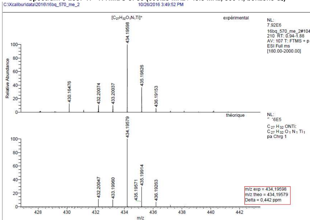
Spectrum 0-234: HRMS of 33 (Positive mode ESI, dichloromethane)
