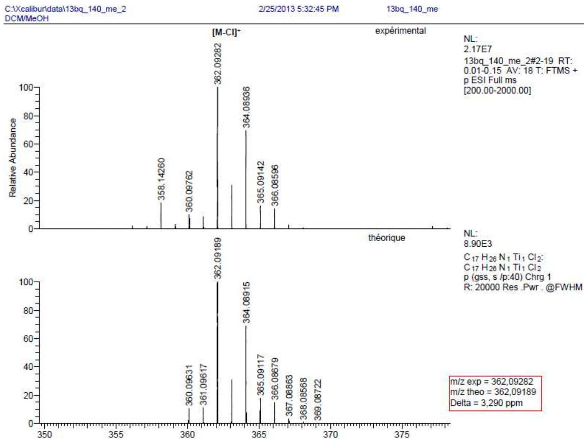
Spectrum 0-105: HRMS of 17 (Positive mode ESI, dichloromethane-methanol)
