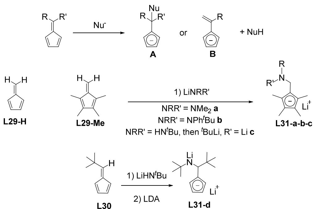
Scheme I-12: reactivity of fulvenes
