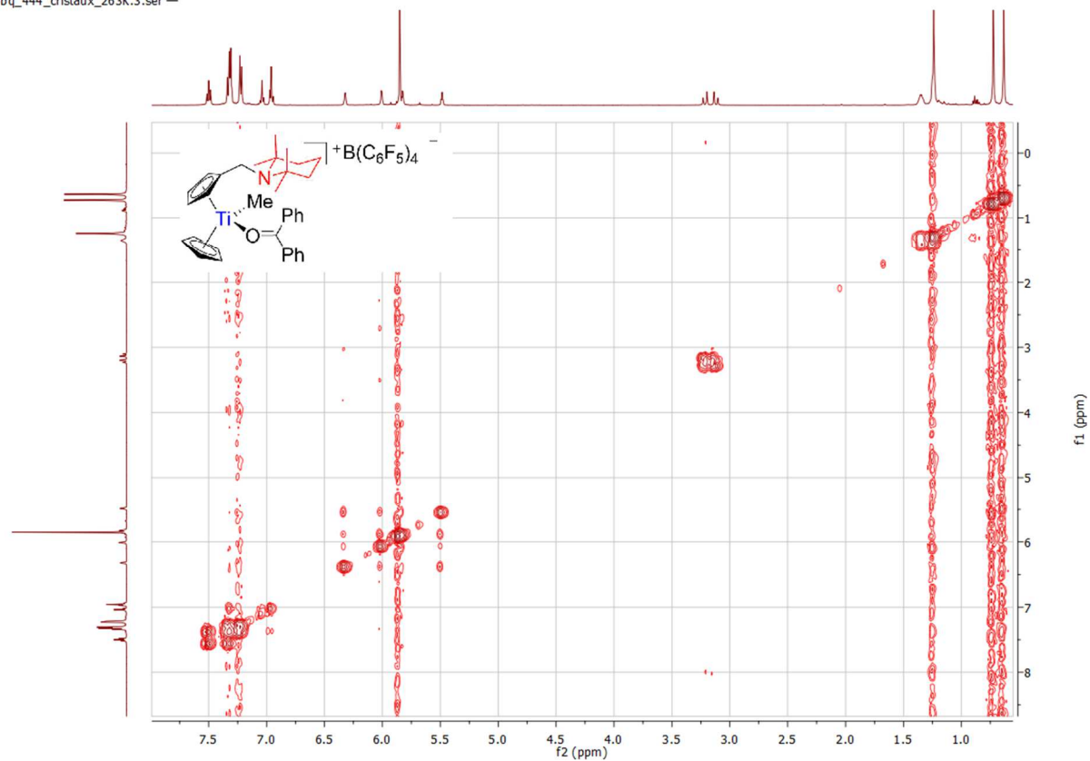
Spectrum 0-275: ^1\text{H} ^1\text{H} COSY of 38 (500.03 MHz, 263 K, bromobenzene- d_5 )
