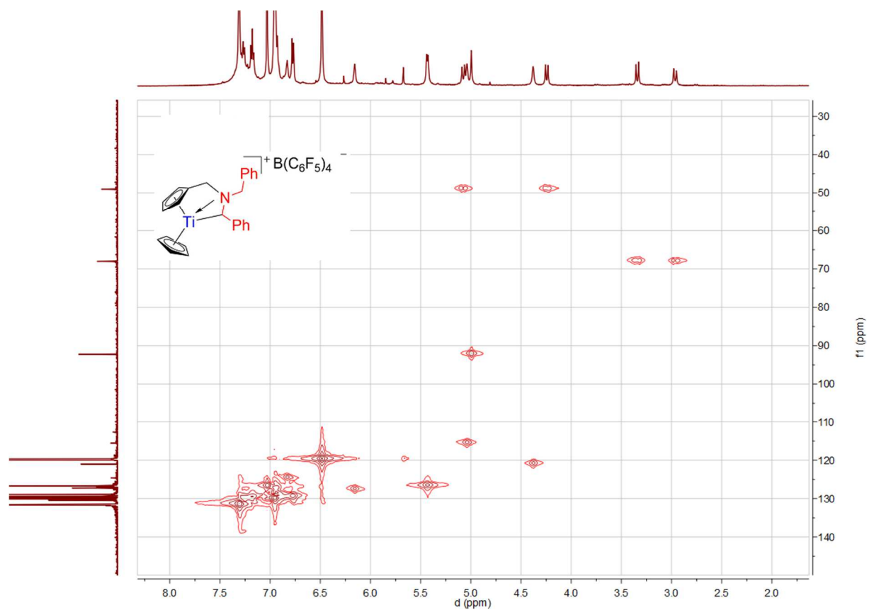
Spectrum 0-295: ^1\text{H} ^{13}\text{C} HMQC of 40 (500.03 MHz / 125.75 MHz, 300 K, bromobenzene- d_5 )
