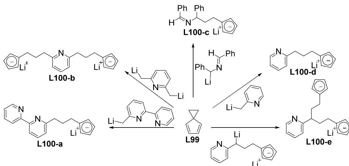
Scheme I-33: synthesis of (aminoalkyl)cyclopentadienides via the spirane route
