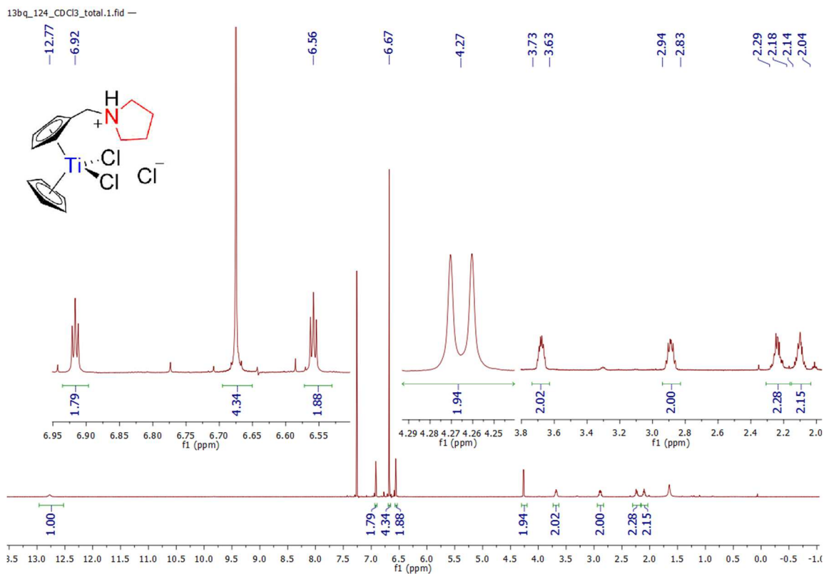
Spectrum 0-84: ^1\text{H} NMR of 15 (600 MHz, 300 K, chloroform- d_1 )
