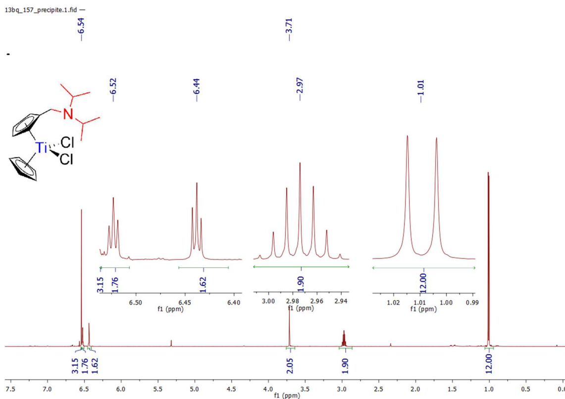
Spectrum 0-58: ^1\text{H} NMR of 12 (600.23 MHz, 300 K, dichloromethane- d_2 )
