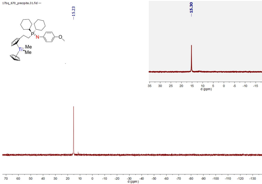
Spectrum 0-539: ^{31}\text{P}\{^1\text{H}\} and ^{31}\text{P} (opacified) NMR of 63 (202.46 MHz, 300 K, benzene- d_6 )
