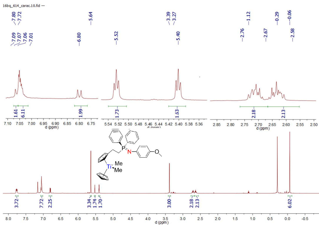
Spectrum 0-522: ^1\text{H} NMR of 62 (500.03 MHz, 300 K, benzene- d_6 )
