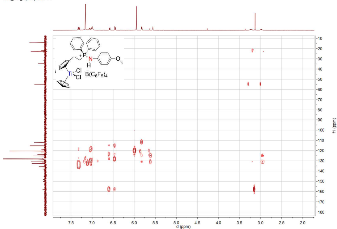
Spectrum 0-516: 1 H 13 C HMBC of 61 (500.03 MHz / 125.75 MHz, 300 K, benzene-d 6 )
