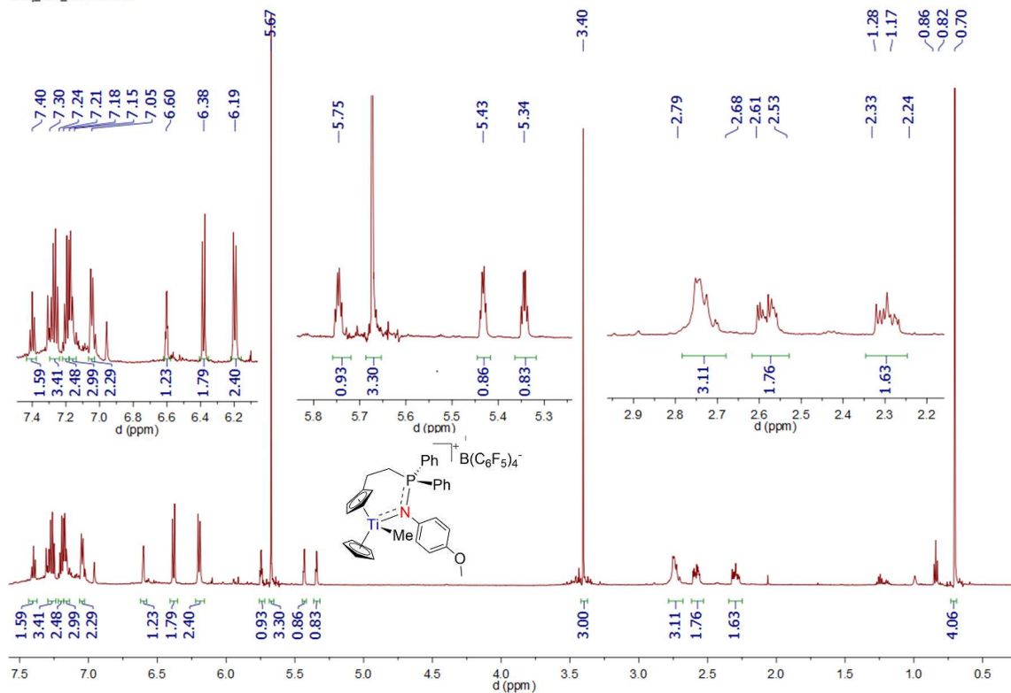
Spectrum 0-548: ^1\text{H}\{^{31}\text{P}\} NMR of 64 (600.23 MHz, 360 K, bromobenzene- d_5 )
