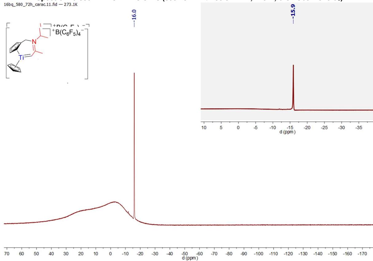
Spectrum 0-331: 11 B{ 1 H} and 11 B(opacified) NMR of 43 (160.42 MHz, 273 K, bromobenzene-d 5 )
