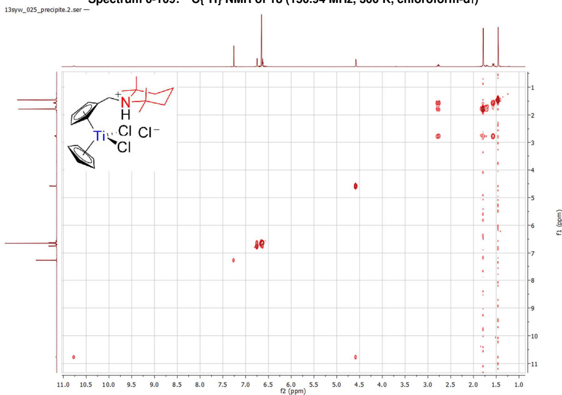
Spectrum 0-110: ^1\text{H} ^1\text{H} COSY of 18 (600.23 MHz, 300 K, chloroform- d_1 )
