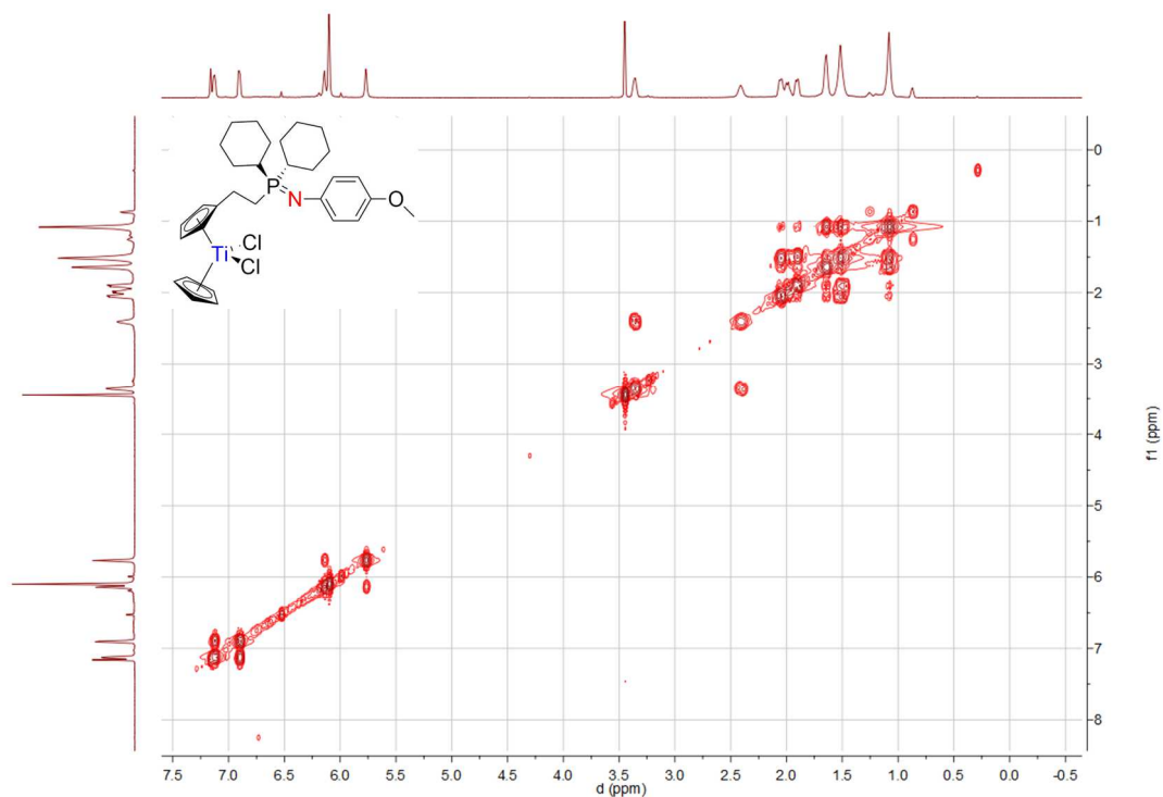
Spectrum 0-490: 1 H 1 H COSY of 59 (500.03 MHz, 300 K, 273 K, benzene-d 6 )
