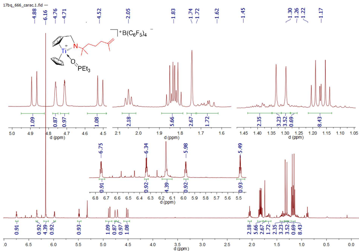
Spectrum 0-262: 1 H NMR of 37 (500.03 MHz, 300 K, dichloromethane-d 2 )
