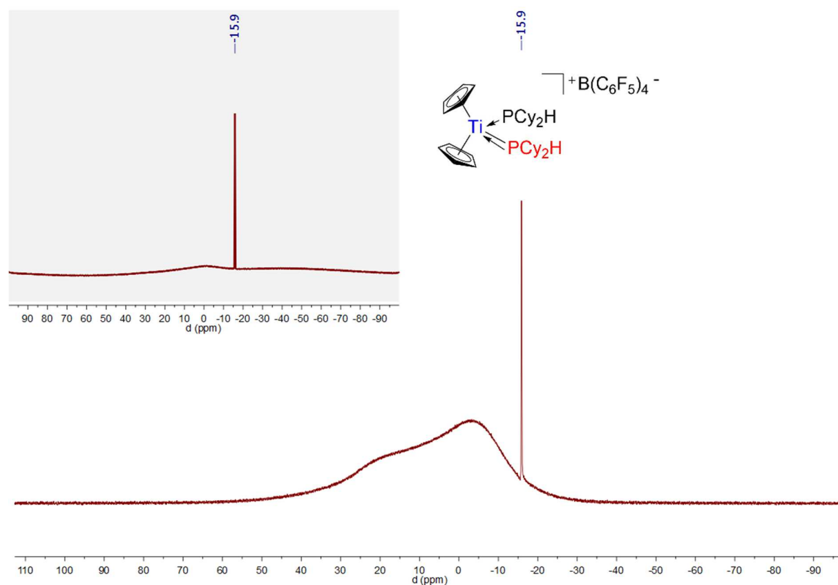
Spectrum 0-395: ^{11}\text{B}\{^1\text{H}\} and ^{11}\text{B} NMR of 51 (160.43 MHz, 300 K, bromobenzene- \text{d}_5 )
