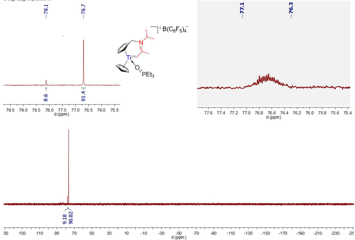
Spectrum 0-355: 31 P{ 1 H} and 31 P (opacified) NMR of 45 (202.46 MHz, 300 K, bromobenzene-d 5 )
