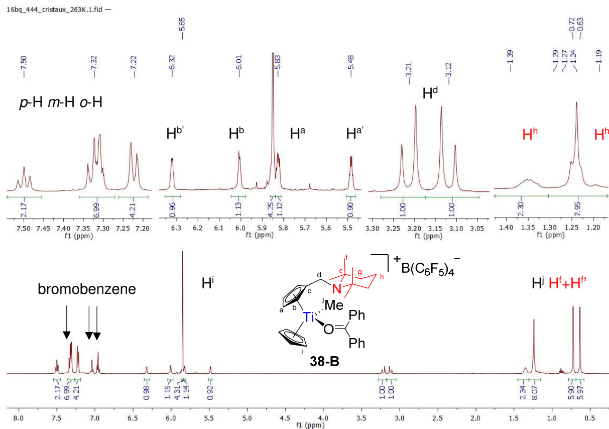
Spectrum III-8: ^1\text{H} NMR of 38-B (500.03 MHz, 263 K, bromobenzene- \text{d}_5 )
