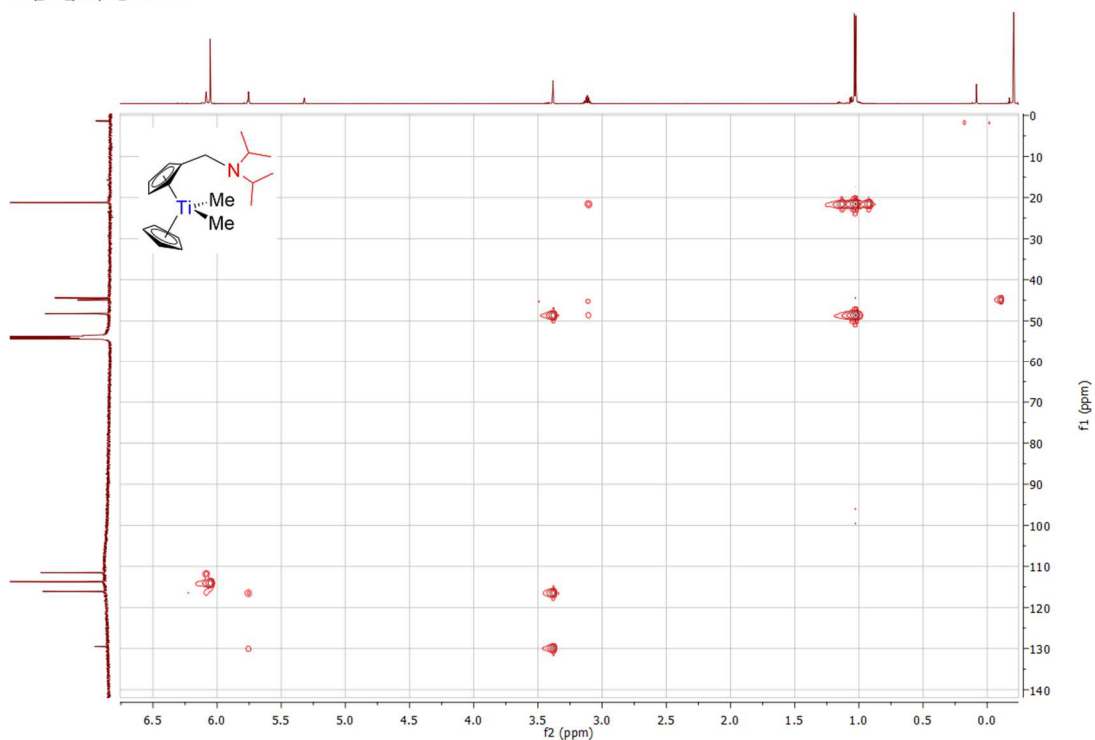
Spectrum 0-239: 1 H 13 C HMBC of 34 (600.23 MHz / 150.9 MHz, 300 K, dichloromethane-d 2 )
