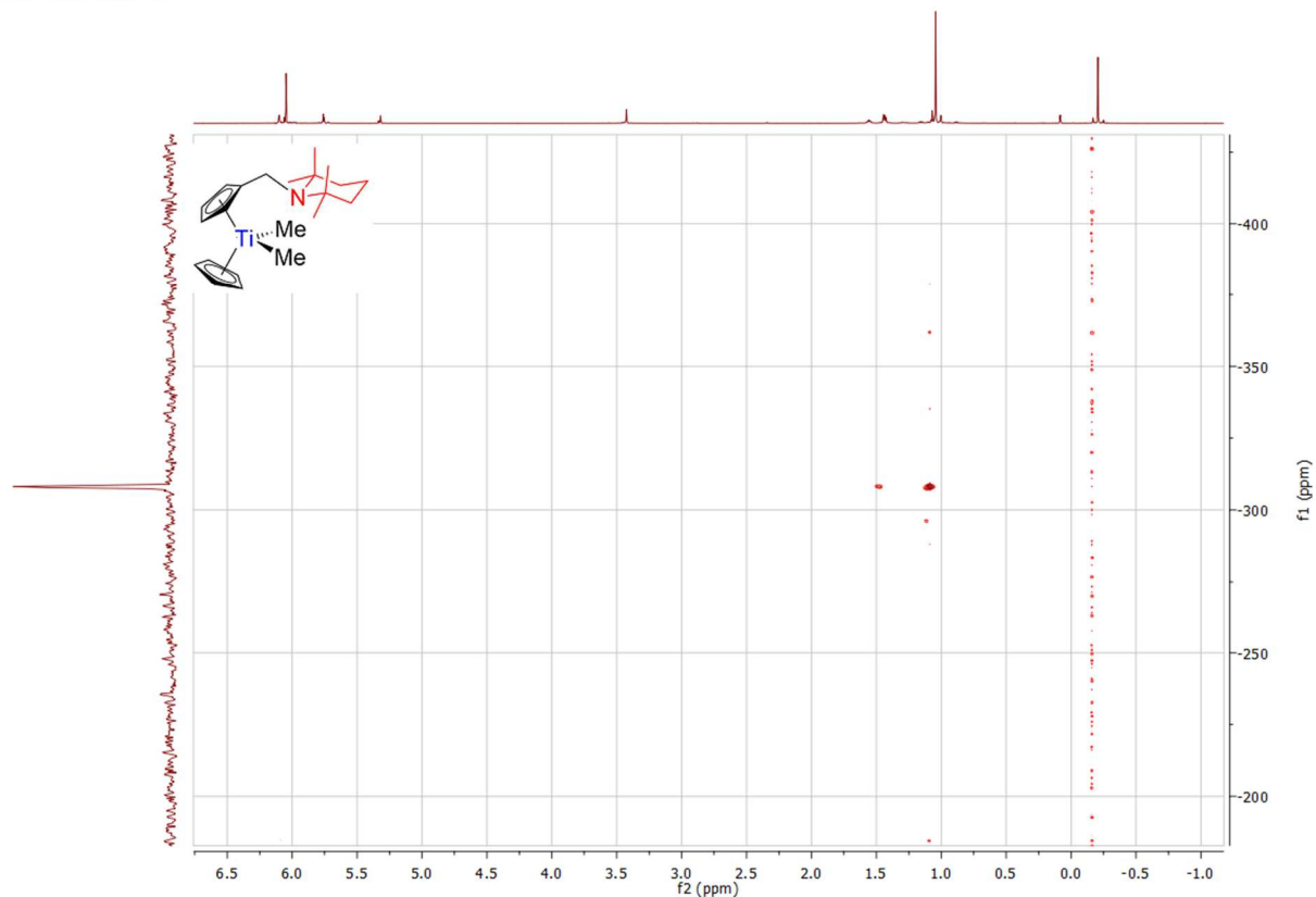
Spectrum 0-249: ^1\text{H} ^{15}\text{N} HMBC of 35 (600.23 MHz / 43.3 MHz, 300 K, dichloromethane- d_2 )
