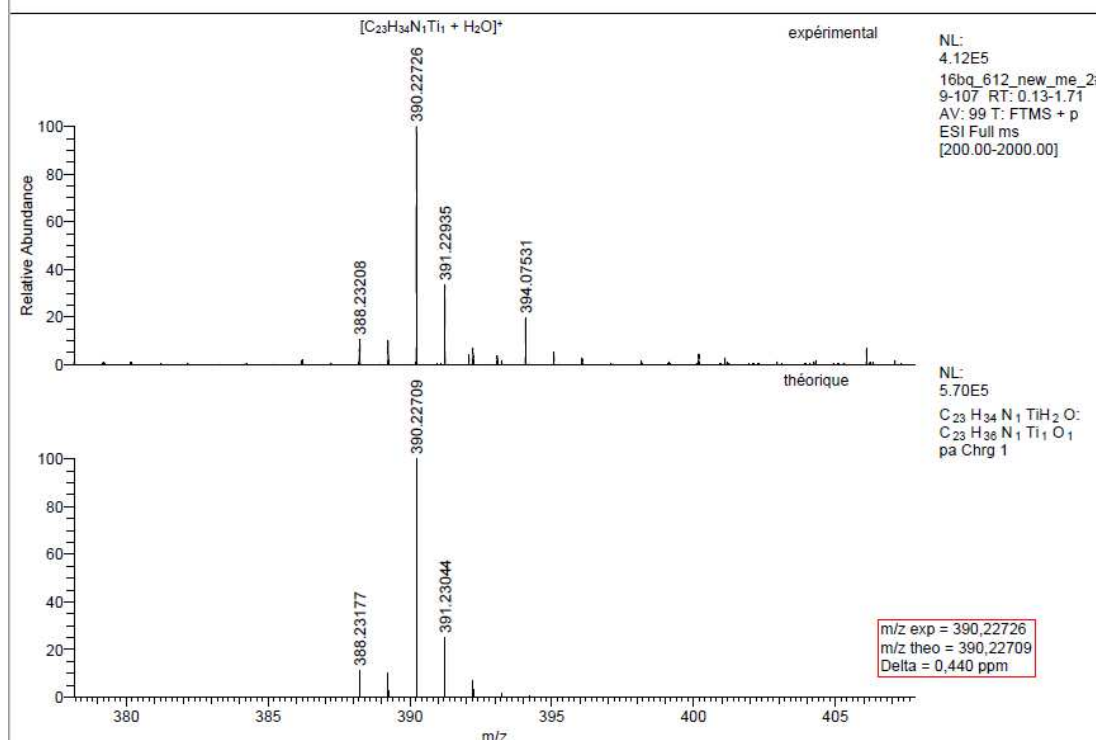
Spectrum 0-372: HRMS of 47 (Positive mode ESI, bromobenzene)
