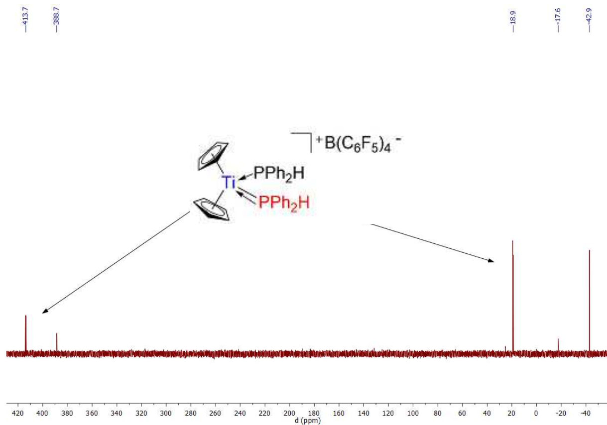
Spectrum 0-447: ^{31}\text{P}\{^1\text{H}\} NMR (202 MHz, \text{d}_8\text{-THF} , 300K), no irradiation.
