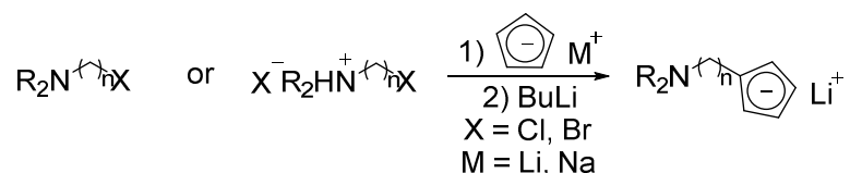
Scheme I-30: general procedure for the synthesis of (aminoalkyl)cyclopentadienides
