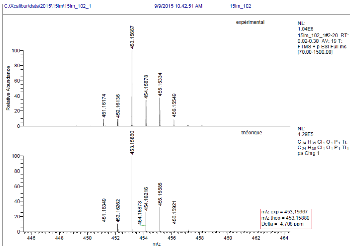
Spectrum 0-507: HRMS of 60 (Positive mode ESI, dichloromethane)
