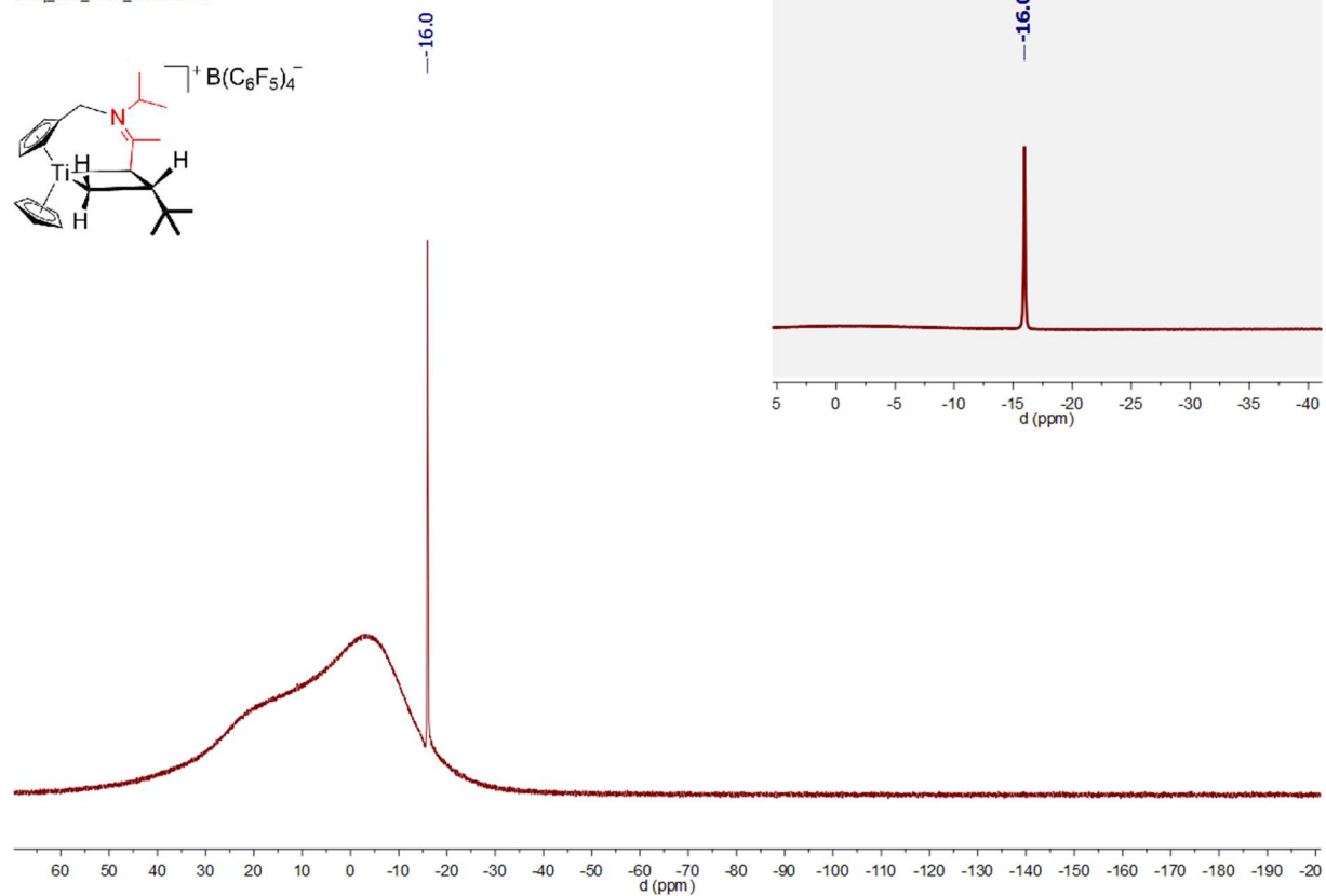
Spectrum 0-369: ^{11}\text{B}\{^1\text{H}\} and ^{11}\text{B} (opacified) NMR of 47 (160.42 MHz, 273 K, bromobenzene- d_5 )
