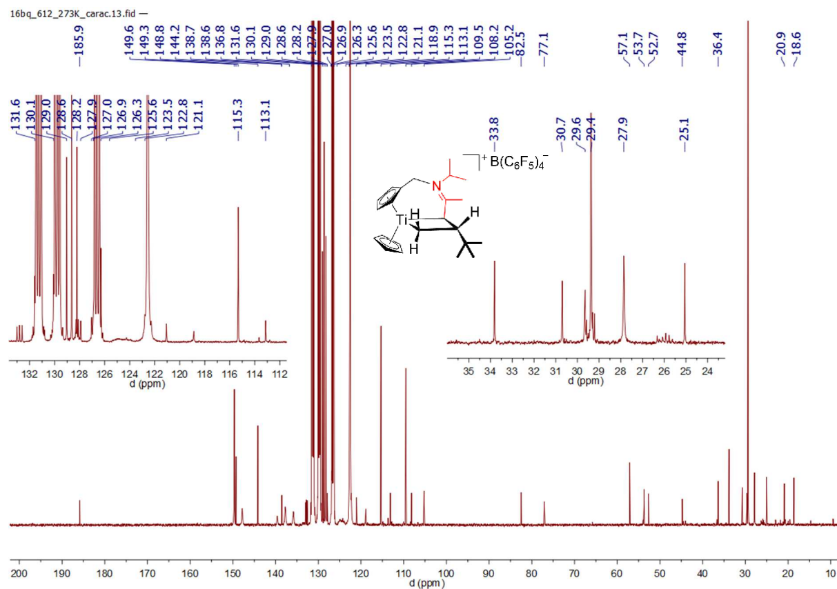
Spectrum 0-363: ^{13}C\{^1H\} NMR of 47 (125.75 MHz, 273 K, bromobenzene- d_5 )
