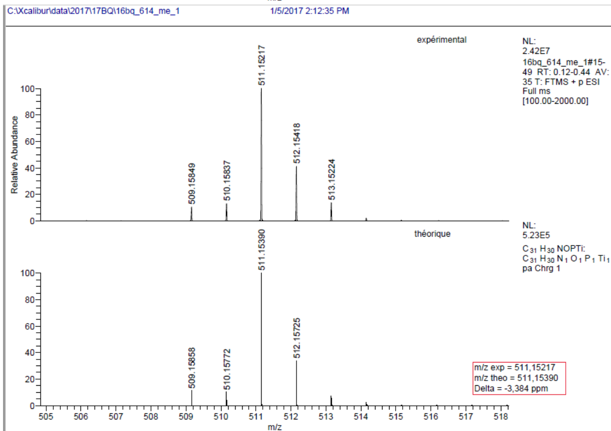
Spectrum 0-530: HRMS of 62 (Positive mode ESI, dichloromethane)
