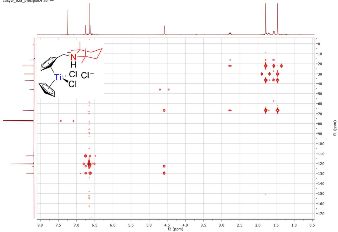
Spectrum 0-112: ^1\text{H} ^{13}\text{C} HMBC of 18 (600.23 MHz / 150.94 MHz, 300 K, chloroform- d_1 )
