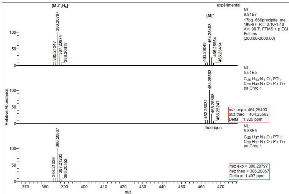
Spectrum 0-272: HRMS of 37 (Positive mode ESI, dichloromethane)
