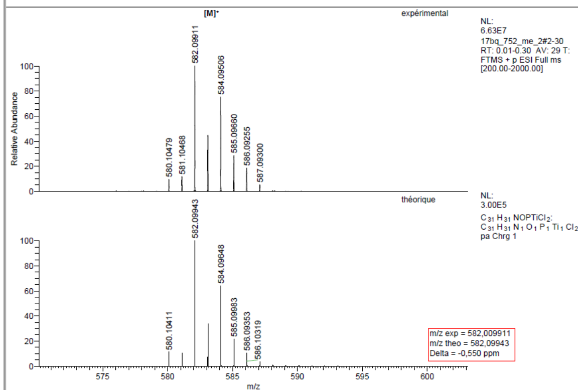
Spectrum 0-520: HRMS of 61 (Positive mode ESI, dichloromethane)
