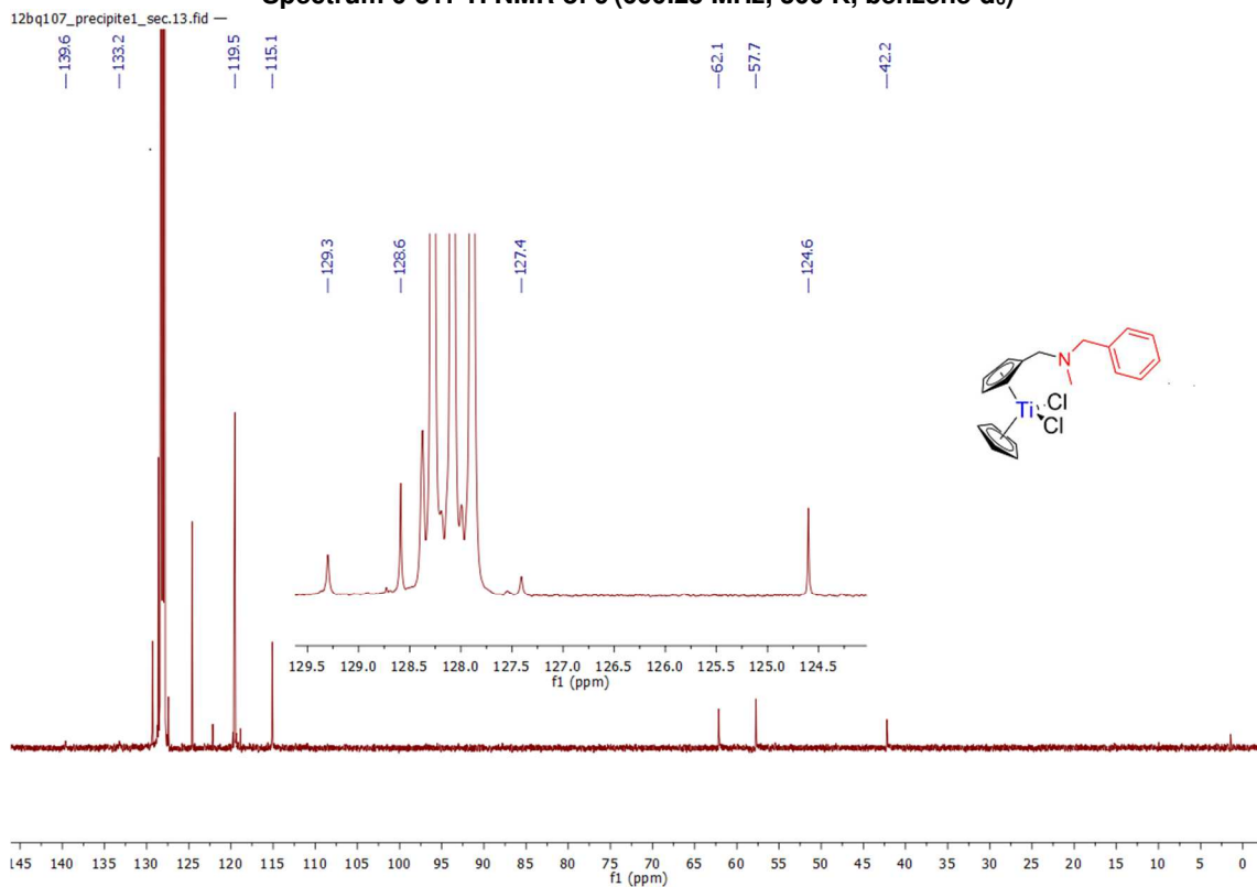
Spectrum 0-32: ^{13}\text{C}\{^1\text{H}\} NMR of 9 (125.77 MHz, 300 K, benzene- d_6 )
