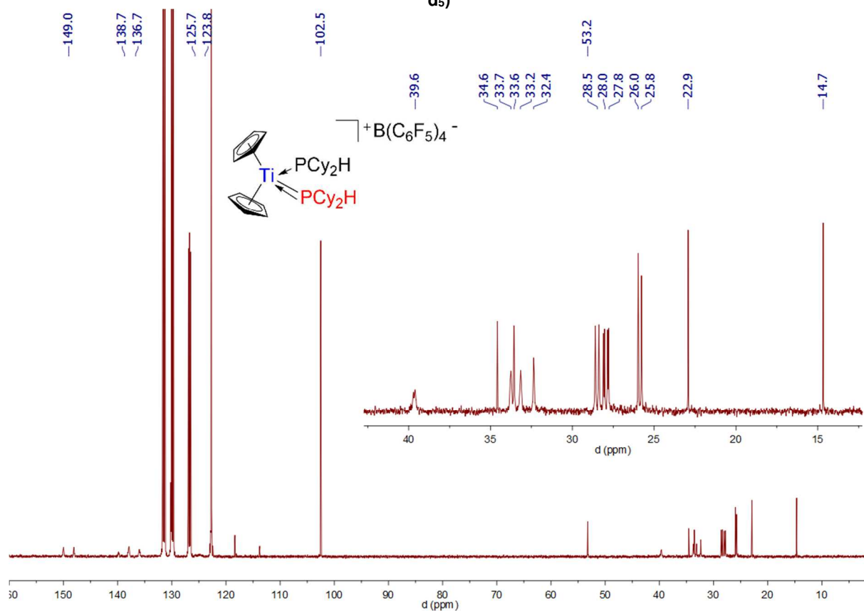
Spectrum 0-390: ^{13}\text{C}\{^1\text{H}\} NMR of 51 (125.75 MHz, 300 K, bromobenzene- d_5 )
