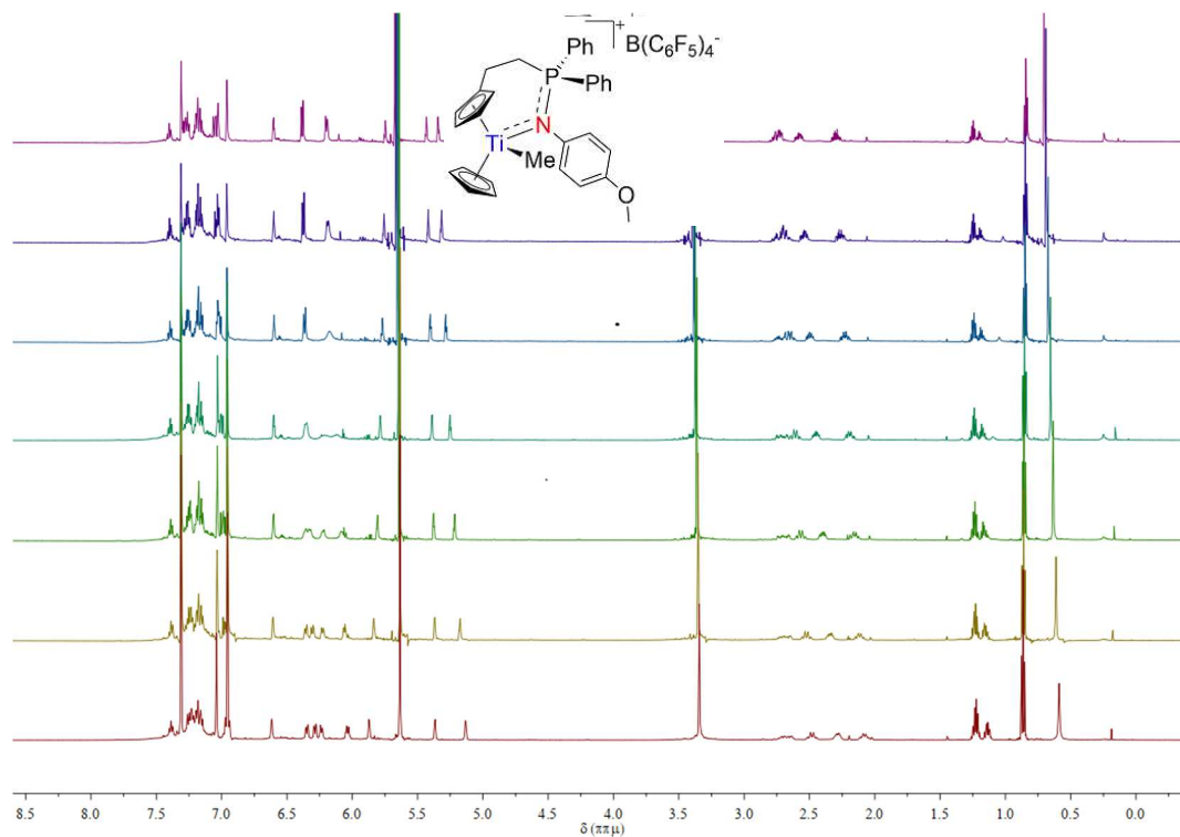
Spectrum 0-544 1 H NMR superposition of 64 (600 MHz, 240-360K, bromobenzene-d 5 )
