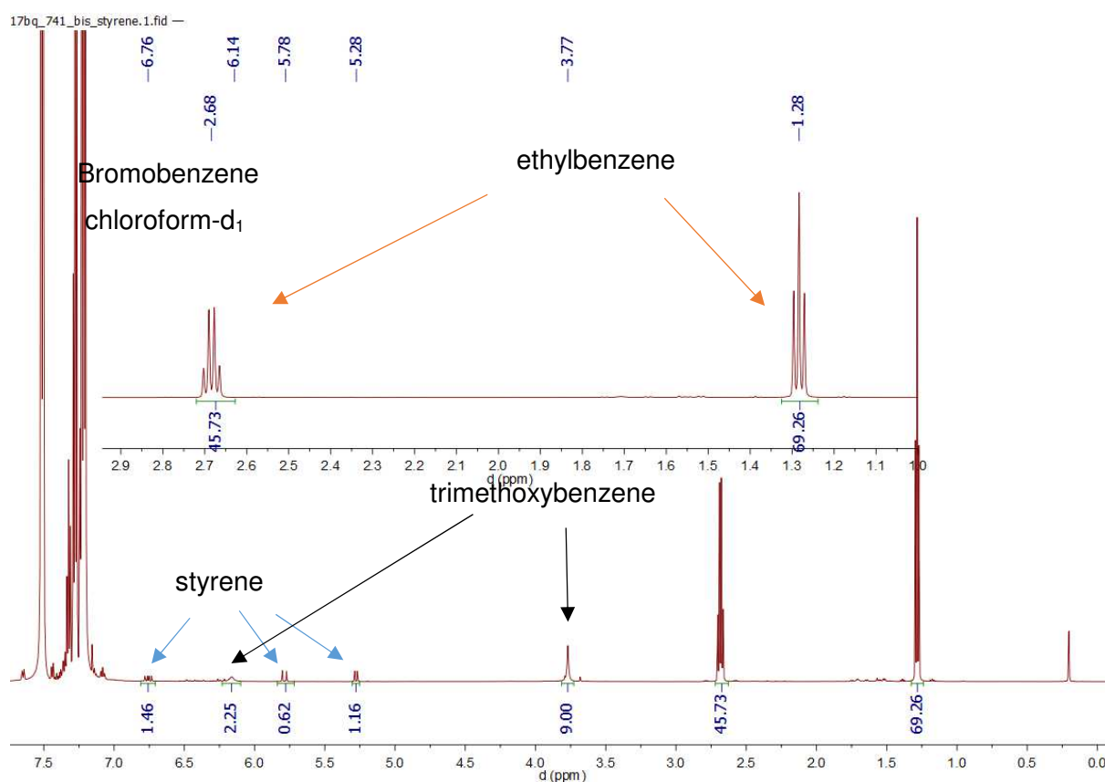
Spectrum 0-462: Hydrogenation of styrene with 53 (600.23 MHz, 300K, Chloroform- d_1 )
