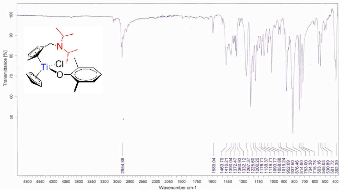
Spectrum 0-197: HRMS of 28 (Positive mode ESI, dichloromethane)
