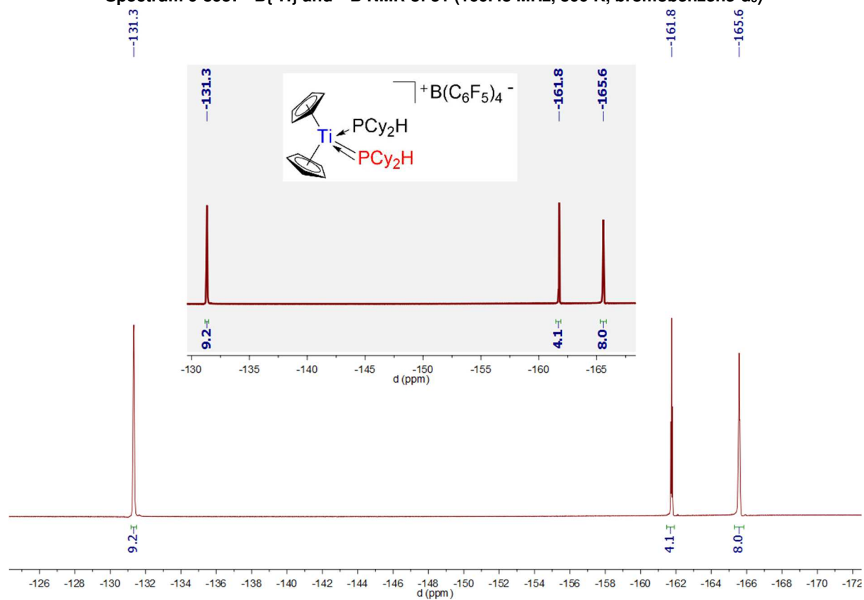
Spectrum 0-396: ^{19}\text{F}\{^1\text{H}\} and ^{19}\text{F} NMR of 51 (470.45 MHz, 300 K, bromobenzene- \text{d}_5 )
