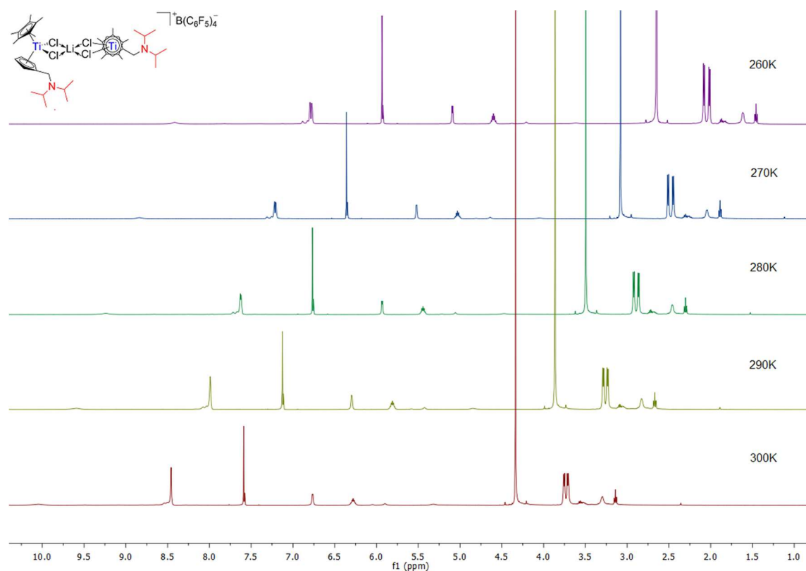
Spectrum 0-165: superposition of the ^1\text{H} NMR spectra from 300K to 260 K (500.03 MHz, 260 K, dichloromethane- d_2 )
