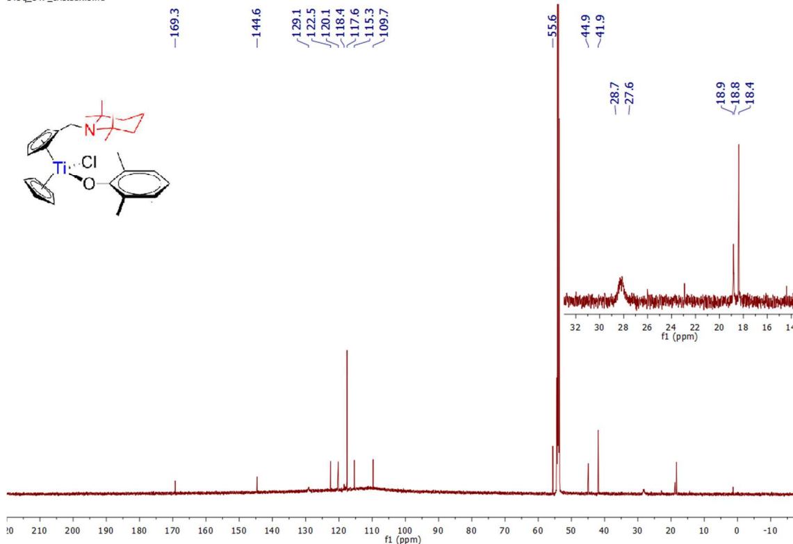
Spectrum 0-201: ^{13}\text{C}\{^1\text{H}\} NMR of 29 (150.94 MHz, 300 K, dichloromethane- d_2 )
