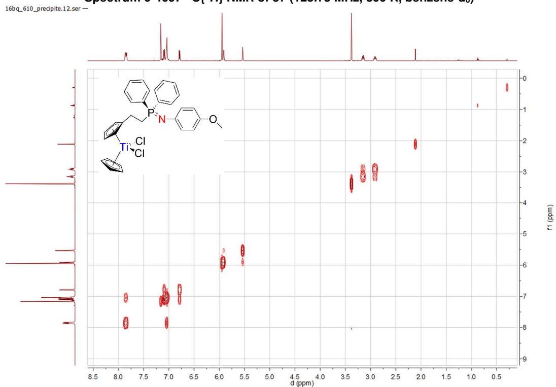
Spectrum 0-470: ^1\text{H} \ ^1\text{H} COSY of 57 (500.03 MHz, 300 K, 273 K, benzene- d_6 )
