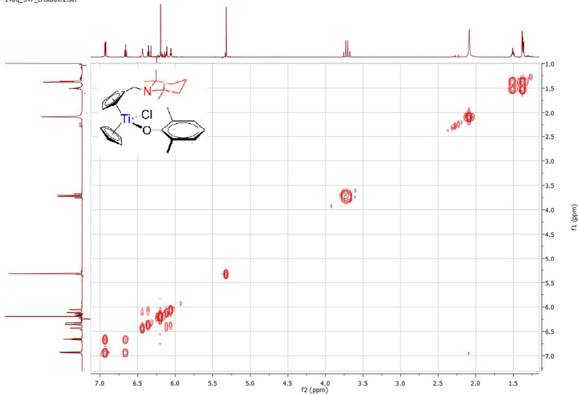
Spectrum 0-202: ^1\text{H} ^1\text{H} COSY of 29 (600.23 MHz, 300 K, dichloromethane- d_2 )
