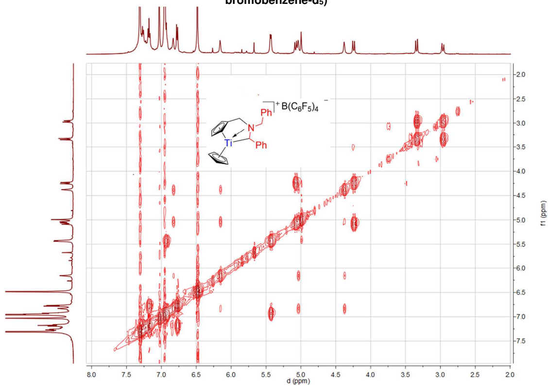
Spectrum 0-294: ^1\text{H} ^1\text{H} COSY of 40 (500.03 MHz, 300 K, bromobenzene- d_5 )
