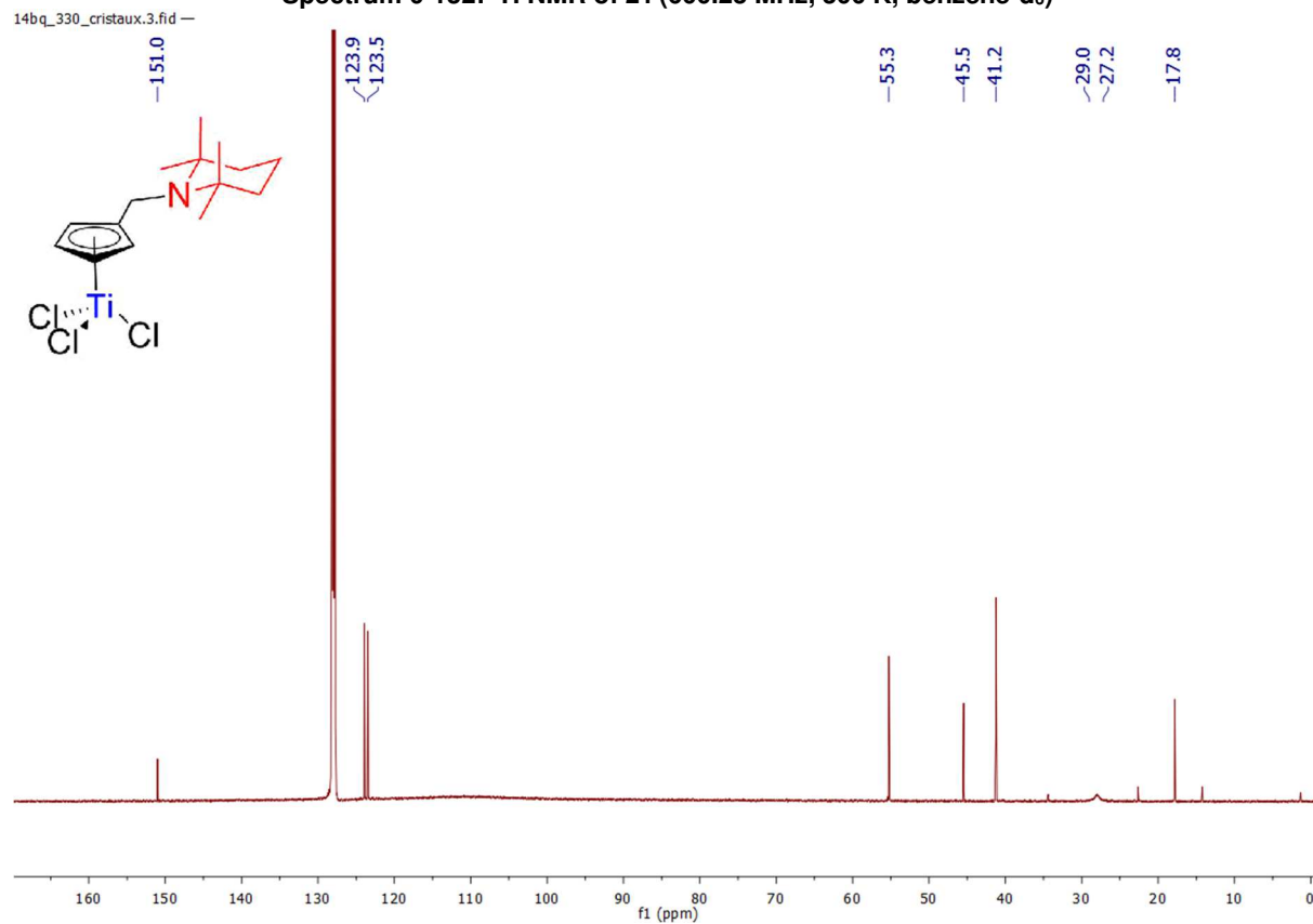
Spectrum 0-133: ^{13}\text{C}\{^1\text{H}\} NMR of 21 (150.94 MHz, 300 K, benzene- d_6 )
