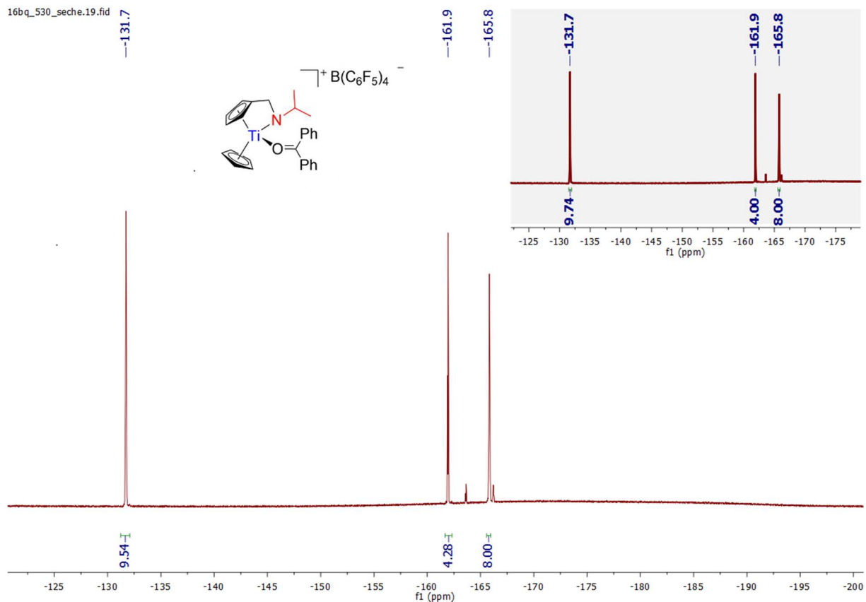
Spectrum 0-309: ^{19}\text{F}\{^1\text{H}\} and ^{19}\text{F} (opacified) NMR of 41 (470.45 MHz, 300 K, bromobenzene- d_5 )
