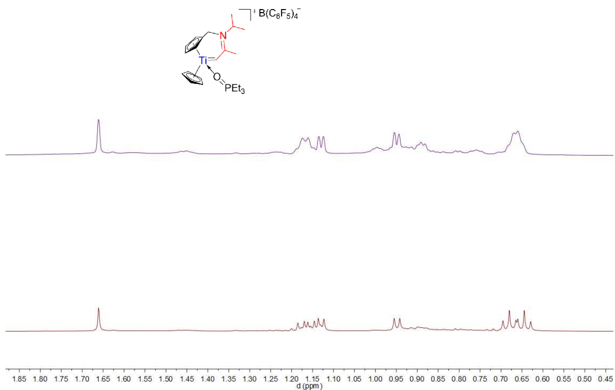
Spectrum 0-350: ^1\text{H}\{^{31}\text{P}\} NMR (top) superposed with ^1\text{H} NMR (bottom) of 45 (600.23 MHz, 300 K, bromobenzene- d_5 )
