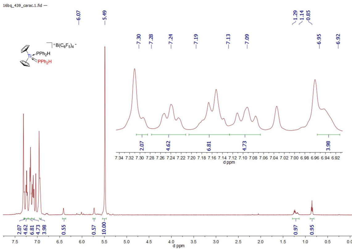
Spectrum 0-377: ^1\text{H} NMR of 50 (500.03 MHz, 300 K, bromobenzene- d_5 )
