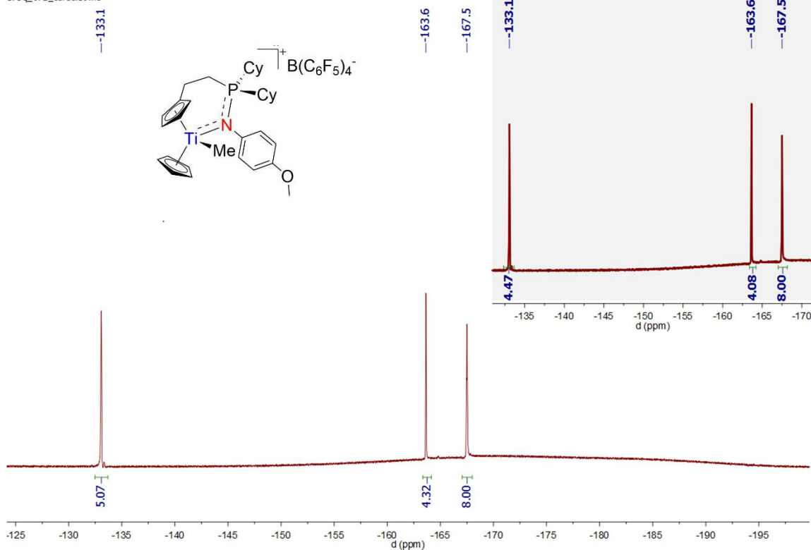
Spectrum 0-566: ^{19}\text{F}\{^1\text{H}\} and ^{19}\text{F} NMR of 65 (470.45 MHz, 300 K, dichloromethane- d_2 )
