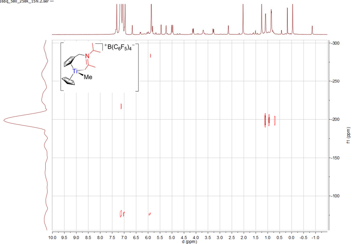
Spectrum 0-322: ^1\text{H} ^{15}\text{N} HMBC of 42 (600.23 MHz / 43.3 MHz, 258 K, bromobenzene- d_5 )
