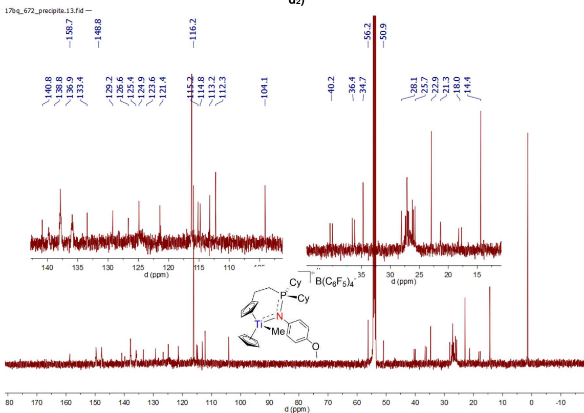
Spectrum 0-560: ^{13}\text{C}\{^1\text{H}\} NMR of 65 (125.75 MHz, 300 K, dichloromethane- d_2 )
