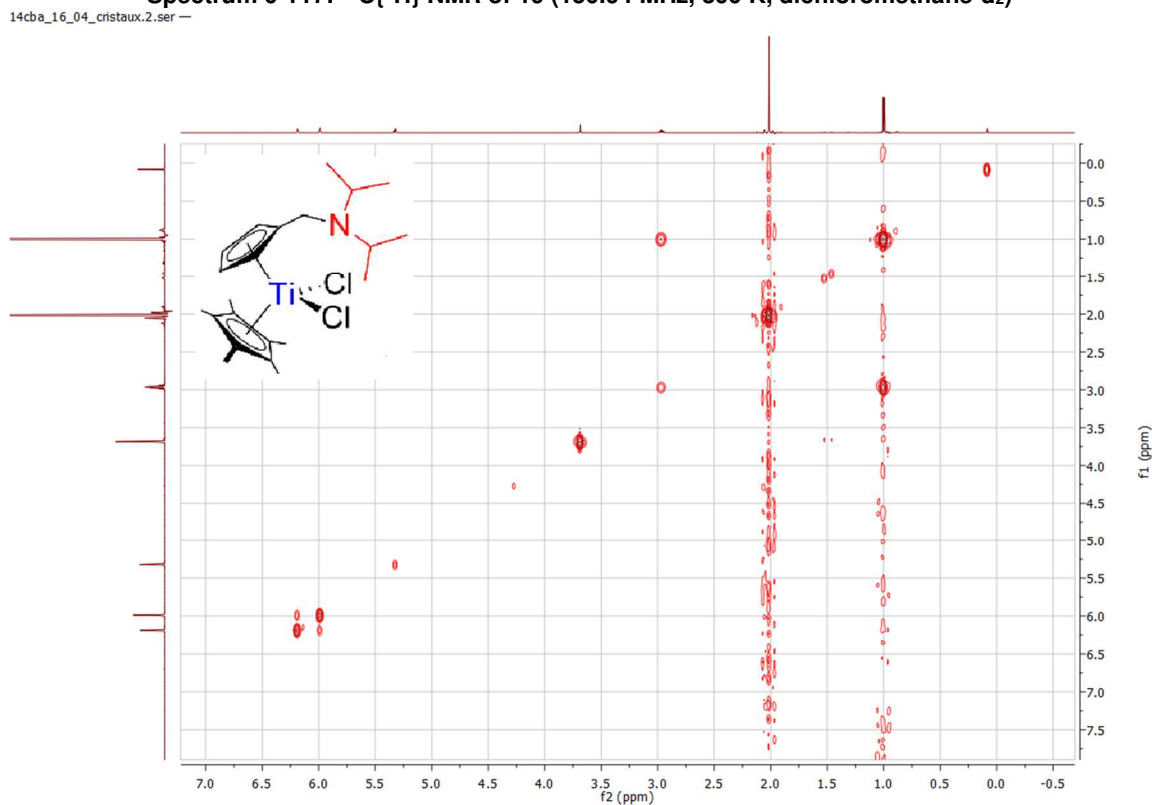
Spectrum 0-118: ^1\text{H} ^1\text{H} COSY of 19 (600.23 MHz, 300 K, dichloromethane- d_2 )
