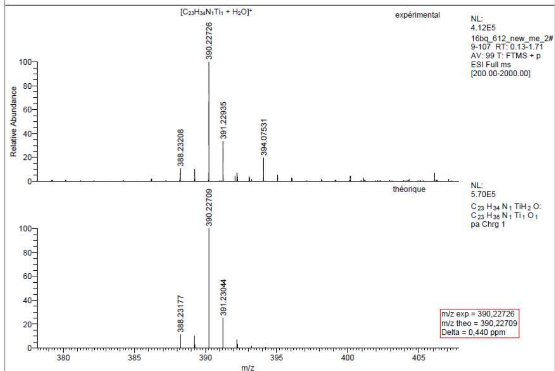
Spectrum 0-372: HRMS of 47 (Positive mode ESI, bromobenzene)
