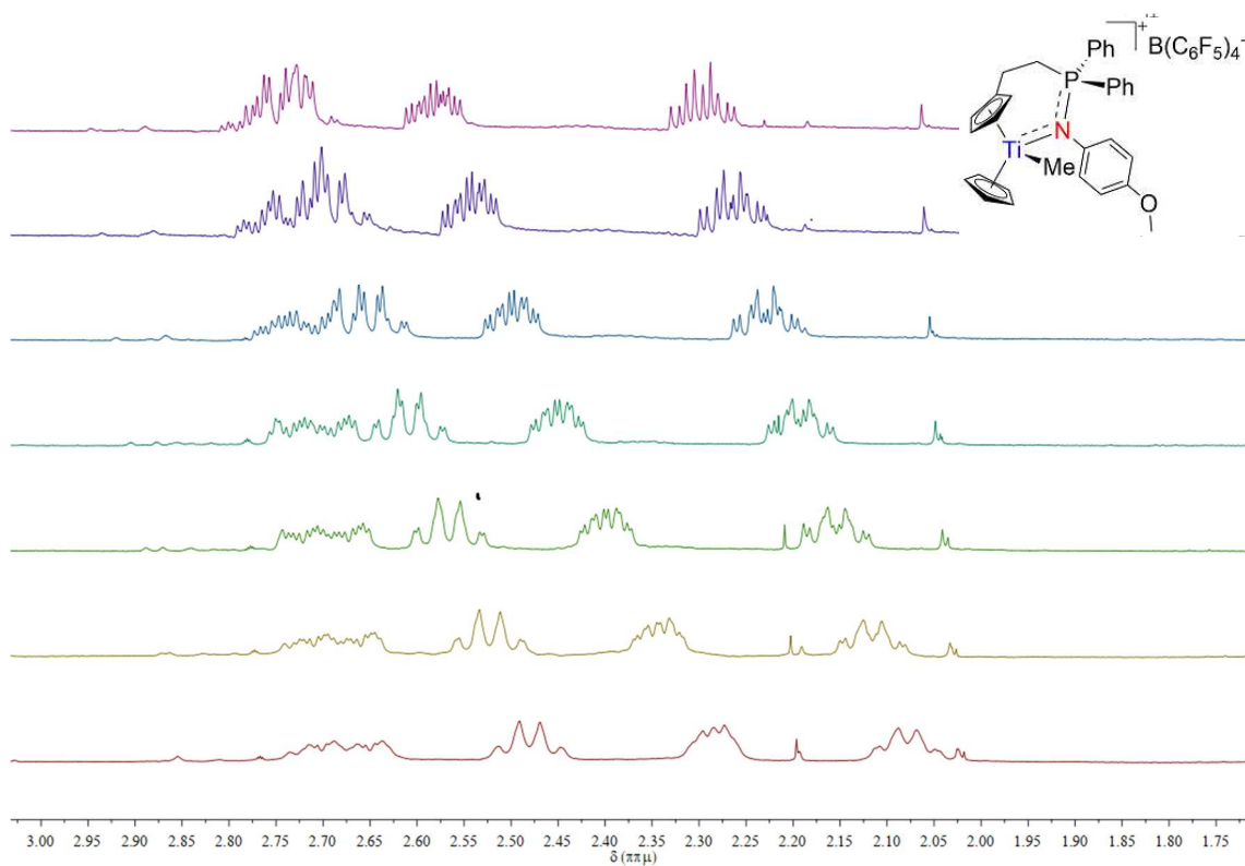
Spectrum 0-545: ^1\text{H} NMR superposition 3.00-1.75 ppm of 64 (600 MHz, 240-360K, bromobenzene- d_5 )
