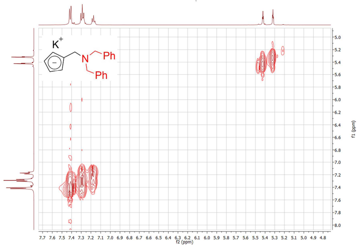
Spectrum 0-15: ^1\text{H} ^1\text{H} COSY of 3-K (500.03 MHz, 300 K, dimethylsulfoxide- \text{d}_6 )
