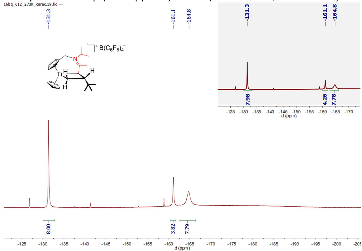
Spectrum 0-370: ^{19}\text{F}\{^1\text{H}\} and ^{19}\text{F} (opacified) NMR of 47 (470.45 MHz, 273 K, bromobenzene- d_5 )
