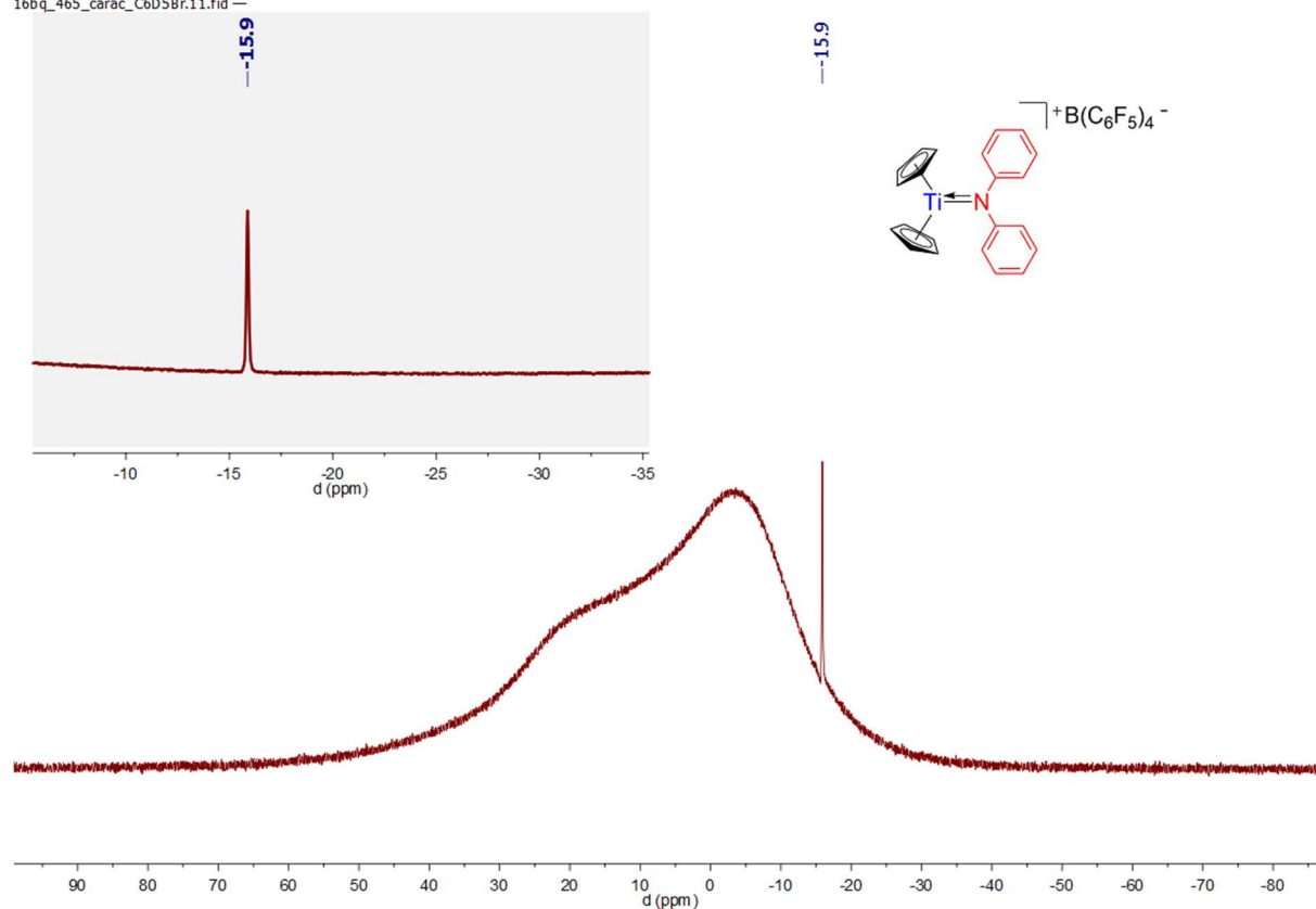
Spectrum 0-414: ^{11}\text{B}\{^1\text{H}\} and ^{11}\text{B} NMR of 53 (160.43 MHz, 300 K, bromobenzene- d_5 )
