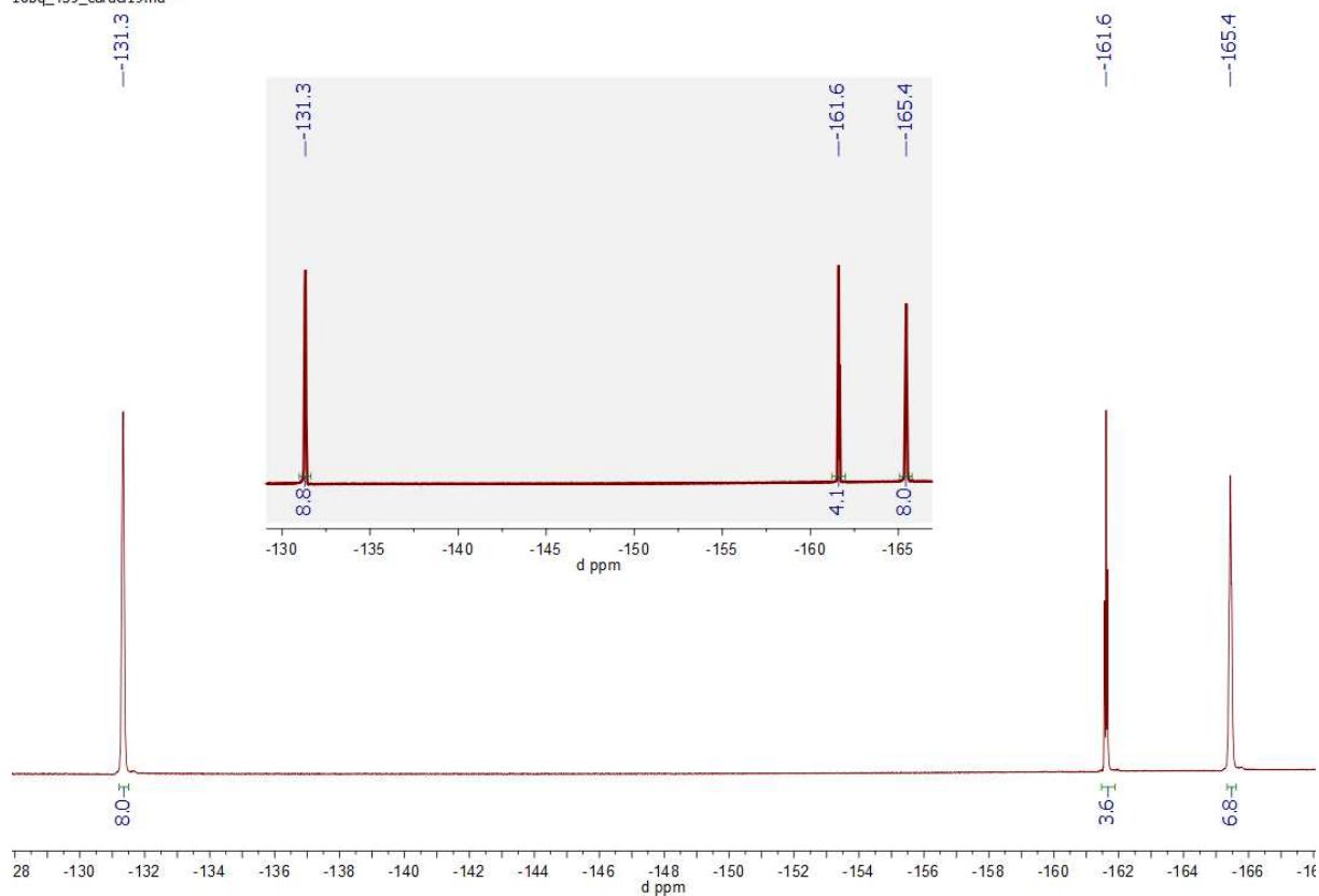
Spectrum 0-386: ^{19}\text{F}\{^1\text{H}\} and ^{19}\text{F} NMR of 50 (470.45 MHz, 300 K, bromobenzene- d_5 )
