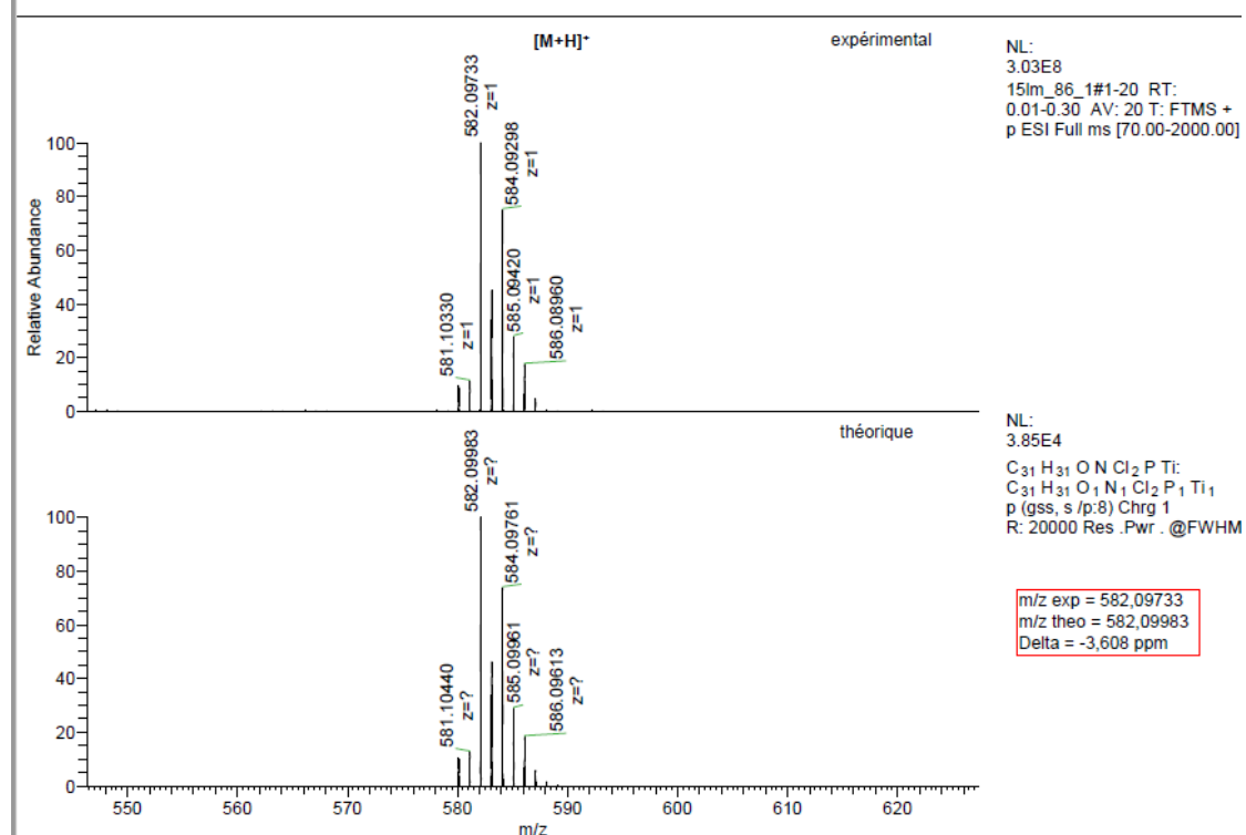
Spectrum 0-483: HRMS of 58 (Positive mode ESI, dichloromethane)
