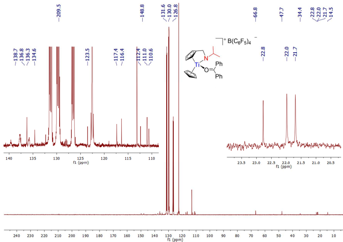
Spectrum 0-302: ^{13}\text{C}\{^1\text{H}\} NMR of 41 (125.75 MHz, 300 K, bromobenzene- d_5 )
