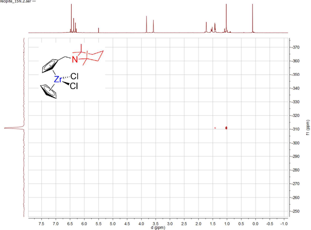
Spectrum 0-162: 1 H 15 N HMBC of 24 (600.23 MHz / 43.3 MHz, 300 K, tetrahydrofuran-d 8 )
