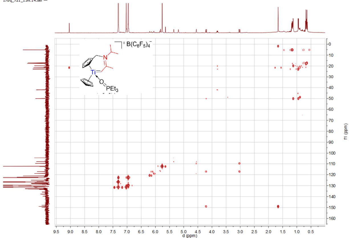
Spectrum 0-354: ^1\text{H} ^{13}\text{C} HMBC of 45 (600.23 MHz / 150.86 MHz, 300 K, bromobenzene- d_5 )
