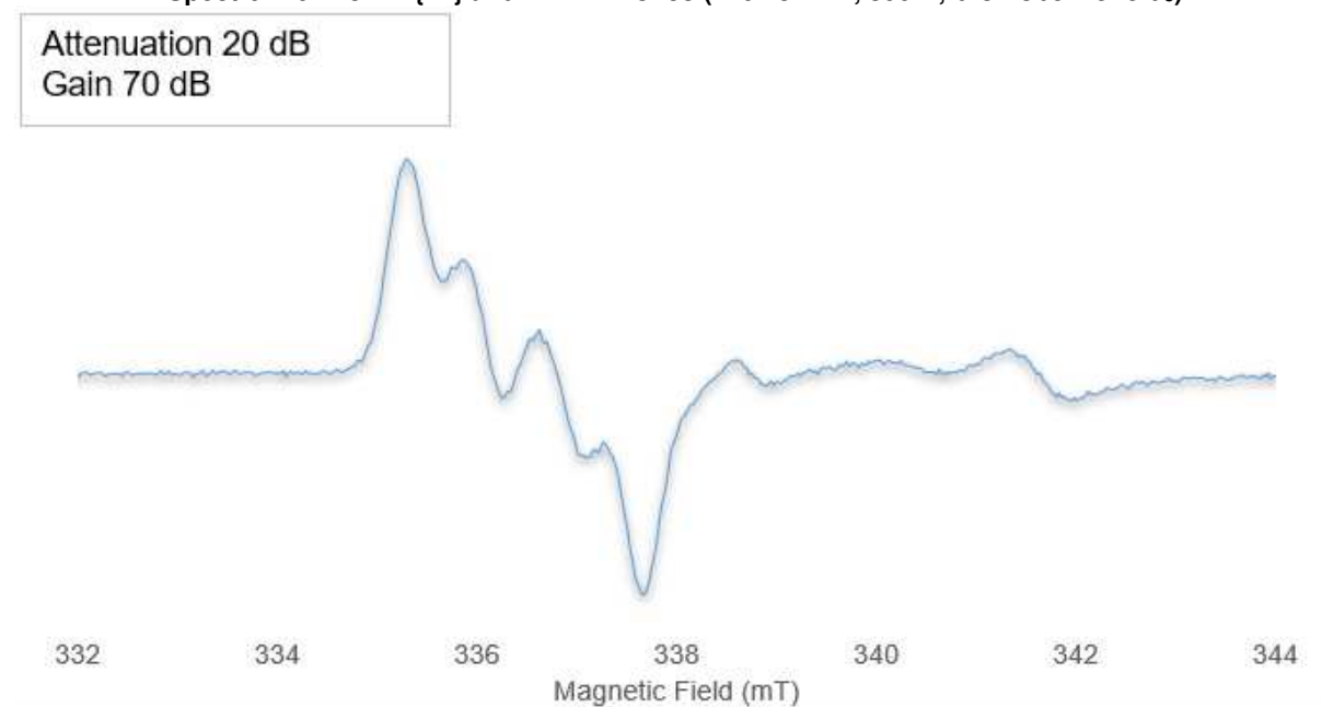
Spectrum 0-416: EPR spectrum of 53 (9.440489 GHz, 295 K, Bromobenzene)
