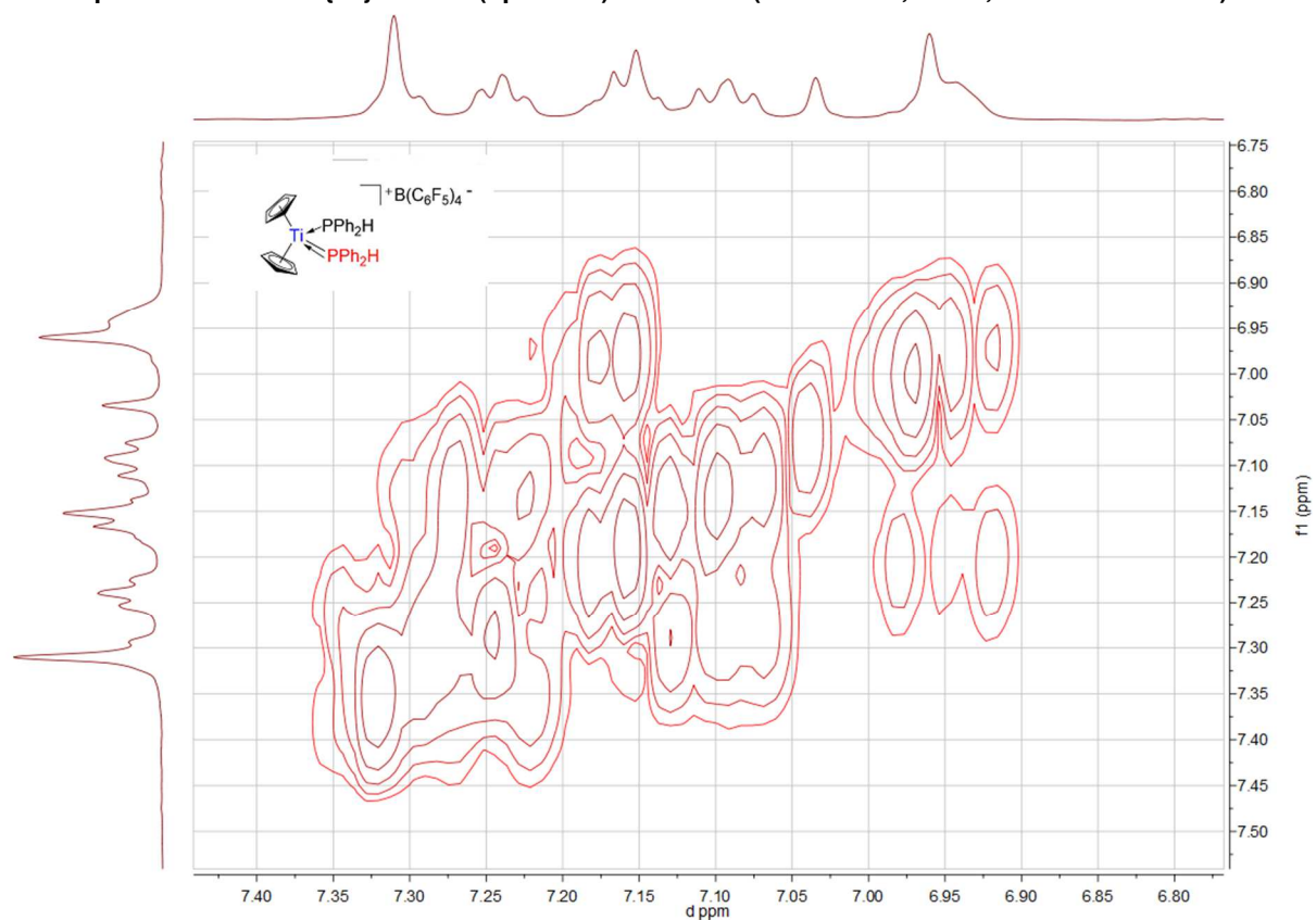
Spectrum 0-382: ^1\text{H} \ ^1\text{H} COSY of 50 (500.03 MHz, 300 K, 273 K, bromobenzene- d_5 )
