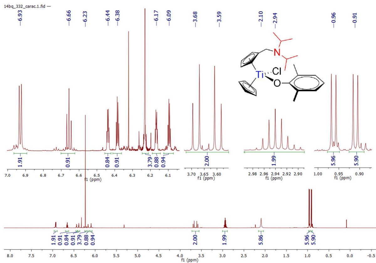
Spectrum 0-191: ^1\text{H} NMR of 28 (600.23 MHz, 300 K, dichloromethane- d_2 )
