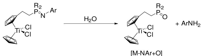
Scheme V-6: hydrolysis process of the titanocenyl iminophosphoranes
