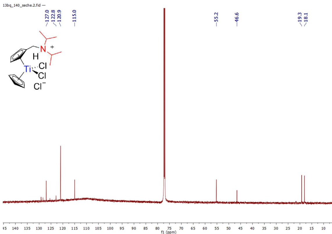
Spectrum 0-101: ^{13}\text{C}\{^1\text{H}\} NMR of 17 (150.94 MHz, 300 K, chloroform- d_1 )
