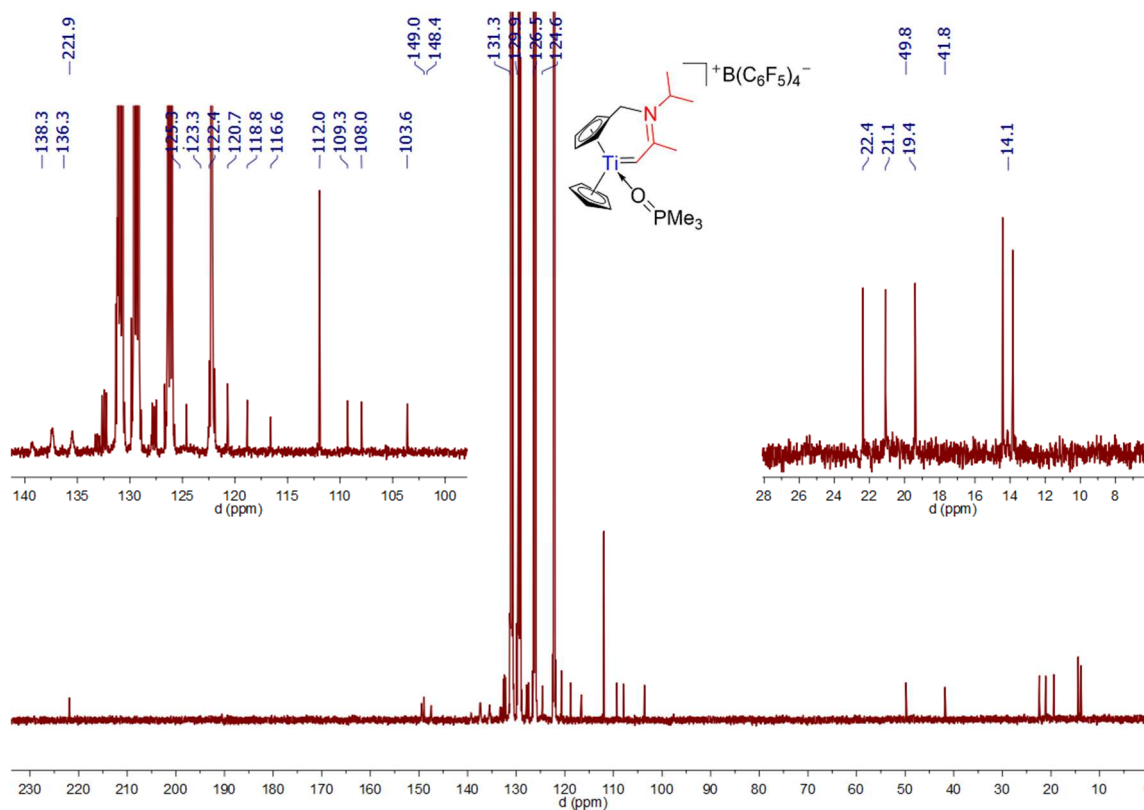
Spectrum 0-339: ^{13}\text{C}\{^1\text{H}\} NMR of 44 (125.75 MHz, 300 K, bromobenzene- d_5 )
