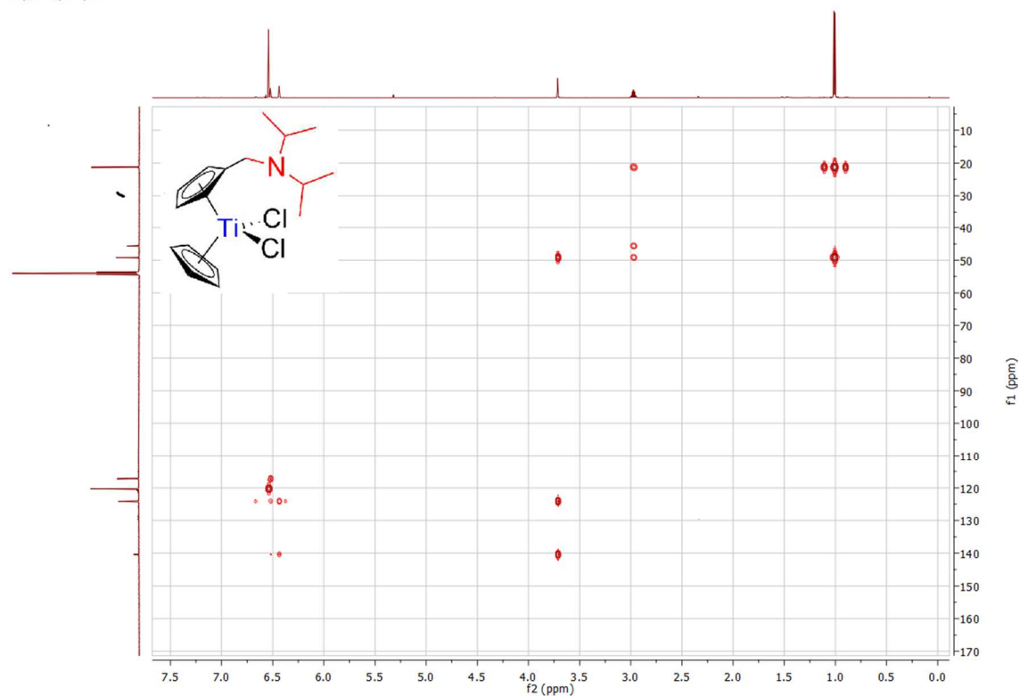
Spectrum 0-62: ^1\text{H} ^{13}\text{C} HMQC of 12 (600.23 MHz / 150.94 MHz, 300 K, dichloromethane- d_2 )
