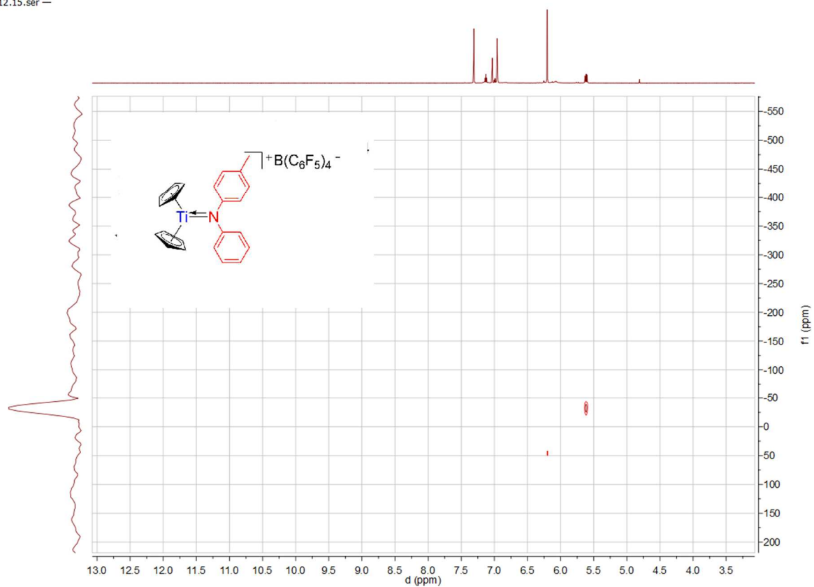
Spectrum 0-422: 1 H 15 N HMBC of 54 (500.03 MHz / 43.3 MHz, 300 K, bromobenzene-d 5 )
