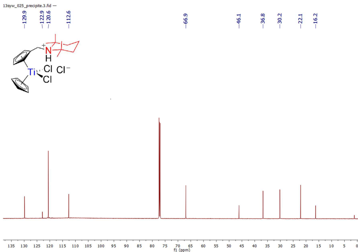
Spectrum 0-109: ^{13}\text{C}\{^1\text{H}\} NMR of 18 (150.94 MHz, 300 K, chloroform- d_1 )
