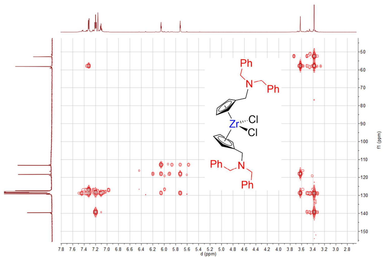
Spectrum 0-145: ^1\text{H} ^{13}\text{C} HMBC of 22 (600.23 MHz / 150.94 MHz, 300 K, benzene- d_6 )
