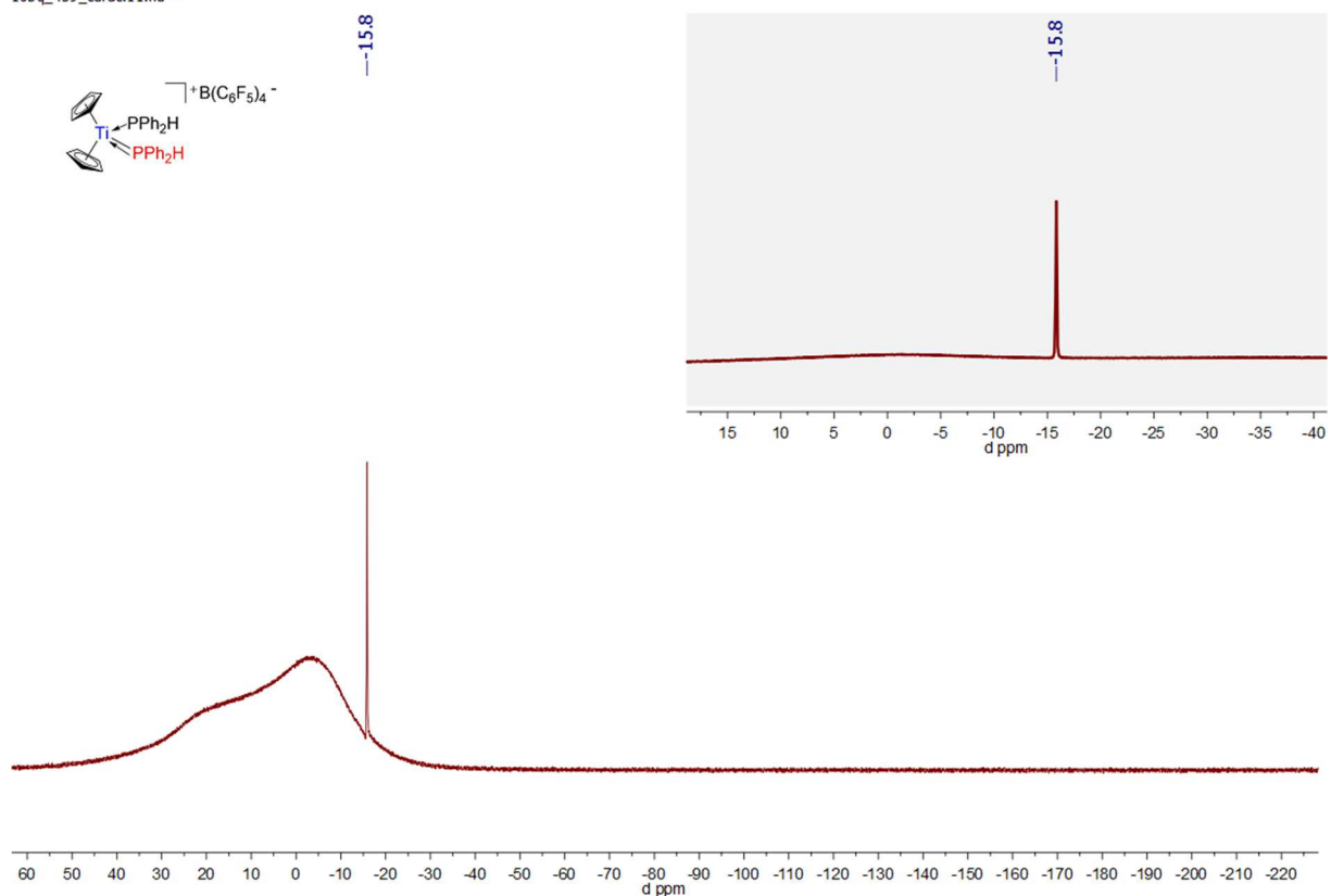
Spectrum 0-385: ^{11}\text{B}\{^1\text{H}\} and ^{11}\text{B} NMR of 50 (160.43 MHz, 300 K, bromobenzene- d_5 )
