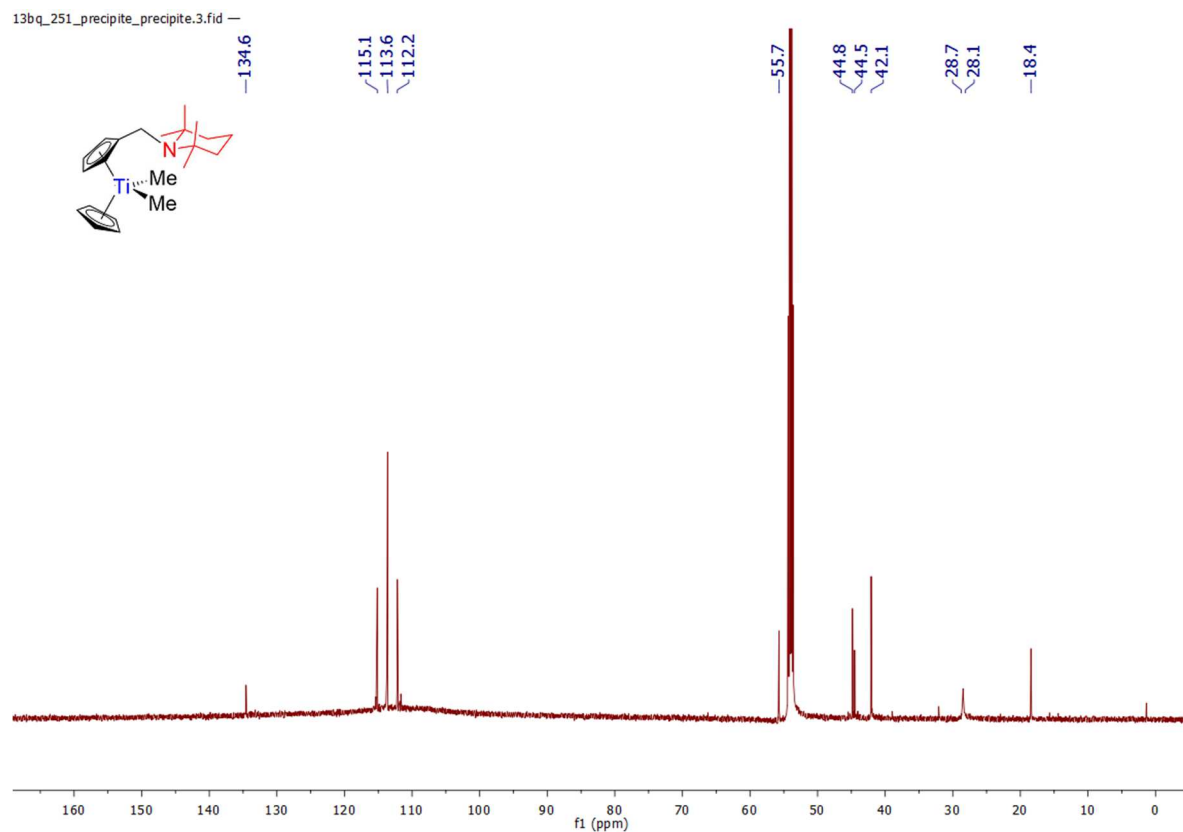
Spectrum 0-245: ^{13}\text{C}\{^1\text{H}\} NMR of 35 (150.9 MHz, 300 K, dichloromethane- d_2 )
