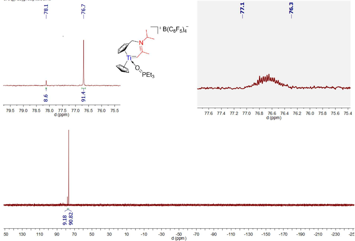
Spectrum 0-355: ^{31}\text{P}\{^1\text{H}\} and ^{31}\text{P} (opacified) NMR of 45 (202.46 MHz, 300 K, bromobenzene- d_5 )
