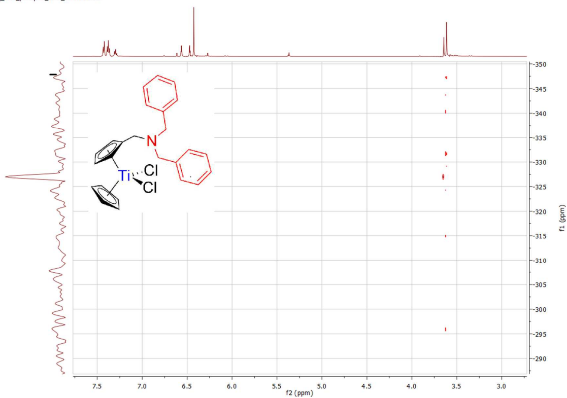
Spectrum 0-54: ^1\text{H} ^{15}\text{N} HMBC of 11 (600.23 MHz / 43.3 MHz, 300 K, dichloromethane- d_2 )
