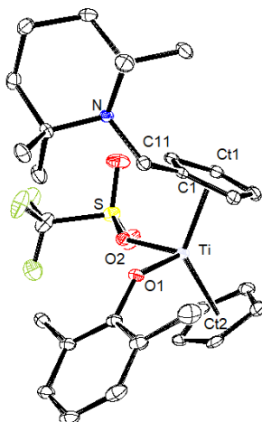
Figure III-3: ORTEP view of 30 (ellipsoids drawn at the 30% probability level, hydrogen atoms removed for clarity, enantiomer omitted for clarity). Selected bond lengths ( \text{\AA} ) and angles ( ^\circ ): Ti-Ct1 = 2.0931(14) / 2.0849(12), Ti-Ct2 = 2.0658(14) / 2.0585(12), Ti-O1 = 1.8748(17) / 1.8754(16), Ti-O2 = 2.0931(14) / 2.0887(17), C1-C11 = 1.514(4) / 1.503(3), C11-N = 1.462(3) / 1.460(3), Ct1-Ti-Ct2 = 131.31(6) / 130.62(5), O1-Ti-O2 = 93.97(7) / 93.76(5), C1-C11-N = 113.0(2) / 112.7(2).
