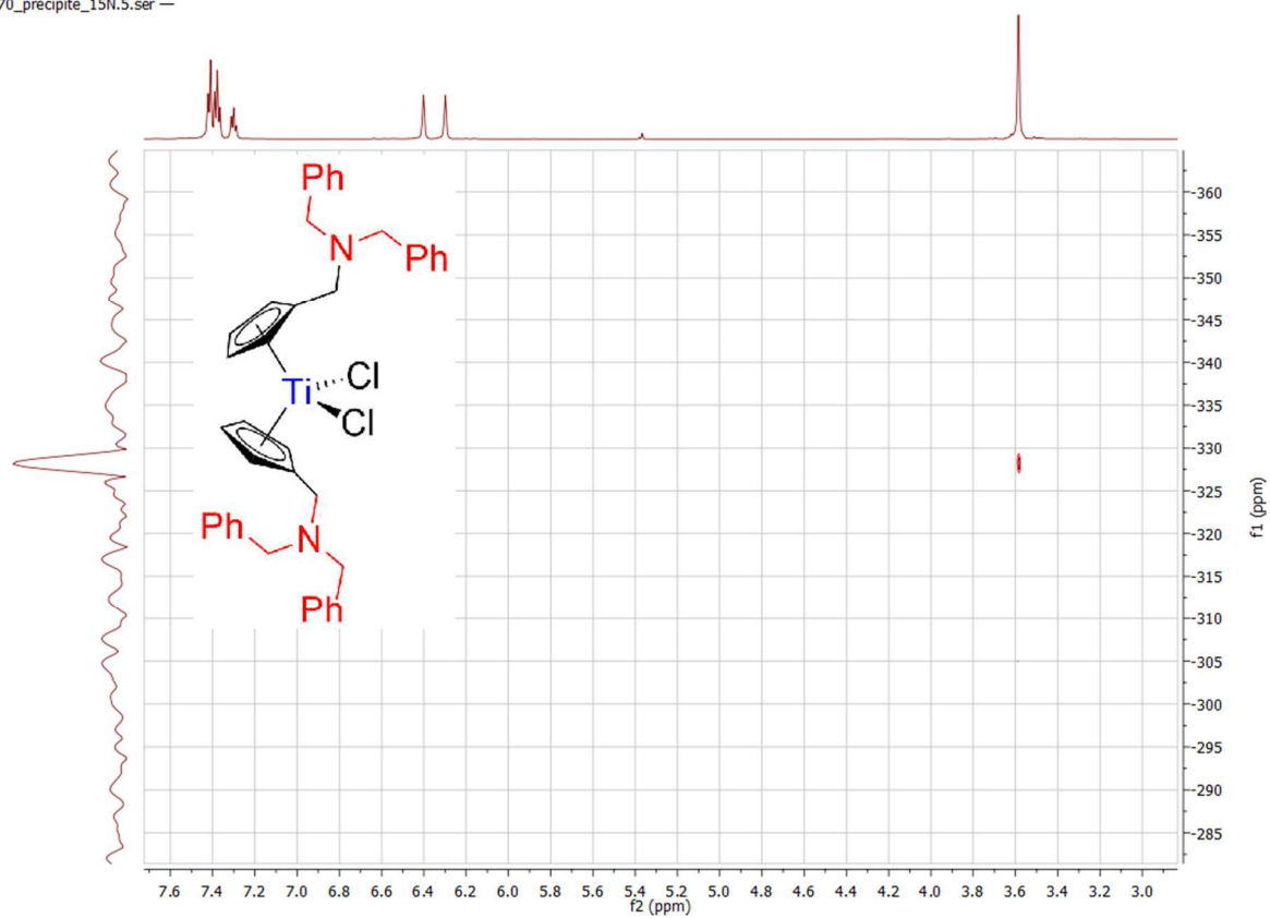
Spectrum 0-130: ^1\text{H} ^{15}\text{N} HMBC of 20 (600.23 MHz / 43.3 MHz, 300 K, benzene- d_6 )
