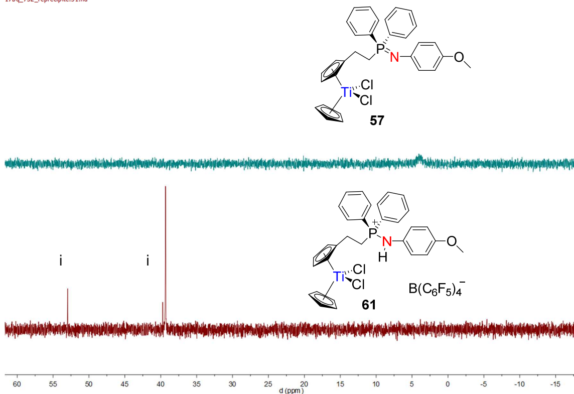
Spectrum V-1: superposition of ^{31}\text{P}\{^1\text{H}\} NMR spectra of 61 (bottom) and 57(top) (500 MHz, 300K, \text{C}_6\text{D}_6 ) 1 : unidentified impurities
