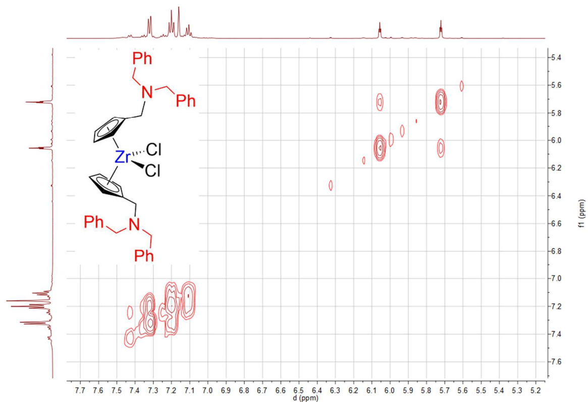
Spectrum 0-143: ^1\text{H} ^1\text{H} COSY of 22 (600.23 MHz, 300 K, benzene- d_6 )
