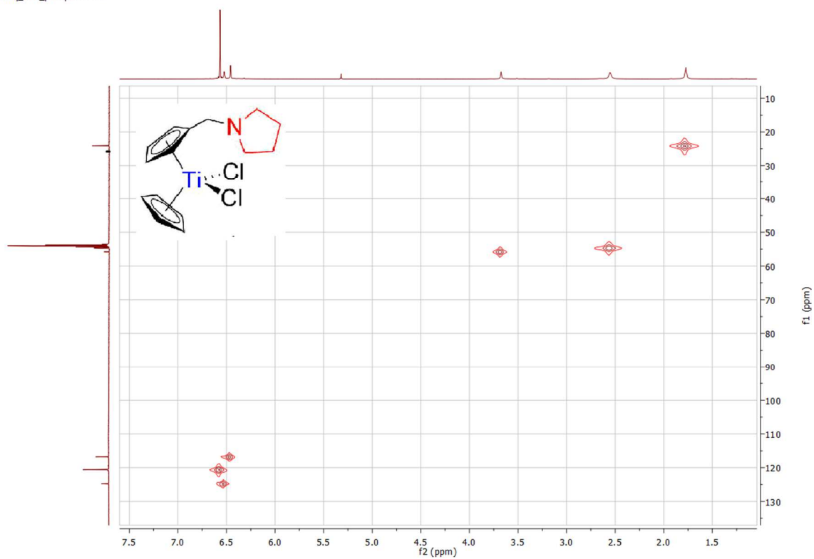
Spectrum 0-43: ^1\text{H} ^{13}\text{C} HMQC of 10 (600.23 MHz / 150.94 MHz, 300 K, dichloromethane- d_2 )
