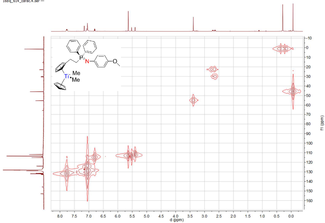
Spectrum 0-526: 1 H 13 C HMQC of 62 (500.03 MHz / 125.75 MHz, 300 K, benzene-d 6 )
