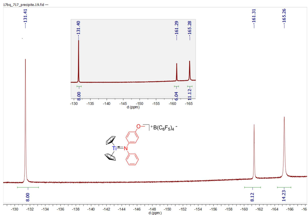
Spectrum 0-433: ^{19}\text{F}\{^1\text{H}\} and ^{19}\text{F} NMR of 55 (470.45 MHz, 300 K, bromobenzene- d_5 )
