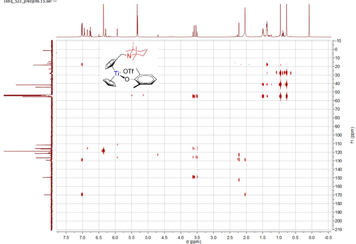
Spectrum 0-217: ^1\text{H} ^{13}\text{C} HMBC of 30 (500.03 MHz / 125.77 MHz, 300 K, dichloromethane- d_2 )
