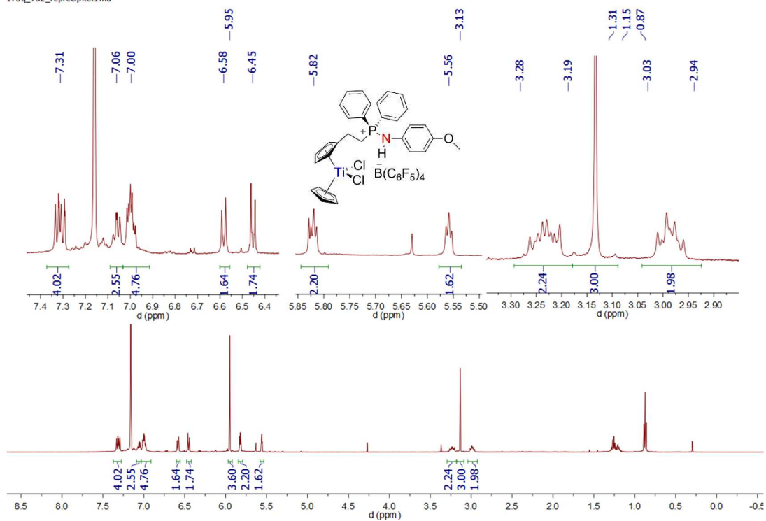
Spectrum 0-510: ^1\text{H} NMR of 61 (500.03 MHz, 300 K, benzene- d_6 )
