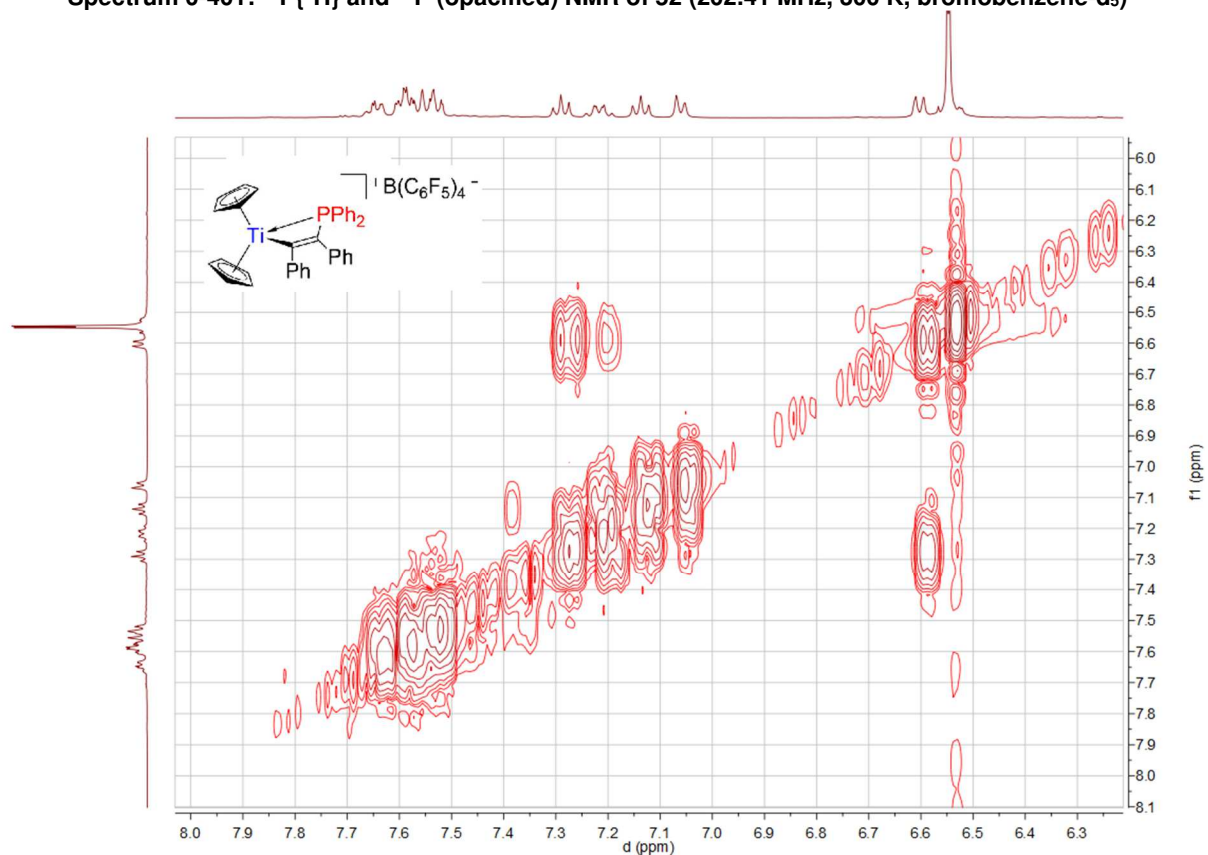
Spectrum 0-402: ^1\text{H} ^1\text{H} COSY of 52 (500.03 MHz, 300 K, 273 K, bromobenzene- d_5 )
