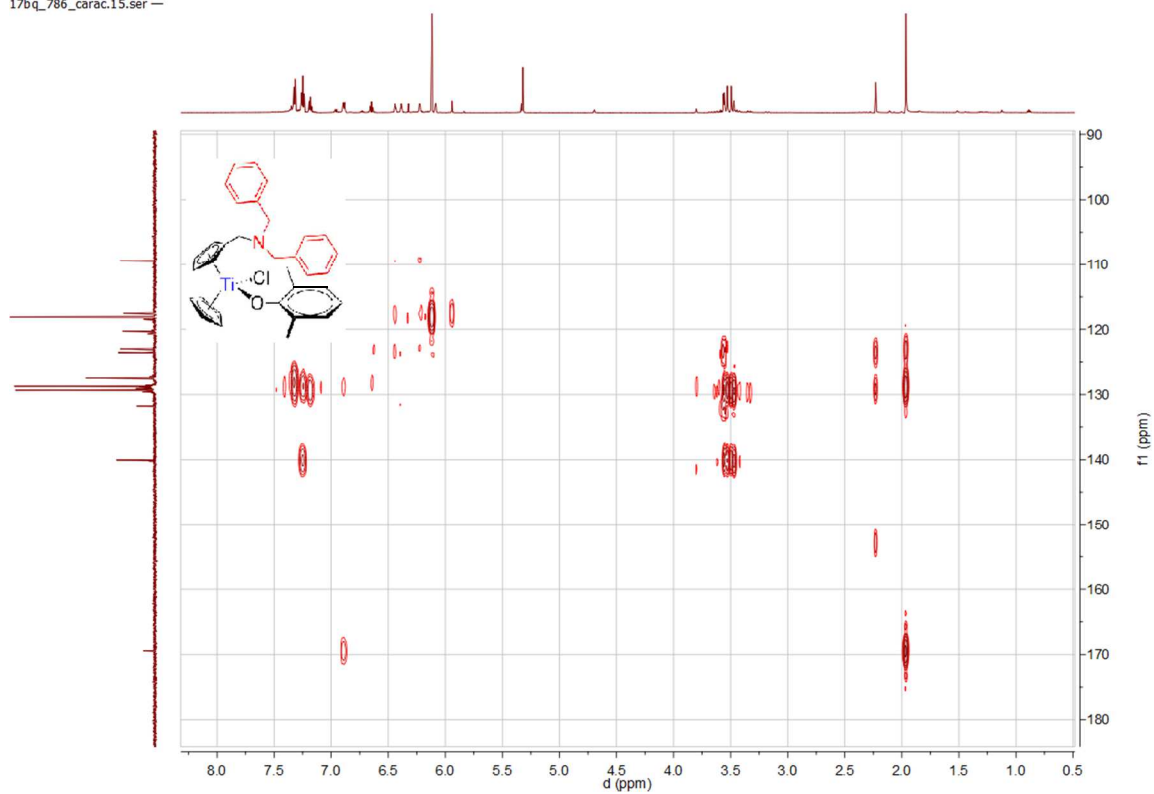
Spectrum 0-186: ^1\text{H} ^{13}\text{C} HMBC of 27 (600.23 MHz / 150.944 MHz, 300 K, dichloromethane- d_2 )
