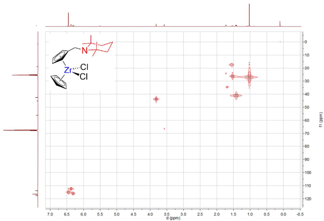
Spectrum 0-160: ^1\text{H} ^{13}\text{C} HMQC of 24 (600.23 MHz / 150.94 MHz, 300 K, tetrahydrofuran- d_8 )
