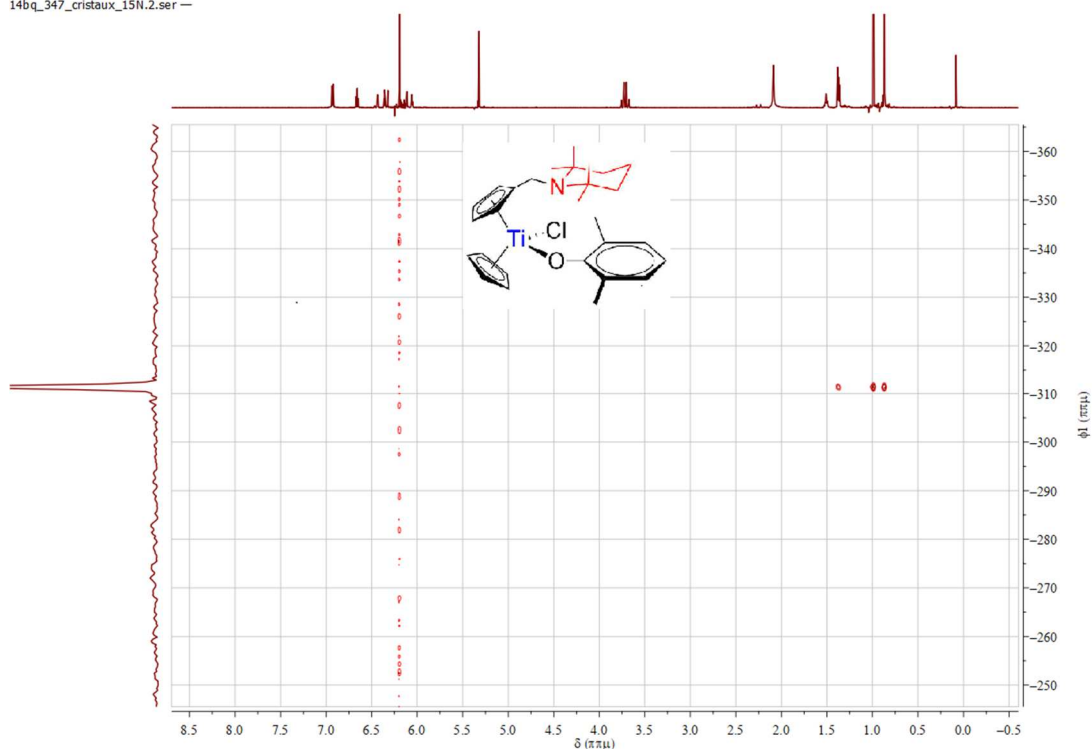
Spectrum 0-205: ^1\text{H} ^{15}\text{N} HMBC of 29 (600.23 MHz / 43.3 MHz, 300 K, dichloromethane- d_2 )
