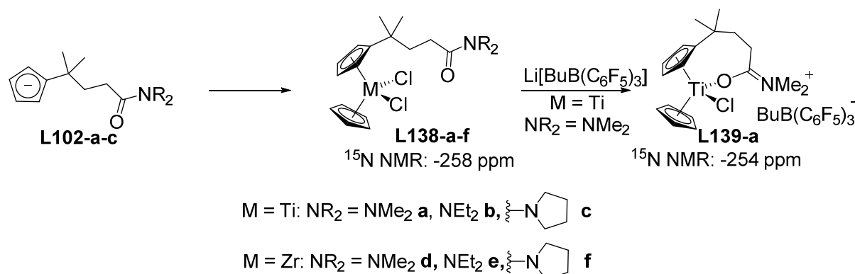
Scheme I-42: carboxamide group 4 metallocenes synthesized by Erker
