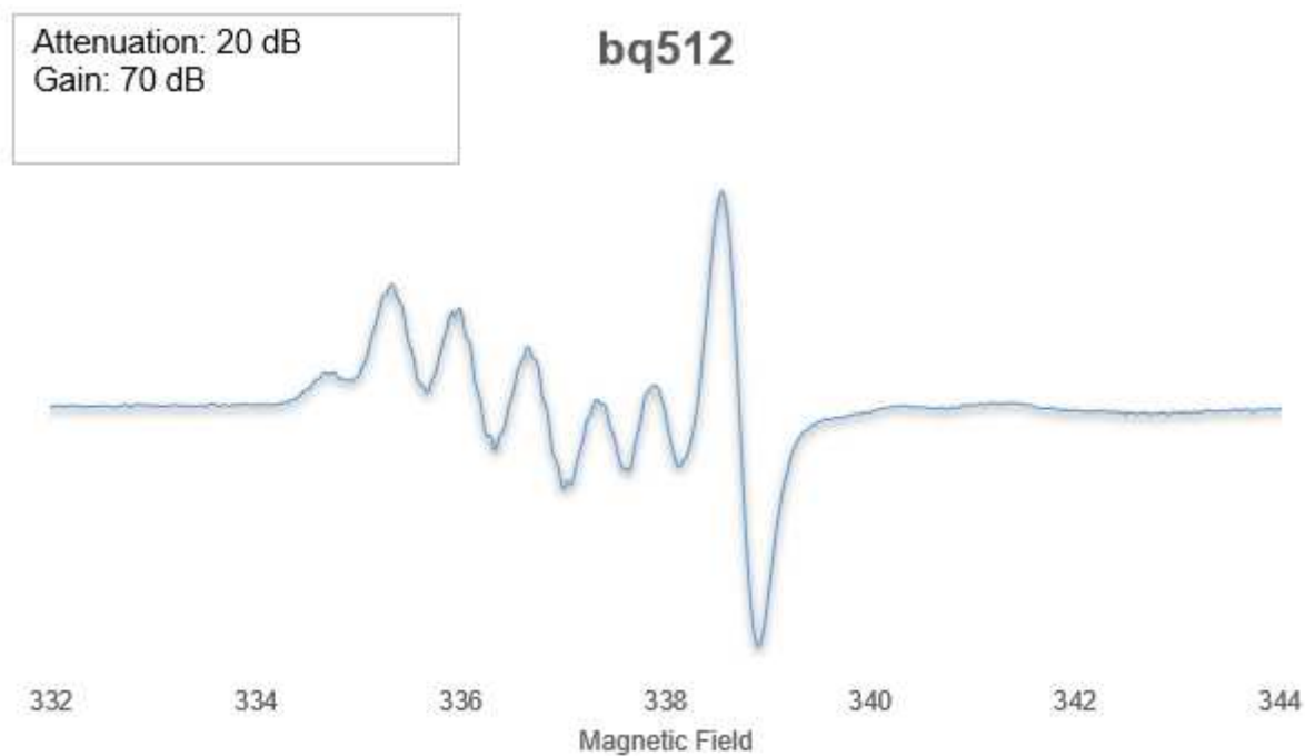
Spectrum 0-425: EPR spectrum of 54 (9.43993 GHz, 295 K, Bromobenzene)
