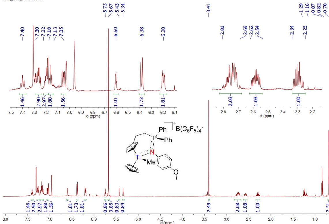
Spectrum 0-547: ^1\text{H} NMR of 64 (600.23 MHz, 360 K, bromobenzene- d_5 )
