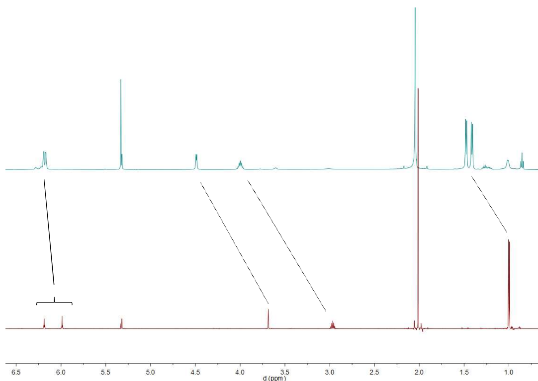
Spectrum III-1: superposition of the ^1\text{H} NMR spectra of 19 (bottom) and after reaction with [\text{Li}][\text{B}(\text{C}_6\text{F}_5)_4] (top) (600.23 MHz, 300 K, dichloromethane- d_2 )
