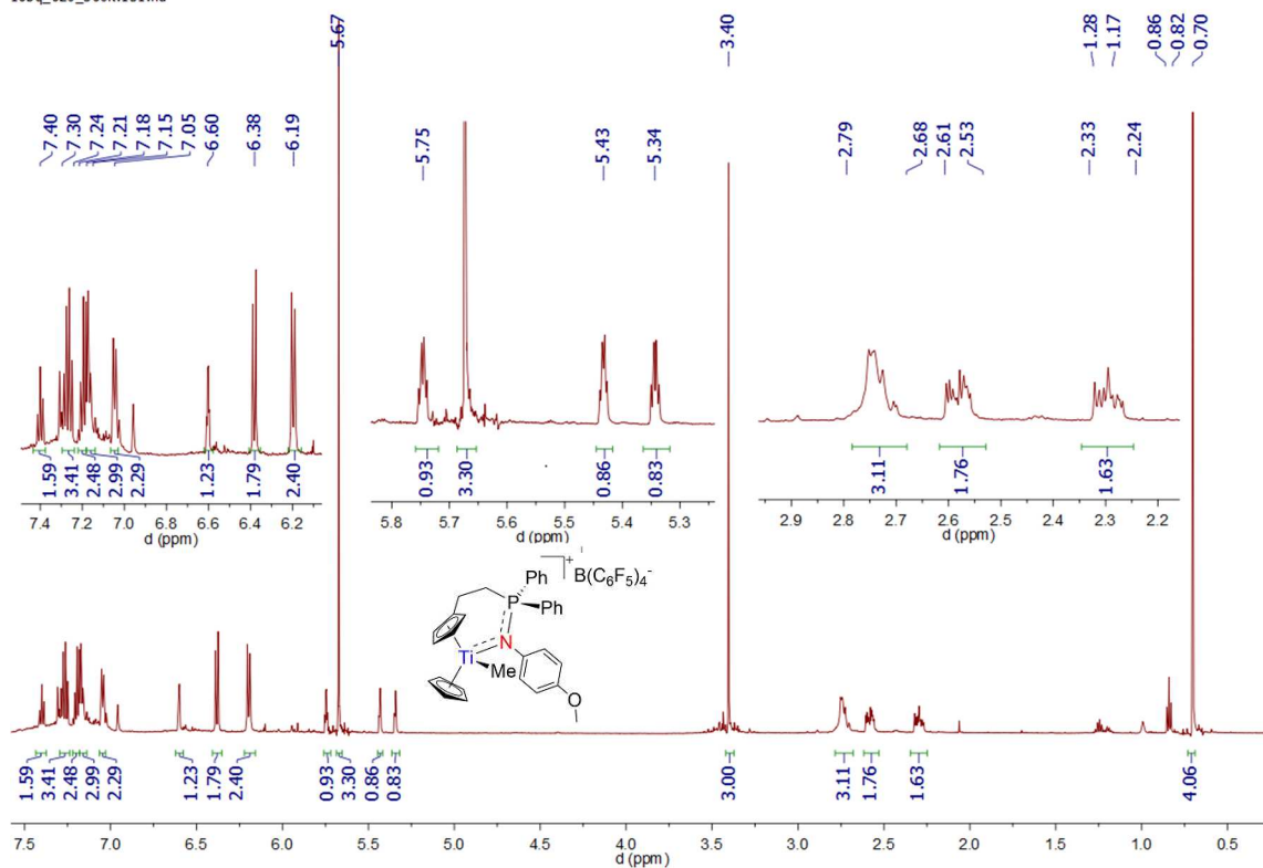
Spectrum 0-548: ^1\text{H}\{^{31}\text{P}\} NMR of 64 (600.23 MHz, 360 K, bromobenzene- d_5 )
