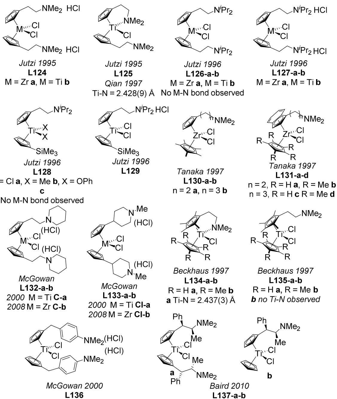
Scheme I-41: screening of various (aminoalkyl)metallocenes of group 4
