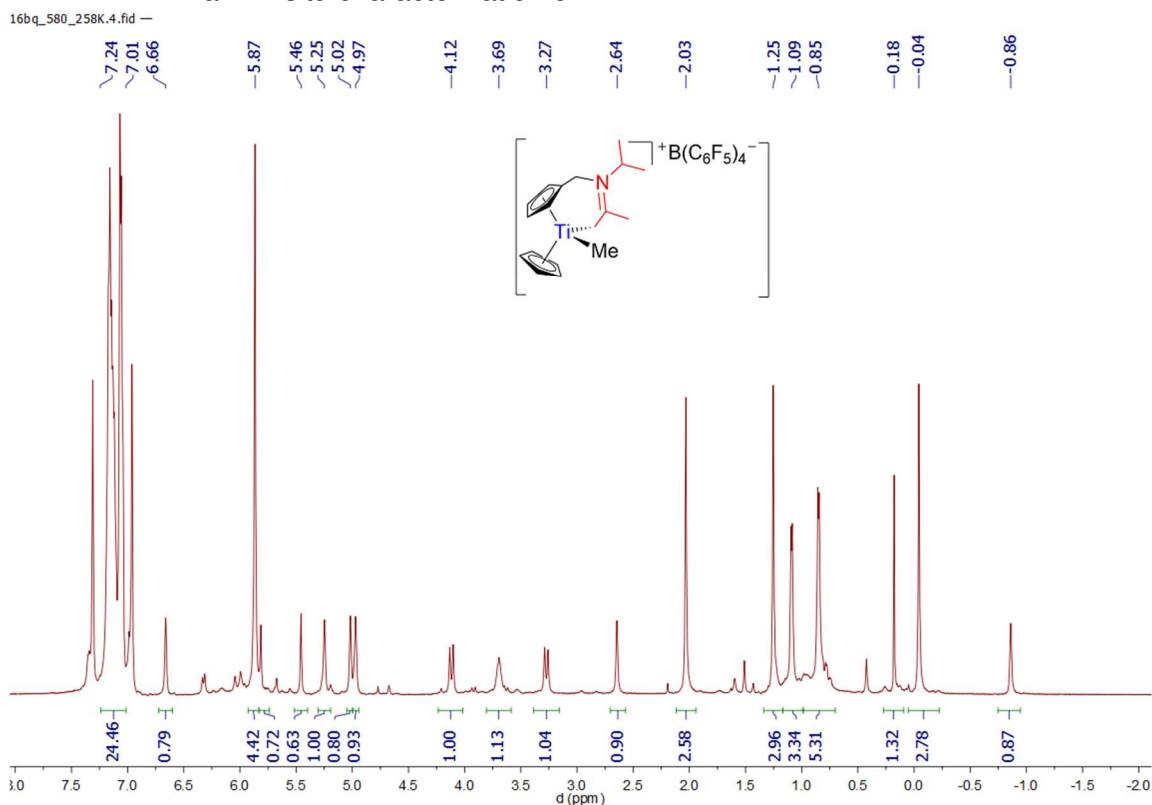
Spectrum 0-314: ^1\text{H} NMR of 42 (500.03 MHz, 258 K, bromobenzene- d_5 )
