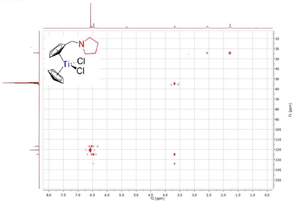
Spectrum 0-44: ^1\text{H} ^{13}\text{C} HMBC of 10 (600.23 MHz / 150.94 MHz, 300 K, dichloromethane- d_2 )
