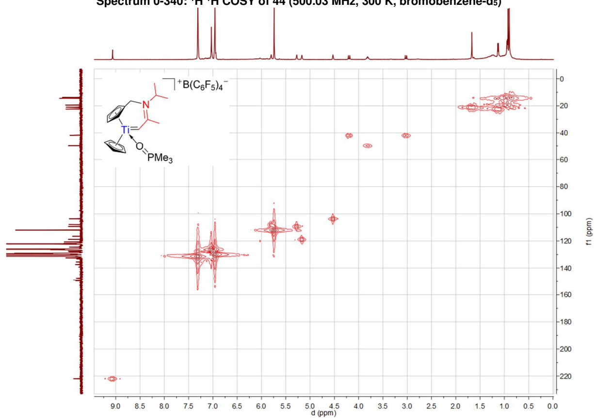
Spectrum 0-341: ^1\text{H} ^{13}\text{C} HMQC of 44 (500.03 MHz / 125.75 MHz, 300 K, bromobenzene- \text{d}_5 )
