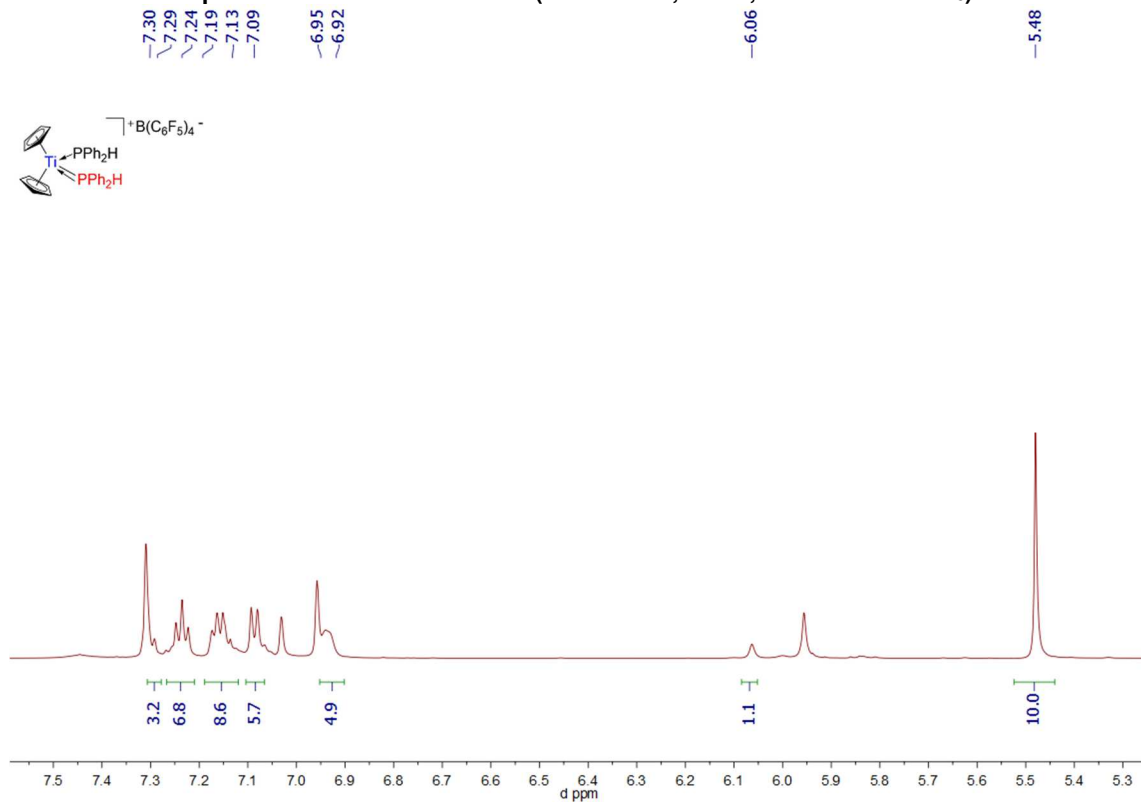
Spectrum 0-378: ^1\text{H}\{^{31}\text{P}\} NMR (top) correlated with ^1\text{H} (bottom) of 50 (500.03 MHz, 300 K, bromobenzene- d_5 )
