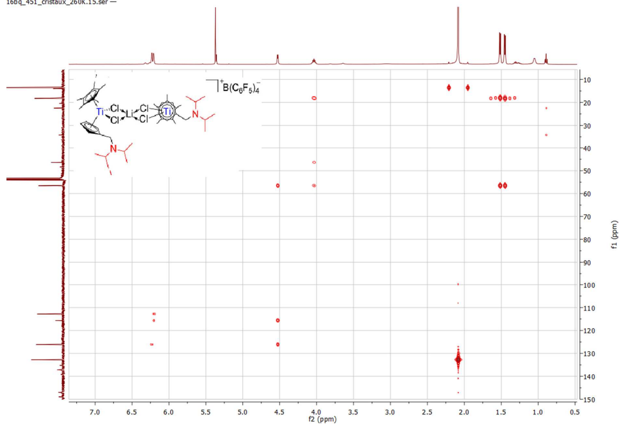
Spectrum 0-170: ^1\text{H} ^{13}\text{C} HMBC of 25 (500.03 MHz / 125.75 MHz, 260 K, dichloromethane- d_2 )
