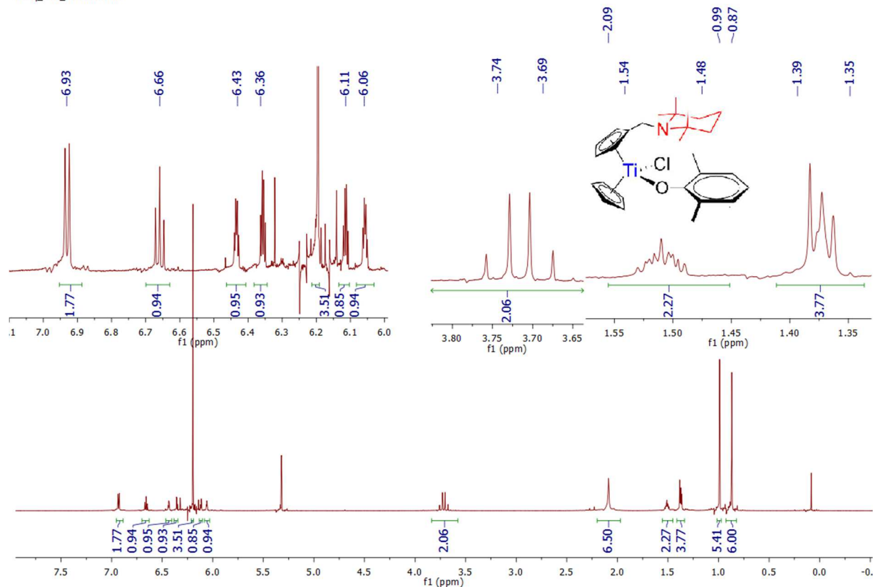
Spectrum 0-200: ^1\text{H} NMR of 29 (600.23 MHz, 300 K, dichloromethane- \text{d}_2 )
