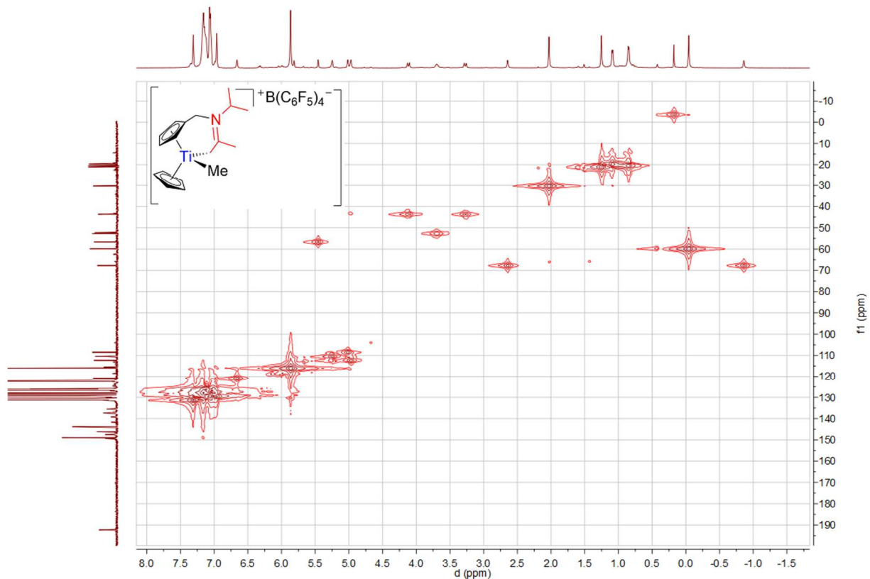
Spectrum 0-318: 1 H 13 C HMQC of 42 (600.23 MHz / 150.94 MHz, 258 K, bromobenzene-d 5 )
