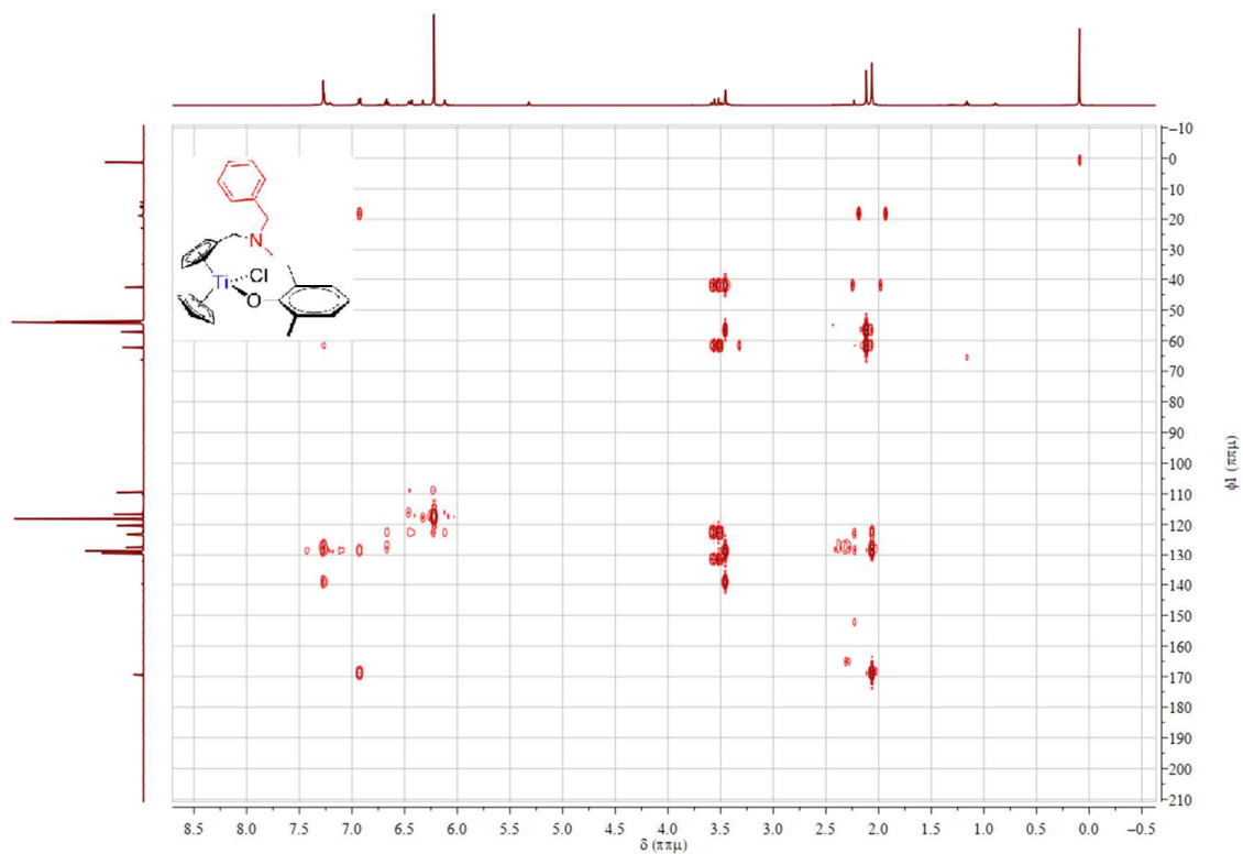
Spectrum 0-179: 1 H 13 C HMBC of 26 (500.03 MHz / 125.77 MHz, 300 K, dichloromethane-d 2 )
