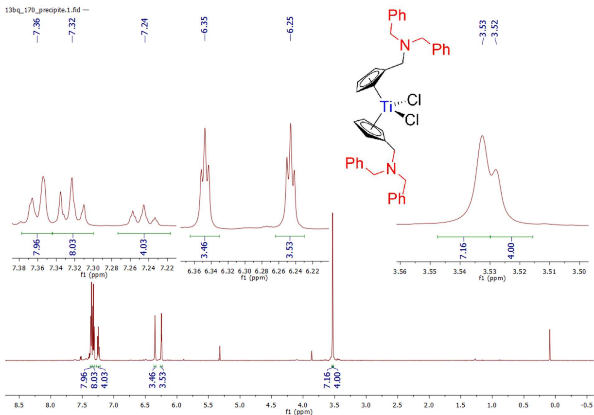
Spectrum 0-125: 1 H NMR of 20 (600.23 MHz, 300 K, dichloromethane-d 2 )
