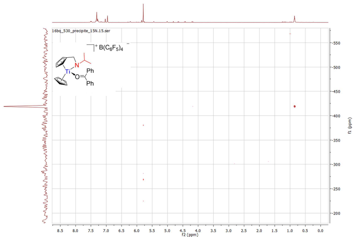
Spectrum 0-307: ^1\text{H} ^{15}\text{N} HMBC of 41 (500.03 MHz / 43.3 MHz, 300 K, bromobenzene- d_5 )
