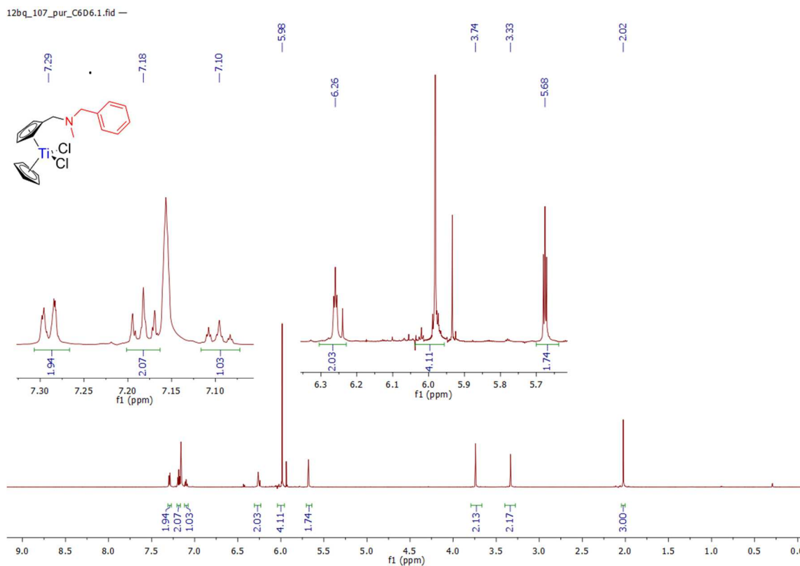
Spectrum 0-31: ^1\text{H} NMR of 9 (600.23 MHz, 300 K, benzene- d_6 )
