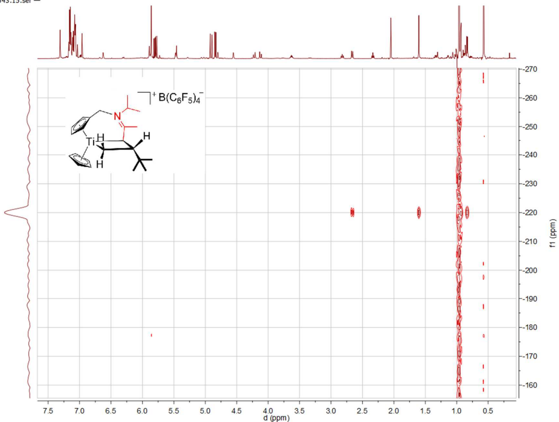
Spectrum 0-371: ^1\text{H} ^{15}\text{N} HMBC of 47 (600.23 MHz / 43.3 MHz, 300 K, bromobenzene- d_5 )
