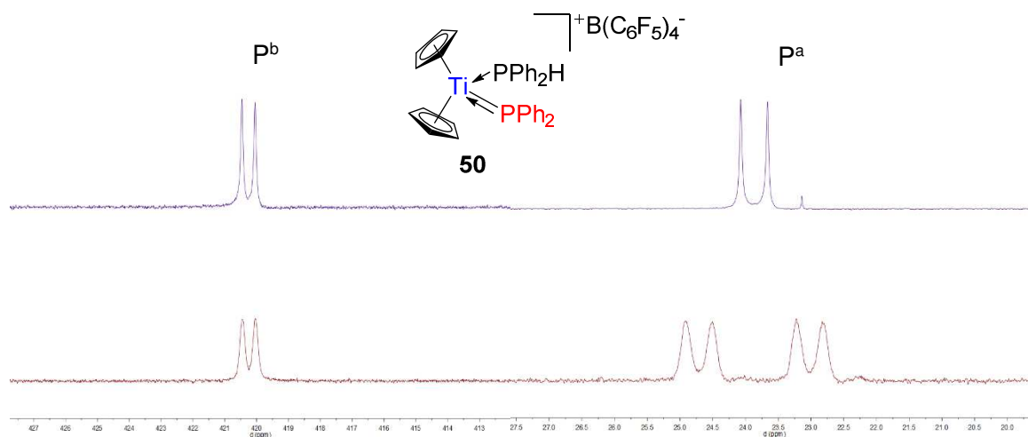
Spectrum IV-3: superposition of the ^{31}\text{P}\{^1\text{H}\} (top) and ^{31}\text{P} (bottom) NMR spectra of 50 (202.46 MHz, 300 K, bromobenzene- \text{d}_5 )
