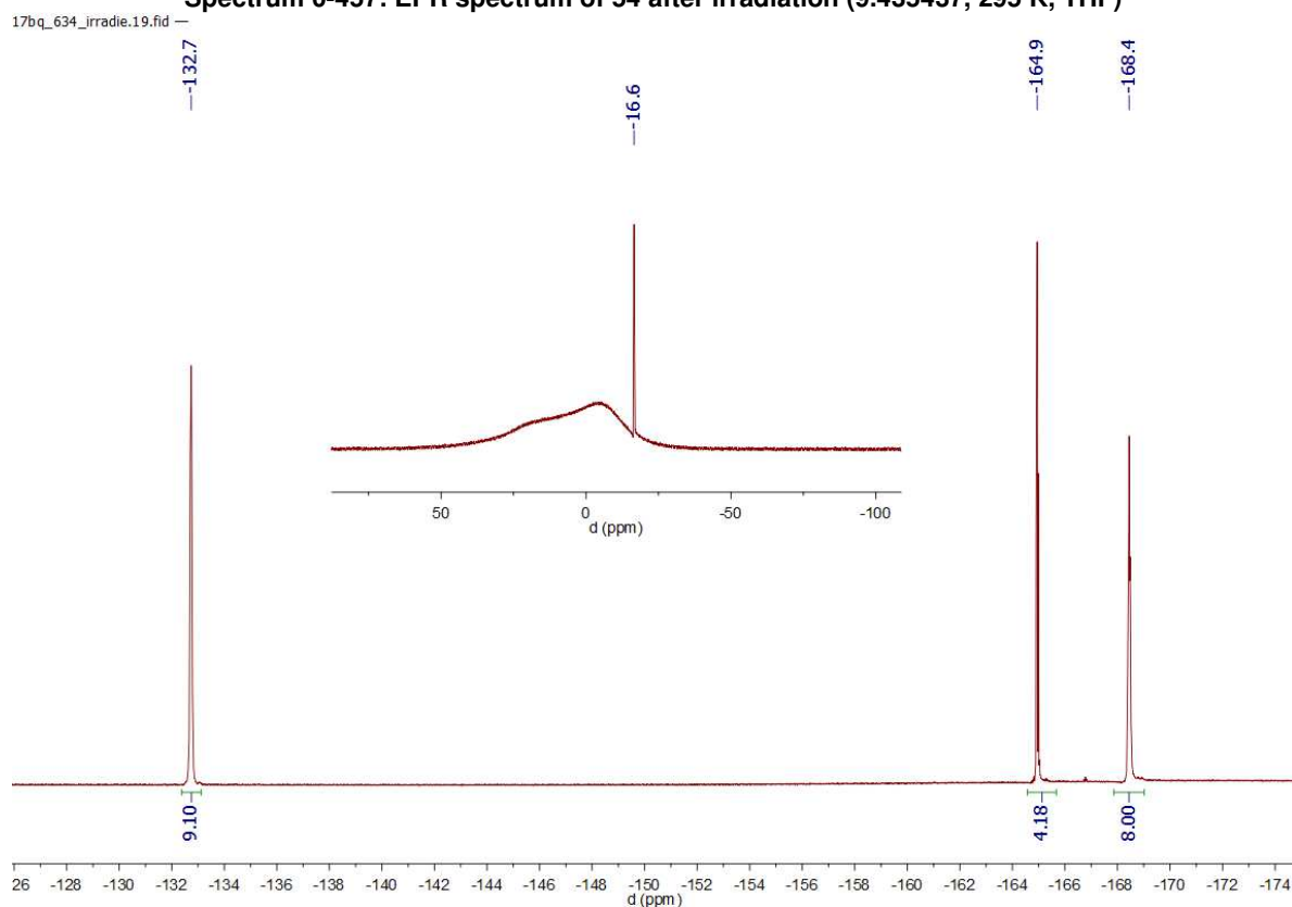
Spectrum 0-458: ^{11}\text{B}\{^1\text{H}\} and ^{19}\text{F}\{^1\text{H}\} NMR spectra of 54 after irradiation (500.03 MHz, 300 K, tetrahydrofuran- d_8 )
