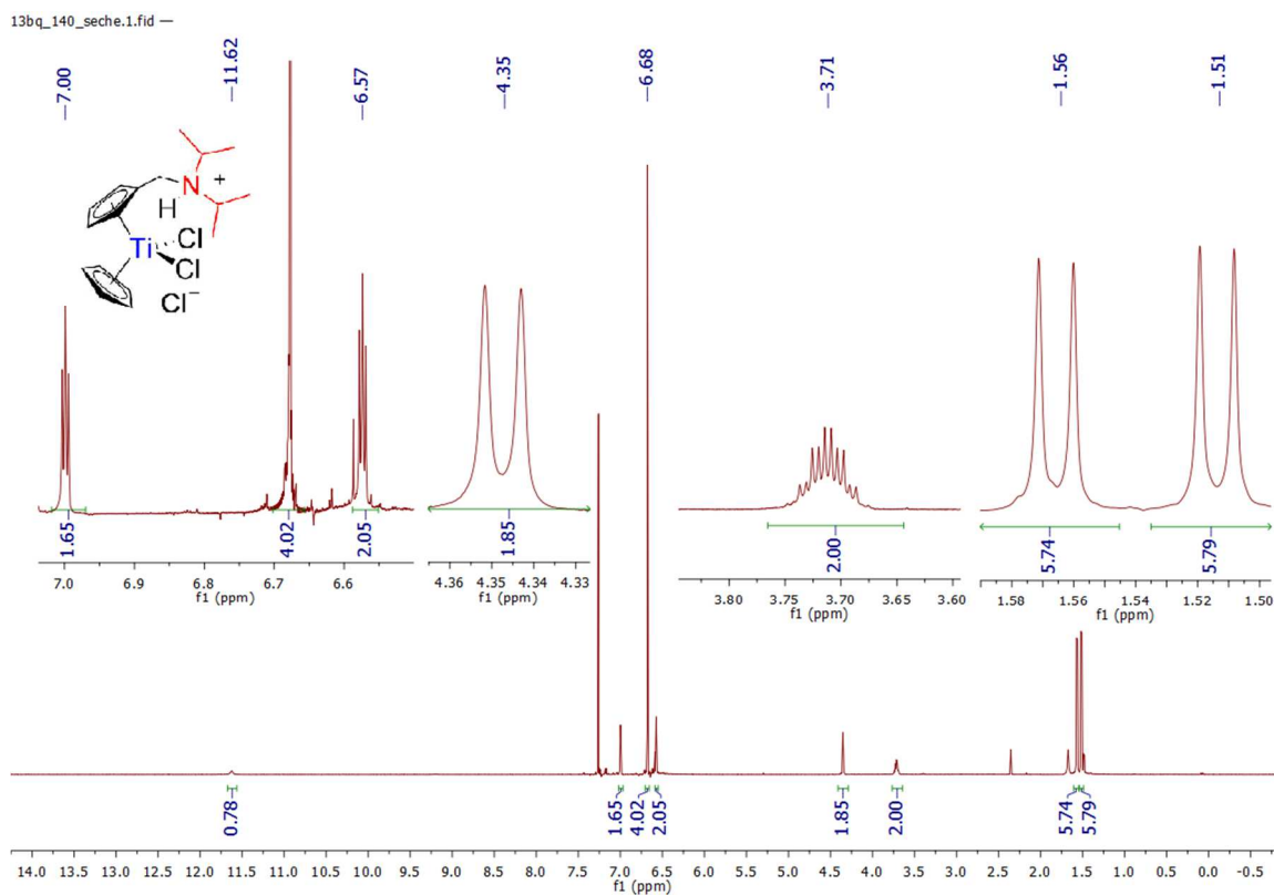
Spectrum 0-100: 1 H NMR of 17 (600.23 MHz, 300 K, chloroform-d 1 )
