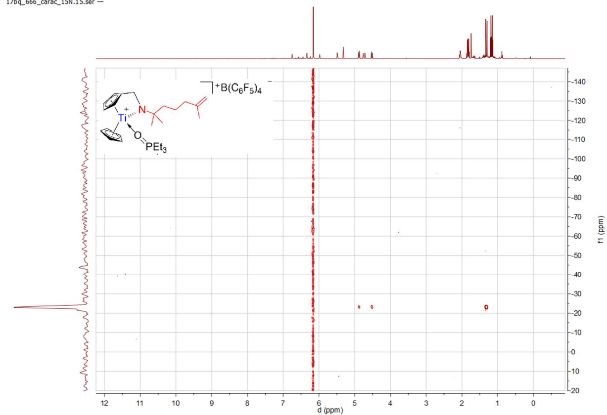
Spectrum 0-268: ^1\text{H} ^{15}\text{N} HMBC of 37 (600.23 MHz / 43.3 MHz, 300 K, dichloromethane- d_2 )
