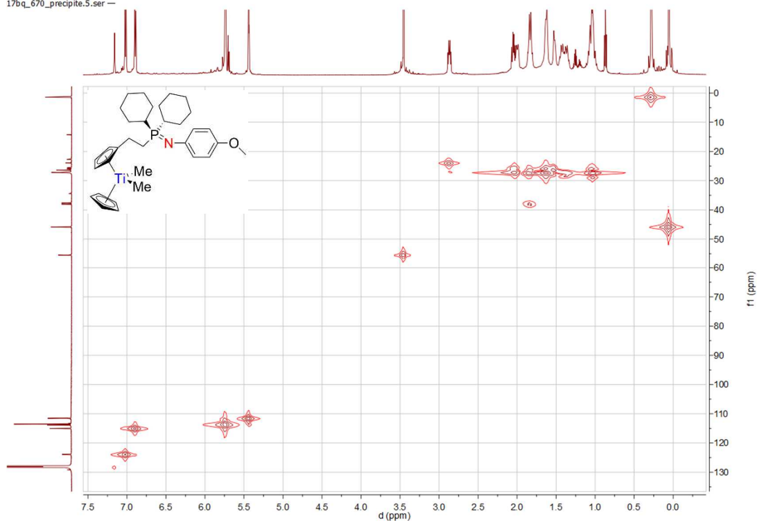
Spectrum 0-537: 1 H 13 C HMQC of 63 (500.03 MHz / 125.75 MHz, 300 K, benzene-d 6 )
