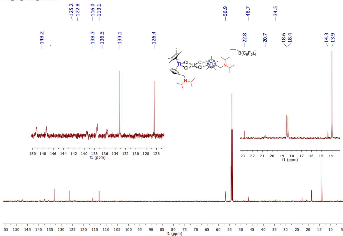
Spectrum 0-167: ^{13}\text{C}\{^1\text{H}\} NMR of 25 (125.75 MHz, 260 K, dichloromethane- d_2 )
