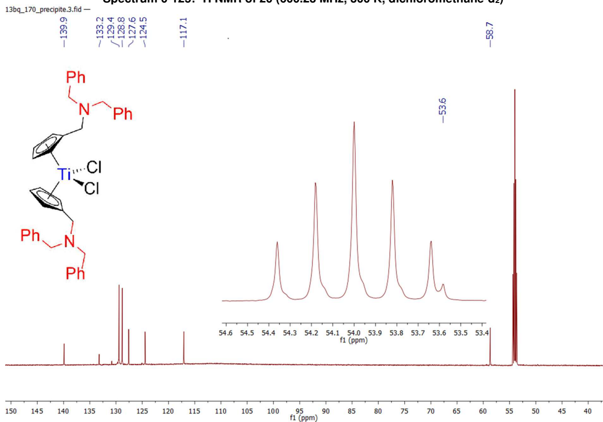
Spectrum 0-126: 13 C{ 1 H} NMR of 20 (150.94 MHz, 300 K, dichloromethane-d 2 )
