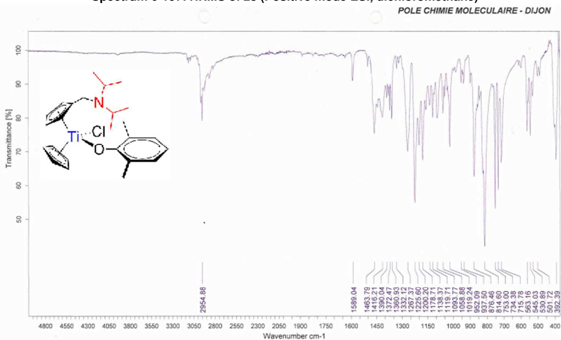
Spectrum 0-197: HRMS of 28 (Positive mode ESI, dichloromethane)
