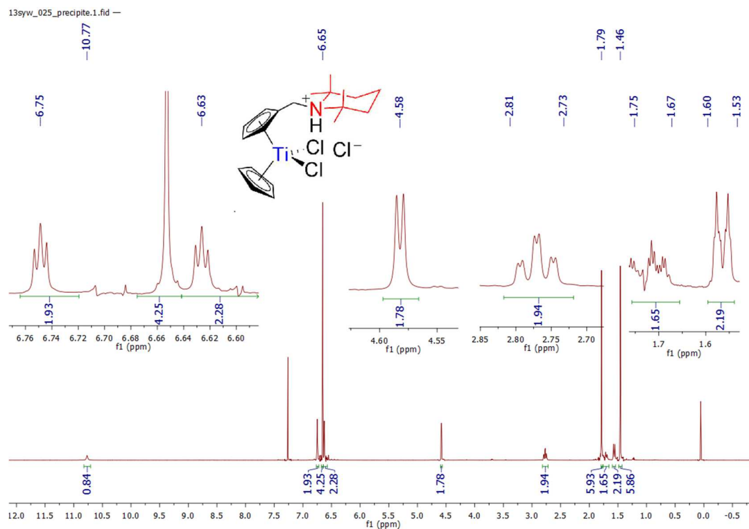
Spectrum 0-108: 1 H NMR of 18 (600.23 MHz, 300 K, chloroform-d 1 )
