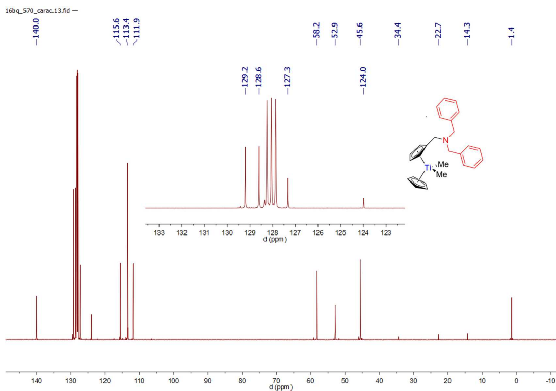
Spectrum 0-229: ^{13}\text{C}\{^1\text{H}\} NMR of 33 (125.75 MHz, 300 K, benzene- d_6 )
