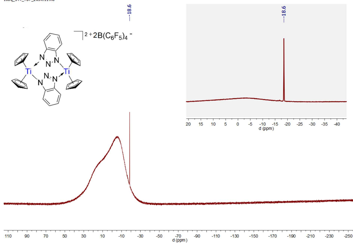
Spectrum 0-440: ^{11}\text{B}\{^1\text{H}\} and ^{11}\text{B} NMR of 56 (160.43 MHz, 300 K, tetrahydrofuran- d_5 )
