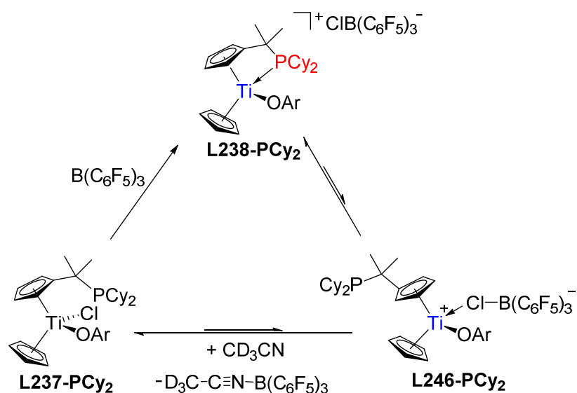
Scheme III-4: an example of chloride abstraction with \text{B}(\text{C}_6\text{F}_5)_3
