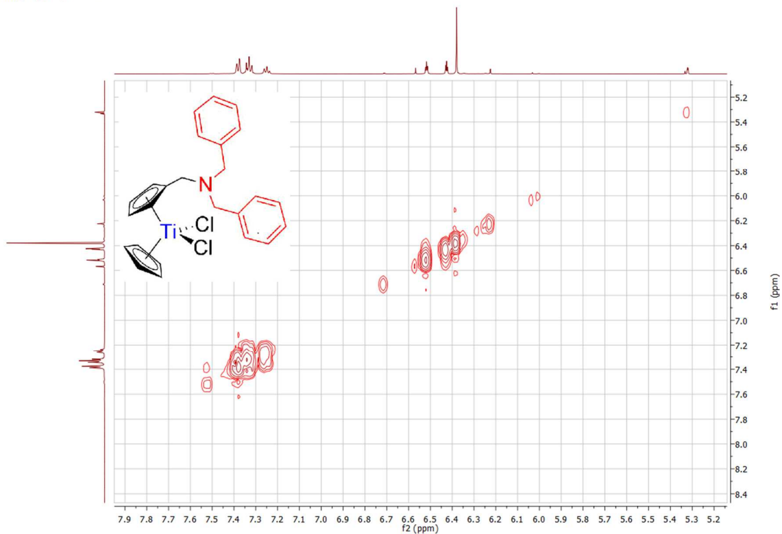
Spectrum 0-51: ^1\text{H} ^1\text{H} COSY of 11 (600.23 MHz, 300 K, dichloromethane- d_2 )
