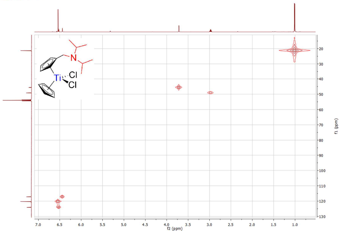
Spectrum 0-61: ^1\text{H} ^{13}\text{C} HMQC of 12 (600.23 MHz / 150.94 MHz, 300 K, dichloromethane- d_2 )
