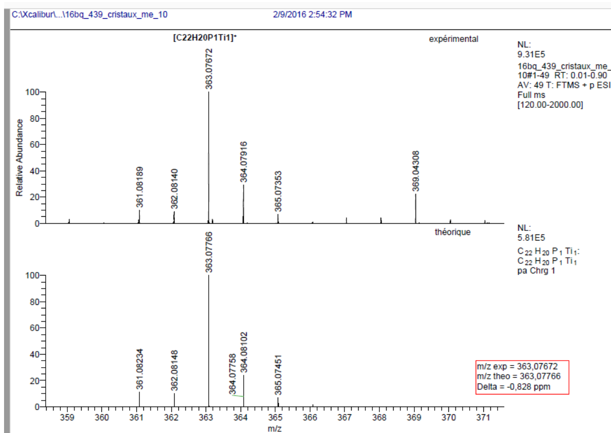
Spectrum 0-387: HRMS of 50 (Positive mode ESI, dichloromethane)
