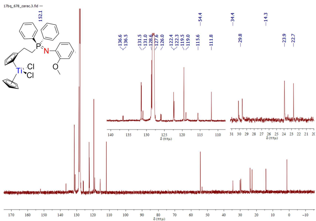
Spectrum 0-478: ^{13}\text{C}\{^1\text{H}\} NMR of 58 (125.75 MHz, 300 K, benzene- d_6 )
