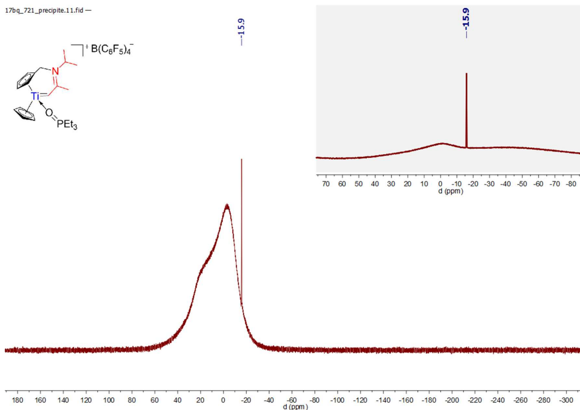
Spectrum 0-356: ^{11}\text{B}\{^1\text{H}\} and ^{11}\text{B} (opacified) NMR of 45 (160.42 MHz, 300 K, bromobenzene- d_5 )
