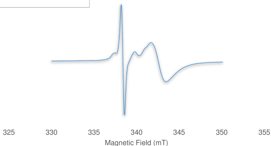
Spectrum IV-9: EPR spectrum of the catalytic hydrogenation of diphenylacetylene with 53 (9.430654 GHz, 295 K, bromobenzene)
