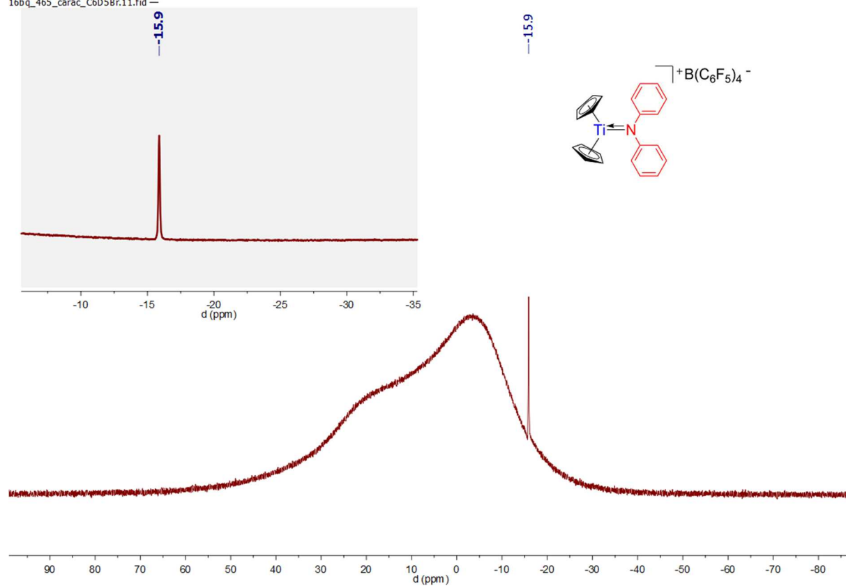
Spectrum 0-414: 11 B{ 1 H} and 11 B NMR of 53 (160.43 MHz, 300 K, bromobenzene-d 5 )
