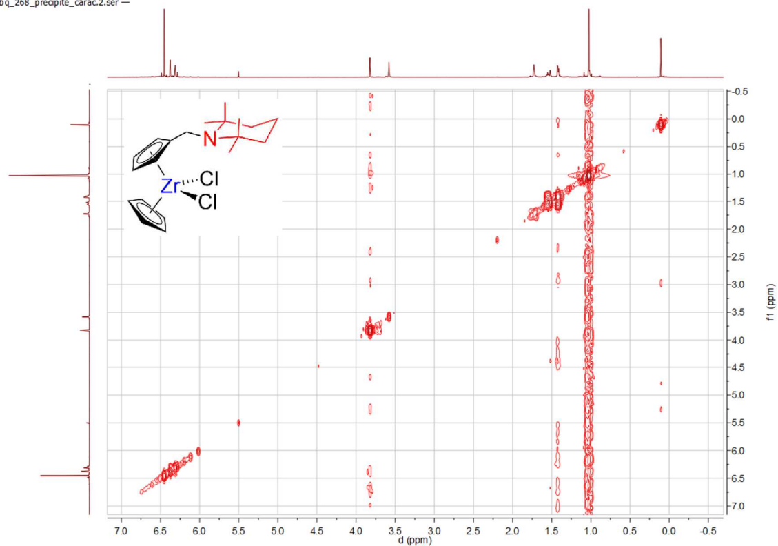
Spectrum 0-159: ^1\text{H} ^1\text{H} COSY of 24 (600.23 MHz, 300 K, tetrahydrofuran- d_8 )
