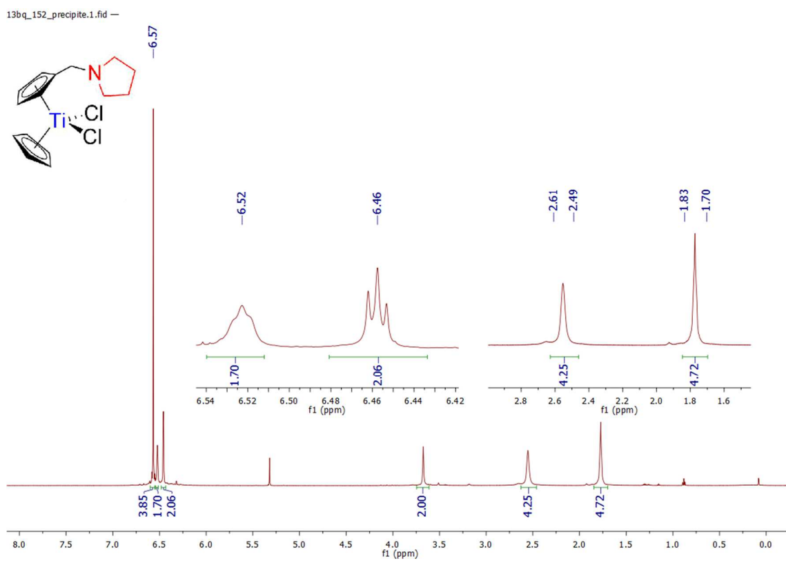
Spectrum 0-40: ^1\text{H} NMR of 10 (600 MHz, 300 K, dichloromethane- d_2 )
