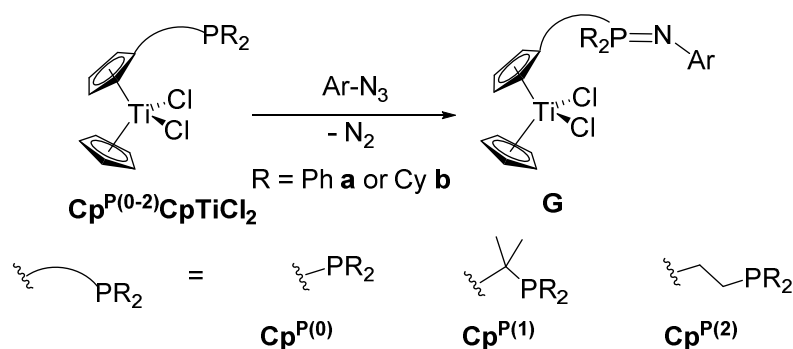
Scheme V-2: synthetic approach to titanocenyl iminophosphoranes
