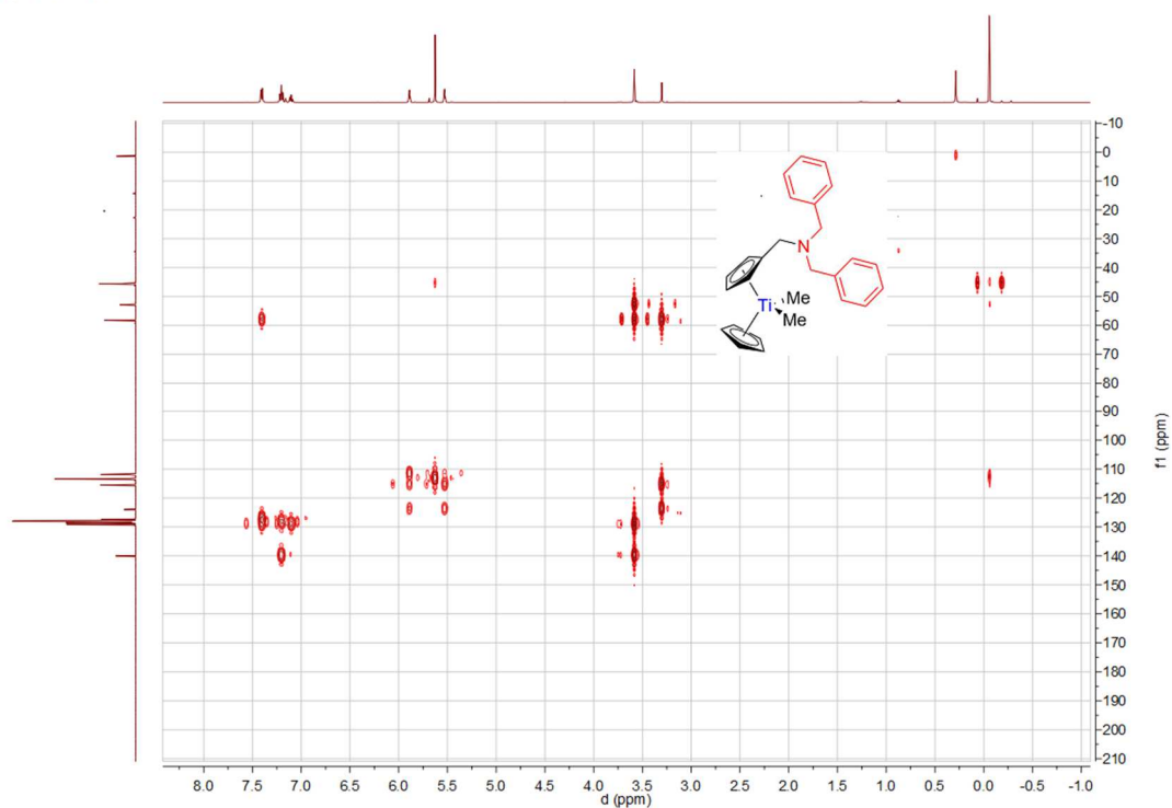
Spectrum 0-232: 1 H 13 C HMBC of 33 (500.03 MHz / 125.75 MHz, 300 K, benzene-d 6 )
