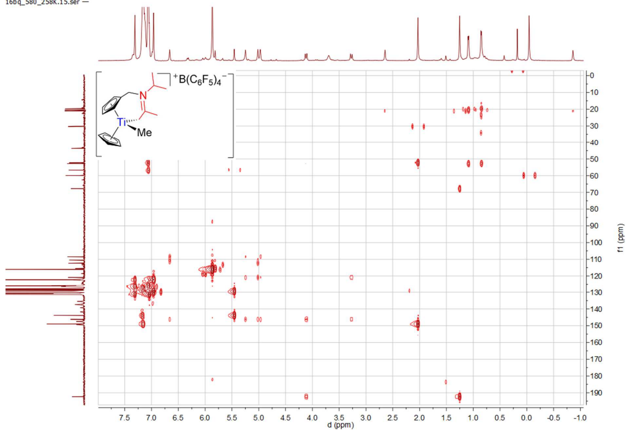
Spectrum 0-319: 1 H 13 C HMBC of 42 (600.23 MHz / 150.94 MHz, 258 K, bromobenzene-d 5 )
