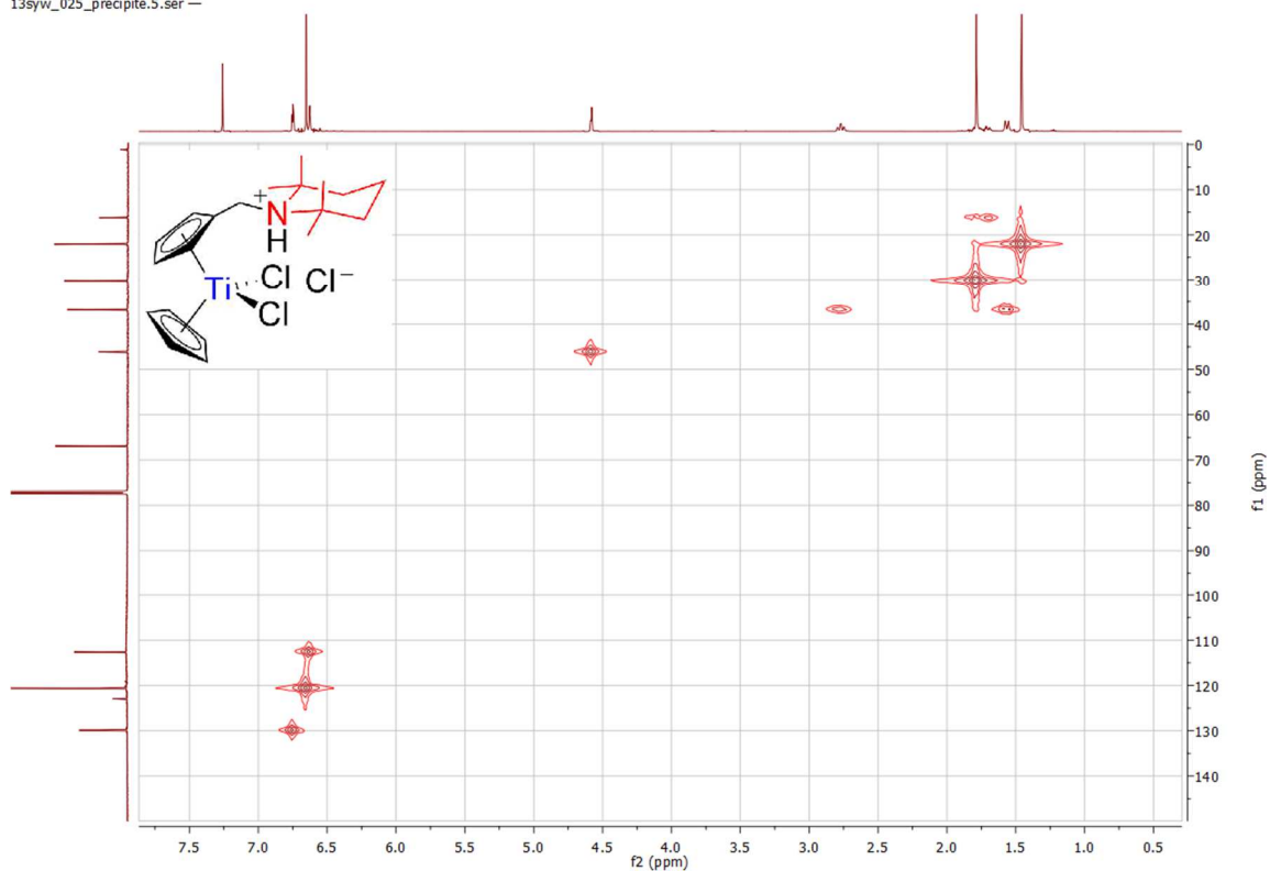
Spectrum 0-111: ^1\text{H} ^{13}\text{C} HMQC of 18 (600.23 MHz / 150.94 MHz, 300 K, chloroform- d_1 )
