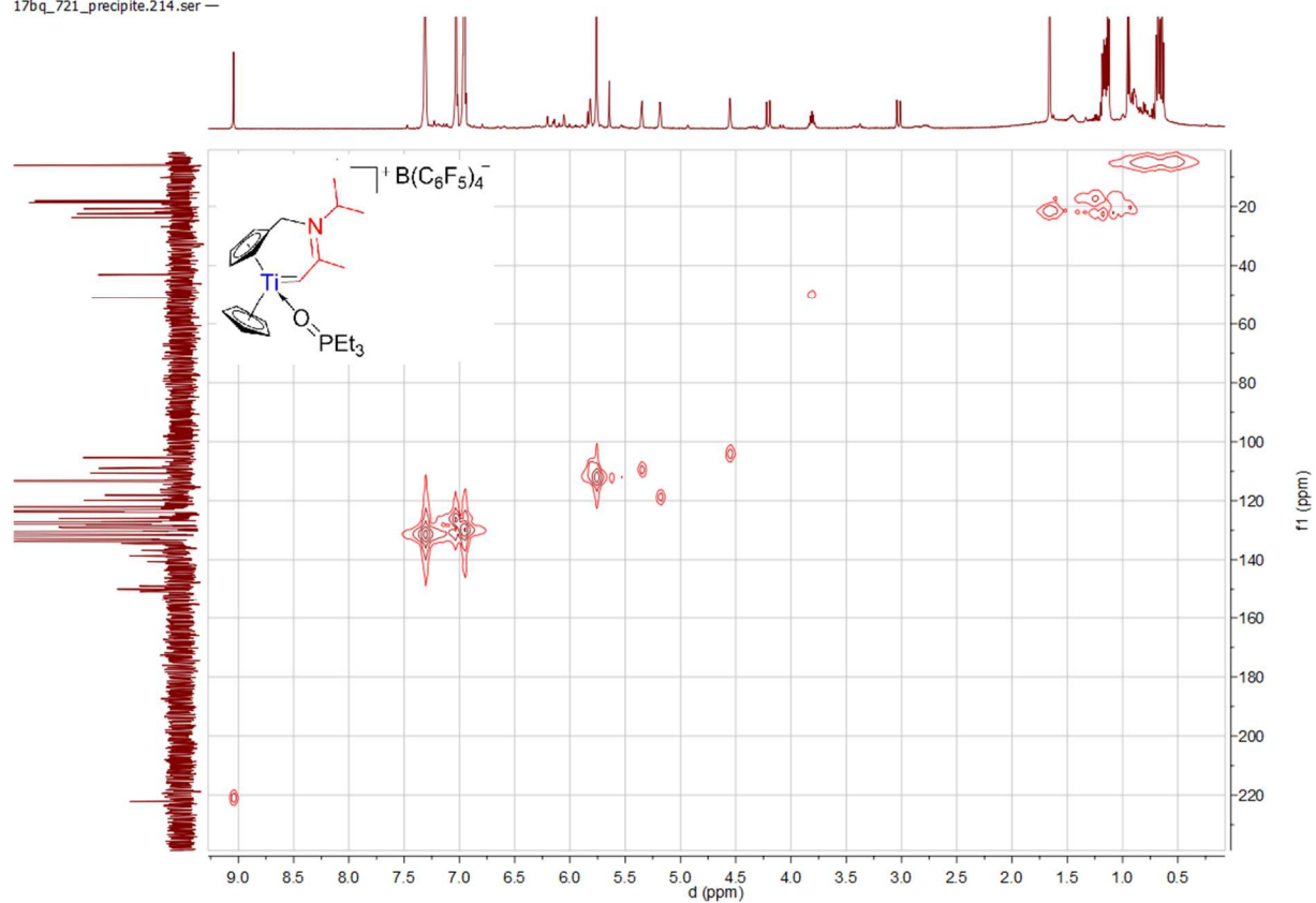
Spectrum 0-353: 1 H 13 C HMQC of 45 (500.03 MHz / 125.75 MHz, 300 K, bromobenzene-d 5 )
