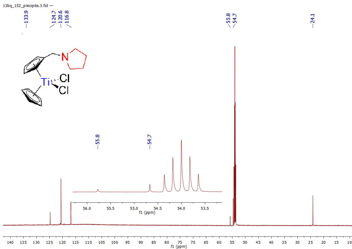
Spectrum 0-41: ^{13}\text{C}\{^1\text{H}\} NMR of 10 (150.94 MHz, 300 K, dichloromethane- d_2 )
