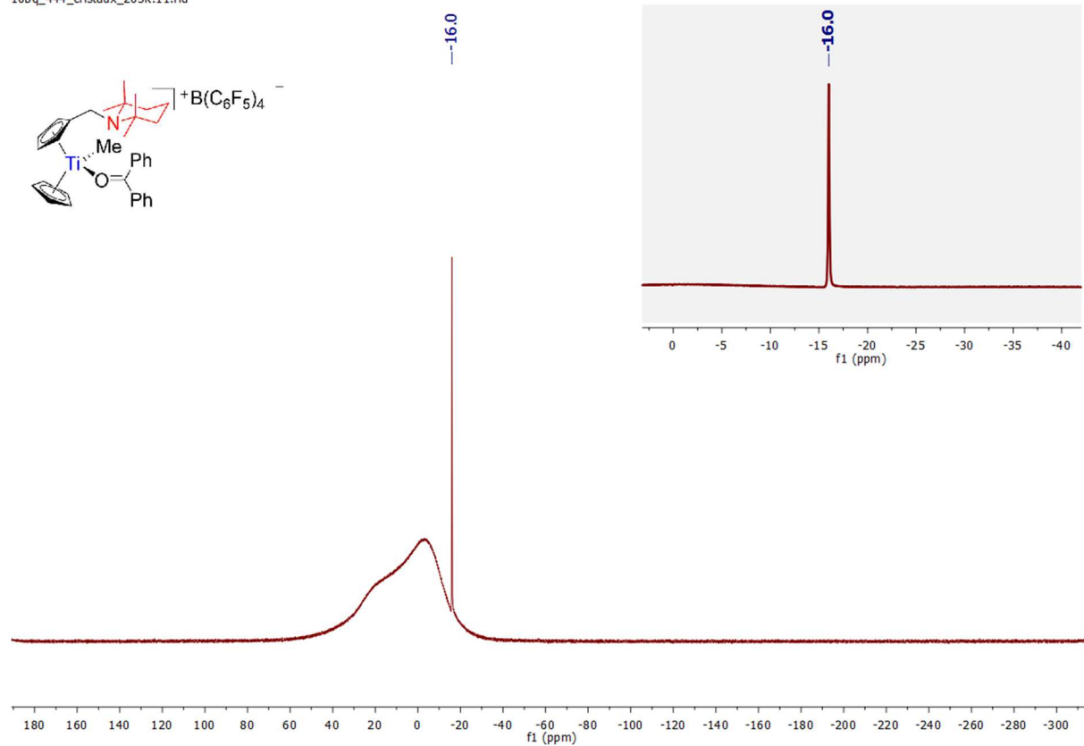
Spectrum 0-278: 11 B{ 1 H} and 11 B (opacified) NMR of 38 (160.42 MHz, 263 K, bromobenzene-d 5 )
