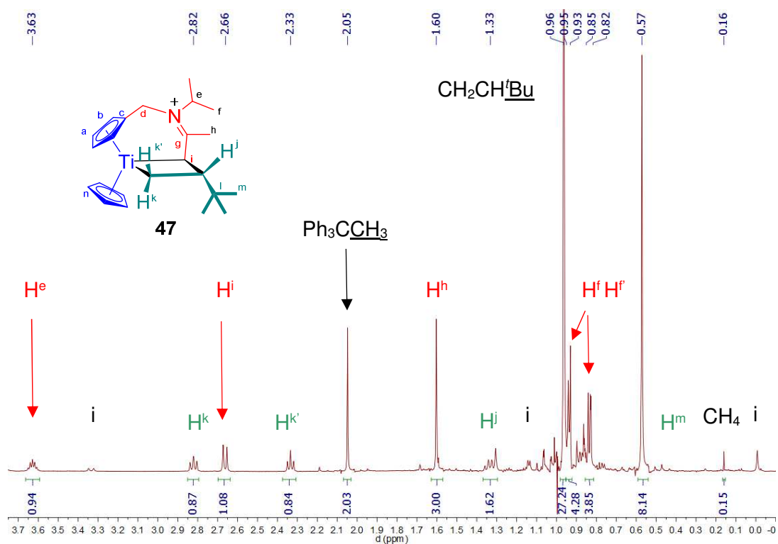
Spectrum III-14: ^1H NMR of 47 [3.9-0.0 ppm] (600.23 MHz, 300 K, bromobenzene- d_5 )
