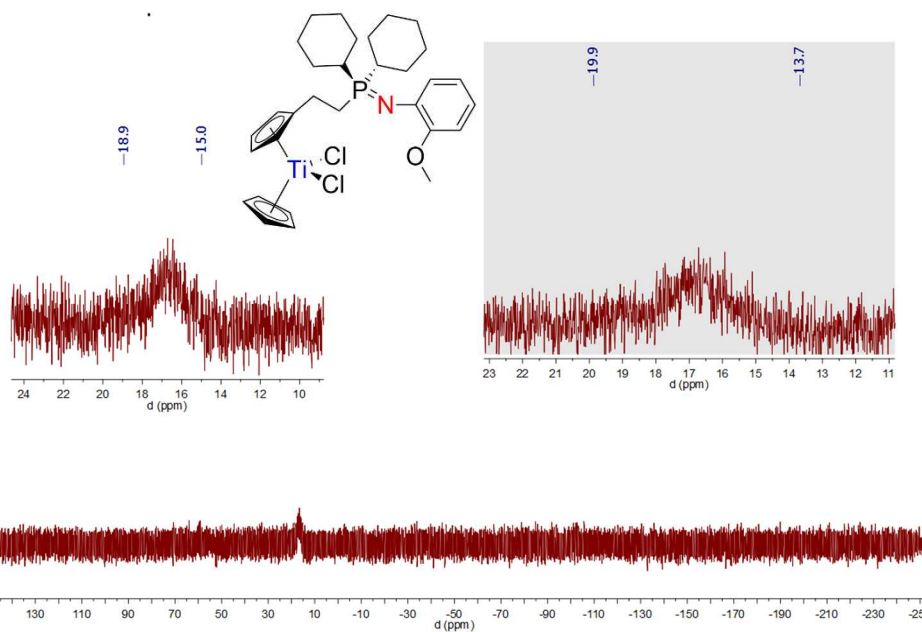
Spectrum 0-505: ^{31}\text{P}\{^1\text{H}\} and ^{31}\text{P} (opacified) NMR of 60 (202.41 MHz, 300 K, benzene- d_6 )
