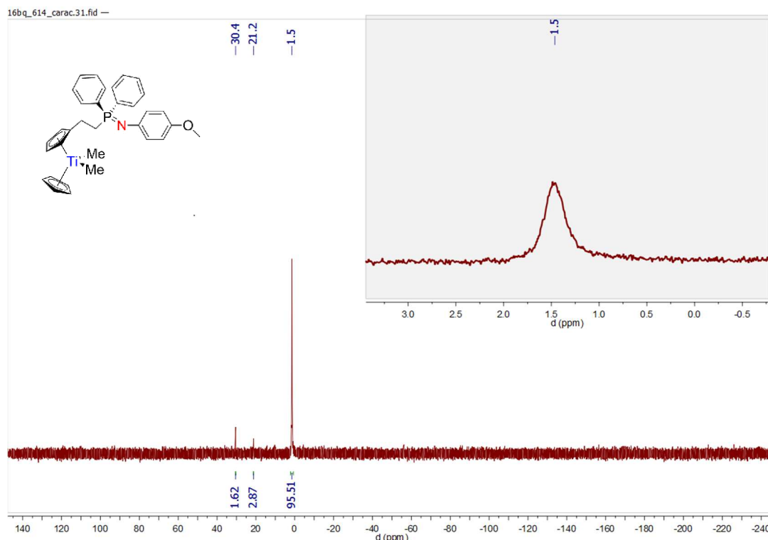
Spectrum 0-528: ^{31}\text{P}\{^1\text{H}\} and ^{31}\text{P} (opacified) NMR of 62 (202.46 MHz, 300 K, benzene- d_6 )
