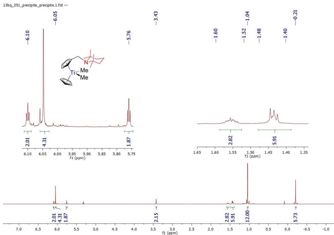
Spectrum 0-244: 1 H NMR of 35 (600.23 MHz, 300 K, dichloromethane-d 2 )
