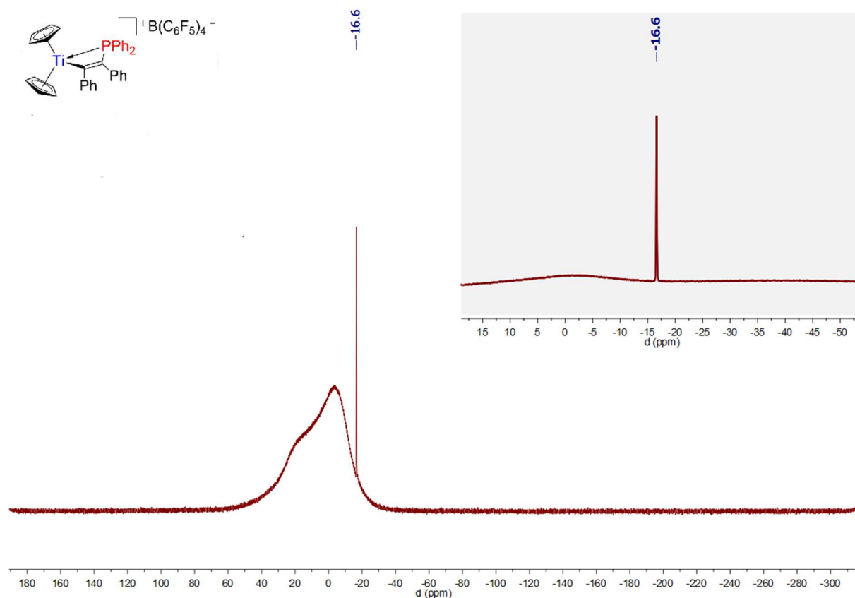
Spectrum 0-405: ^{11}\text{B}\{^1\text{H}\} and ^{11}\text{B} NMR of 52 (160.43 MHz, 300 K, bromobenzene- d_5 )
