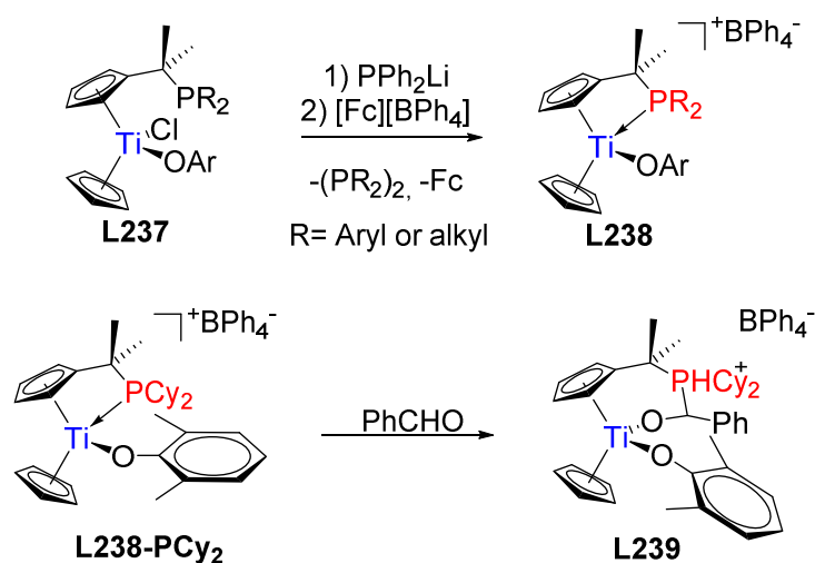
Scheme I-74: Ti-based OmFLP reported by Erker and Le Gendre
