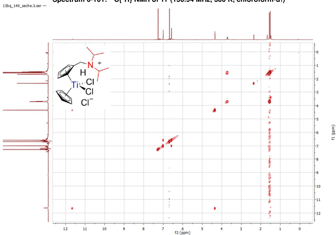
Spectrum 0-102: ^1\text{H} ^1\text{H} COSY of 17 (600.23 MHz, 300 K, chloroform- d_1 )
