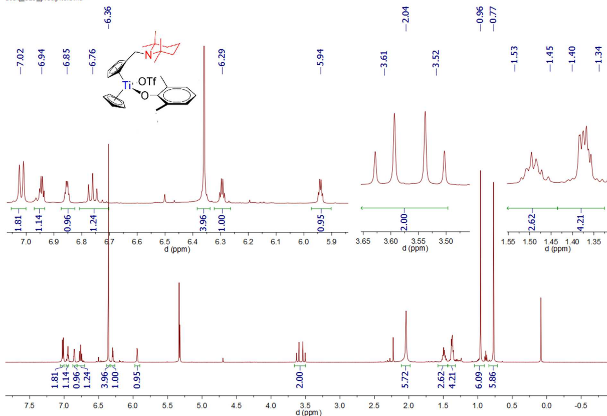
Spectrum 0-213: 1 H NMR of 30 (500.03 MHz, 300 K, dichloromethane-d 2 )
