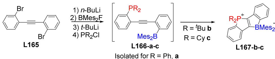
Scheme I-53: Yamaguchi's synthesis of \pi -ladder-conjugated skeleton
