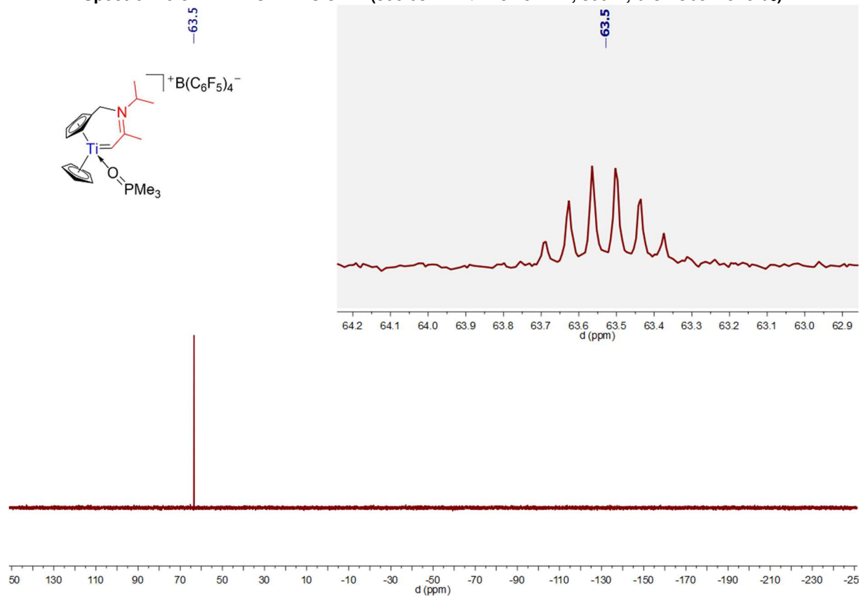
Spectrum 0-343: ^{31}\text{P}\{^1\text{H}\} and ^{31}\text{P} (opacified) NMR of 44 (202.46 MHz, 300 K, bromobenzene- d_5 )
