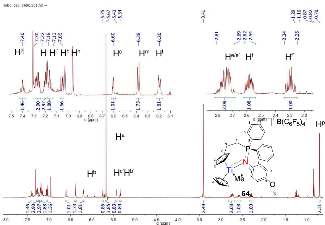
Spectrum V-5: ^1\text{H} NMR spectrum of 64 (600.23 MHz, 360 K, bromobenzene- d_5 )
