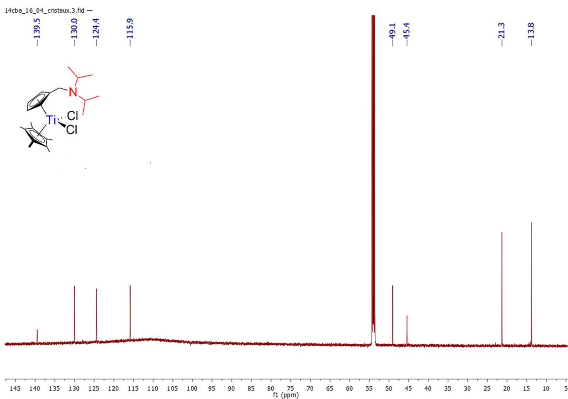
Spectrum 0-117: ^{13}\text{C}\{^1\text{H}\} NMR of 19 (150.94 MHz, 300 K, dichloromethane- d_2 )
