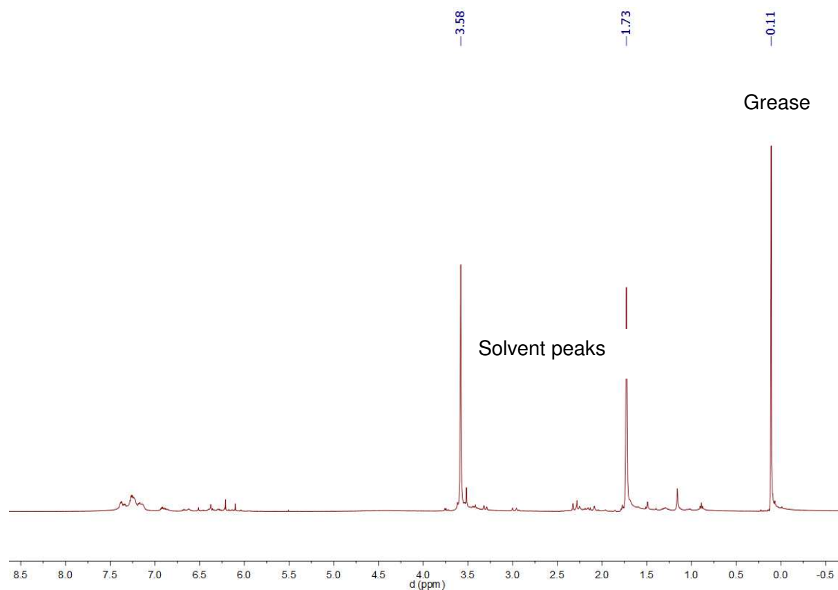
Spectrum 0-211: 1 H NMR spectrum of 29-III (500.53 MHz, 300K, tetrahydrofuran-d 8 )
