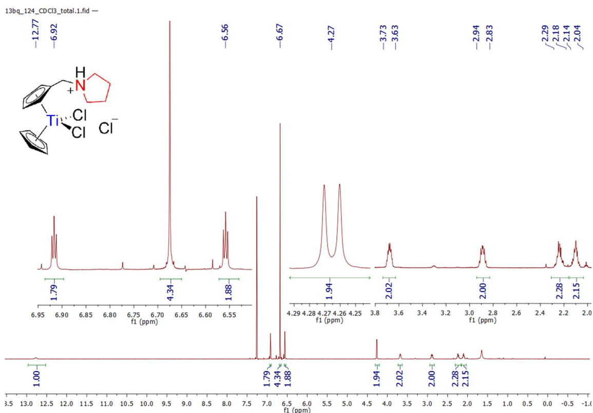
Spectrum 0-84: 1 H NMR of 15 (600 MHz, 300 K, chloroform-d 1 )
