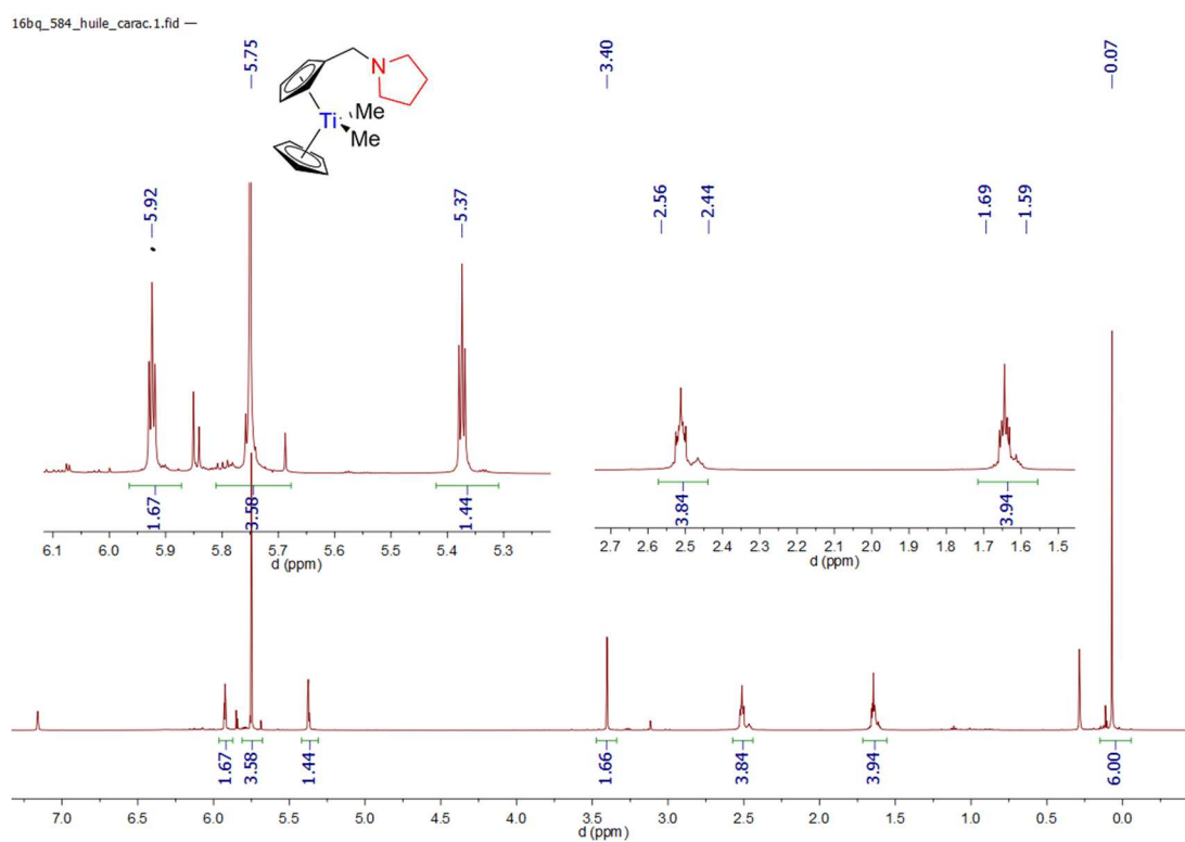
Spectrum 0-221: ^1\text{H} NMR of 32 (500.03 MHz, 300 K, benzene- \text{d}_6 )
