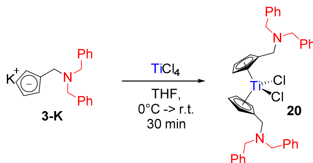
Scheme II-17: synthesis of 20
