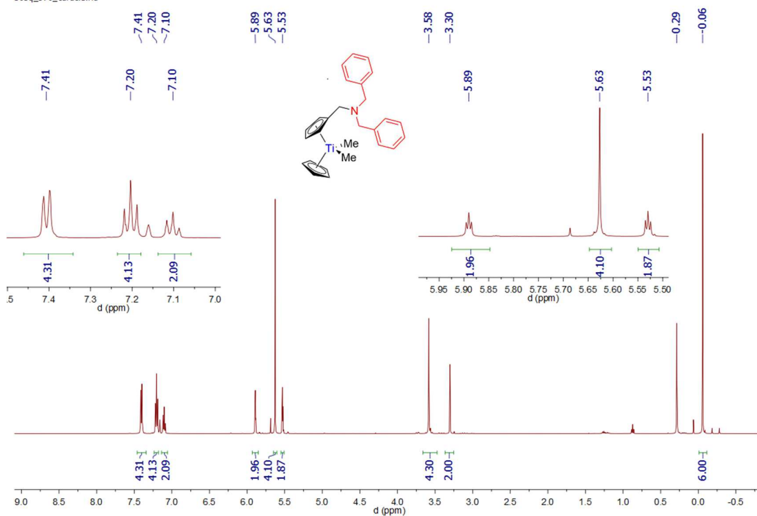
Spectrum 0-228: 1 H NMR of 33 (500.03 MHz, 300 K, benzene-d 6 )
