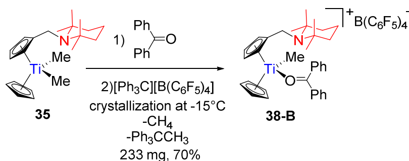
Scheme III-17: synthesis of 38
