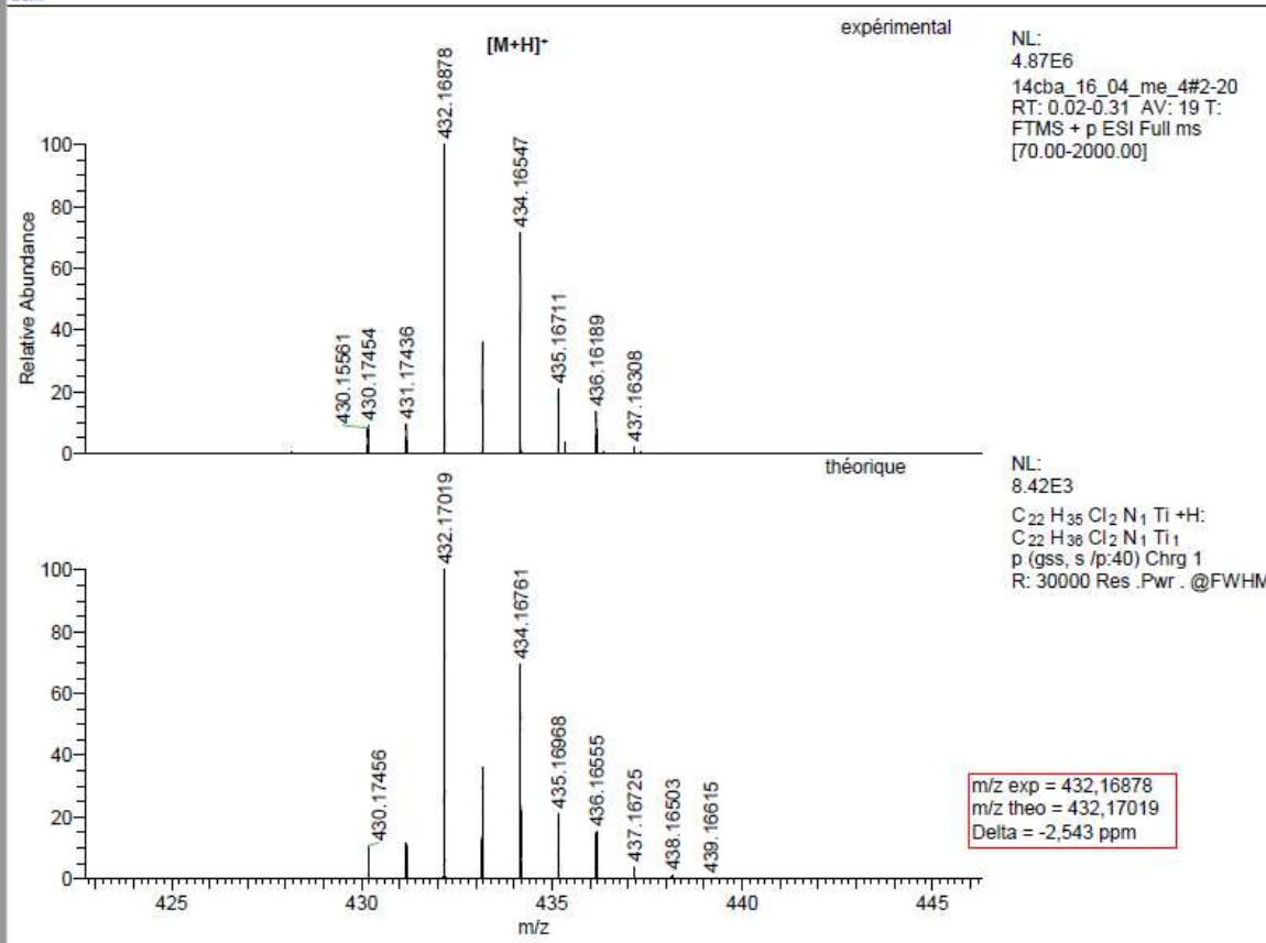
Spectrum 0-122: HRMS of 19 (Positive mode ESI, dichloromethane)
