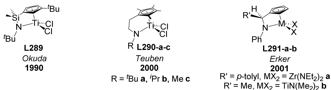
Scheme IV-6: selected examples of CGC complexes
