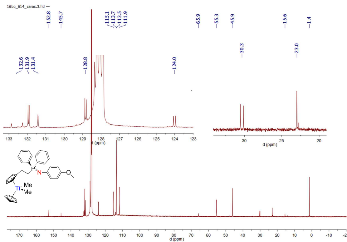
Spectrum 0-524: ^{13}\text{C}\{^1\text{H}\} NMR of 62 (125.75 MHz, 300 K, benzene- d_6 )
