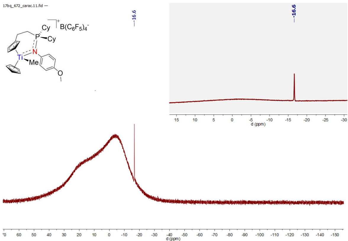
Spectrum 0-565: ^{11}B\{^1H\} and ^{11}B NMR of 65 (160.43 MHz, 300 K, dichloromethane- d_2 )
