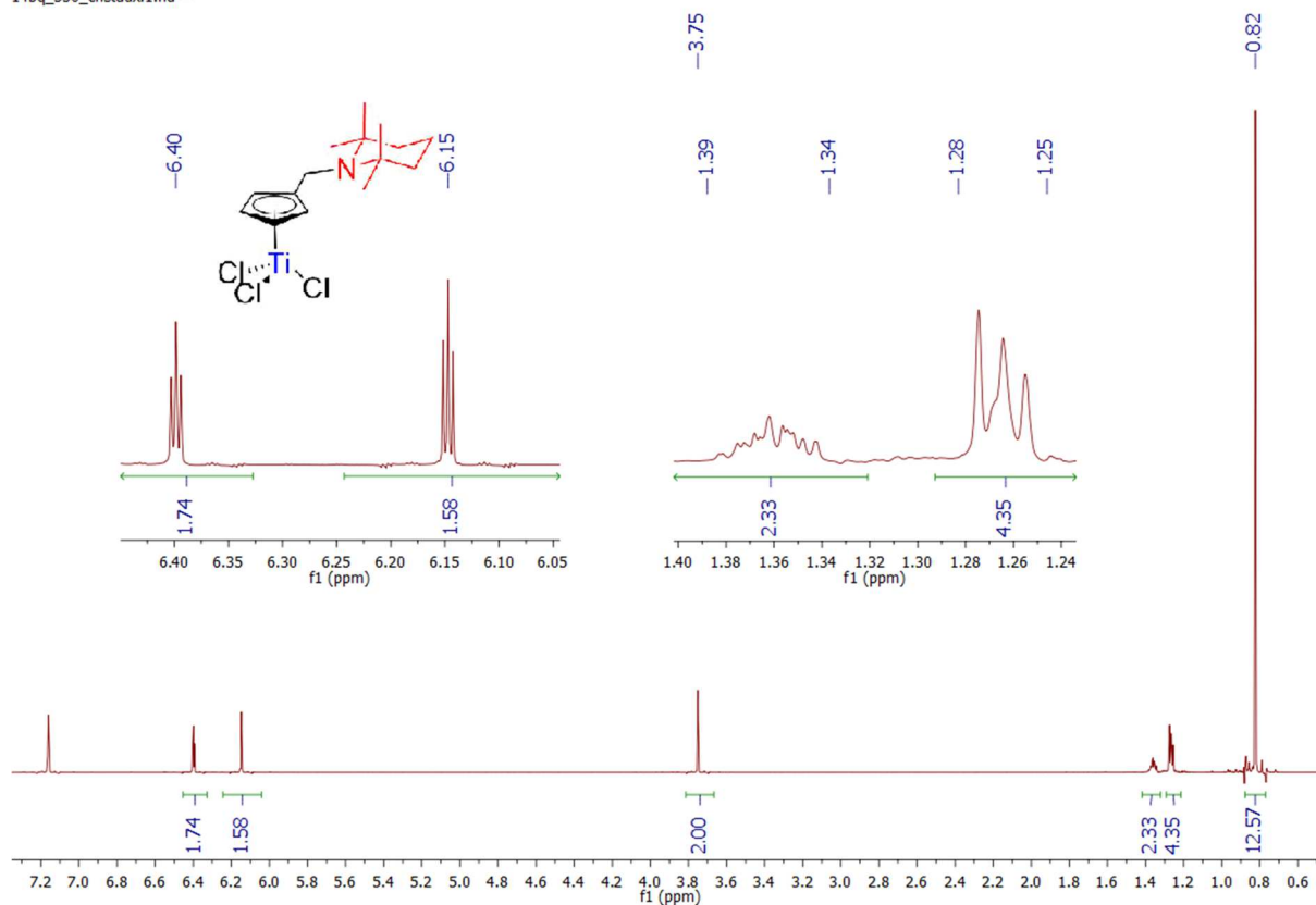
Spectrum 0-131: HRMS of 20 (Positive mode ESI, dichloromethane) 18. Compound 21:
