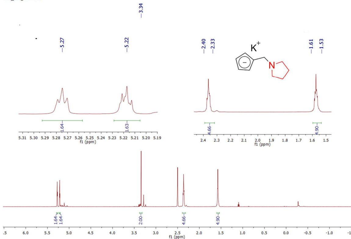
Spectrum 0-7: ^1\text{H} NMR of 2-K (600.23 MHz, 300 K, dimethylsulfoxide- d_6 )
