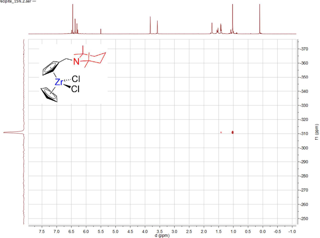
Spectrum 0-162: ^1\text{H} ^{15}\text{N} HMBC of 24 (600.23 MHz / 43.3 MHz, 300 K, tetrahydrofuran- d_6 )
