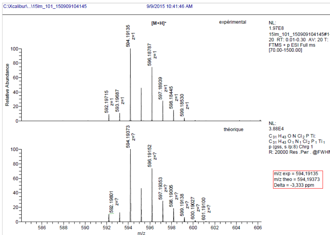
Spectrum 0-494: HRMS of 59 (Positive mode ESI, dichloromethane)
