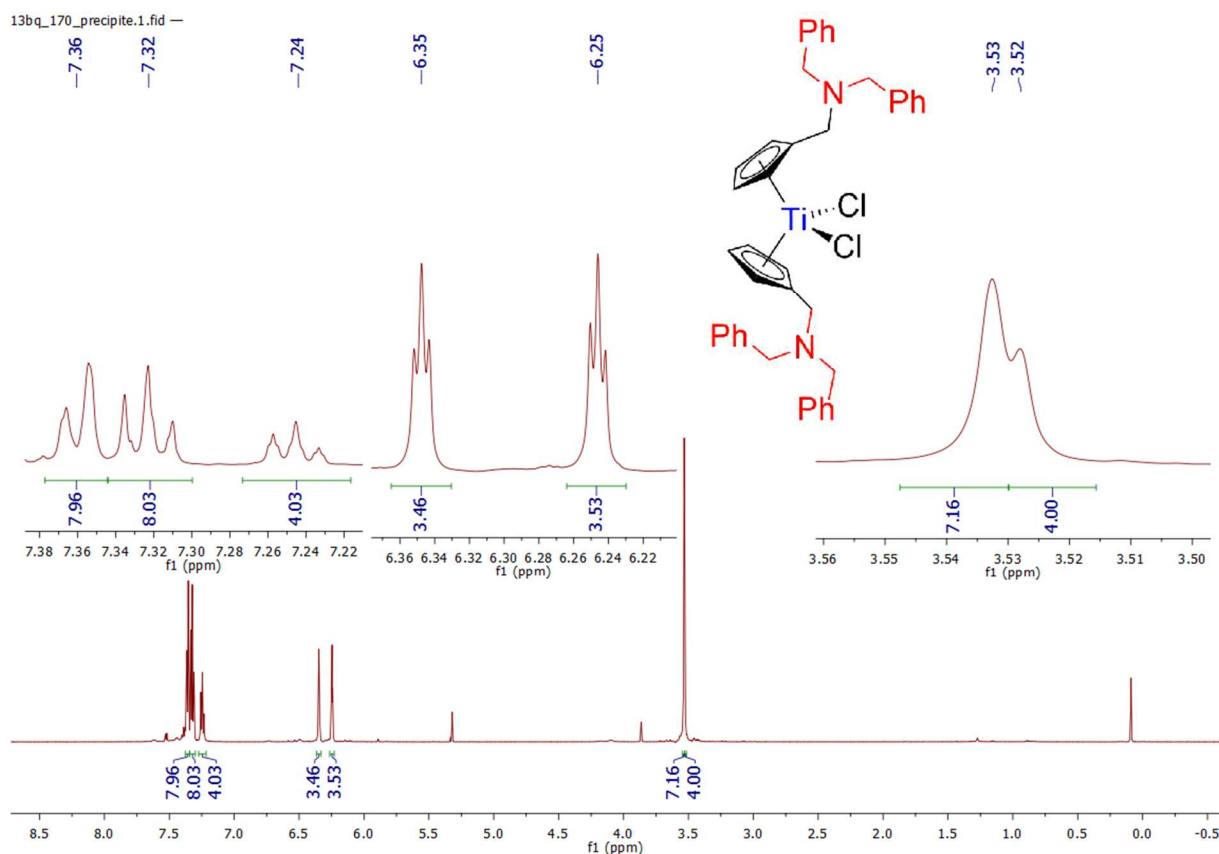
Spectrum 0-125: ^1\text{H} NMR of 20 (600.23 MHz, 300 K, dichloromethane- d_2 )
