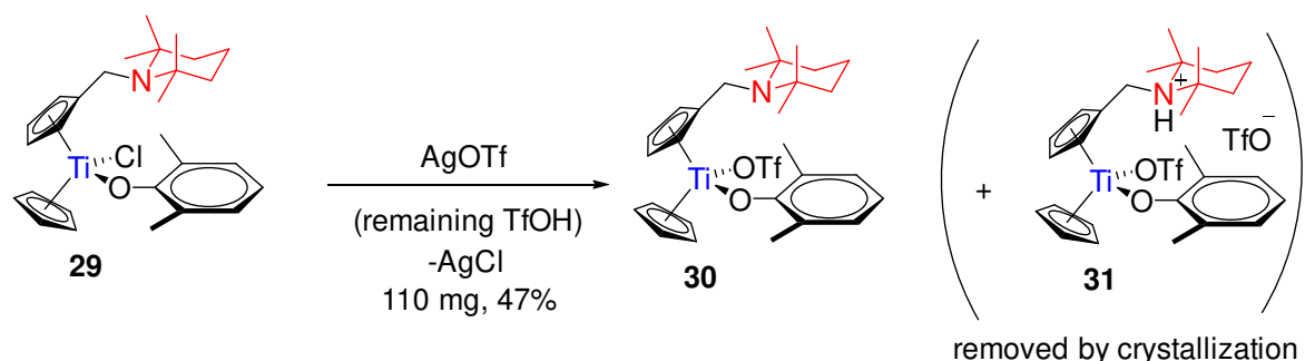
Scheme III-10: synthesis of 30
