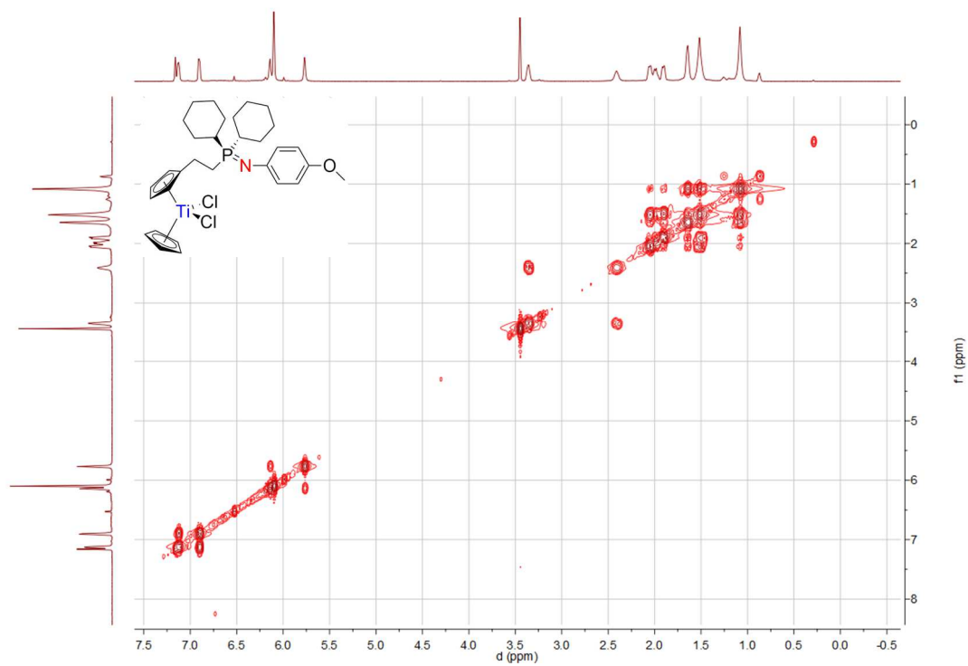
Spectrum 0-490: ^1\text{H} ^1\text{H} COSY of 59 (500.03 MHz, 300 K, 273 K, benzene- d_6 )
