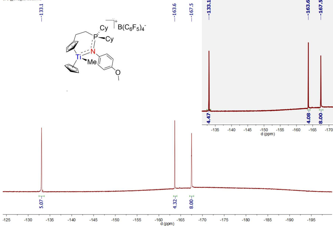
Spectrum 0-566: ^{19}F\{^1H\} and ^{19}F NMR of 65 (470.45 MHz, 300 K, dichloromethane- d_2 )
