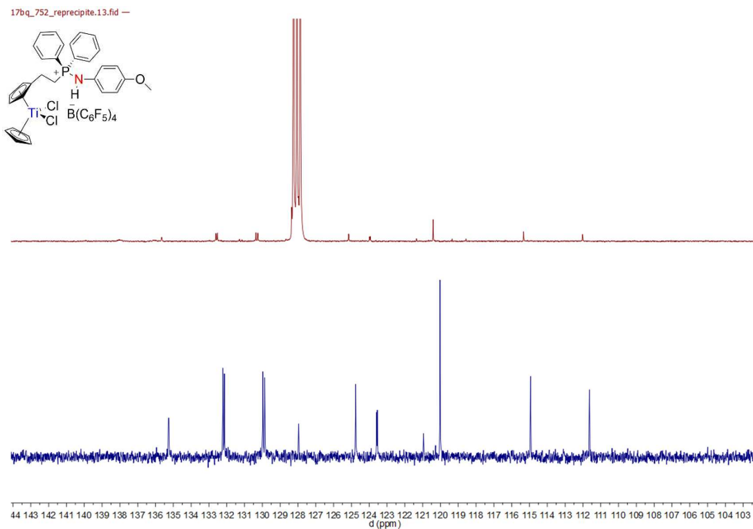
Spectrum 0-513: ^{13}\text{C}\{^1\text{H}\} and dept135 NMR superposition of 61 (125.75 MHz, 300 K, benzene- \text{d}_6 )
