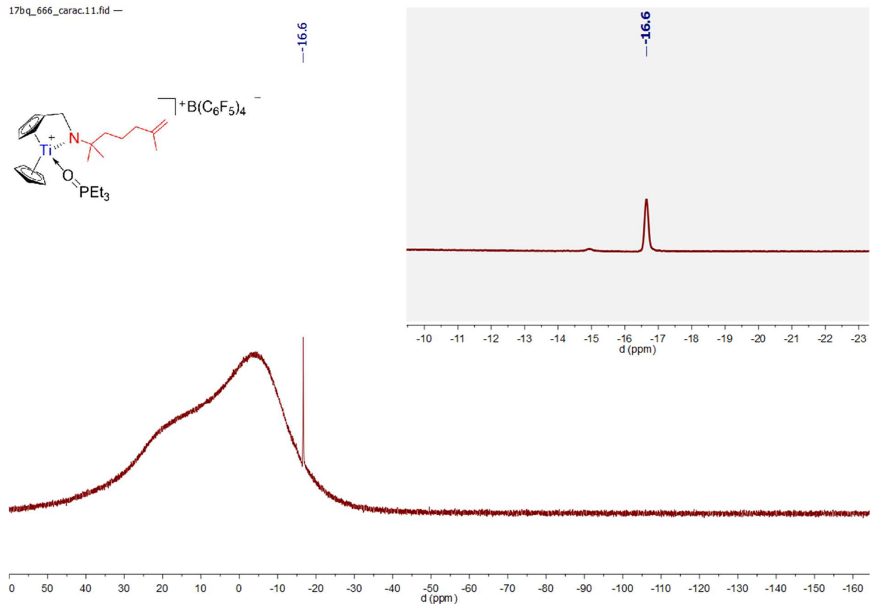
Spectrum 0-269: ^{11}\text{B}\{^1\text{H}\} NMR and ^{11}\text{B} (opacified) of 37 (160.42 MHz, 300 K, dichloromethane- d_2 )
