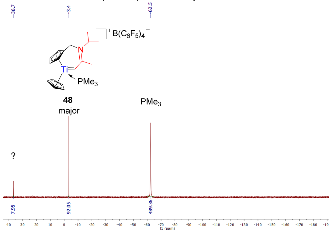
Spectrum III-16: ^{31}\text{P}\{^1\text{H}\} NMR of crude 48 (600.23 MHz, 300 K, bromobenzene- d_5 )
