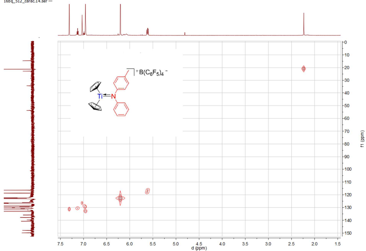
Spectrum 0-420: 1 H 13 C HMQC of 54 (500.03 MHz / 125.75 MHz, 300 K, bromobenzene-d 5 )
