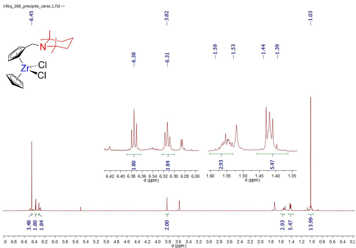
Spectrum 0-157: ^1\text{H NMR} of 24 (600.23 MHz, 300 K, tetrahydrofuran- d_6 )
