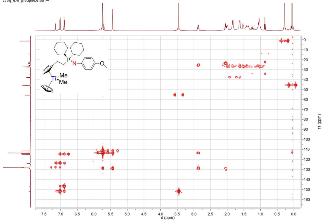
Spectrum 0-538: 1 H 13 C HMBC of 63 (600.23 MHz / 150.86 MHz, 300 K, benzene-d 6 )
