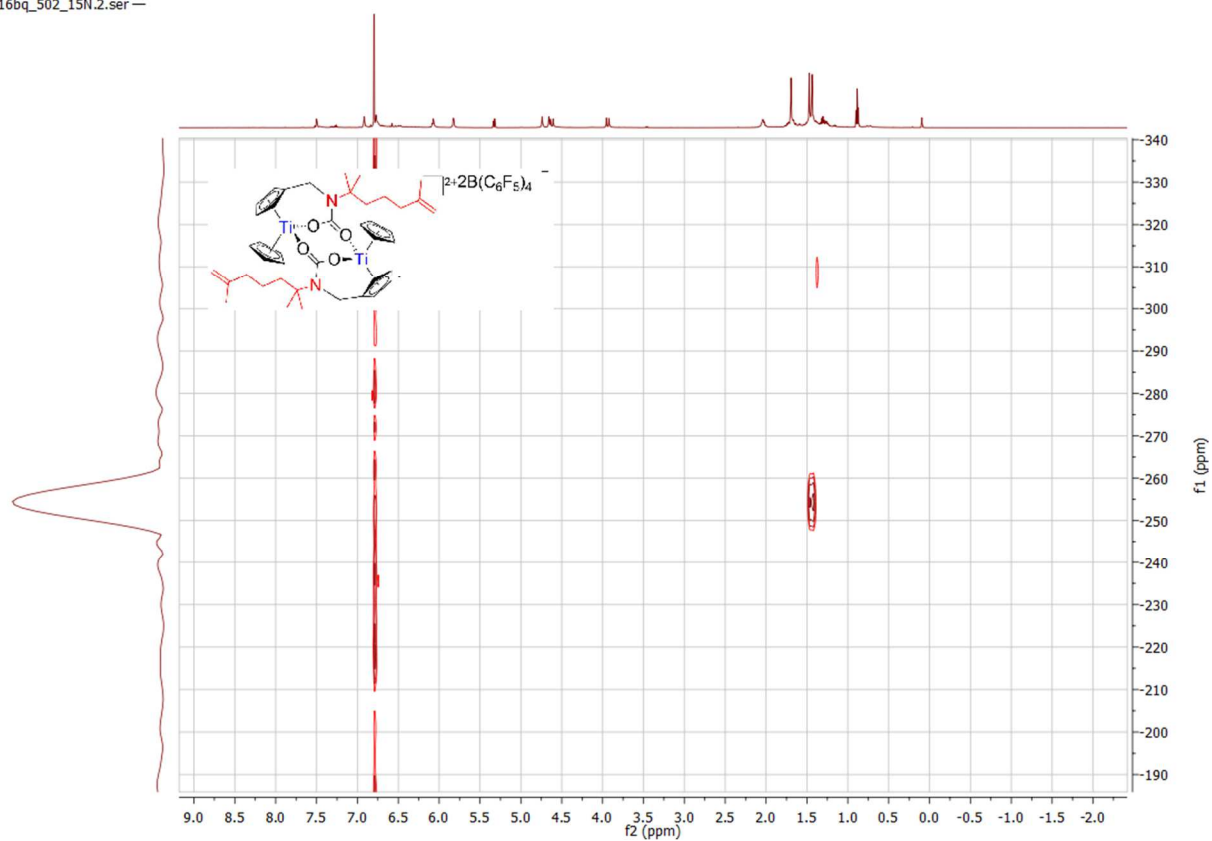
Spectrum 0-287: ^1H ^{15}N HMBC of 39 (600.23 MHz / 43.3 MHz, 300 K, dichloromethane- d_2 )
