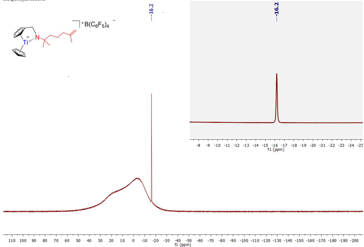
Spectrum 0-259: ^{11}\text{B}\{^1\text{H}\} and ^{11}\text{B} (opacified) NMR of 36 (160.42 MHz, 300 K, bromobenzene- d_5 )
