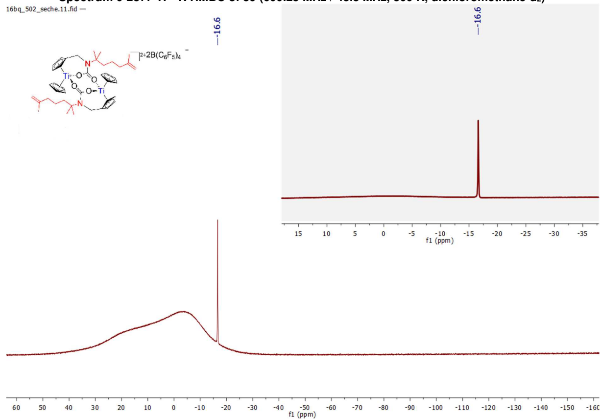
Spectrum 0-288: ^{11}B\{^1H\} and ^{11}B (opacified) NMR of 39 (160.42 MHz, 300 K, dichloromethane- d_2 )
