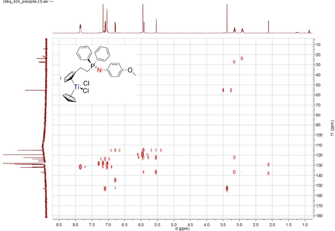
Spectrum 0-472: ^1\text{H} ^{13}\text{C} HMBC of 57 (600.23 MHz / 150.86 MHz, 300 K, benzene- d_6 )
