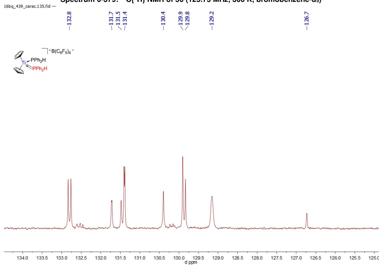
Spectrum 0-380: dept135 NMR of 50 (125.75 MHz, 300 K, bromobenzene- d_5 )
