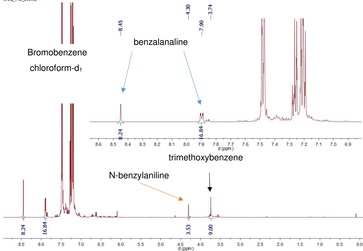
Spectrum 0-466: Hydrogenation of benzalnaline with 53 (500.03 MHz, 300K, Chloroform-d 1 )
