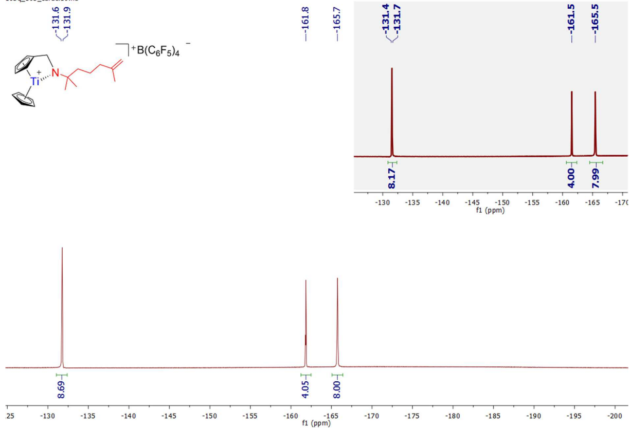
Spectrum 0-260: ^{19}\text{F}\{^1\text{H}\} and ^{19}\text{F} (opacified) NMR of 36 (470.45 MHz, 300 K, bromobenzene- d_5 )
