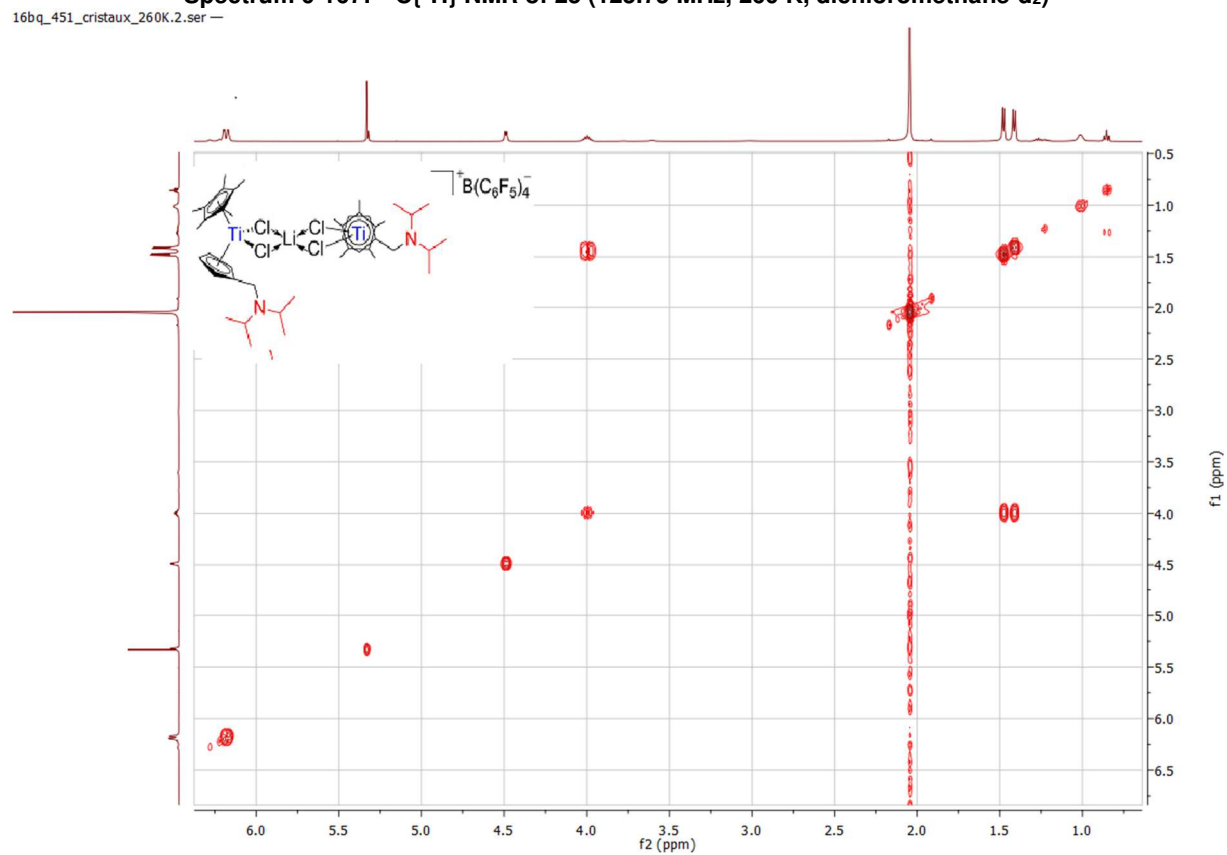
Spectrum 0-168: ^1\text{H} ^1\text{H} COSY of 25 (500.03 MHz, 260 K, dichloromethane- d_2 )
