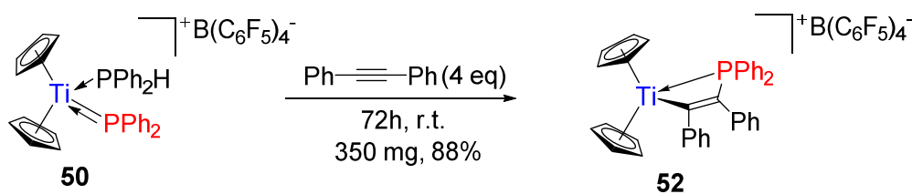
Scheme IV-9: synthesis of 52
