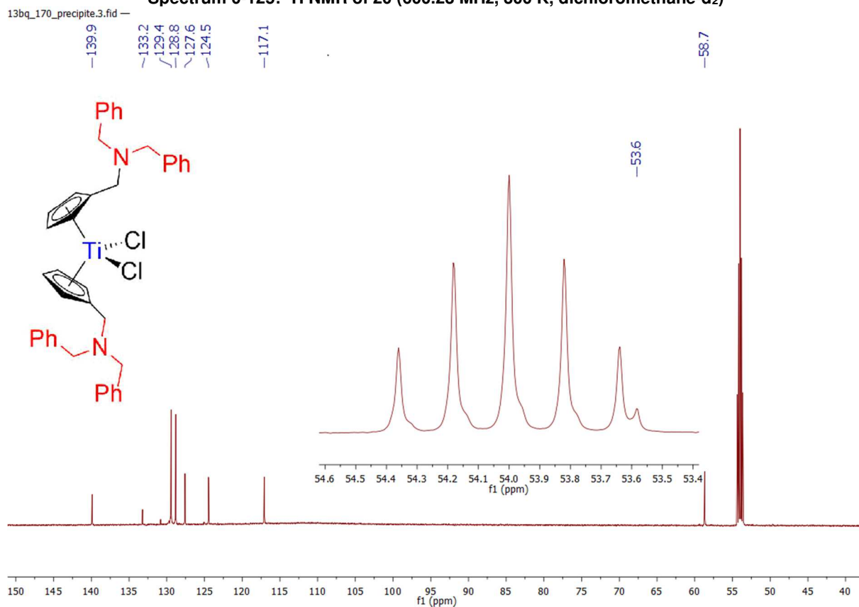
Spectrum 0-126: ^{13}\text{C}\{^1\text{H}\} NMR of 20 (150.94 MHz, 300 K, dichloromethane- d_2 )
