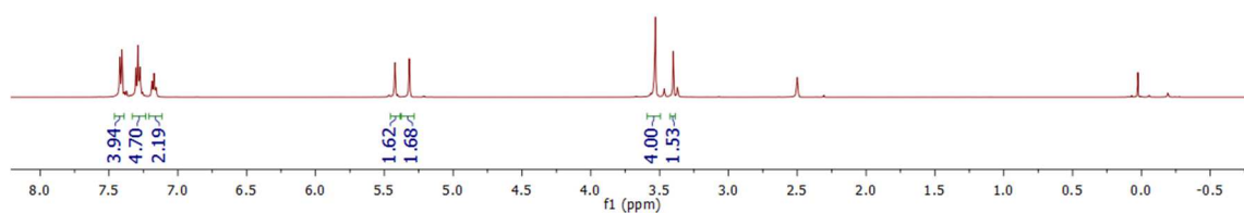
Spectrum 0-13: 1 H NMR of 3-K (500.03 MHz, 300 K, dimethylsulfoxide-d 6 )
