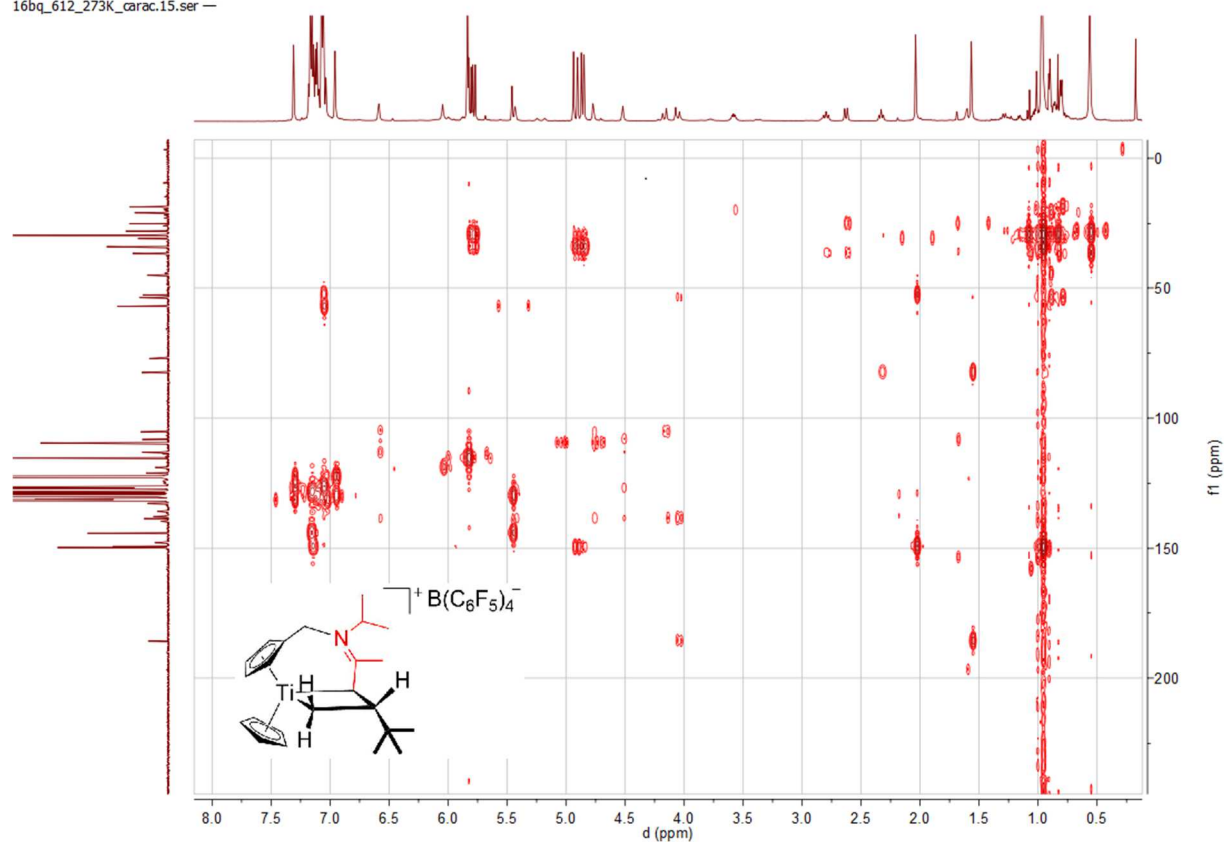
Spectrum 0-368: ^1\text{H} ^{13}\text{C} HMBC of 47 (500.03 MHz / 125.75 MHz, 273 K, bromobenzene- d_5 )
