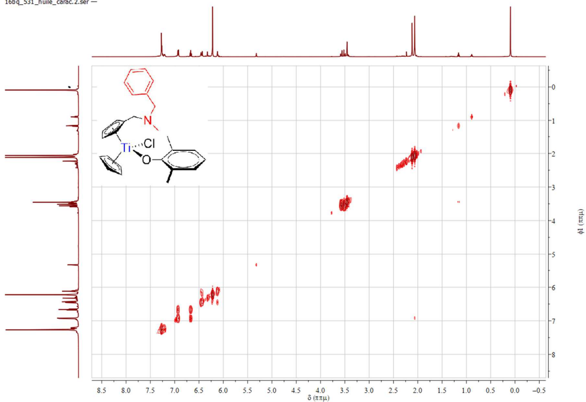
Spectrum 0-177: ^1\text{H} ^1\text{H} COSY of 26 (500.03 MHz, 300 K, dichloromethane- d_2 )
