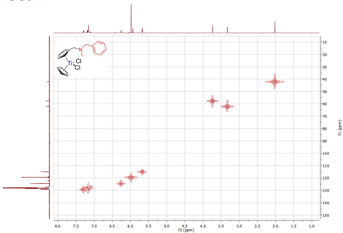
Spectrum 0-34: ^1\text{H} ^{13}\text{C} HMQC of 9 (600.23 MHz / 150.94 MHz, 300 K, benzene- d_6 )
