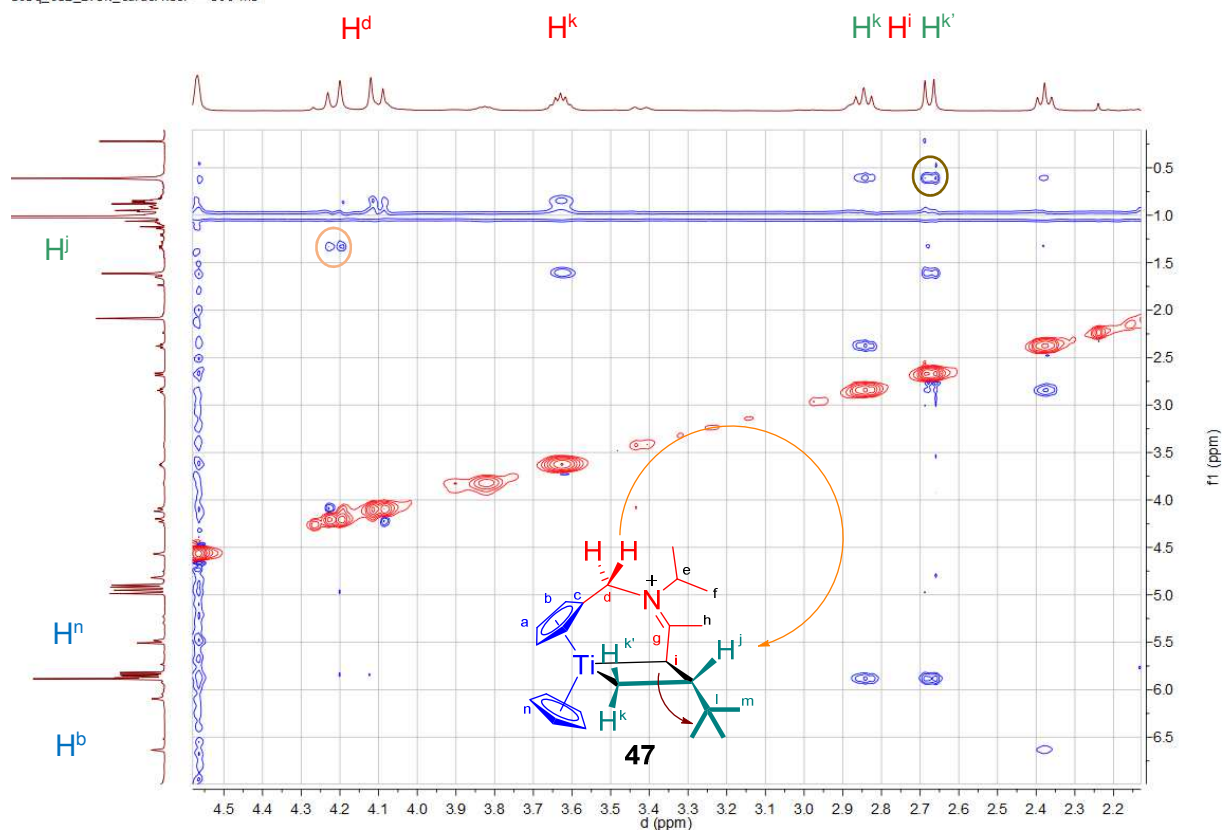
Spectrum III-15: ^1\text{H} ^1\text{H} NOESY of 47 (600.23 MHz, 273 K, bromobenzene- d_5 )
