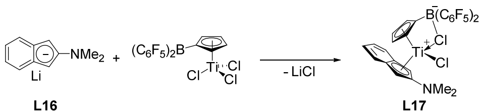
Scheme I-6: intriguing boryl-(aminoindenyl)titanocene from Bochmann's work
