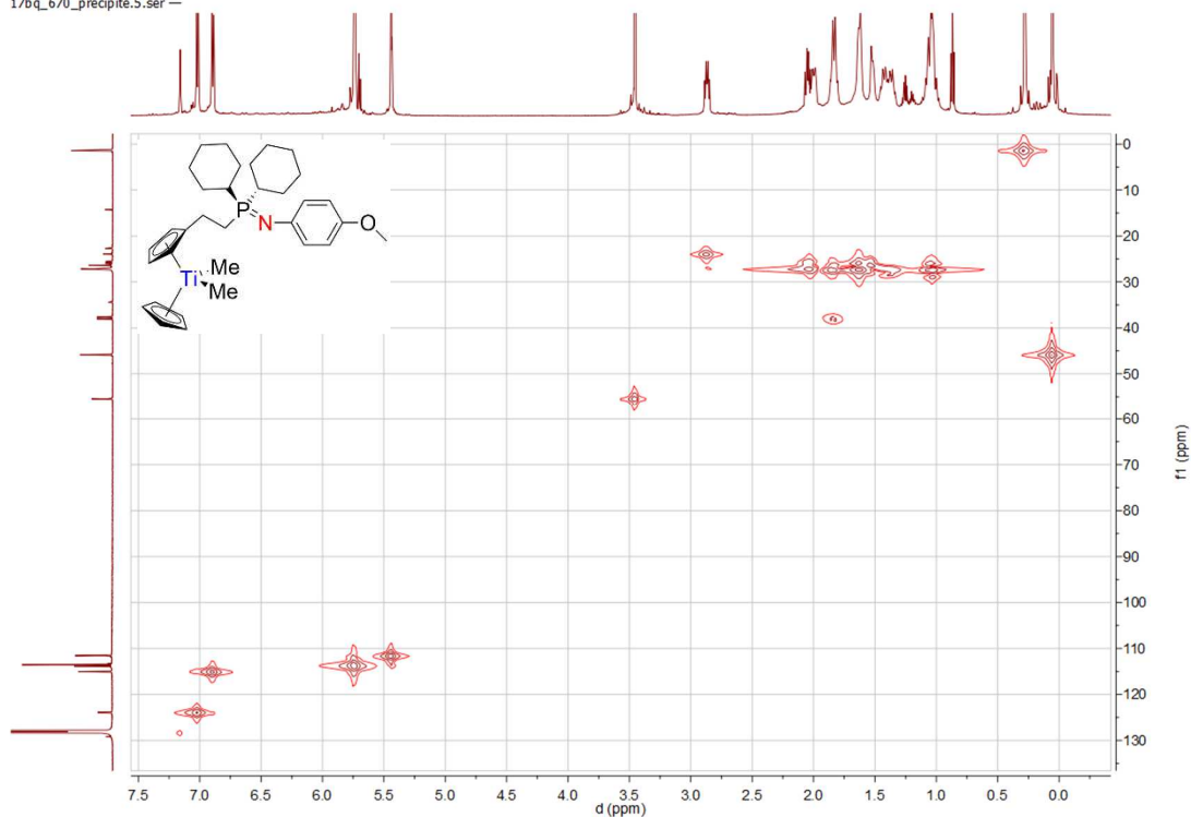
Spectrum 0-537: 1 H 13 C HMQC of 63 (500.03 MHz / 125.75 MHz, 300 K, benzene-d 6 )
