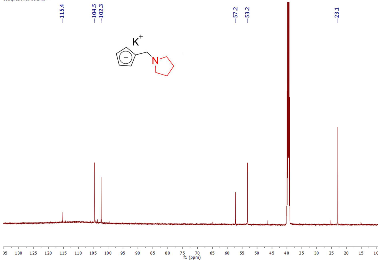
Spectrum 0-8: ^{13}\text{C}\{^1\text{H}\} NMR of 2-K (150.94 MHz, 300 K, dimethylsulfoxide- d_6 )
