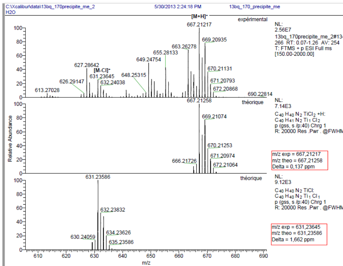
Spectrum 0-131: HRMS of 20 (Positive mode ESI, dichloromethane) 18. Compound 21:
