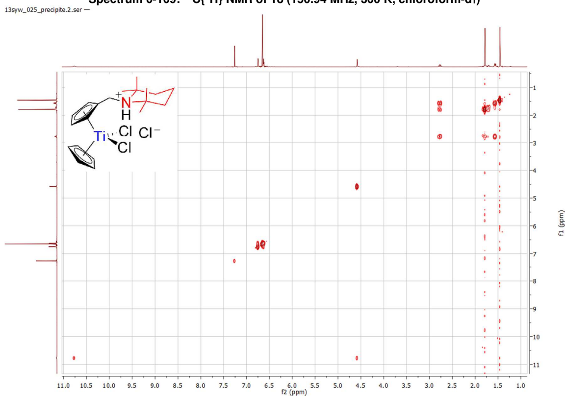
Spectrum 0-110: 1 H 1 H COSY of 18 (600.23 MHz, 300 K, chloroform-d 1 )
