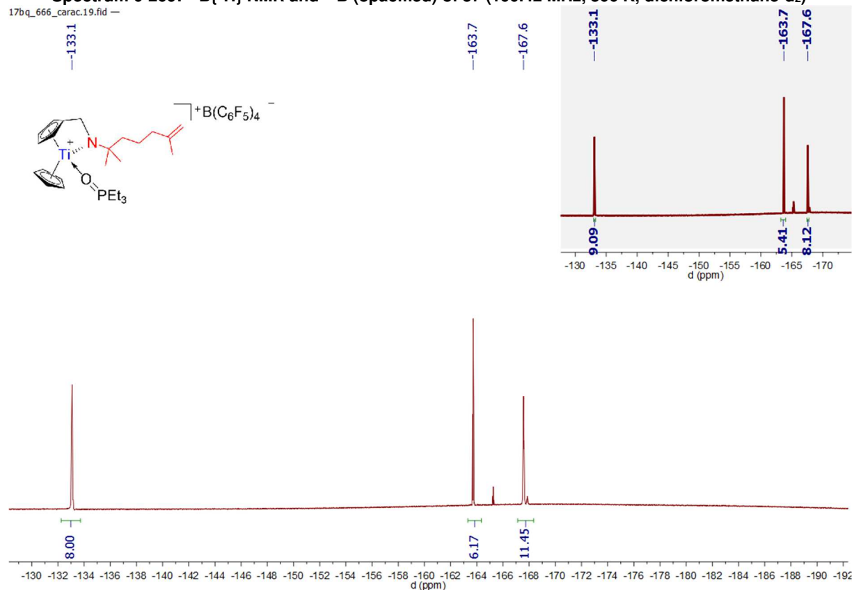
Spectrum 0-270: ^{19}\text{F}\{^1\text{H}\} NMR and ^{19}\text{F} (opacified) of 37 (470.45 MHz, 300 K, dichloromethane- d_2 )
