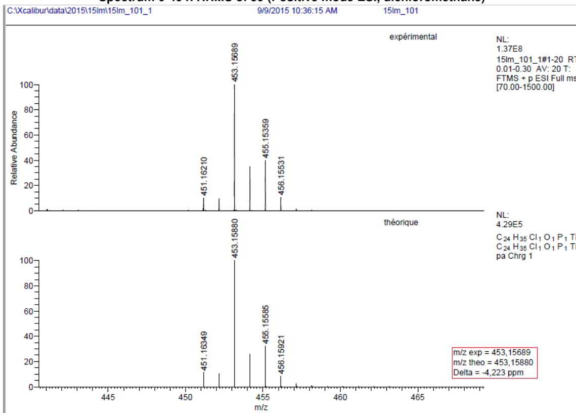
Spectrum 0-495: HRMS of 59 (Positive mode ESI, dichloromethane)
