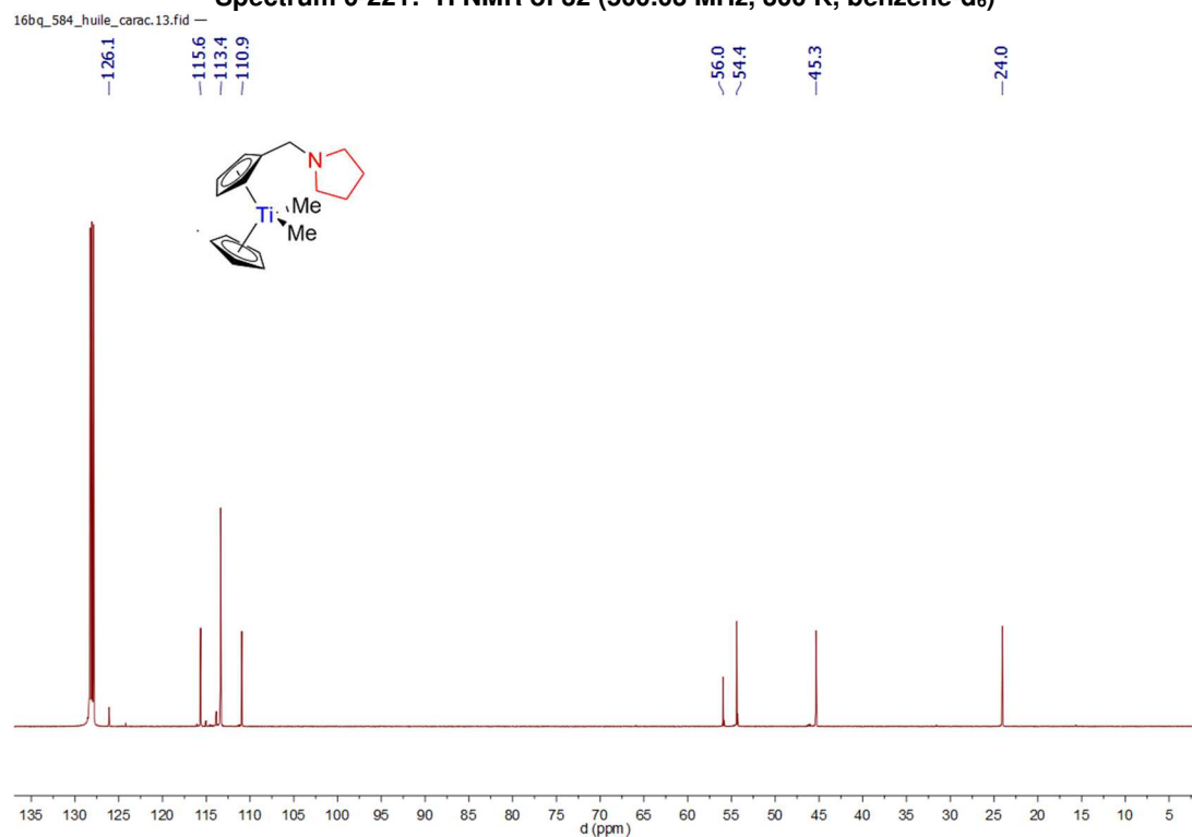
Spectrum 0-222: ^{13}\text{C}\{^1\text{H}\} NMR of 32 (125.75 MHz, 300 K, benzene- \text{d}_6 )
