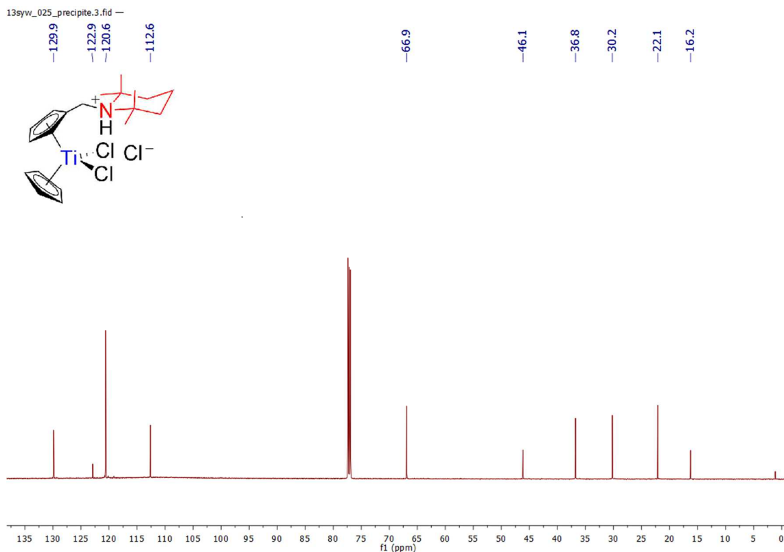
Spectrum 0-109: 13 C{ 1 H} NMR of 18 (150.94 MHz, 300 K, chloroform-d 1 )
