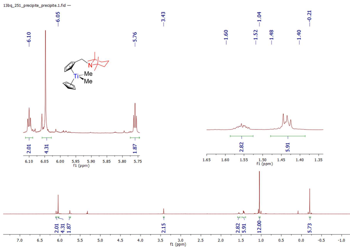
Spectrum 0-244: ^1\text{H} NMR of 35 (600.23 MHz, 300 K, dichloromethane- d_2 )
