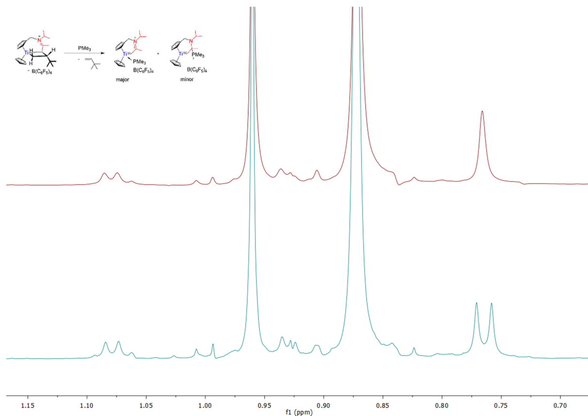
Spectrum 0-375: 1 H{ 31 P} NMR of 48 (600.23 MHz, 300 K, bromobenzene-d 5 )
