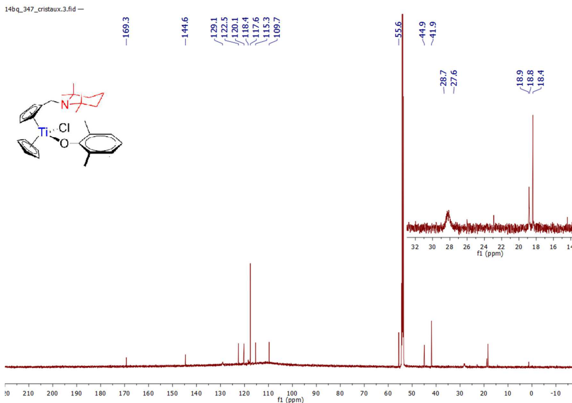
Spectrum 0-201: ^{13}\text{C}\{^1\text{H}\} NMR of 29 (150.94 MHz, 300 K, dichloromethane- d_2 )
