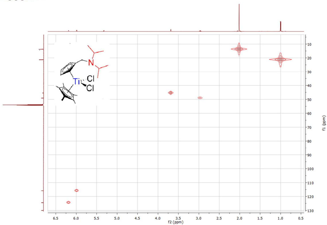
Spectrum 0-119: ^1\text{H} ^{13}\text{C} HMQC of 19 (600.23 MHz / 150.94 MHz, 300 K, dichloromethane- d_2 )
