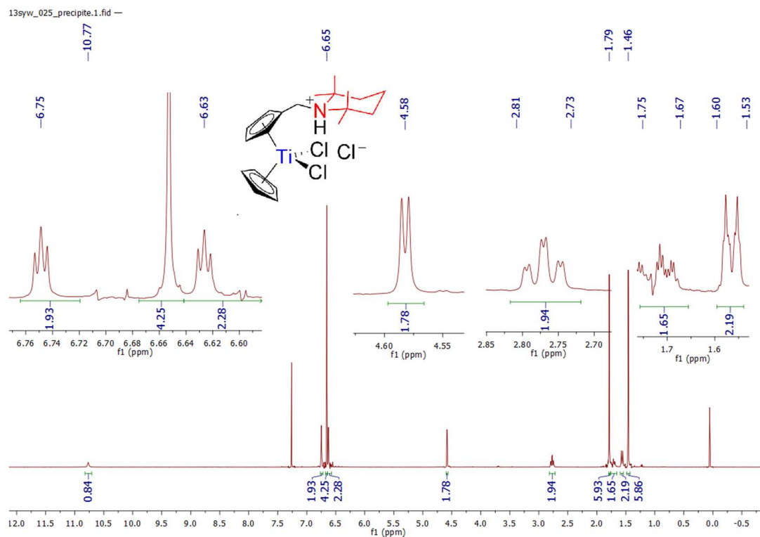
Spectrum 0-107: FIR of 17
