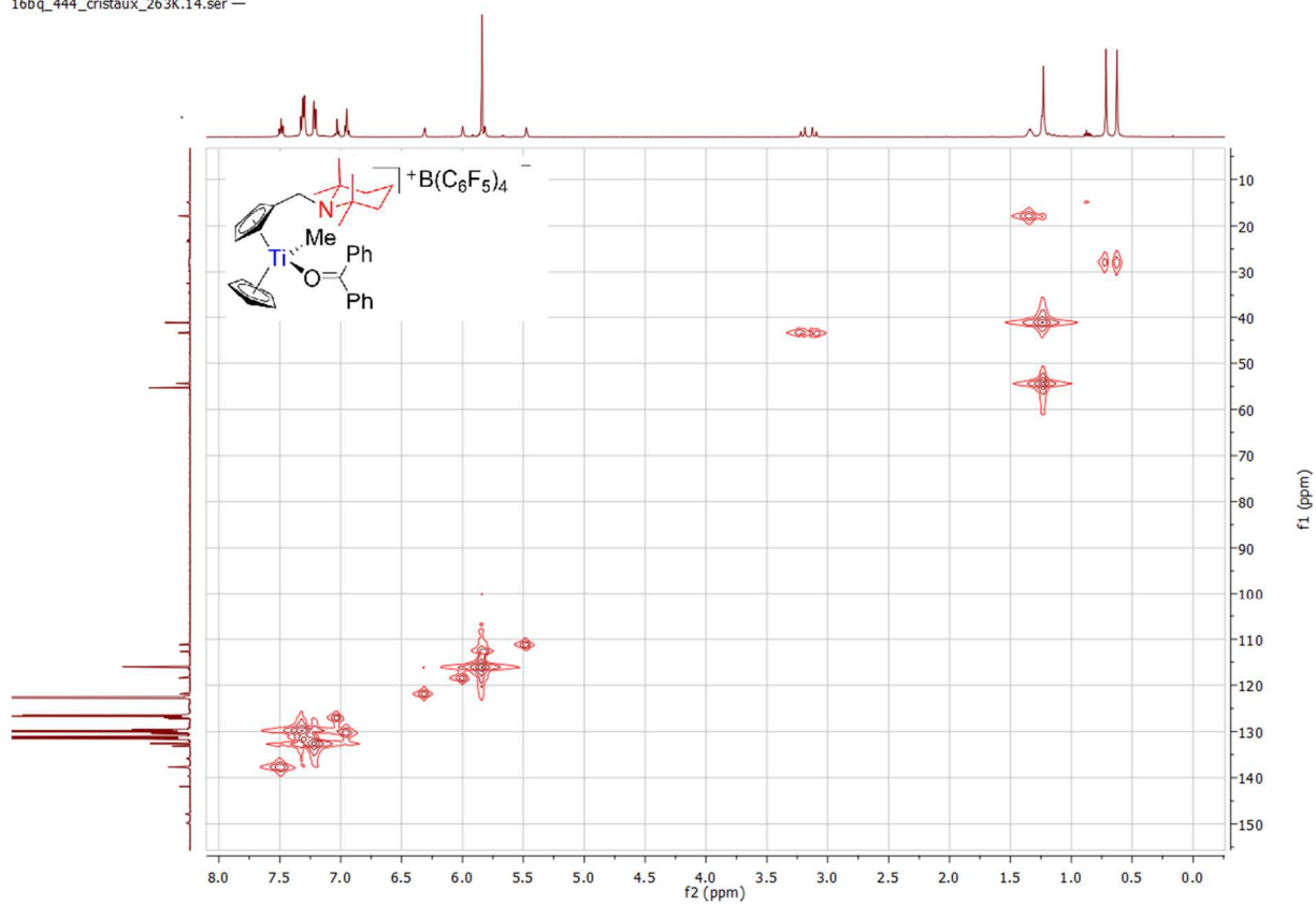
Spectrum 0-276: ^1\text{H} ^{13}\text{C} HMQC 38 (500.03 MHz / 125.03 MHz, 263 K, bromobenzene- d_5 )
