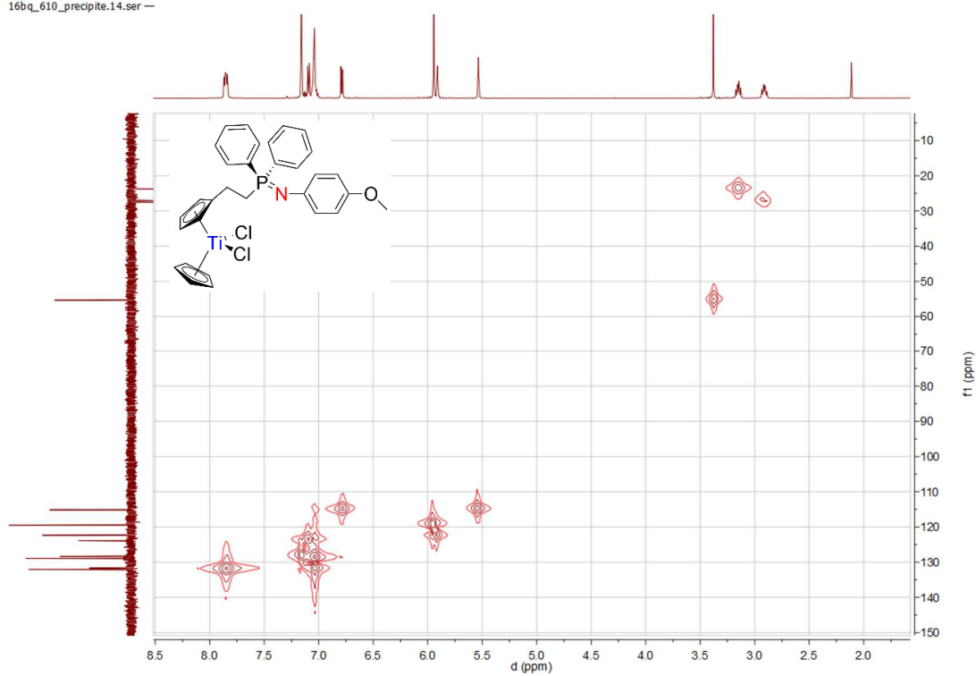
Spectrum 0-471: ^1\text{H} ^{13}\text{C} HMQC of 57 (500.03 MHz / 125.75 MHz, 300 K, benzene- d_6 )
