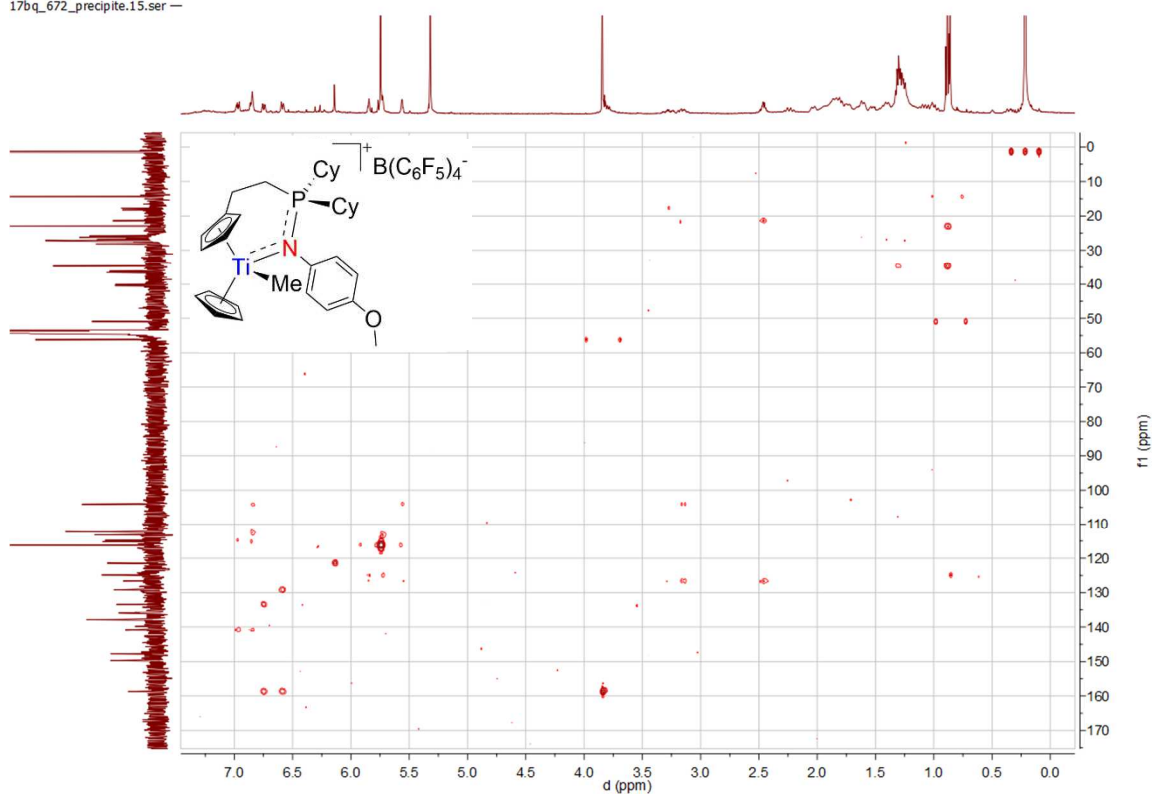
Spectrum 0-564: ^1\text{H} ^{13}\text{C} HMBC of 65 (500.03 MHz / 125.75 MHz, 300 K, dichloromethane- d_2 )
