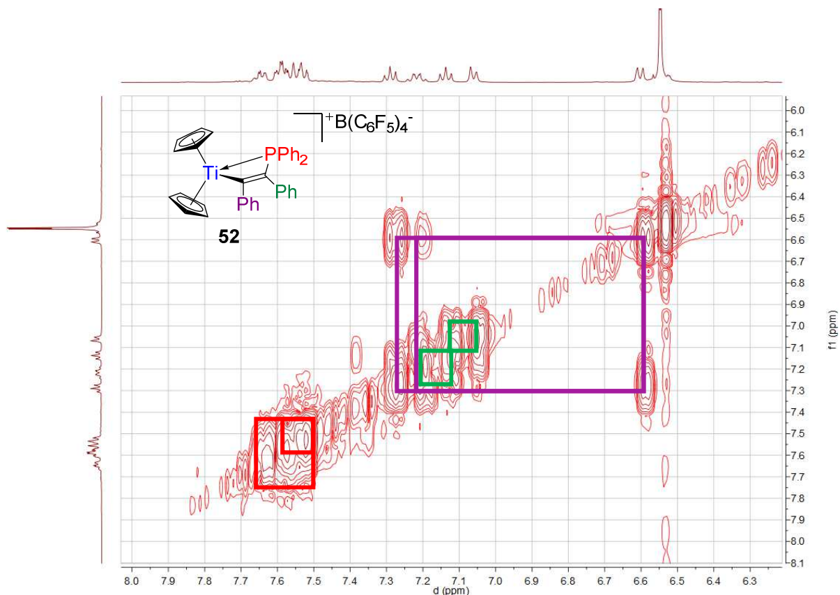
Spectrum IV-4: ^1\text{H} ^1\text{H} COSY NMR spectrum of 52 (500.03 MHz, 300 K, dichloromethane- d_2 )
