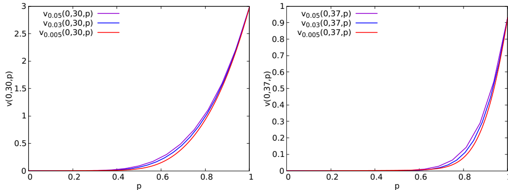
Figure 4.1 – The functions v_{\pi, \delta}(t, x, \cdot) , t = 0 and x \in \{30, 37\} . We drop the subscript \pi in the legend above as h = \delta .
