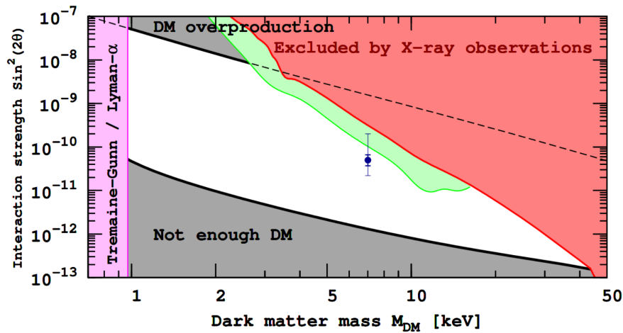
Figure 1.9: The bounds on neutrino dark matter from X-ray observations. A lower mass limit is set by the Tremaine-Gunn bound, the interaction strength has an (model dependent) upper limit to prevent overproduction in the big bang. The bounds set by non-observed lines are shown in different colors for different studies. The data point marks the observed 3.5 keV line. The plot was taken from [BRIF14].
