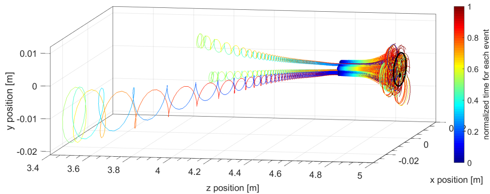
Figure 11.42: The tracks of 100 simulated wall electrons. The electrons are started at z = 4.65 m and then gyrate around the field lines towards the detector. Three electrons are back-scattered, move then towards the spectrometer center, where they are reflected and return to the detector. The color code shows the normalized time of each simulation step, where the last step for each event is at time = 1. The detector chip is shown as black cylinder. The smaller black cylinder within is one pixel of the detector, as defined in the analysis.
