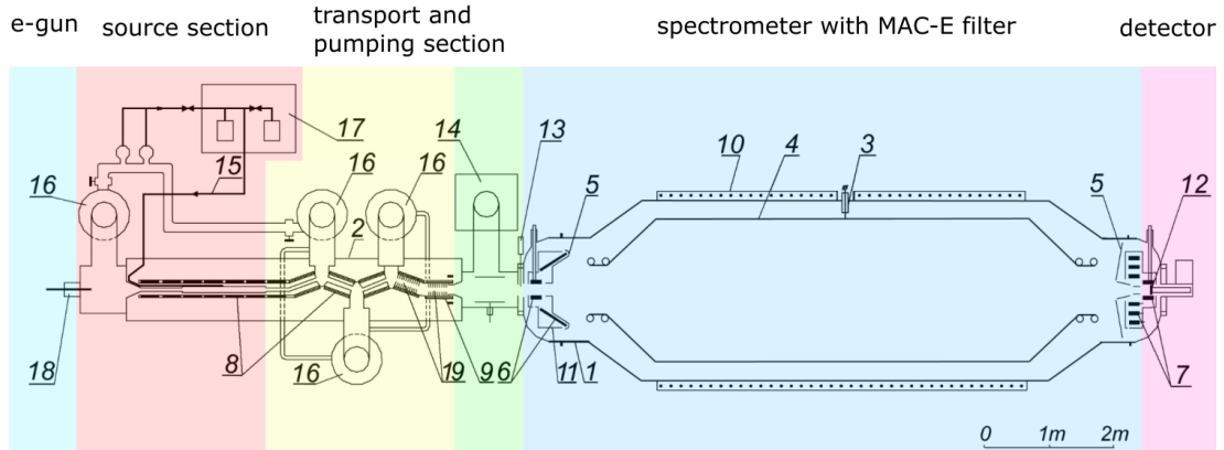
Figure 8.5: A detailed sketch of the Troitsk \nu -mass setup: 1) spectrometer vacuum tank; 2) source vacuum tank; 3) high voltage feed-through; 4) spectrometer electrode; 5) ground electrodes; 6), 7), 8), 9) superconducting magnets; 10) warm coil; 11) liquid nitrogen jacket; 12) silicon detector with cooling system; 13) gate valve; 14) titanium sublimation pump; 15) tritium loop; 16) mercury diffusion pumps; 17) tritium storage and purification system; 18) electron gun; 19) cryo argon pump. Sketch adapted from [A + 15a].
