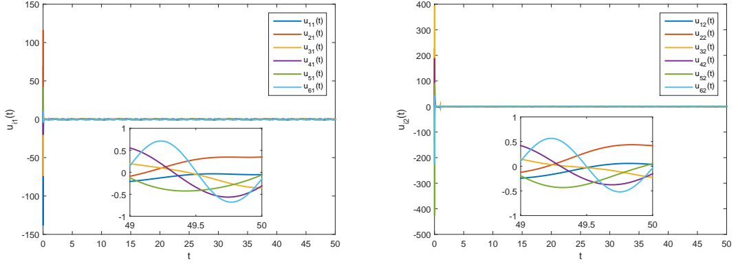
(a) Control inputs of u_{i1}(i = 1, \dots, 6)
