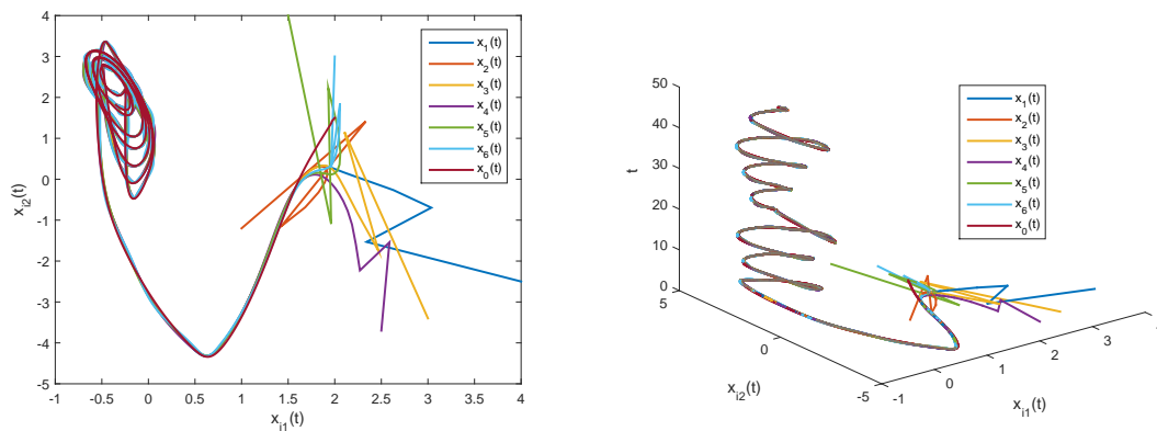
(a) Phase portraits in 2D (b) Phase portraits in 3D
