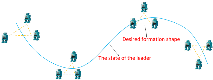
Fig. 1.8. Formation tracking problem
