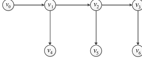
Fig. 5.1. The communication topology with one leader and six followers
