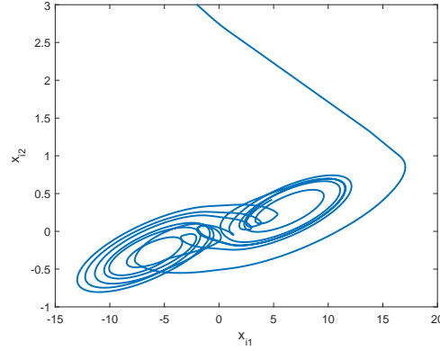
Fig. 5.2. Chaotic behavior of agent i with initial value [-2, 3]^T
