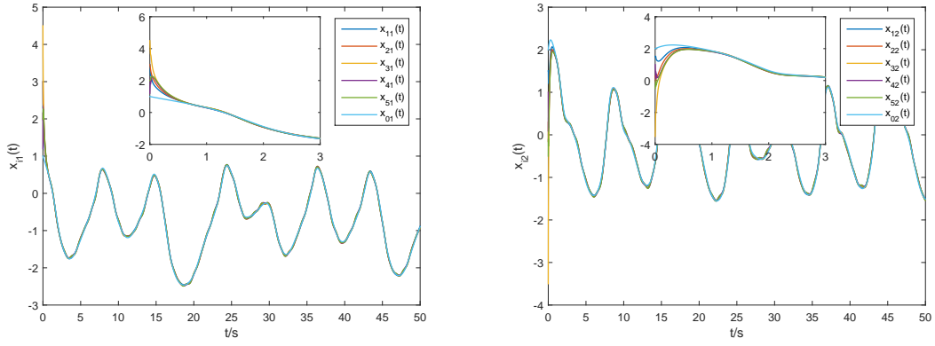
(a) State trajectories of x_{i1}(i = 0, 1, \dots, 5) (b) State trajectories of x_{i2}(i = 0, 1, \dots, 5)
