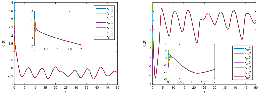
(a) State trajectories of x_{i1}(i = 0, 1, \dots, 6)
