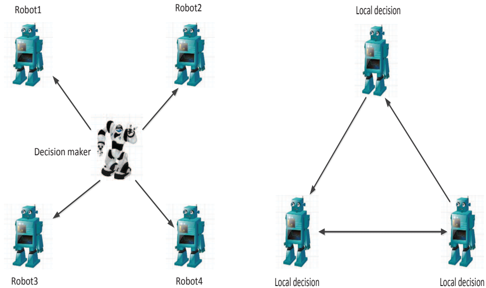
(a) The centralized control
