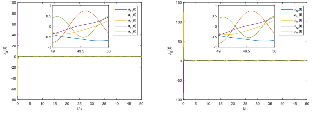
(a) Control inputs of u_{i1}(i = 1, \dots, 5)
