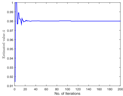
(a) Identified parameter value \tilde{\alpha}
