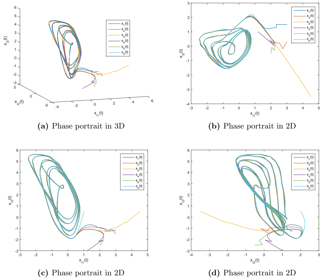
Fig. 3.6. Phase portraits for all agents ( i = 0, 1, \dots, 5 ) by control algorithm (3.16) with d_i = 0.2
