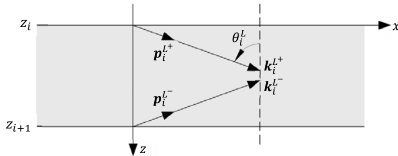
Figure 2-3: Wave propagation in a fluid layer i .
