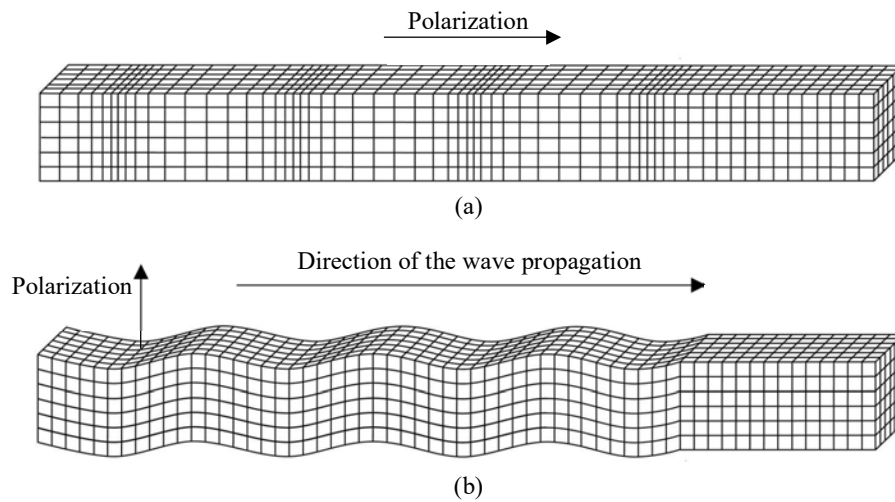
Figure 1-2: (a) Longitudinal and (b) Shear waves propagation in an isotropic elastic solid.
