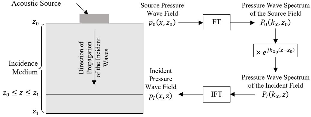
Figure 4-1: Diagram of the steps followed for obtaining the incident pressure wave field in the incidence medium ( z_0 \leq z \leq z_1 ).
