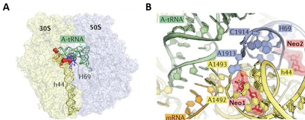
Figure 7: Interactions of aminoglycoside molecule neomycin with the decoding center of the ribosome.
