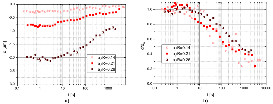
Figure I-13a) Influence of the scratching Tabor deformation on the recovery depth at a 4 a_c distance from end of scratch versus time elapsed since tip removal on CR39 at 30^\circ\text{C} b) same experience normed by the first measured recovery depth
