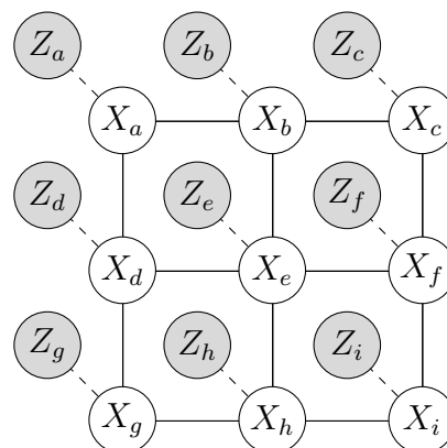
Hidden MRF
