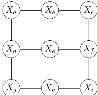
Figure 1.1: Conditional independence graphs corresponding to different Markov models.
