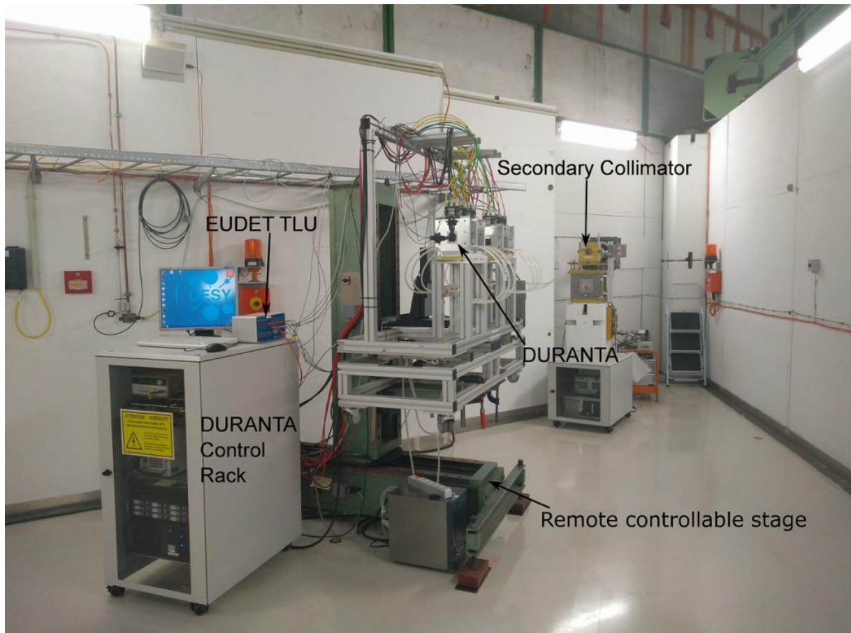
Figure 6.2 – A photo of the test beam area T22 at DESY [115].
