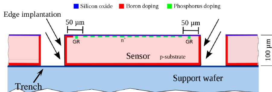
Figure 5.6 – Schematic view of the sensor processing at ADVACAM with a four-quadrant Boron ion implantation, extending the p^+ implant of the back-side to the edges [110].
