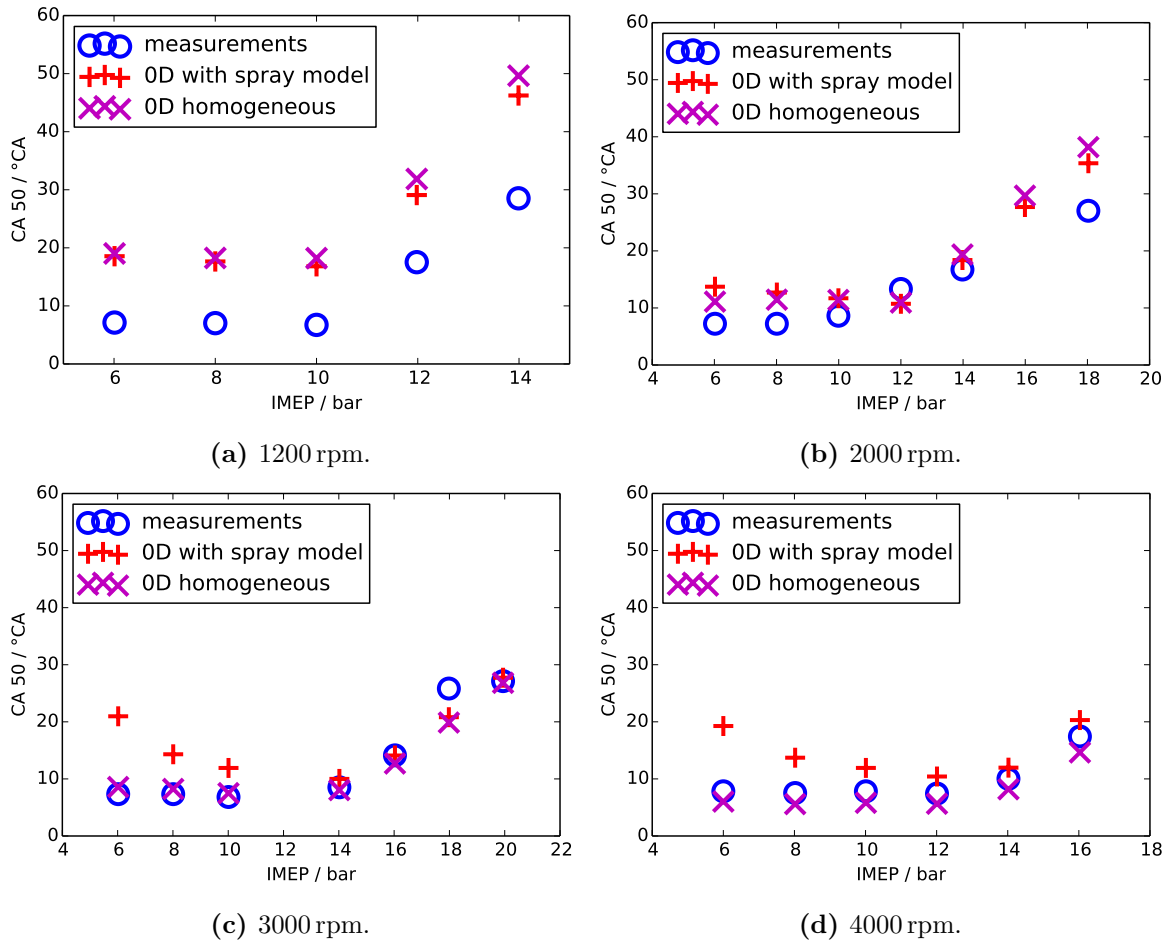
Figure 6.20: ICAMDAC engine: heat release. The values of CA 50 are plotted against the nominal IMEP for four different crank speeds. Red “+” for the developed 0D model (with detailed spray description), magenta “X” for the base 0D model (no spray description) and blue “O” for test bed measurements. The operating points shown cover the whole engine map realized in the framework of the ICAMDAC project (de Francqueville, 2013).
