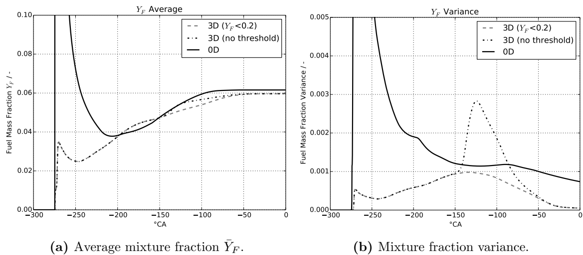
Figure 6.16: ICAMDAC engine: operating point at N = 4000 rpm and \text{IMEP} = 18 bar. The two plots show the average mixture fraction \bar{Y}_F (a) and its variance (b) against the crank angle. Solid line for 0D, black dash dotted line for 3D, grey dashed line for 3D with threshold Y_F < 0.2 . Cutting off cells with higher fuel concentrations attenuates the variance peak at at 125^\circ\text{CA} before TDC with little effect on the mean value.
