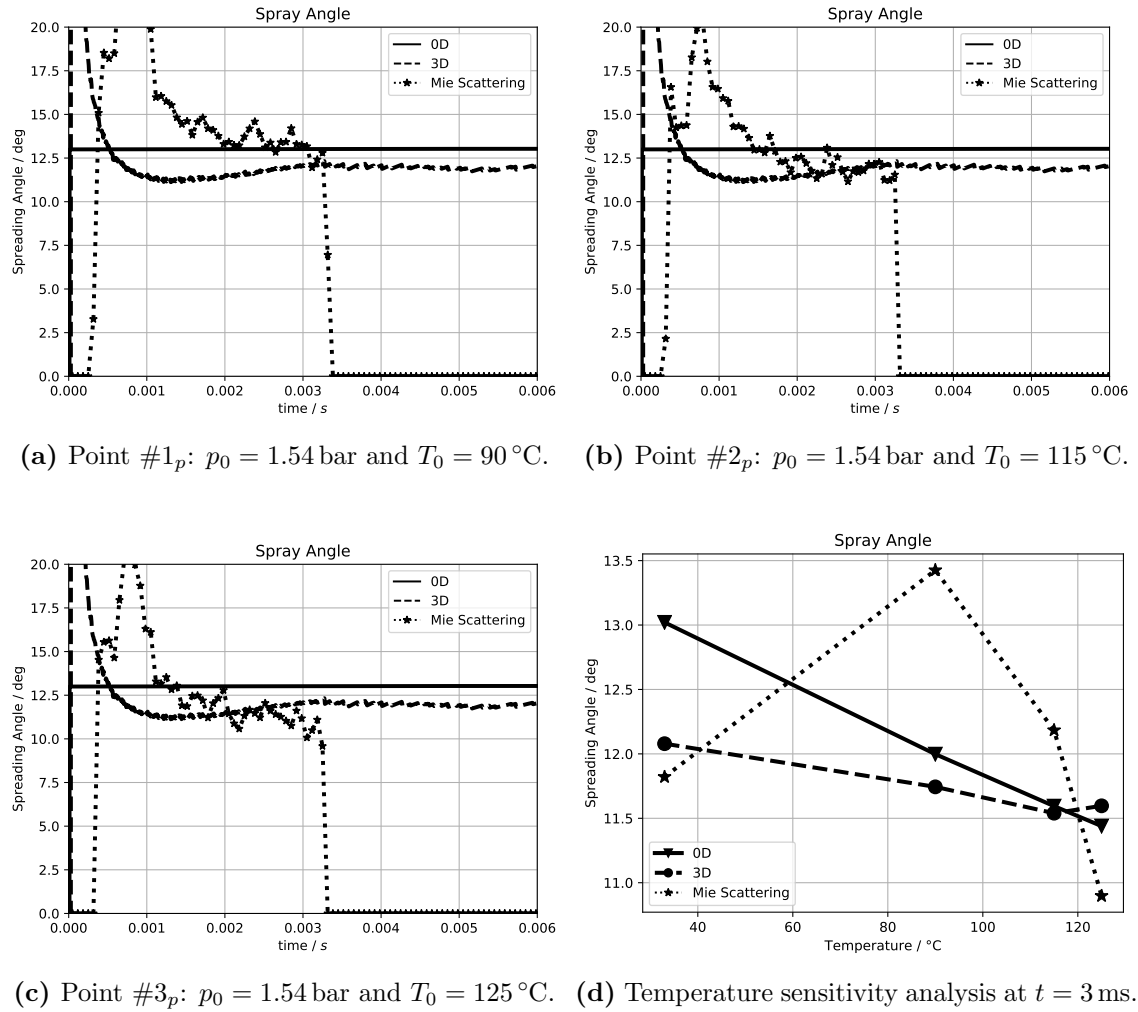
Figure 5.10: Constant-volume vessel (MAGIE): isobaric variations (Table 5.1) – spray spreading angle . (a) – (c): time evolution in different operating conditions. (d): sensitivity to the initial temperature T_0 (also includes the reference point shown in Fig. 5.5 (a)). Solid lines for 0D, dashed lines for 3D and dotted lines for experiment.
