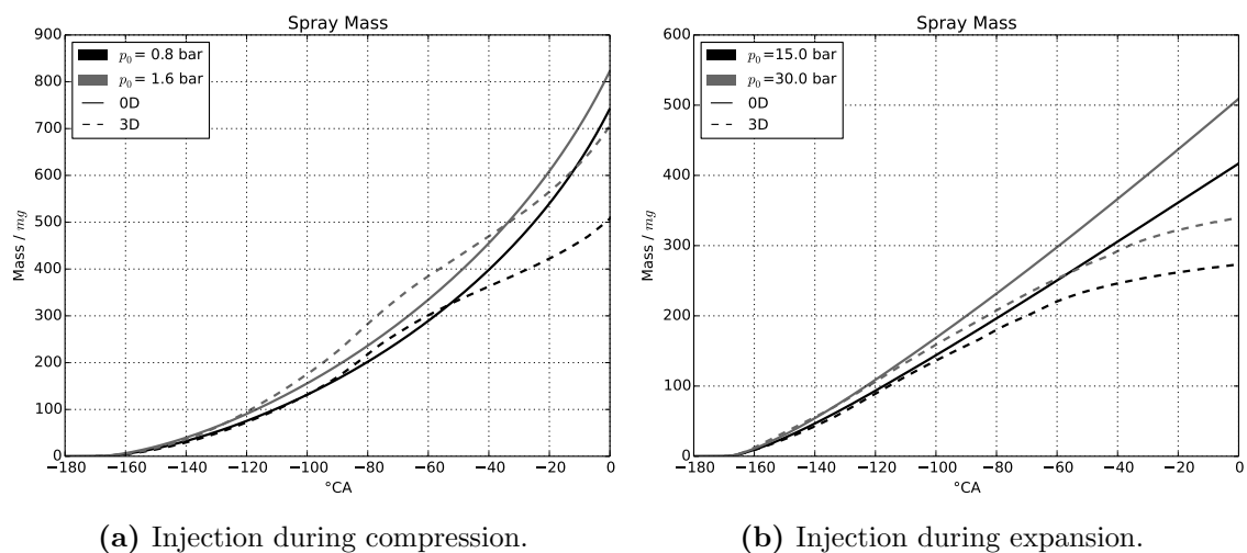
Figure 5.35: Variable-volume vessel – spray mass . (a): injection during compression. (b): injection during expansion. Solid lines for 0D and dashed lines for 3D (reference).
