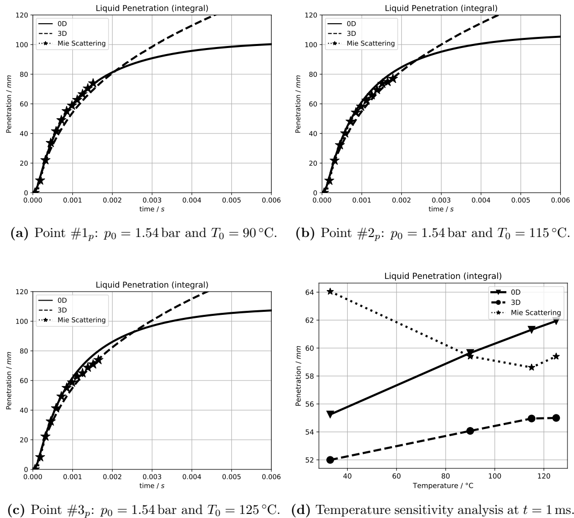
Figure 5.8: Constant-volume vessel (MAGIE): isobaric variations (Table 5.1) – spray liquid penetration. (a) – (c): time evolution in different operating conditions. (d): sensitivity to the initial temperature T_0 (also includes the reference point shown in Fig. 5.5 (a)). Solid lines for 0D, dashed lines for 3D and dotted lines for experiment.
