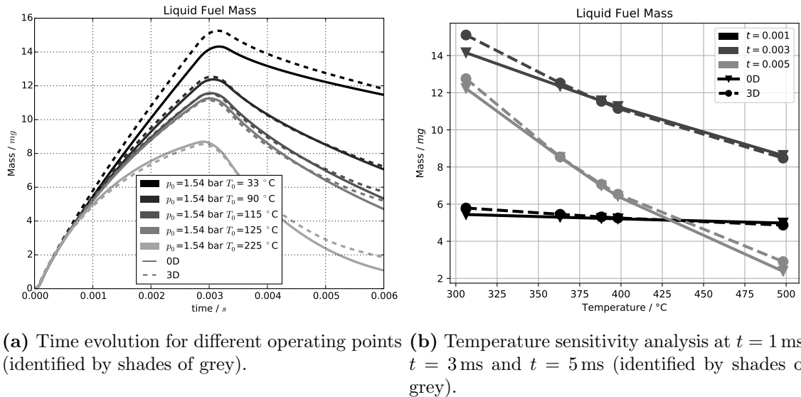
Figure 5.14: Constant-volume vessel (MAGIE): reference point and isobaric variations (Table 5.1)) – liquid fuel mass . Left pane (a): time evolution for different operating conditions. Right pane (b): sensitivity to initial temperature T_0 for different times after SOI. Solid lines for 0D and dashed lines for 3D.
