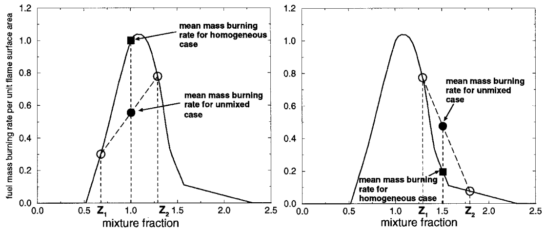
Figure 2.7: Plots of the laminar fuel mass burning rate \dot{M}_f = \rho Y_f S s_L against the mixture fraction Z . Differences in laminar flame speed do not average out because of the non linearity of the s_L(Z) relation: the mean burning rate of a stratified mixture can therefore differ from that of an iso- \bar{Z} homogeneous mixture. Figure from Hélie and Trouvé (2000) .
