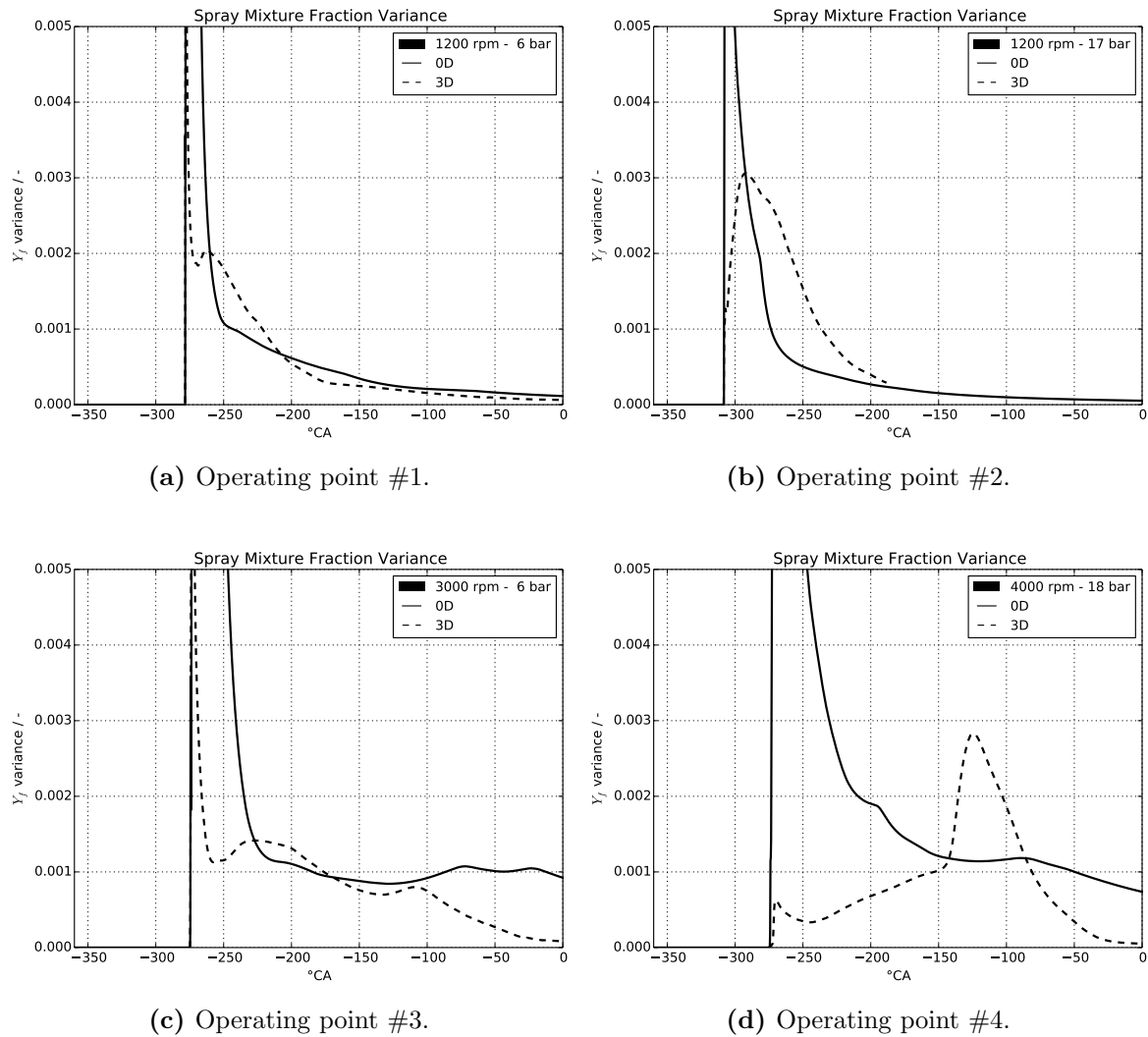
Figure 6.14: Mixture formation in the ICAMDAC engine – mixture fraction Y_F variance: the four panes plot compare 0D (solid lines) and 3D reference data (dashed lines) for each of the operating points in Table 6.2.
