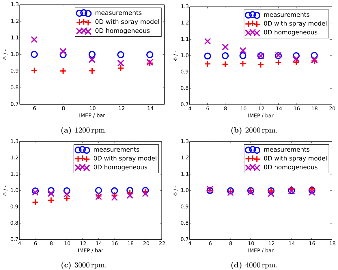
Figure 6.22: ICAMDAC engine. The values of the equivalence ratio are plotted against the nominal IMEP for four different crank speeds. Red “+” for the developed 0D model (with detailed spray description), magenta “X” for the base 0D model (no spray description) and blue “O” for test bed measurements. The operating points shown cover the whole engine map realized in the framework of the ICAMDAC project (de Francqueville, 2013).
