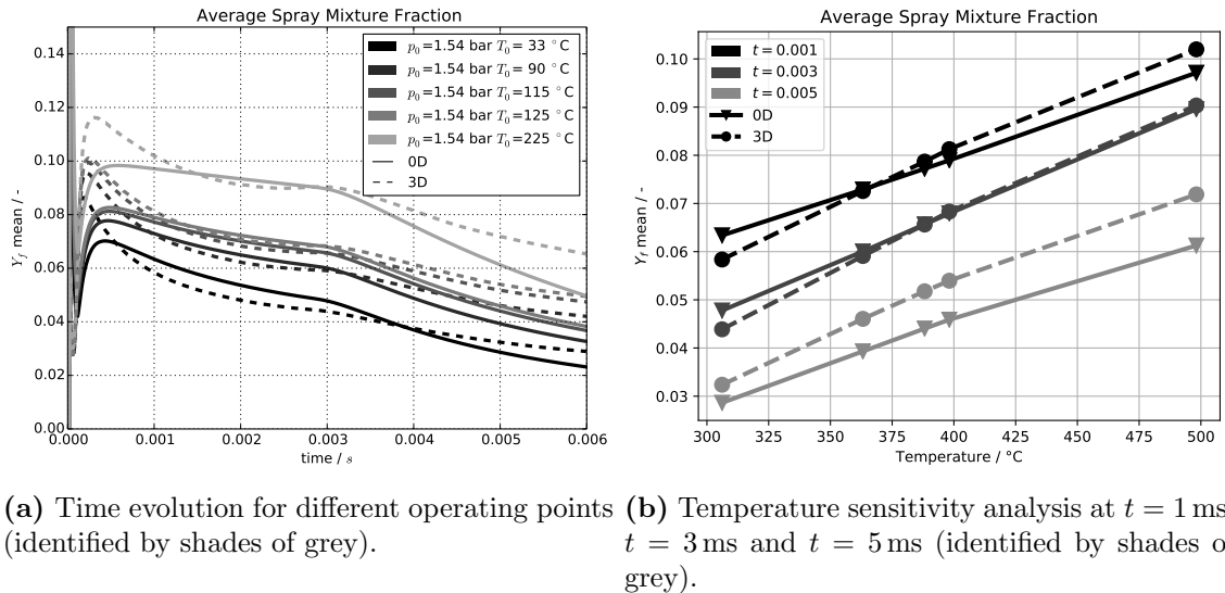
Figure 5.18: Constant-volume vessel (MAGIE): reference point and isobaric variations (Table 5.1) – spray average mixture fraction . Left pane (a): time evolution for different operating conditions. Right pane (b): sensitivity to initial temperature T_0 for different times after SOI. Solid lines for 0D and dashed lines for 3D.
