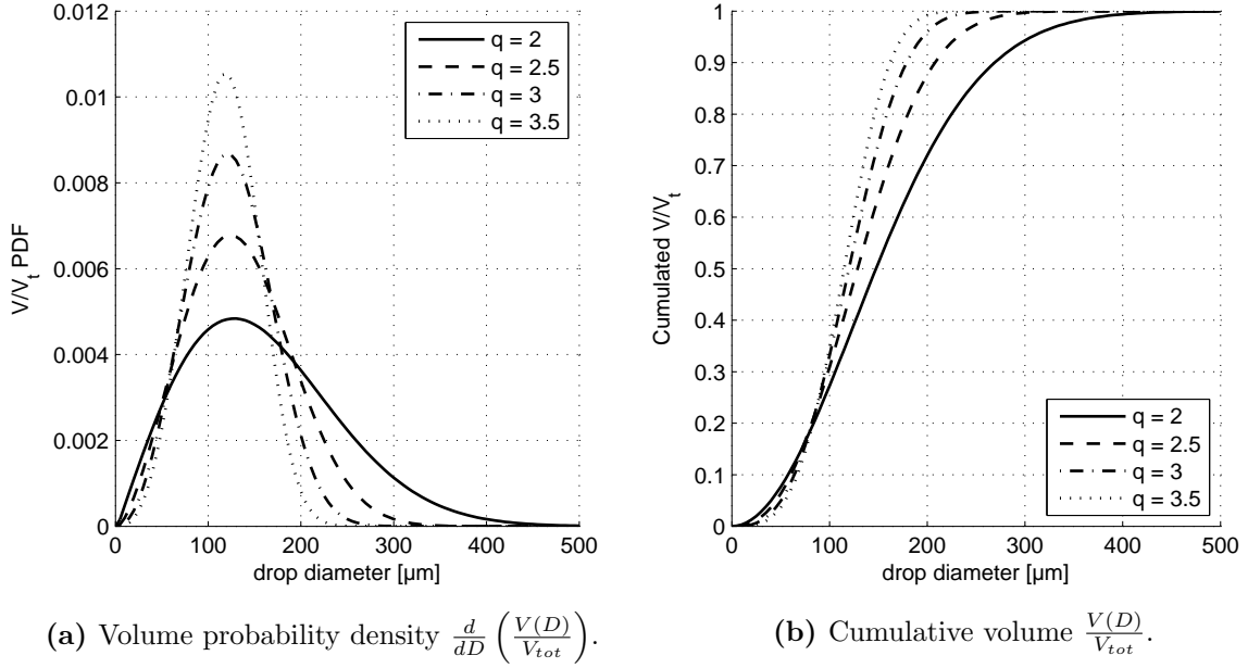
Figure 2.1: Rosin-Rammler distribution for SMD = 100 \mu m and different values of the exponent q .
