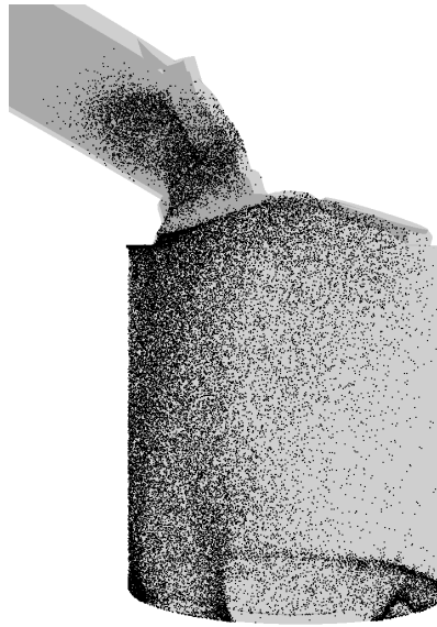
Figure 6.10: 3D RANS simulation of the 3000 rpm 6 bar IMEP operating point. The image shows a snapshot of the disperse phase in the computational domain at -155^{\circ}\text{CA} , right before IVC ( -151.6^{\circ}\text{CA} ). Particles in the intake ducts are a result of backflow.
