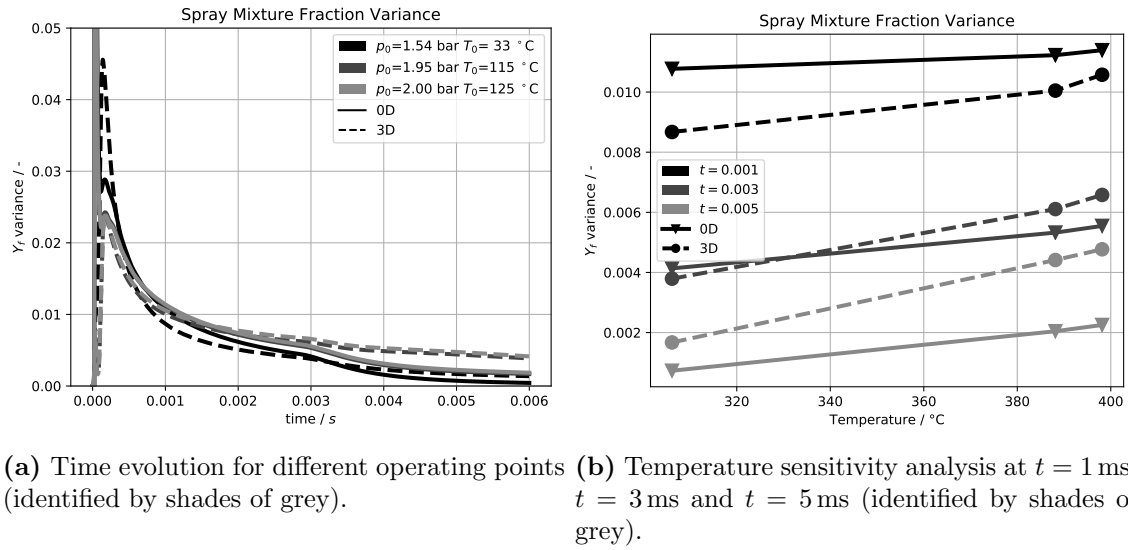
Figure 5.19: Constant-volume vessel (MAGIE): reference point and isopycnic variations (Table 5.1) – spray mixture fraction variance . Left pane (a): time evolution for different operating conditions. Right pane (b): sensitivity to initial temperature T_0 for different times after SOI. Solid lines for 0D and dashed lines for 3D.
