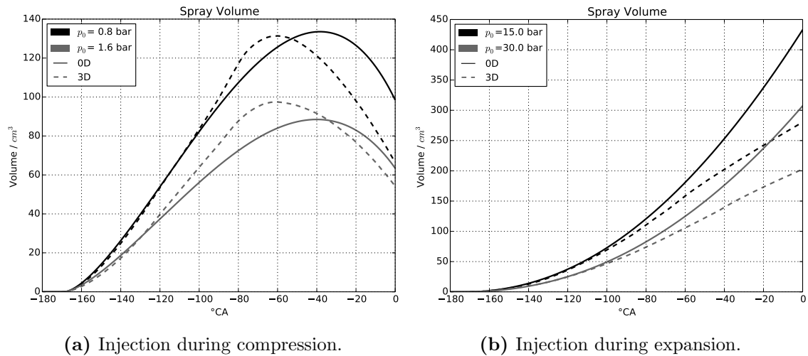
Figure 5.34: Variable-volume vessel – spray volume . (a): injection during compression. (b): injection during expansion. Solid lines for 0D and dashed lines for 3D (reference).
