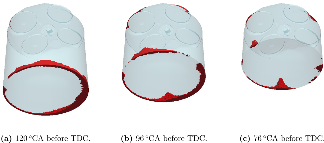
Figure 6.17: ICAMDAC engine: operating point at N = 4000 rpm and \text{IMEP} = 18 bar. The three plots show the computational domain in light blue at different crank angles. The cells with a fuel mass concentration greater than 0.2 ( Y_F > 0.2 ) are highlighted in red, suggesting an accumulation of hot drops at the piston/liner interface.
