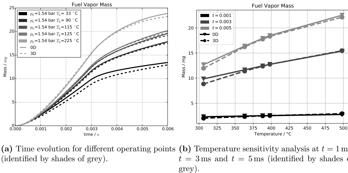
Figure 5.16: Constant-volume vessel (MAGIE): reference point and isobaric variations (Table 5.1) – fuel vapor mass . Left pane (a): time evolution for different operating conditions. Right pane (b): sensitivity to initial temperature T_0 for different times after SOI. Solid lines for 0D and dashed lines for 3D.
