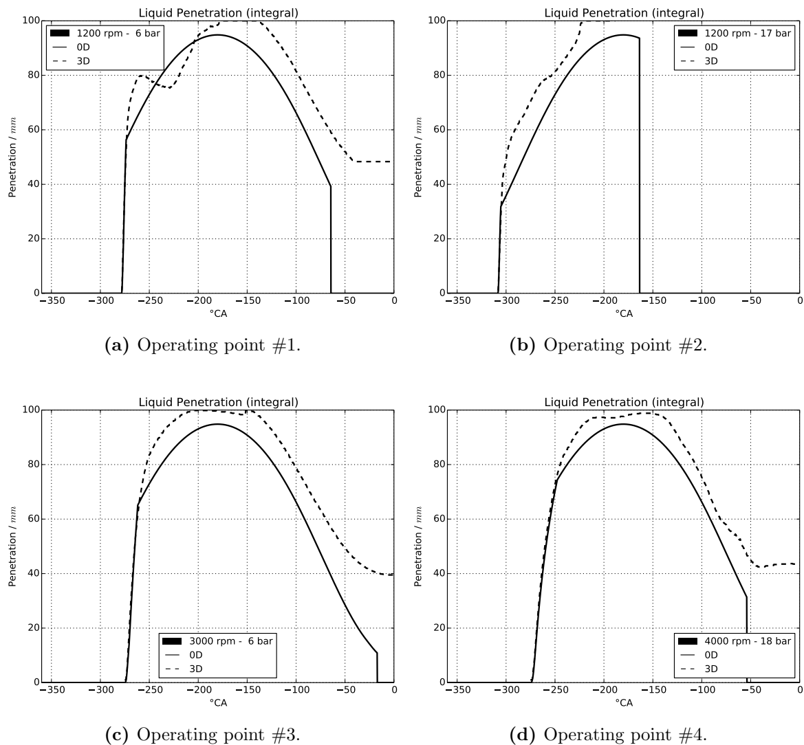
Figure 6.4: Mixture formation in the ICAMDAC engine – liquid penetration: the four plots compare 0D (solid lines) and 3D reference data (dashed lines) for each of the operating points in Table 6.2. The 0D model calculates the liquid penetration until the disperse phase has completely evaporated.
