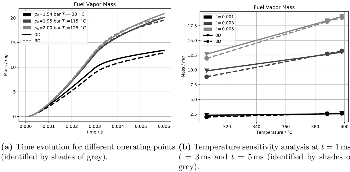
Figure 5.15: Constant-volume vessel (MAGIE): reference point and isopycnic variations (Table 5.1) – fuel vapor mass . Left pane (a): time evolution for different operating conditions. Right pane (b): sensitivity to initial temperature T_0 for different times after SOI. Solid lines for 0D and dashed lines for 3D.
