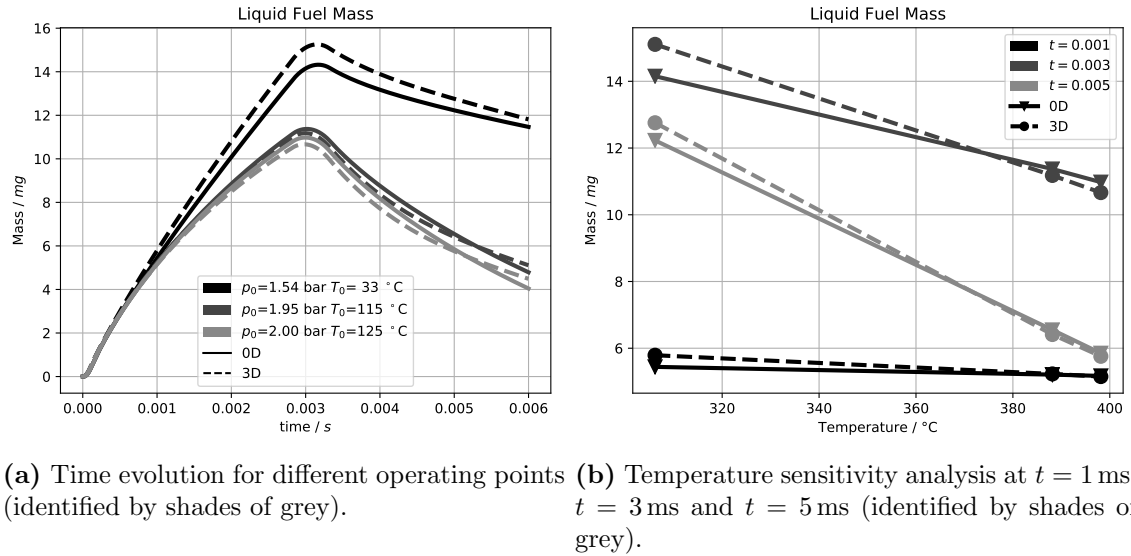
Figure 5.13: Constant-volume vessel (MAGIE): reference point and isopycnic variations (Table 5.1)) – liquid fuel mass . Left pane (a): time evolution for different operating conditions. Right pane (b): sensitivity to initial temperature T_0 for different times after SOI. Solid lines for 0D, dashed lines for 3D and dotted lines for experiment.
