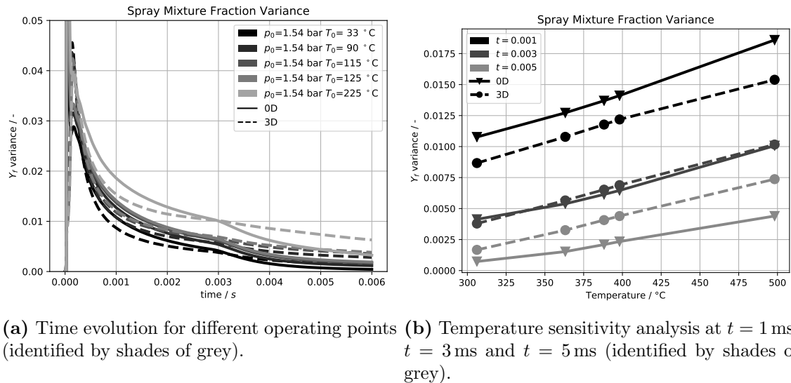
Figure 5.20: Constant-volume vessel (MAGIE): reference point and isobaric variations (Table 5.1) – spray mixture fraction variance . Left pane (a): time evolution for different operating conditions. Right pane (b): sensitivity to initial temperature T_0 for different times after SOI. Solid lines for 0D and dashed lines for 3D.
