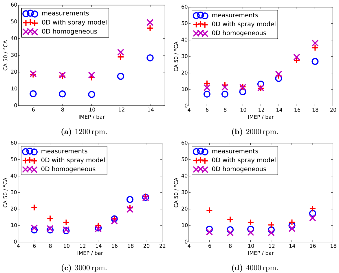
Figure 6.20: ICAMDAC engine: heat release . The values of CA 50 are plotted against the nominal IMEP for four different crank speeds. Red “+” for the developed OD model (with detailed spray description), magenta “X” for the base OD model (no spray description) and blue “O” for test bed measurements. The operating points shown cover the whole engine map realized in the framework of the ICAMDAC project (de Francqueville, 2013).
