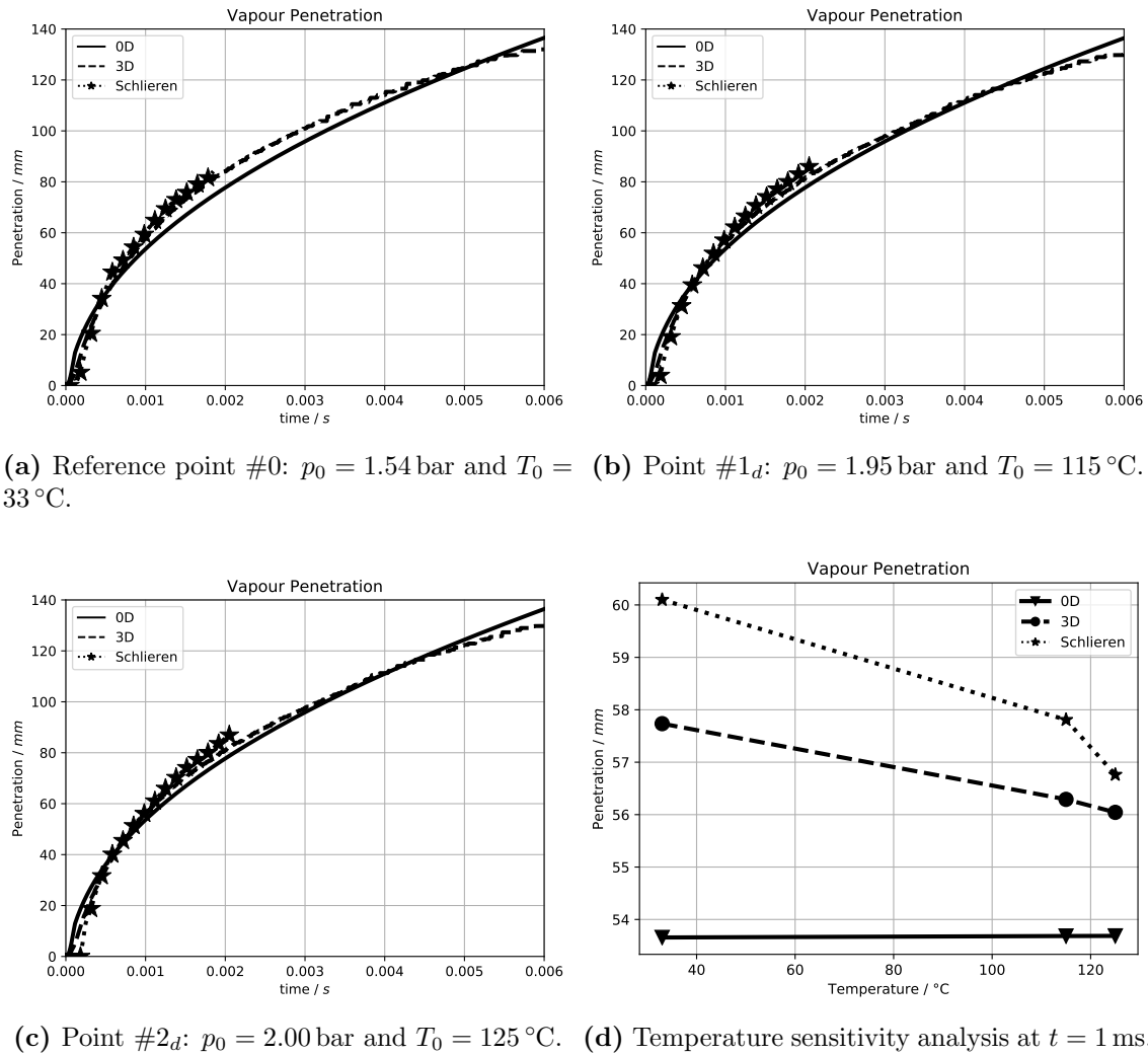
Figure 5.5: Constant-volume vessel (MAGIE): reference point and isopycnic variations (Table 5.1)) – spray vapor penetration . (a) – (c): time evolution in different operating conditions. (d): sensitivity to the initial temperature T_0 (also includes the reference point shown in Fig. 5.5 (a)). Solid lines for 0D, dashed lines for 3D and dotted lines for experiment.
