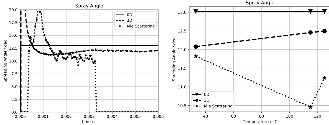
(c) Point #2 d : p_0 = 1.54 bar and T_0 = 125^\circ\text{C} . (d) Temperature sensitivity analysis at t = 3 ms.
