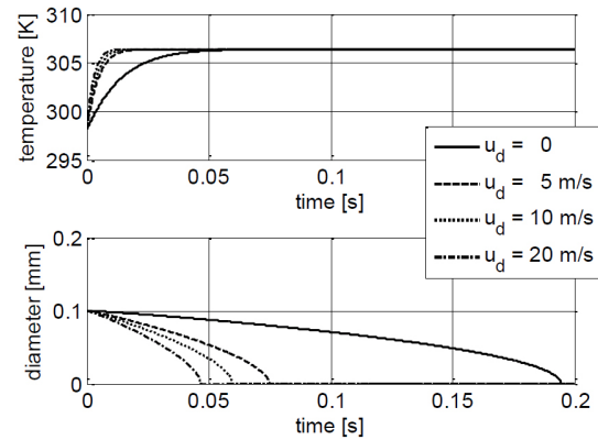
Figure 4. Evolution of the diameter and temperature of an evaporating drop subject to forced convection, for different velocities. Evaporating fuel is isooctane, surrounding gas is air at 2 bar and 100 °C. Drop velocity u_d is held constant.
