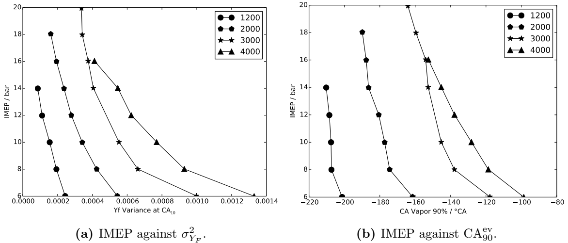
Figure 6.25: ICAMDAC engine: correlation between engine charge and spray statistics. The values of the mesured IMEP are plotted against the computed mixture fraction variance, \sigma_{Y_F}^2 , and the end of evaporation crank angle, CA 90 ev , for four different crank speeds. The operating points shown cover the whole engine map realized in the framework of the ICAMDAC project (de Francqueville, 2013).
