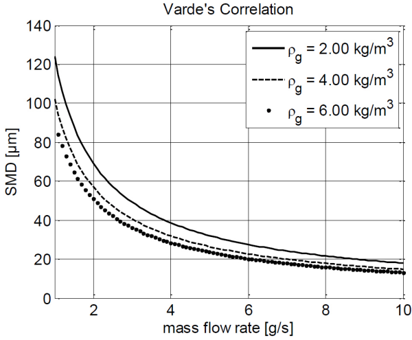
Figure 3. Varde's correlation: Sauter mean diameter against the injection rate, for different gas densities. Fuel is isooctane ( \sigma_l = 18.77 \cdot 10^{-3} N/m and v_l = 5.0 \cdot 10^{-6} m 2 /s), D_{noz} = 200\mu\text{m} .
