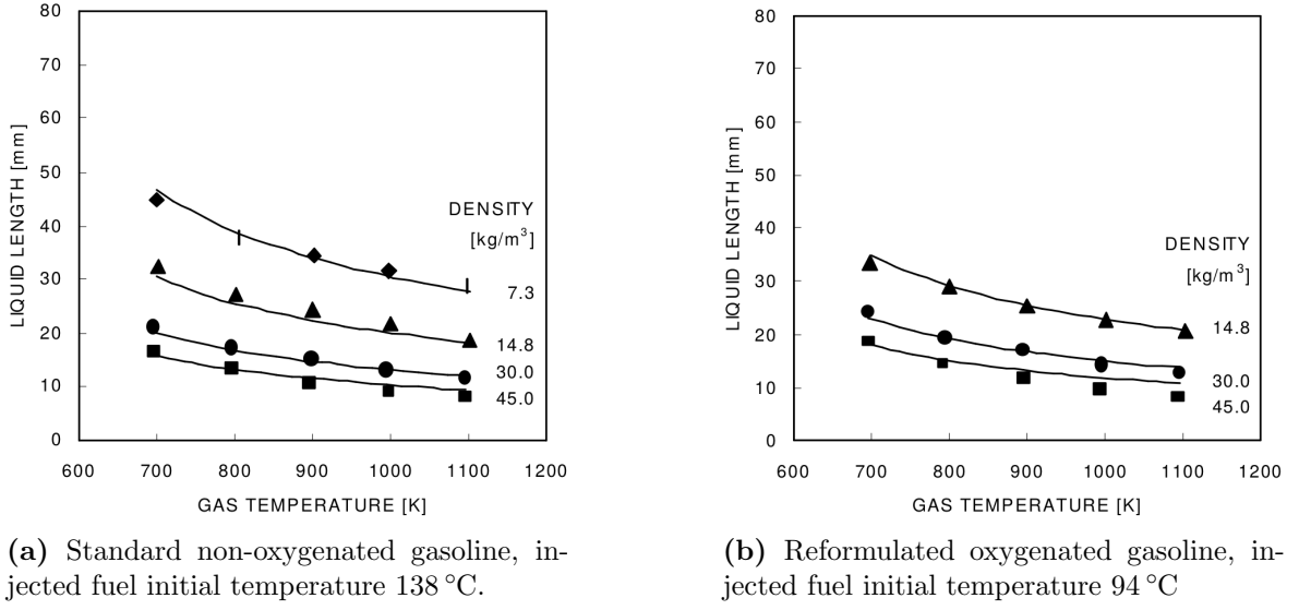
Figure 2.4: Liquid length against cylinder gas temperature for different gas densities: predictions given by Eq.(2.47) (solid lines) are compared to measurements (markers). (a): standard gasoline. (b): oxygenated gasoline. Figures from Higgins et al. (1999).
