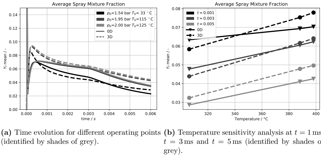
Figure 5.17: Constant-volume vessel (MAGIE): reference point and isopycnic variations (Table 5.1) – spray average mixture fraction . Left pane (a): time evolution for different operating conditions. Right pane (b): sensitivity to initial temperature T_0 for different times after SOI. Solid lines for 0D and dashed lines for 3D.
