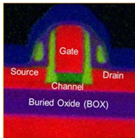
Figure 3. 3 Cross section of the UTBB FDSOI transistor
