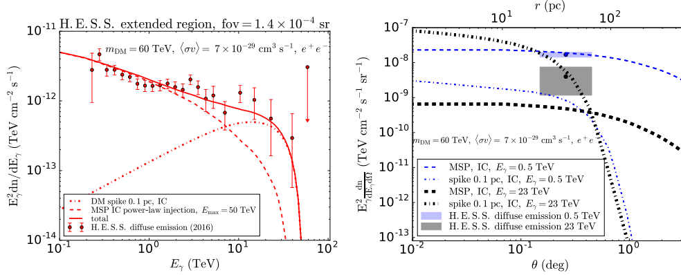
Figure 4.6: VHE emission from a combination of millisecond pulsars and dark matter spike. Left panel: Spectra from 100 GeV to 100 TeV for the H.E.S.S. diffuse emission. IC emission from MSPs is depicted as a dashed line. IC emission from a spike of radius 0.1 pc, for a 60 TeV DM candidate annihilating exclusively to e^+e^- with a cross section of \langle\sigma v\rangle = 7 \times 10^{-29} \text{ cm}^3 \text{ s}^{-1} is shown as a dot-dashed line. The solid line represents the total spectrum. Right panel: IC emission intensity from MSPs (dashed) and a 0.1 pc DM spike (dot-dashed) as a function of angular distance from the GC, at 0.5 TeV (thin blue) and 23 TeV (thick black). The data points at these energies and their statistical error bars are depicted as shaded rectangles. Figures extracted from Ref. [? ].
