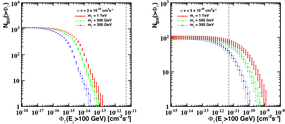
Figure 2.3: Intermediate-mass black hole luminosity functions. Integrated luminosity function of IMBHs for the scenarii A (left panel, IMBH masses of \sim 10^2 M_\odot ), and B (right panel, IMBH masses of \sim 10^5 M_\odot ), respectively, for a Milky Way-sized halo obtained from an average of 200 stochastic realizations. Neutralino masses of 300, 500 GeV and 1 TeV, respectively, and a velocity-weighted annihilation cross section \sigma v = 3 \times 10^{-26} \text{ cm}^3 \text{ s}^{-1} are considered. Figure extracted from Ref. [? ].
