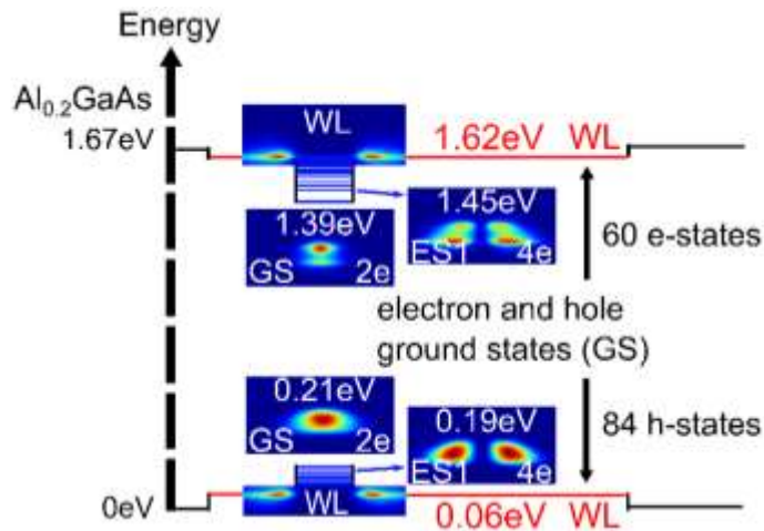
Figure 3.3-22: Energy diagram of a “medium” size typical In(Ga)As QD with \text{Al}_{0.2}\text{GaAs} host material in black lines, InGaAs WL in red lines and ground state (GS) with excited states (ES) in blue lines. There are about 60 electron states and 84 hole states from GS to WL energies. Also electron wavefunction probability color plots side cuts ( y=0 , middle of QD) are shown for electron and hole GS, ES and also WL state.
