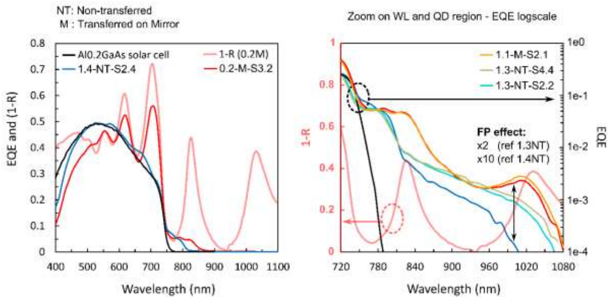
Figure 5.2-5: EQE comparison of non-transferred and transferred solar cells. Reflectometry measurements is shown as an indication of the FP cavity. A typical \text{Al}_{0.2}\text{GaAs} p-i-n solar cell grown in Okada laboratory is shown which gives an indication on the host material bandgap. On the right figure, we zoom on the WL and QD spectral region. WL bandgap is around 800 nm and QD bandgaps depend on the sample position as previously indicated in chapter 3: Figure 3.3-4. We estimate a x2 or x10 FP ratio enhancement in comparison with non-transferred solar cells form 1.3 or 1.4 samples which positions are indicated in Figure 5.2-2.
