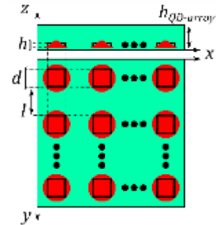
Figure 3.1-4: Schematic representation of a QD array: x-z side view (top) and x-y top view (bottom). QD diameter ( d ), height ( h ) and lateral interdot spacing ( l ) are shown. Delocalized nature of light (green) compared to localized electron wavefunction in QDs (red).
