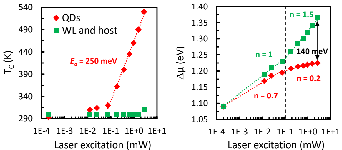
Figure 4.1-35: Evolution of temperatures T_c (left) and QFLS \Delta\mu (right) for carrier populations inside QDs (red) in comparison with population in the WL and \text{Al}_{0.2}\text{GaAs} host material. An activation energy of 250 meV is found related to temperature increase inside QDs. Different behavior of QFLS are noticed for low-excitation ( < 0.2 mW) and high-excitation regimes ( > 0.2 mW). For WL and host material we find same idealities of n=1 and n=1.5 as in the optical I-V investigation. For QDs, we find about the same ideality for the low-excitation regime, n=0.7 as in the optical I-V investigation. However, for high-excitation it is very reduced ( n=0.2 ). A maximum difference of 140 meV is found between QFLS for the highest laser excitation.
