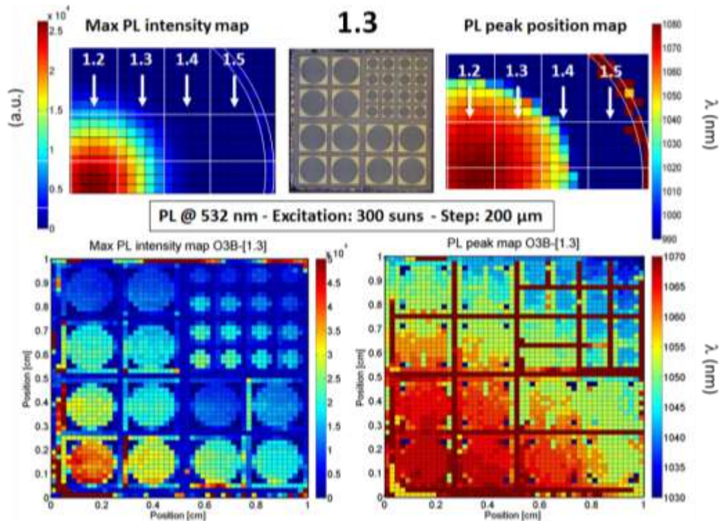
Figure 3.3-3: Non-transferred (NT) samples fabricated and their positions on wafer Okd-3. Sample 1.2NT is in the center and sample 1.5NT on the edge. As an example detailed PL mapping of 1.3NT sample is given. Colorbar scale are not the same for top and bottom figures.
