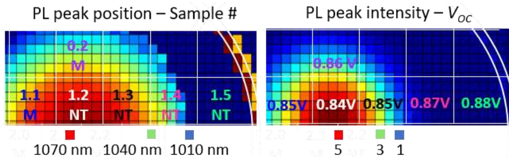
Figure 5.2-4: Comparison of non-transferred (NT) and transferred-on-mirror (M) samples fabricated from Okd-3 3-inch wafer growth. PL mapping results are shown to indicate their positions as in Figure 5.2-2. (left) PL peak position and sample indicative number. (right) PL peak intensity and averaged V_{oc} of characterized solar cells for each sample.
