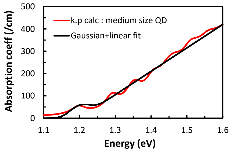
Figure 4.1-25: Absorption coefficient deduce from k-p calculation (in red) for medium size QDs with GS at 1.2 eV and same QDs density as in O3BNT1.4 sample which means 10 layers of QDs with about 700 QDs/ \mu\text{m}^2 for a 515 nm-thick solar cell absorber thickness. Gaussian fit plus linear (in black) to estimate absorption profile trend for a Gaussian distribution.
