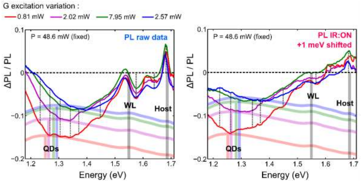
Figure 4.2-8: \Delta\text{PL}/\text{PL} ratio evolution with increasing the 532 nm laser excitation (G) for a fixed IR pump (P). On the left, the ratio is presented for PL raw data and on the right with a +1 meV shift correction on PL IR : ON that is attributed to IR laser heating. PL spectral IR : OFF are arbitrarily positioned in the background as an guide for the eye. Different bands of colors represent the position of QDs PL peaks for different excitation regimes. Grey bands are also positioned at WL and host material PL peaks energy positions. Dotted black lines are underlining local maxima.
