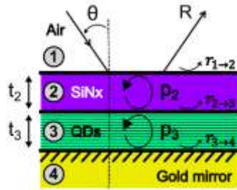
Figure 3.4-13: Schematic drawing of the structure for the calculation of the reflection in a double layer Fabry-Pérot (DLFP) structure following Rouard's method with the analytical expression of reflection in function of Fresnel coefficients, wave propagation and reflection.
