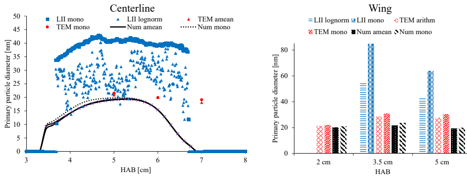
Figure 6.11: d_{pp} along the centerline and at three HAB on the wing for F80. Comparison of numerical results to the LII results [84] and the TEM data [77]
