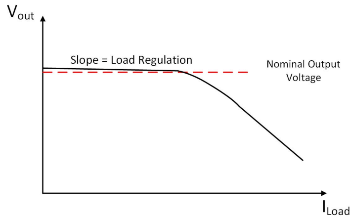
Figure 3.3 – Load Regulation
