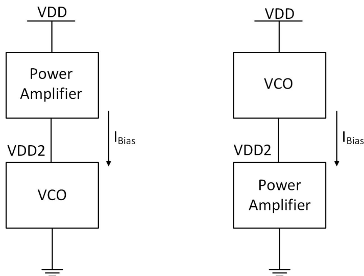
Figure 4.25 – Block diagrams of current reuse transmitter. The two possible solutions are reported depending on the position of the VCO and the PA
