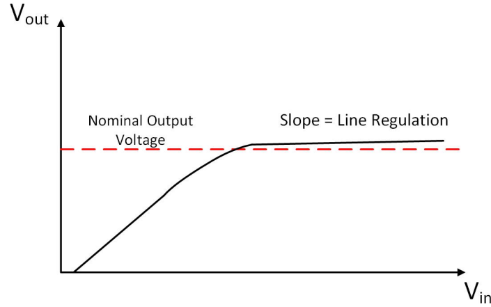
Figure 3.4 – Line Regulation
