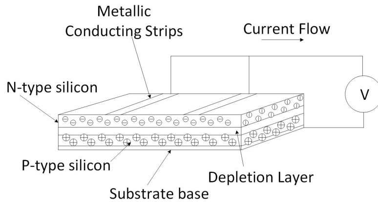
Figure 1.1 – Section of Photovoltaic Cell
