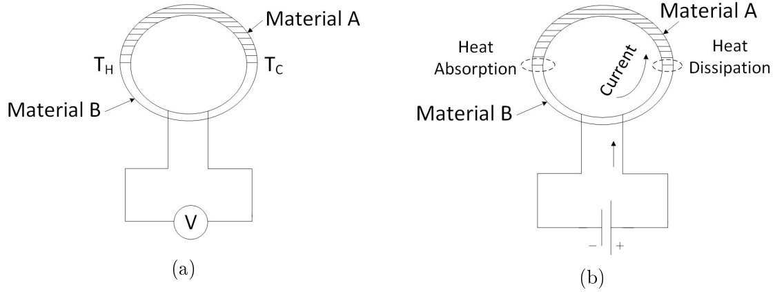
Figure 1.3 – (a) Seebeck effect, the generated voltage is proportional to the temperature gradient between the hot point T_H and the cold point T_C (b) Peltier effect the current generated by the applied voltage causes a thermal diffusion from the heat dissipation to the heat absorption.
