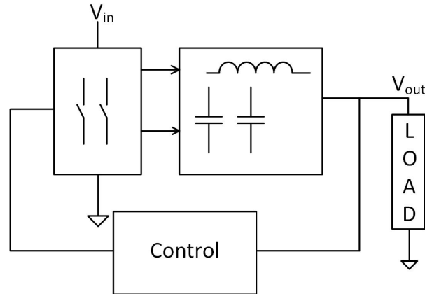
Figure 3.6 – Switching Regulator
