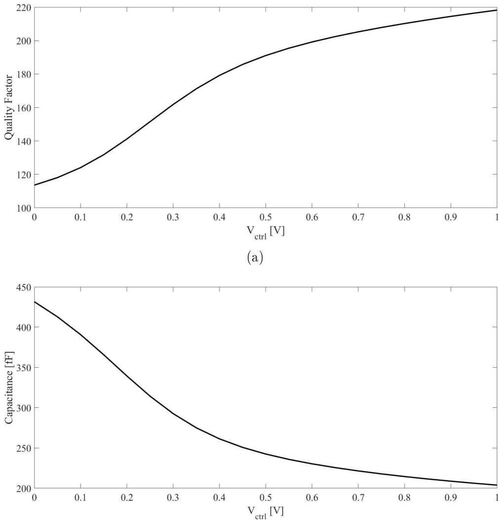
Figure 4.20 – Varactor quality factor (a) and capacitance versus tuning voltage (b)
