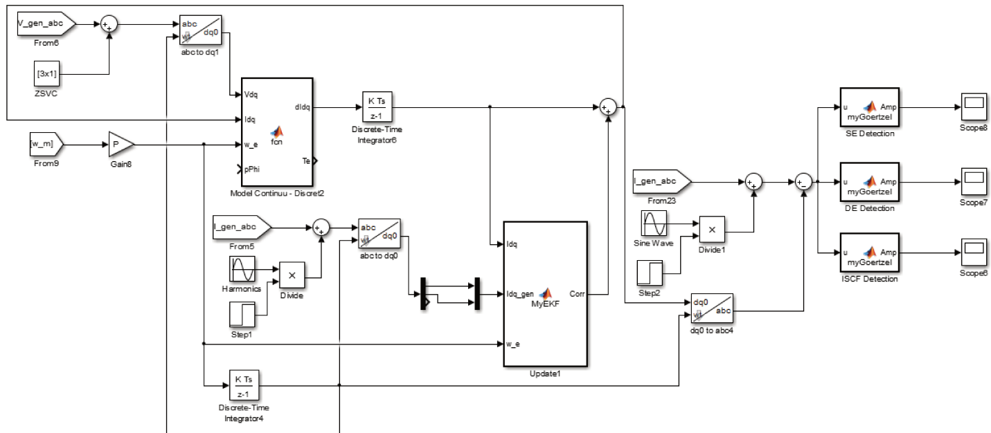
FIGURE D.3: The Simulink schematic of the fault diagnosis using the Extended Kalman Filter and the Goertzel Filters.
