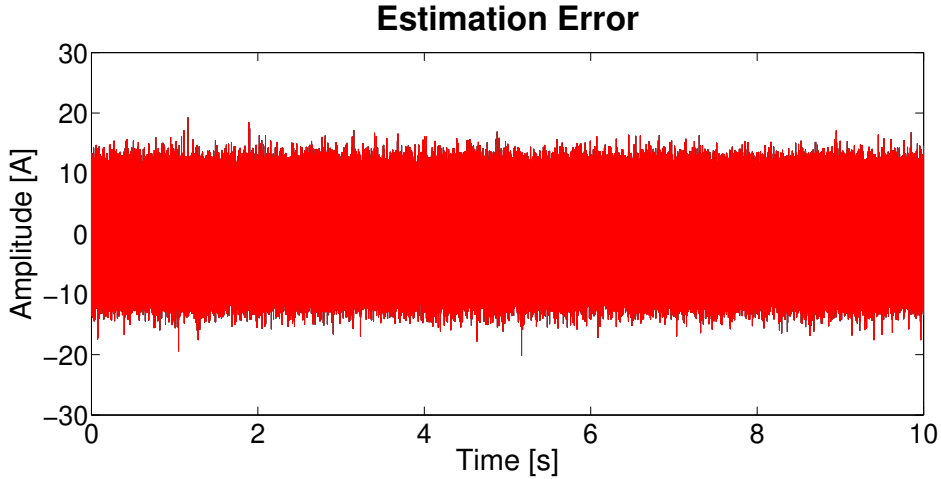
FIGURE 3.11: The estimation error using the EKF with the method from (Akhlaghi, Zhou, and Huang, 2017), in the presence of zero mean noises.
