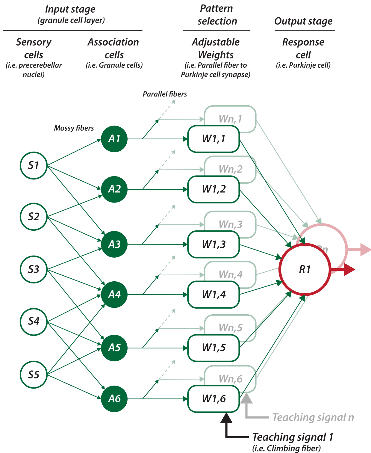
Figure 7 : The Marr-Albus-Ito model for supervised learning
