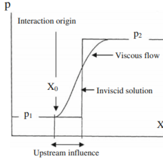
FIGURE 1.7 – Pressure distribution at the wall for an inviscid shock wave regular reflection and for a viscous weak SWBLI from Délerly and Dussauge [2009].
