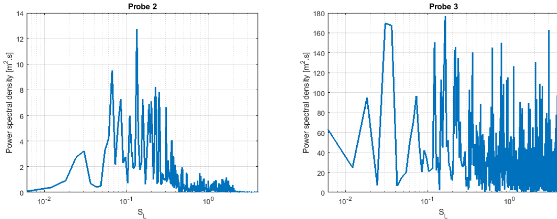
FIGURE 4.9 – Premultiplied power spectral density of the longitudinal velocity component. Left: probe 2. Right: probe 3.
