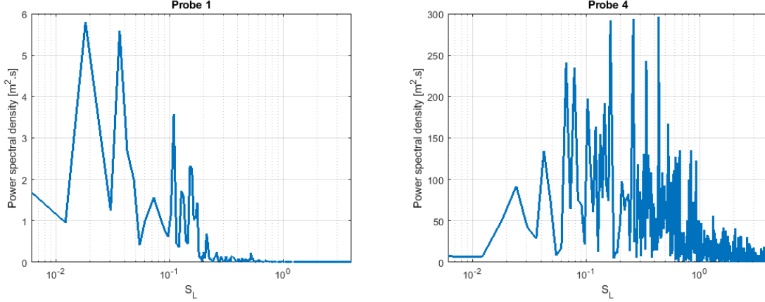
FIGURE 4.8 – Premultiplied power spectral density of the longitudinal velocity component. Left: probe 1. Right: probe 4.
