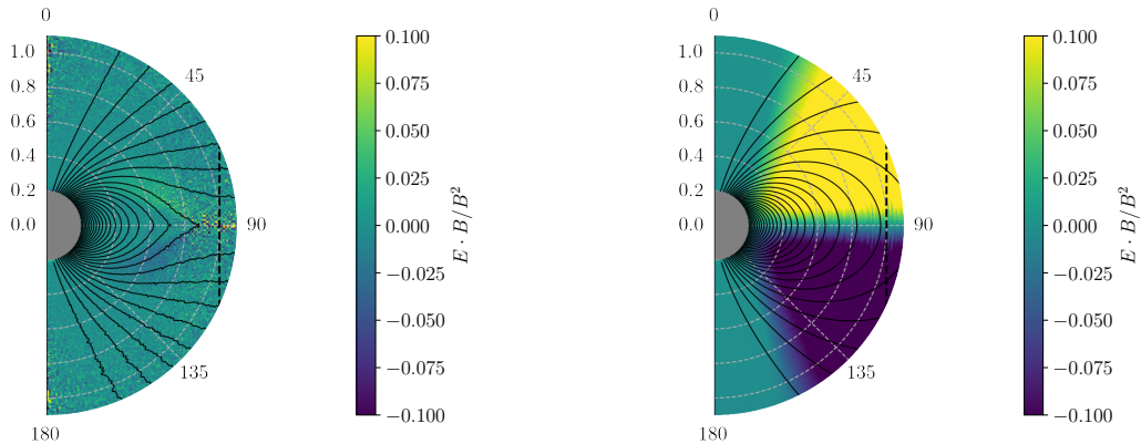
Figure 3.8: Parallel electric field \mathbf{E} \cdot \mathbf{B}/B^2 in the inner part of the magnetosphere ( r \leq R_{\text{LC}} ), for f_{\text{pp}} = 0.01 (left) and f_{\text{pp}} = 0.30 (right).
