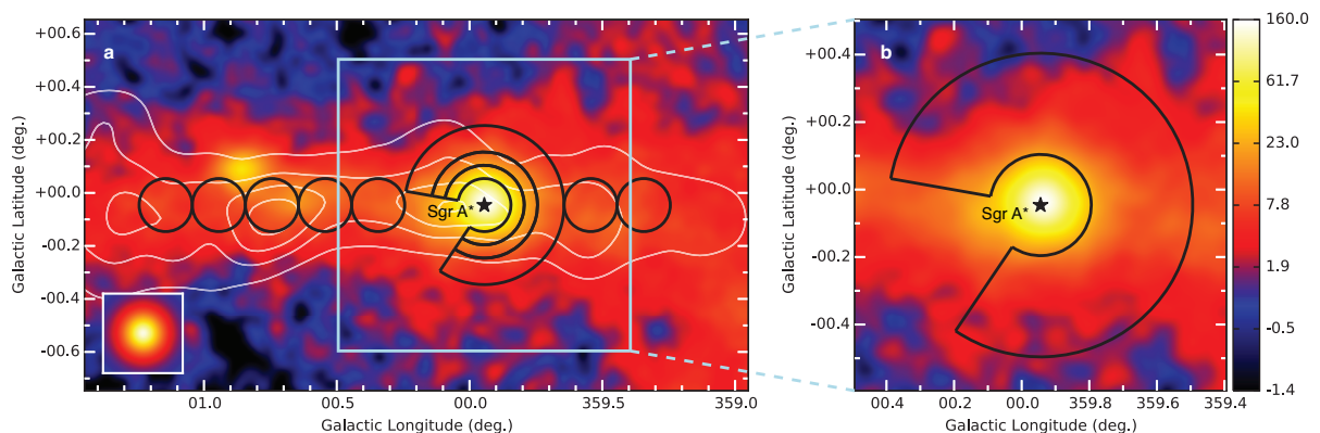
Figure 4.2: Galactic center region in very-high-energy gamma rays, from HESS Collaboration et al. (2016). The color scale indicate counts, white contours indicate the molecular gas density distribution. The right panel is a zoomed view around Sagittarius A*, and the black contour define the 50 pc region used to extract the diffuse emission spectrum.
