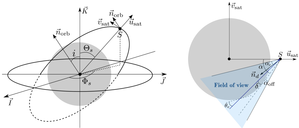
Figure 6.3: Orbital characteristics and notations (left) and illustration of the geometrical configuration in the orbital plane ( \vec{u}_{sat}, \vec{v}_{sat} ) (right). The satellite is located at point S . A neutrino arriving at the detector is characterized by its Earth emergence angle \theta_e and the corresponding viewing angle \delta from the satellite point of view. The detector has a conical FOV of opening angle \alpha_c , with an offset angle \alpha_{off} (away from the Earth limb) and pointing direction \vec{n}_d .
