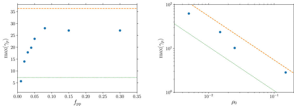
Figure 3.9: Maximum Lorentz factor of escaping protons, as a function of f_{\text{pp}} for \rho_0 = 0.015 (left) and of \rho_0 = m_e c^2/eB for f_{\text{pp}} = 0.05 (right). The dots correspond to simulation results, whereas the lines represent the maximum Lorentz factor of protons experiencing the vacuum potential drop, from pole to equator (orange, dashed) or across the polar cap (green, dotted).
