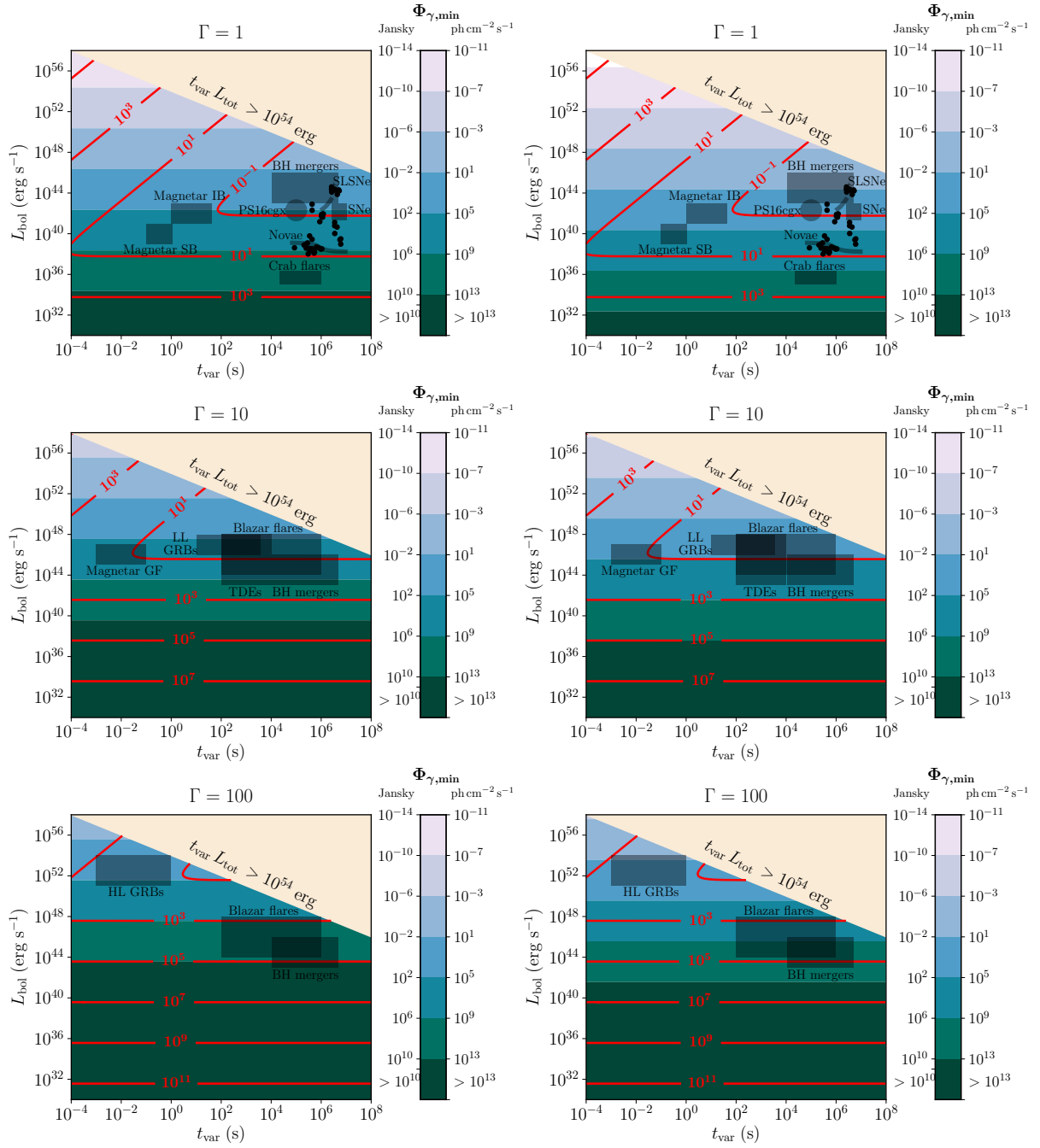
Figure 2.3: What is the minimum source photon flux required to enable neutrino detection with IceCube? The color map shows the minimum photon flux \Phi_{\gamma, \text{min}} (in Jy and \text{ph cm}^{-2} \text{s}^{-1} ) as a function of the bolometric luminosity L_{\text{bol}} and the variability timescale t_{\text{var}} of the flaring event for an outflow bulk Lorentz factor \Gamma = 1, 10, 100 . A neutrino flare can be detectable if the observed photon flux \Phi_{\gamma, \text{obs}} \gtrsim \Phi_{\gamma, \text{min}} , above the minimum threshold energy \epsilon_{\text{th}} (red lines) for soft photon spectra, and at the observed photon break energy \epsilon_b for hard spectra. Here \eta_B = 1 . On the left \eta_p = 1 and on the right \eta_p = 100 . Overlaid objects as in figure 2.2. Type Ibc supernovae should be treated with care (see Section 2.5.2).
