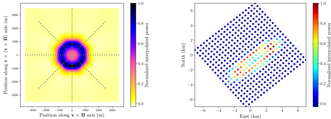
Figure 6.17: For one shower, normalized interpolated power in the v \times B - v \times v \times B plane with the star shape pattern superimposed (left) and projected on the ground on the antenna array (right).
