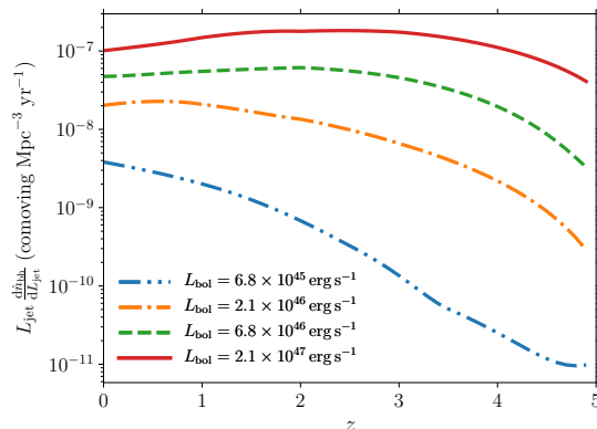
Figure 5.6: Comoving TDE luminosity density in their medium state as a function of redshift, as derived in our model, for \dot{N}_{\text{TDE}} = 10^{-5} \text{ yr}^{-1} . The different luminosities correspond to different black hole masses.
