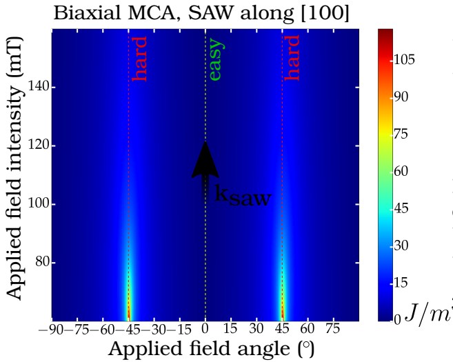
Figure 2.16: Norm, \|\text{Re}(\mathbf{T})\|_{[100]} = \left| \frac{B_1 \sin(2\varphi)}{\omega^2 - \omega_0^2} \right| \sqrt{A_\theta^2 + A_\varphi^2} vs intensity and direction of the magnetic field.
