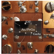
Figure 4.13: Chamber, used for the acoustic measurements.
