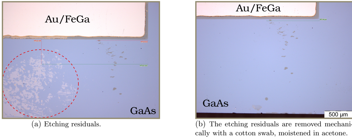
Figure 4.7: Result of the wet etching. Red dashed line encircles the residuals of the etched material. As can be seen, the acid attacked under the resist, resulting in a non-straight border of the ferromagnetic film square.
