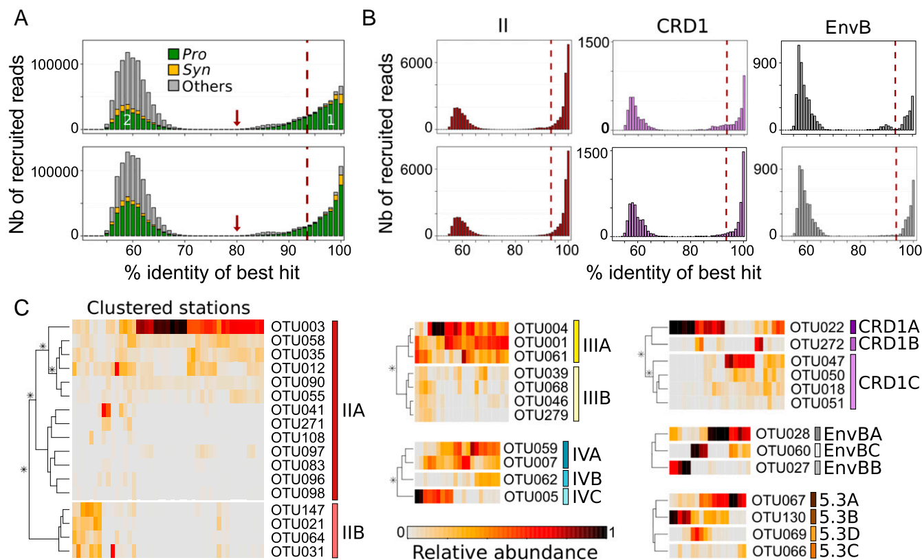
Fig. 2. Percent identity of Tara Oceans petB - mi tags versus sequences of the reference database and abundance at different stations along the transect of OTUs clustered into ESTUs. (A) Distribution of the percent identity of best hits of all petB candidate reads recruited from the Tara Oceans bacterial-size fraction metagenomes against the petB reference database. Populations 1 and 2 correspond, respectively, to genuine petB reads and to nonspecific signal, due either to petB reads from organisms not included in the reference database or to petB -related genes. The gray part in population 1 corresponds to petB reads attributable to photosynthetic organisms of the reference database other than Prochlorococcus and Synechococcus . The red arrow shows the 80% cutoff used to separate the petB signal from noise. The Top and Bottom panels correspond to recruitments made before and after addition of the 136 newly assembled environmental petB sequences, respectively. (B) Same as A but for some selected Synechococcus taxa (see Fig. S2 for all other picocyanobacterial taxa). (C) Determination of ESTUs based on the distribution patterns of within-clade 94% OTUs. At each station, the number of reads assigned to a given OTU is normalized by the total number of reads assigned to the clade in this station. Stations and OTUs are filtered based on the number of reads recruited and hierarchically clustered (Bray–Curtis distance) according to distribution pattern. Only Synechococcus clades split into different ESTUs are shown (see Fig. S4 for Prochlorococcus ). Stars indicate nodes supported by a P value < 0.05 as determined using similarity profile analysis (SIMPROF; test not applicable to pair comparisons).
