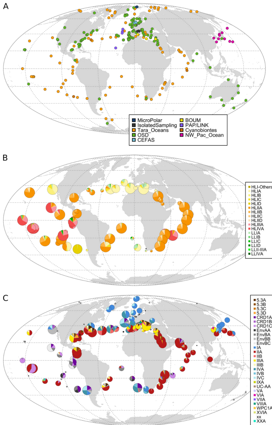
Figure 64 Worldwide distribution of marine picocyanobacterial taxa as assessed using petB gene. A. Transects of all the cruises and sampling campaign for which petB metabarcodes or petB miTags were analysed during this PhD. B. Global distribution of Prochlorococcus ESTUs. The size of circles is proportional to the number of petB reads. Only Tara Oceans transect is shown, as Prochlorococcus petB is not well amplified by primers used for metabarcodes, and this genus was almost absent from OSD dataset. C. Global distribution of Synechococcus ESTUs.
