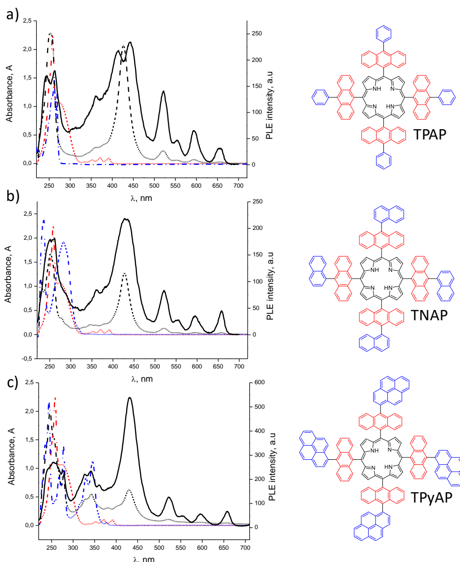
Fig. IV-7 PLE spectra (black solid lines, \lambda_{\text{exc}} = 720 \text{ nm} ) in DCM of a) TPAP ; b) TNAP ; c) TPyAP ; superimposed with the absorption spectra (dash lines) of reference external PAHs (toluene/naphthalene/pyrene, blue), 9-bromoanthracene (red) and corresponding TPAP , TNAP , TPyAP (black).
