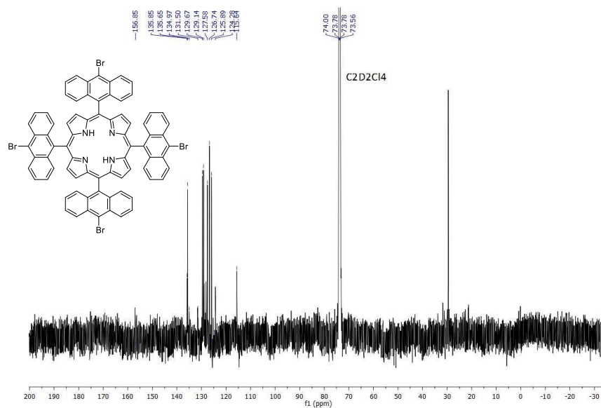
Fig. II-7 13 C NMR spectrum of BrTAP (125 MHz, C 2 D 2 Cl 4 , 333K).
