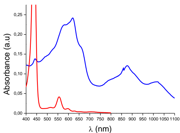
Fig. III-21 Absorption spectra of tetra-fused ZnTPyP (blue line) and starting ZnTPyP (red line). Insert caption showed the change of colour of the solutions of the starting material and of the fused product.
