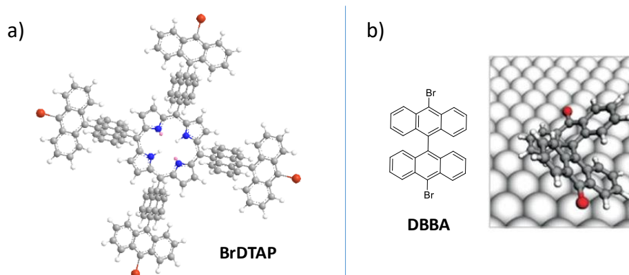
Fig. V-1 a) Calculated 3D model of BrDTAP ; b) chemical structure and illustration of the perpendicular arrangement the two adjacent anthracenes of DBBA on surface.
