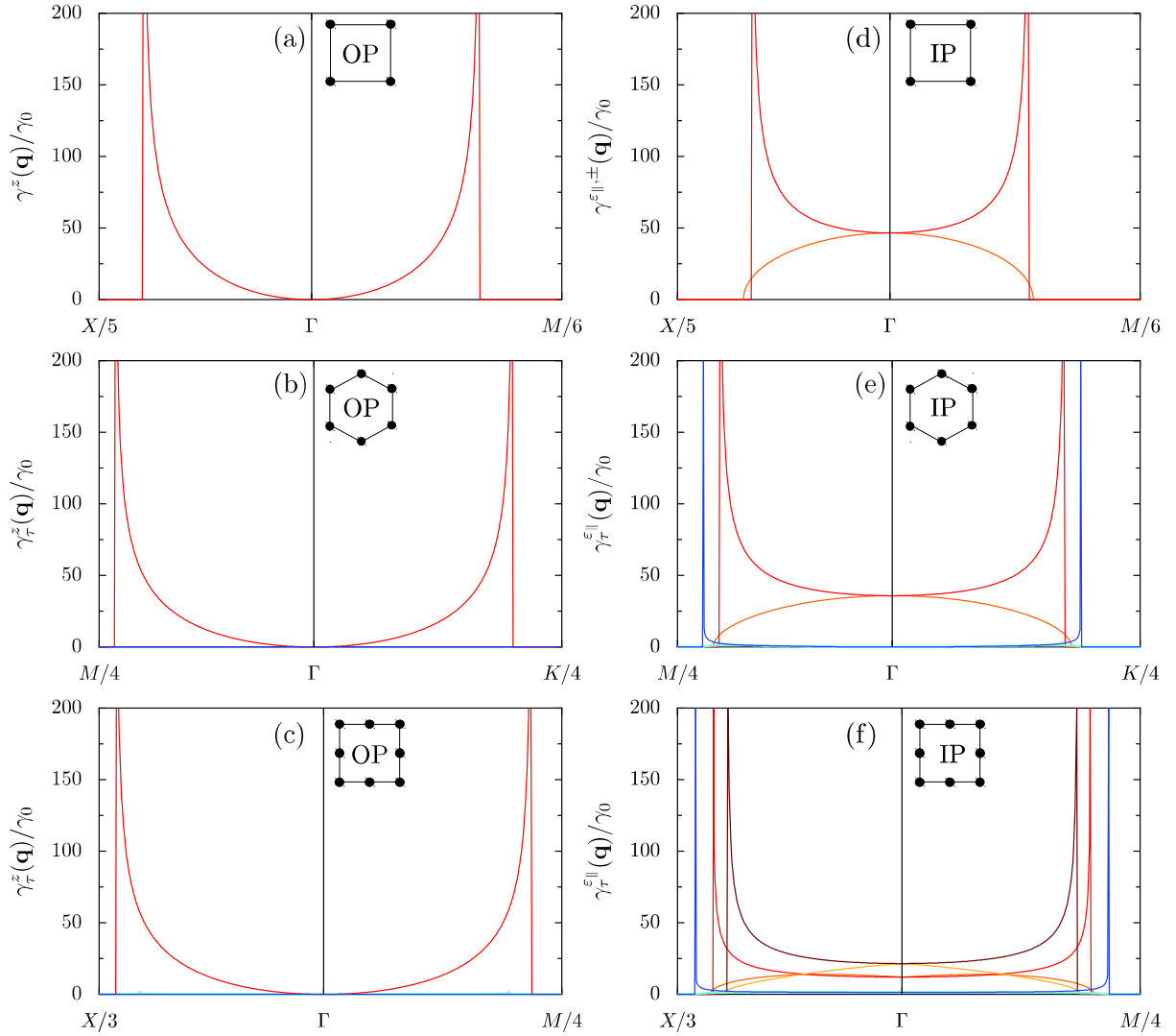
Figure 6.3: The colored lines display the radiative damping rate \gamma_r^\varepsilon(\mathbf{q}) from Eq. (6.33) [scaled by \gamma_0 , cf. Eq. (1.7)] for (a),(d) the square, (b),(e) the honeycomb, and (c),(f) the Lieb lattices. Panels (a)–(c) [(d)–(f)] show the damping for the OP [IP] modes. Same parameters as in Fig. 6.1.
