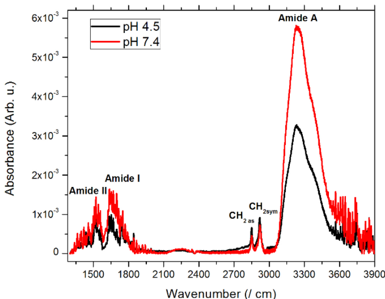
Figure 58. FTIR spectra of \alpha - E. coli immobilized on MHDA/MUDO (1:9) SAM-coated GaAs surface following 1-hour exposure to 100 \mu g/mL antibody solutions at different pH conditions.
