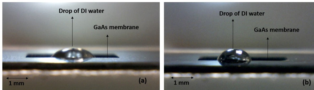
Figure 47: Photos of a 2 \mu l drop of deionized water on the surface of GaAs membrane (a) freshly deoxidized and (b) functionalized with MHDA/MUDO (1:9) (N = 6 samples)
