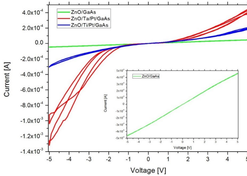
Figure 39. I-V characteristic of ZnO/GaAs and ZnO/Pt/GaAs devices
