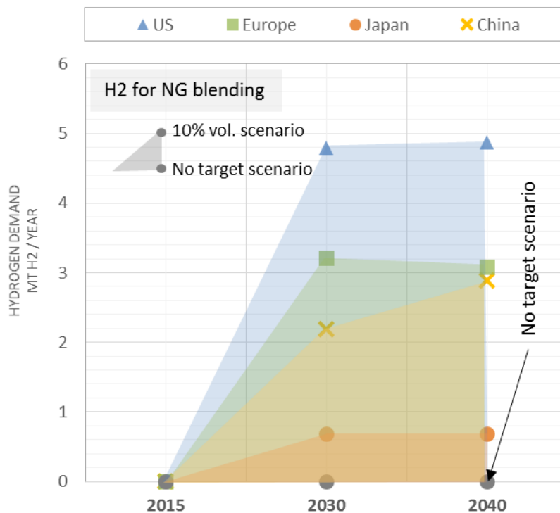
Figure 14: Prospective potential of hydrogen injection into NG networks in the four regions
