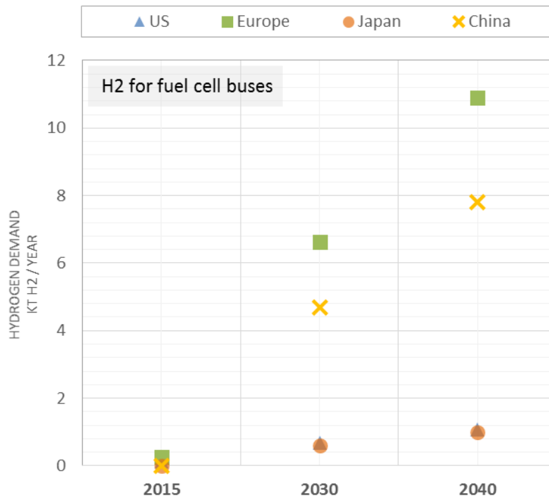
Figure 11: Prospective hydrogen demand for fuel cell bus fleets in the four regions (the US and Japan data has been superimposed)
