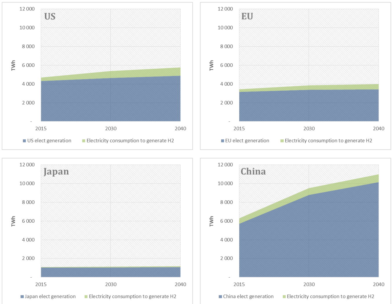
Figure 16: Prospective additional electricity demand for hydrogen generation via electrolysis in the four regions
