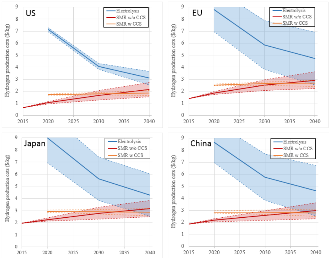
Figure 31: Hydrogen production cost evolution in the considered regions
