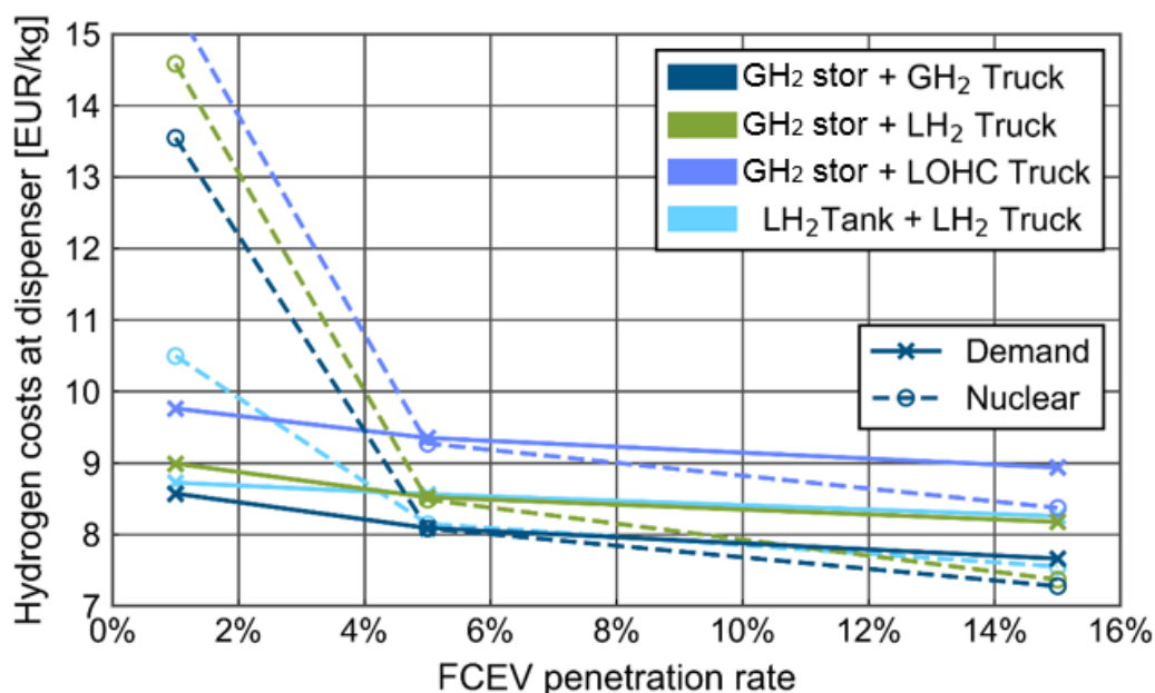
Figure 83: Comparison of total hydrogen costs at the dispenser for the placement next to nuclear power plants and next to the demand for supply pathways
