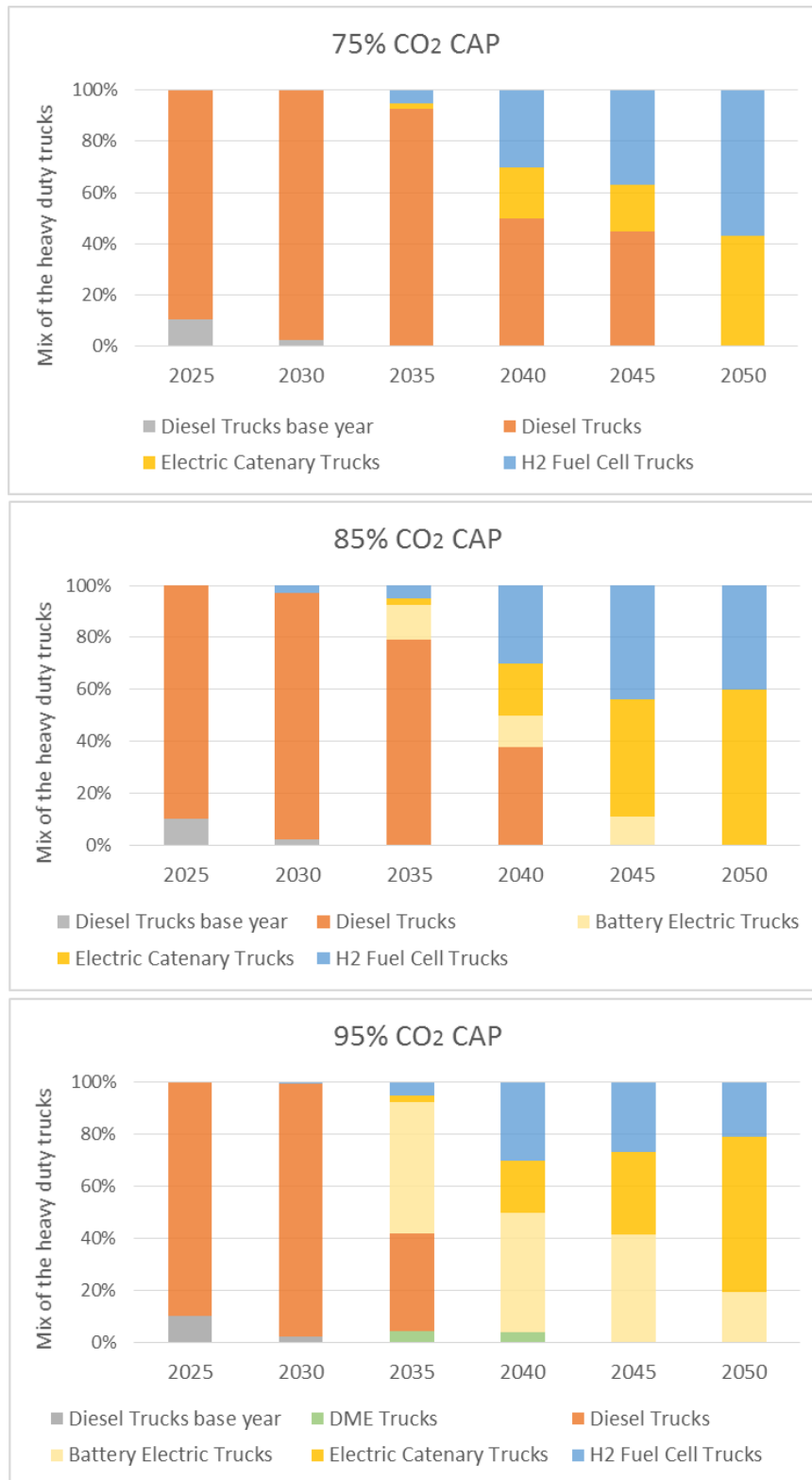
Figure 45: The transport technology mix considering the heavy-duty truck segment
