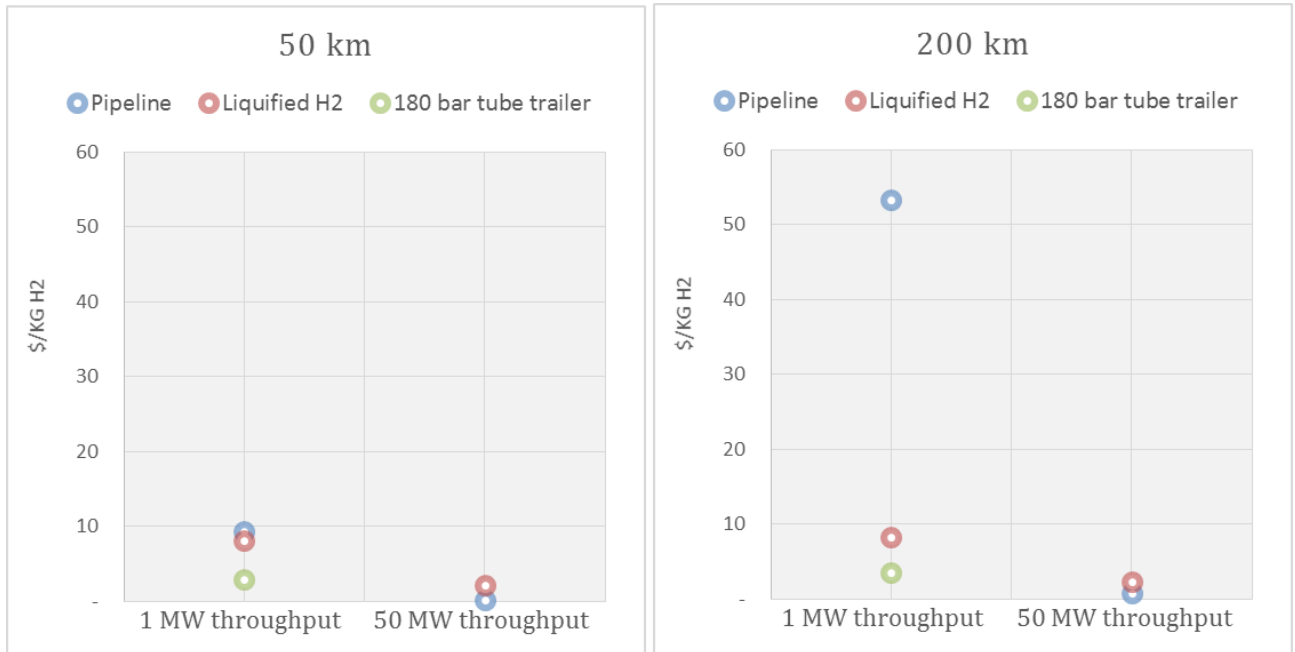
Figure 29: Hydrogen transport pathways comparison (adapted from [14])
