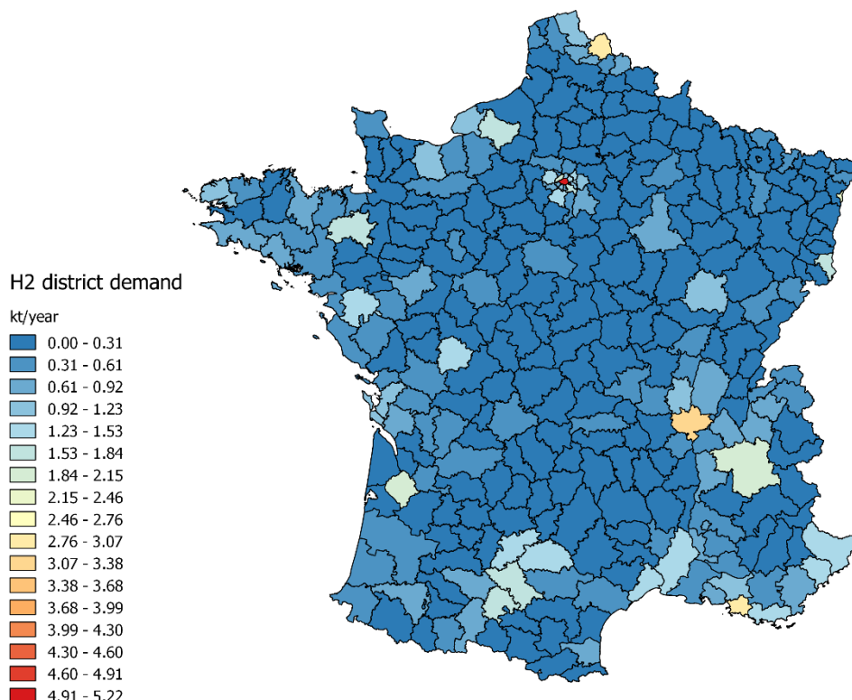
Figure 76: Distribution of hydrogen demand for mobility use for the scenario of 5% market penetration
