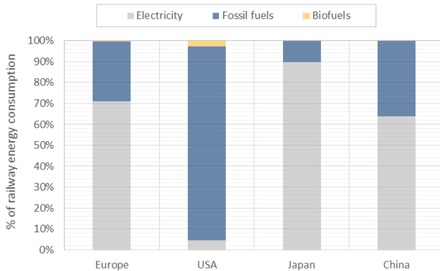
Figure 12: Current railway energy consumption by region - adapted from [50]
