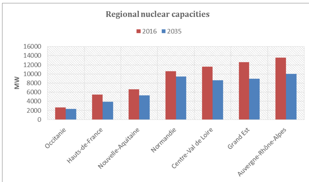
Figure 57: Nuclear capacity distribution by region - designed scenario
