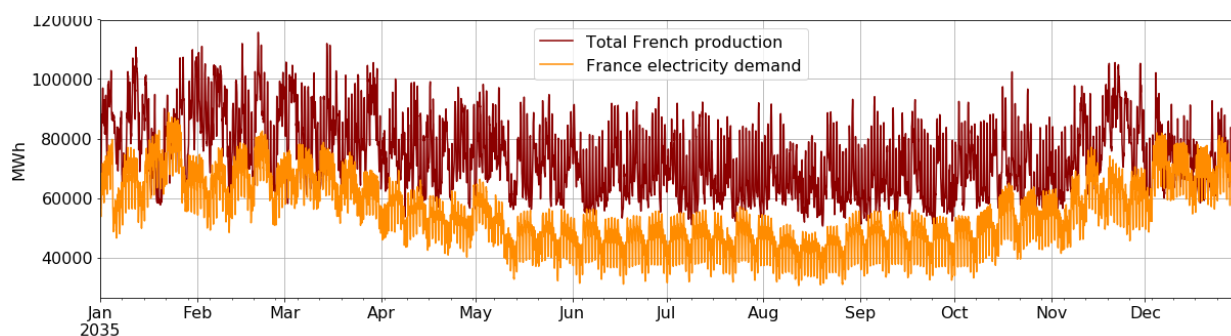
Figure 65: Hourly profile of the electric demand and the total electricity production in France
