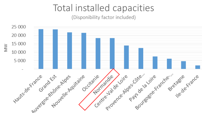
Figure 59: Total installed generation capacity by region
