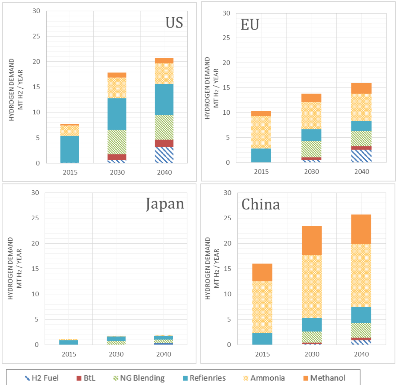
Figure 15: Prospective hydrogen market sizes by region
