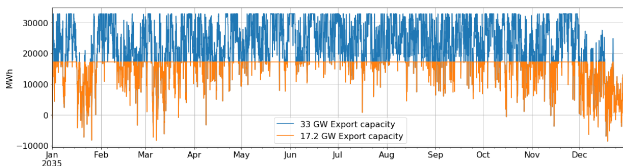
Figure 64: Interconnection balance profiles throughout the year 2035 for the two considered scenarios
