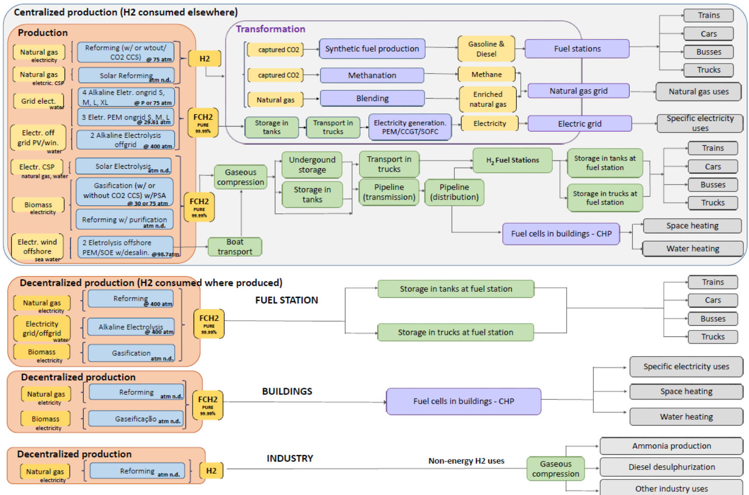
Figure 37: Hydrogen modelling structure in TIMES-PT
