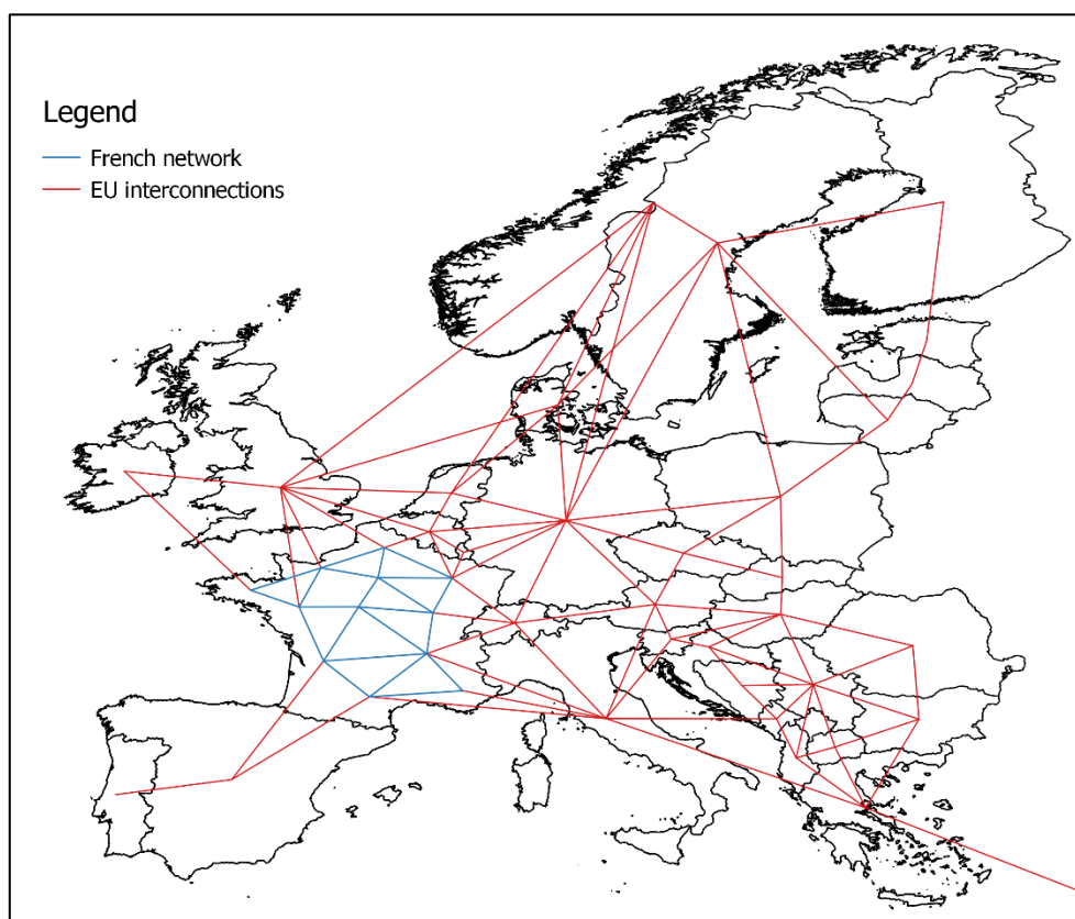
Figure 56: Electric grid lines as implemented in the model
