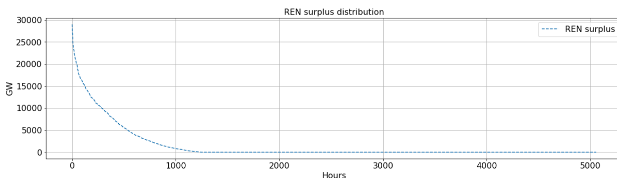
Figure 61: Hourly distribution of the renewable surplus in France
