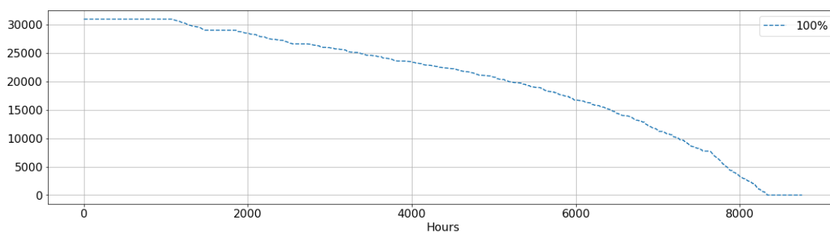
Figure 63: Hourly distribution of the available nuclear energy in [MW]
