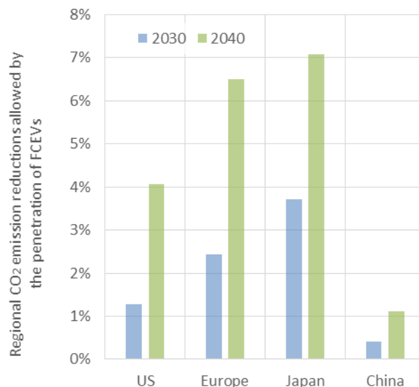
Figure 18: Share of CO 2 emissions avoided by FCEVs in the total transport sector emissions by region
