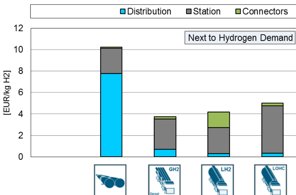
Figure 81: Hydrogen delivery cost (scenario 5% market penetration)
