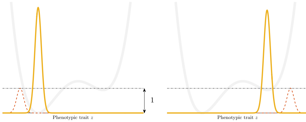
Figure III.1: Numerical simulations of the stationary problem (PF_\varepsilon) with \varepsilon = 0.1 in an asymmetric double-well mortality rate (grey line). The numerical equilibrium is in yellow plain line. The only difference between the two simulations is the initial data (red dashed line). The simulations illustrate the lack of uniqueness for problem (PF_\varepsilon) .
