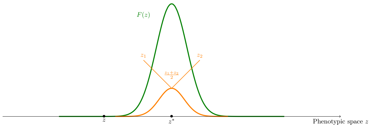
Figure V.6: In orange the distribution law \sigma\mathcal{N}\left(0, \frac{1}{2}\right) of the deviation from the mean trait of parents.
