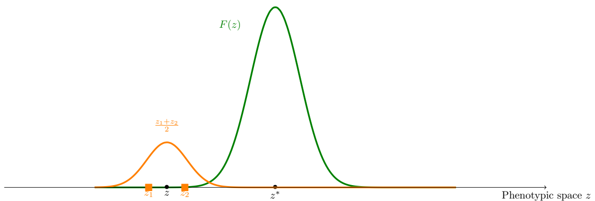
Figure V.7: Both parents have a trait in a very low density zone of F .
