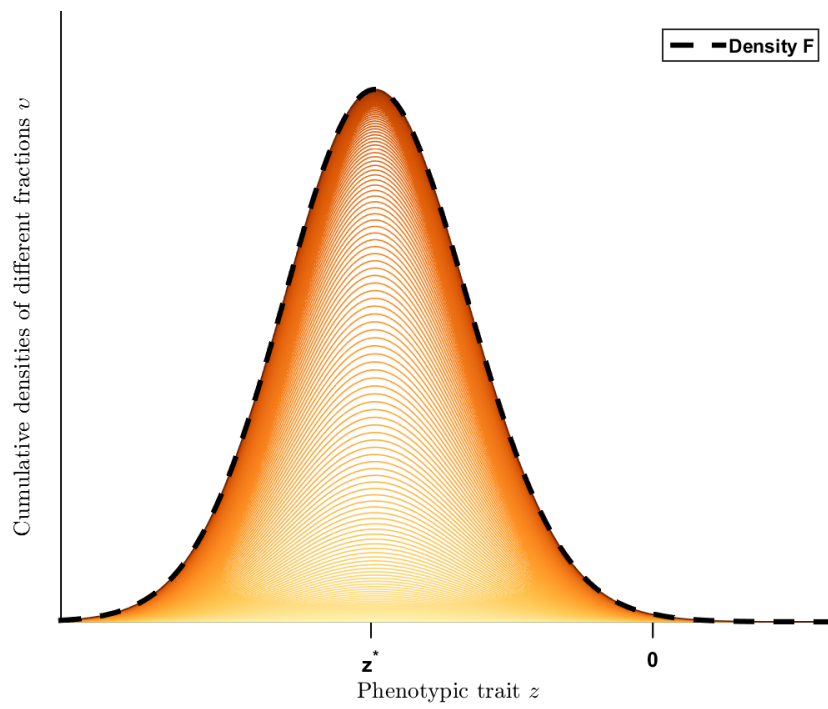
Figure V.12: Cumulative densities of the fractions v_k .
