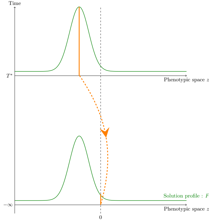
Figure V.5: Lineage arriving at dominant trait mostly come from optimum trait.
