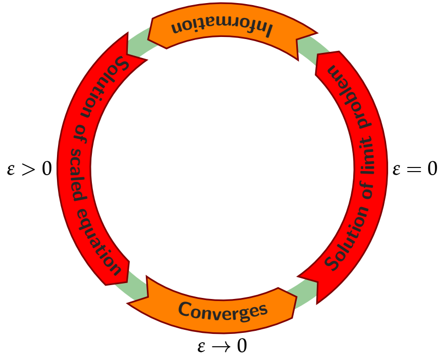
FIGURE I.1 : Math flow
