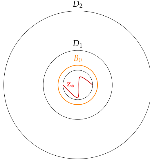
Figure IV.2: Illustration of the division of the space in successive dyadic rings.
