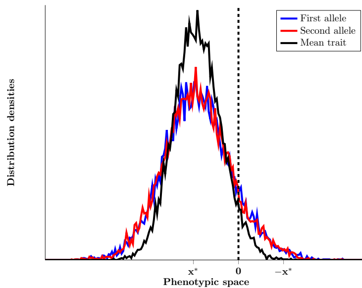
Figure V.16: Profile of the distributions of the first allele and second allele of all individuals in the population, and its mean.
