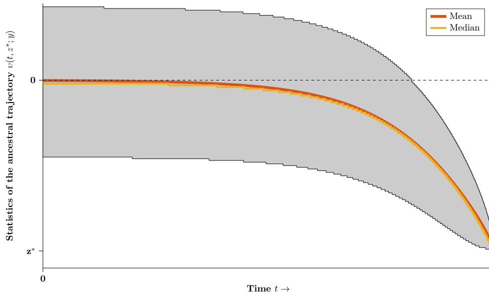
Figure V.14: Evolution of the mean and median of v(t, z^*; y) along time. The grey area corresponds to the region between the 5% and the 95% quantile of the distribution.
