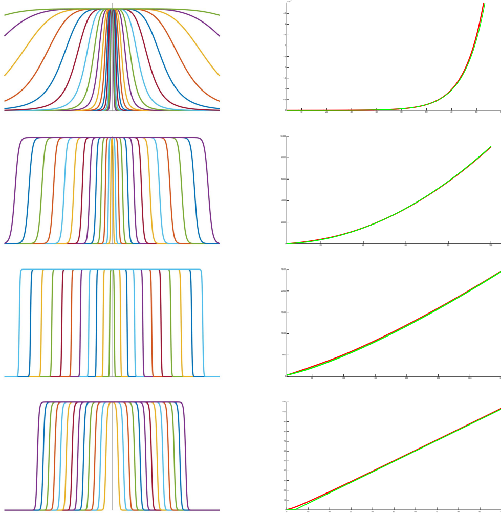
Figure II.1: Numerical simulations of the Cauchy problem (II.1.1), for various kernels J . The first line corresponds to J \sim |x|^{-5} , the second line to J \sim \exp(-|x|^{1/2}) , the third line to J \sim \exp(-|x|^{3/4}) and the last line to a Gaussian kernel J \sim \exp(-|x|^2) . For each kernel, we present in the left column the evolution of the solution by plotting it on the same figure for various successive (linearly chosen) values of time t . To quantify this and recover and illustrate Theorem (II.6), we present in the right column the time evolution of the level set \{x \in \mathbb{R} : n(t, x) = 1/2\} for each kernel. The red bold curve is the numerical simulation, starting from an initial condition of the form J . The green curve is the expected asymptotic rate of expansion predicted by Theorem (II.5), that is J^{-1}(e^{-t}) , except for the Gaussian kernel, in which case it is a line. Each kernel is successively more thin-tailed, yielding an interpolation between the obvious acceleration for the first kernel and the linear propagation for the last kernel.
