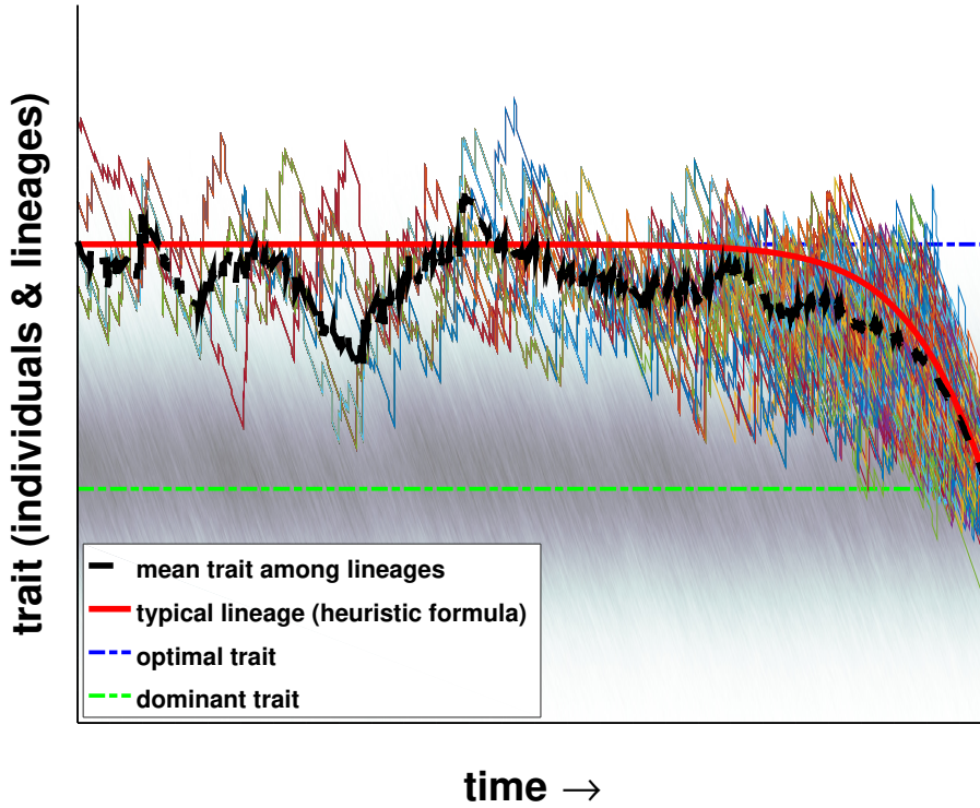
Figure V.4: The grey background is the stationary density of individuals F . The y axis represents the phenotype z in the moving frame ( z = x - ct ).
