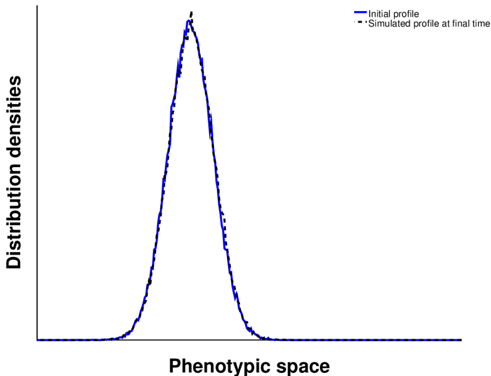
Figure V.9: The x axis represents the phenotype z in the moving frame ( z = x - ct ).
