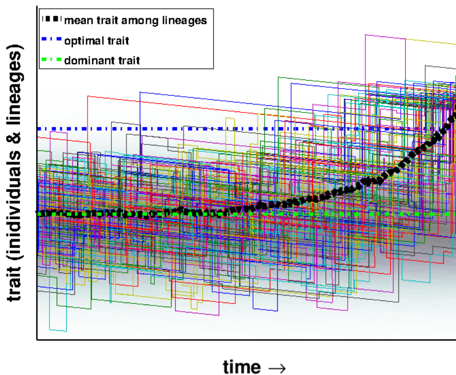
Figure V.10: The grey background is the stationary density of individuals F . The y axis represents the phenotype z in the moving frame ( z = x - ct ).
