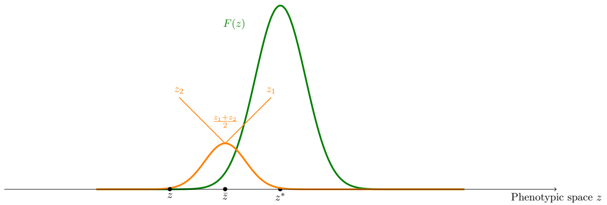
Figure V.8: Most probable scenario : both parents at \bar{z} .
