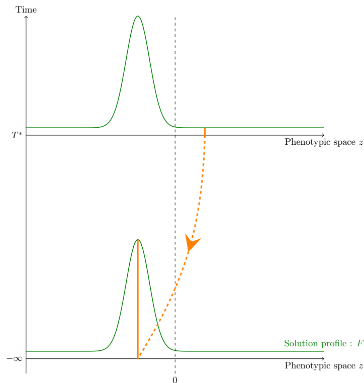
Figure V.11: Lineage arriving at any trait mostly come from dominant trait.
