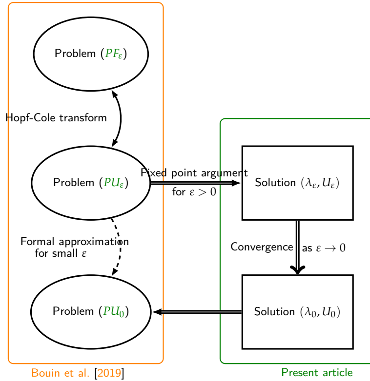
Figure III.2: Scope of our paper compared to precedent work
