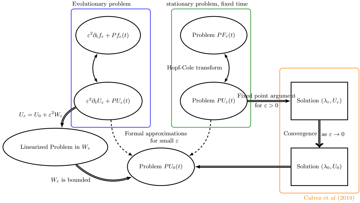
Figure IV.1: Scope of our paper compared to precedent work
