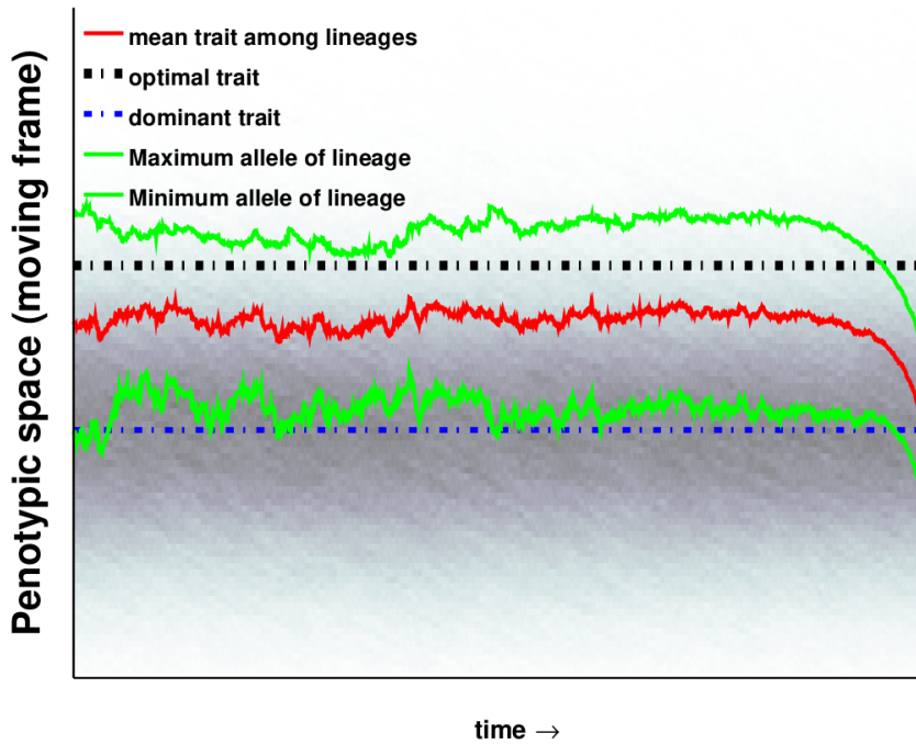
Figure V.17: The green plots represent the mean (over all ancestors) of the maximum and minimum alleles. In gray, the invariant density profile of the mean of alleles.
