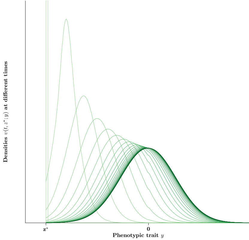
Figure V.15: Snapshots of the whole distribution v(t, z; y) at different times.
