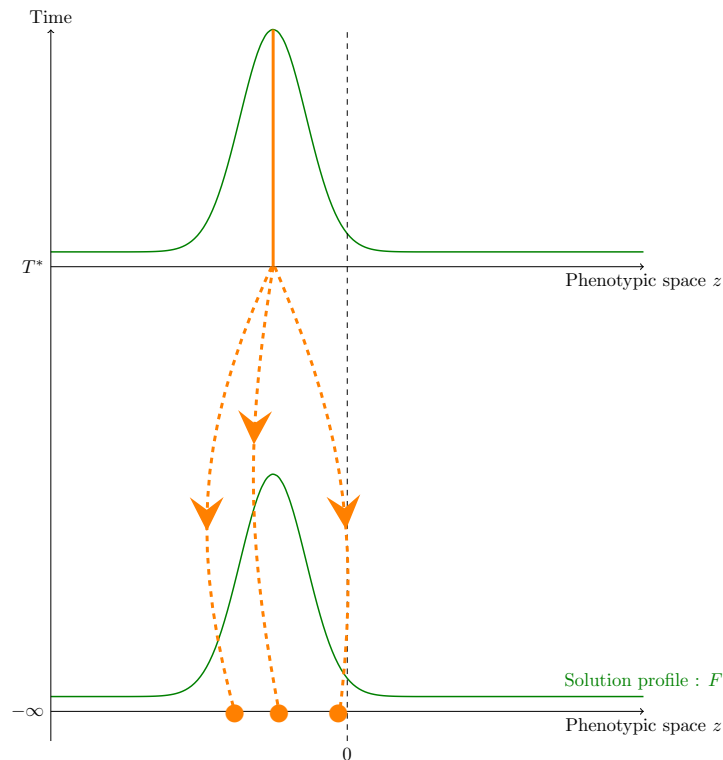
Figure V.1: Potential lineages arriving at the dominant trait z^* at time T^* . Which one of the orange arrows is the typical behavior of lineages?
