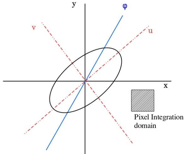
Figure 3.3: Filter transformation description. The integration domain is limited by four lines, the equations of which we can write in the new system of axes through a coordinate change..
