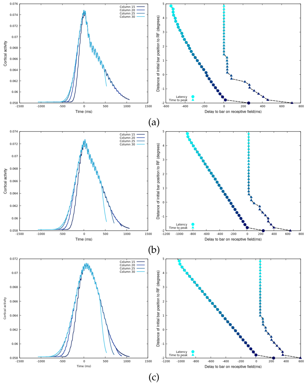
Figure 6.18: The effect of conduction velocity. Time course of responses and latency-time to peak curves, for a conduction of (a) 50 mm/s (b) 100 mm/s and (c) 400 mm/s.
