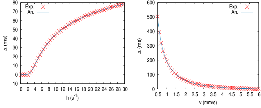
Figure 4.3: Anticipation time \Delta for a Gaussian pulse. Red points correspond to the numerical simulations and blue line to the analytic approximation (4.6). Left: \Delta as function of h ( v = 3 mm/s; \sigma = 0.162 mm). Right: \Delta as function of v ( \sigma = 0.162 mm; h = 6.1 s ^{-1} ).
