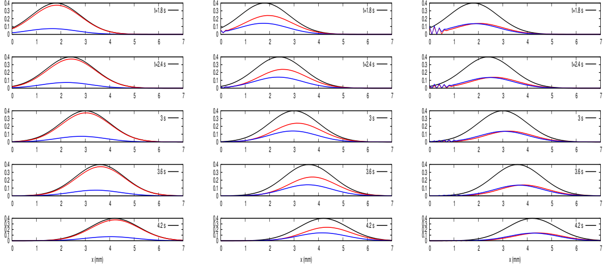
Figure 4.6: . Effect of a Gaussian drive (in black) propagating in one dimension, on the bipolar cells voltage (red) and on the amacrine cells voltage (blue). There are 100 cells, spaced by 0.1 mm. The Gaussian drive (4.2) travels at a speed 1\text{mm/s} . Other parameters are fixed as in the Appendix. We illustrate the effects on increasing the coupling w , where w^+ = w , w^- = -w , with \frac{1}{T} = 0 . Left. Weak coupling, w = 1\text{ s}^{-1} . Middle. Moderate coupling where w = 3\text{ s}^{-1} . Here w is smaller than the first instability threshold (here w_{99,c} = 3.53639\text{ s}^{-1} ) given by (4.31). Right. Strong coupling, w = 5 , above the instability threshold w_{67,c} = 3.53639\text{ s}^{-1} . That is the modes n = 67, \dots, 99 are linearly unstable here, but gain control and the non linearity stabilize the divergence. Compare with fig. 4.7 below.
