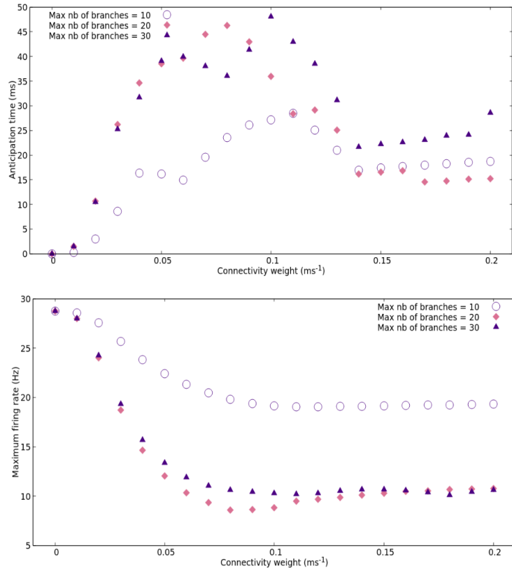
Figure 5.13: Variability of anticipation time and maximum firing rate with the maximum number of branches.
