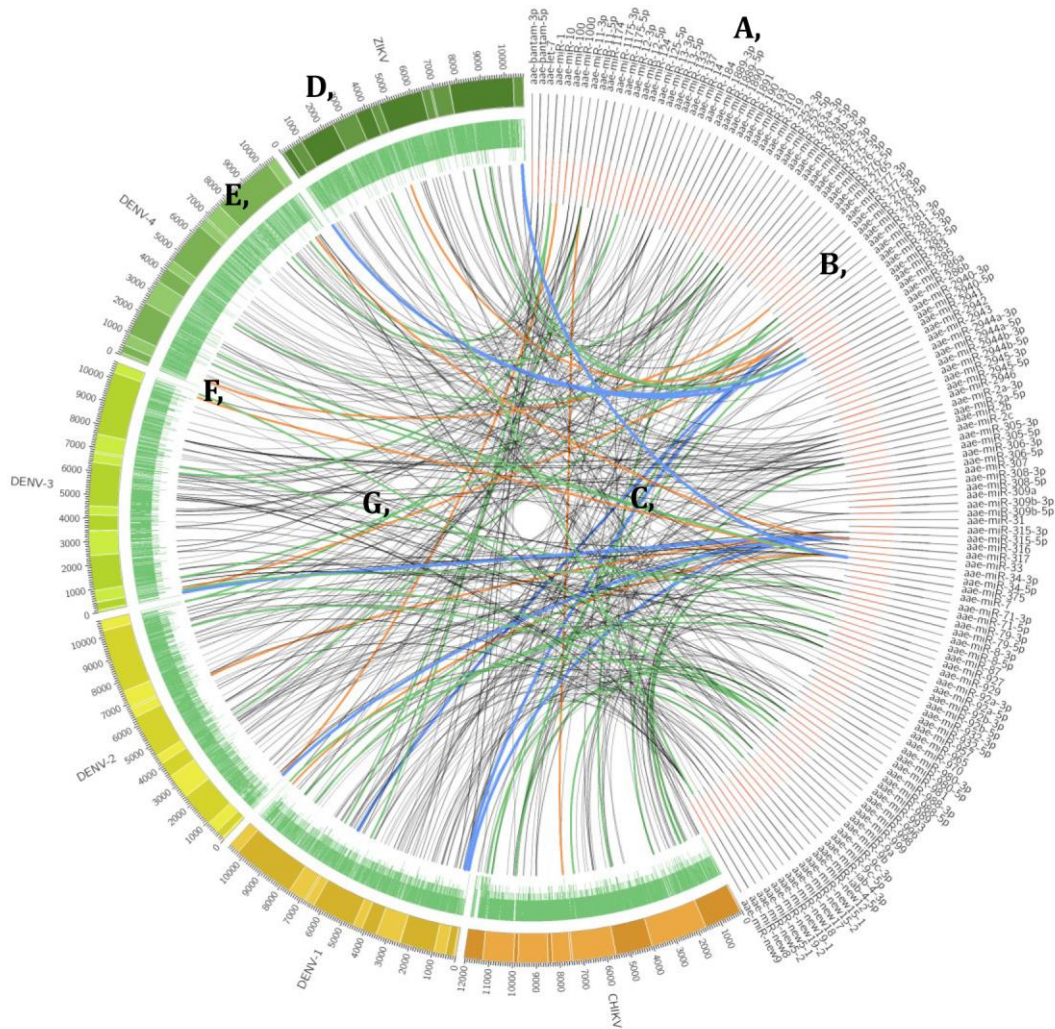
FIG 7 The interactome of Ae. aegypti miRNAs with DENV, ZIKV and CHIKV genomes as predicted by miRanda and TargetSpy. (A) miRNAs of Ae. aegypti ; (B) miRNA and its seed region (seed region in red); (C), links between miRNAs and potential binding regions on the viruses; (D) genomes of arboviruses; (E) dark and light areas represent the protein coding regions in each virus; (F) conservation scores of virus among all the genotypes; green links, the miRNA binding site that shared among most of genotypes discussed in this study; orange links, the miRNA-vRNA with low energy; blue links, the miRNA-vRNA with low energy and is shared among most arboviruses; black links, remaining miRNA-vRNA interactions.
