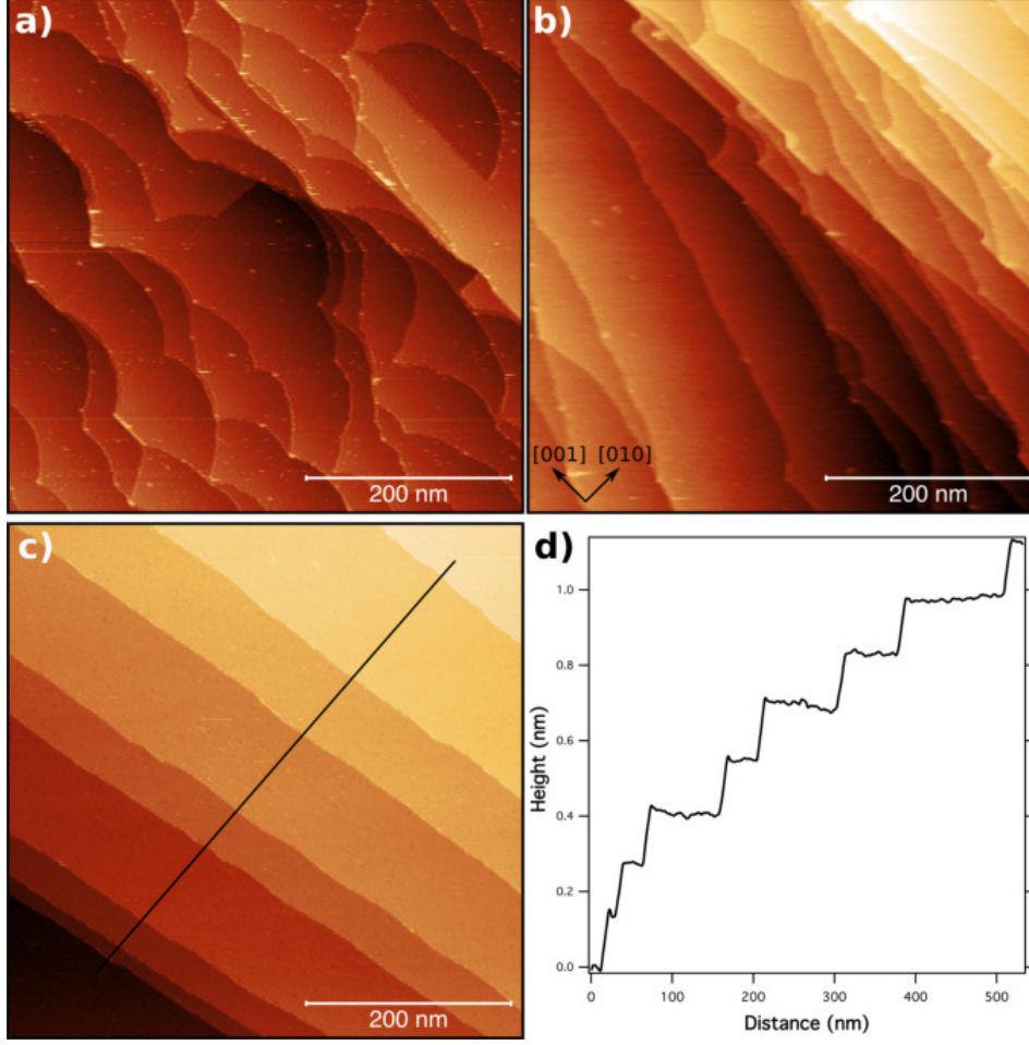
Figure 5.18: Large scale STM images ( 500 \times 500 \text{ nm}^2 ) of the \text{Fe}_{0.85}\text{Al}_{0.15} (100) surface after annealing at three different temperatures: a) 1051 K ( U_b = 1.5 \text{ V} , I_t = 0.4 \text{ nA} ), b) 1078 K ( U_b = 0.9 \text{ V} , I_t = 0.1 \text{ nA} ), c) 1178 K ( U_b = -0.9 \text{ V} , I_t = 0.3 \text{ nA} ). d) Line profile drawn on the image c.
