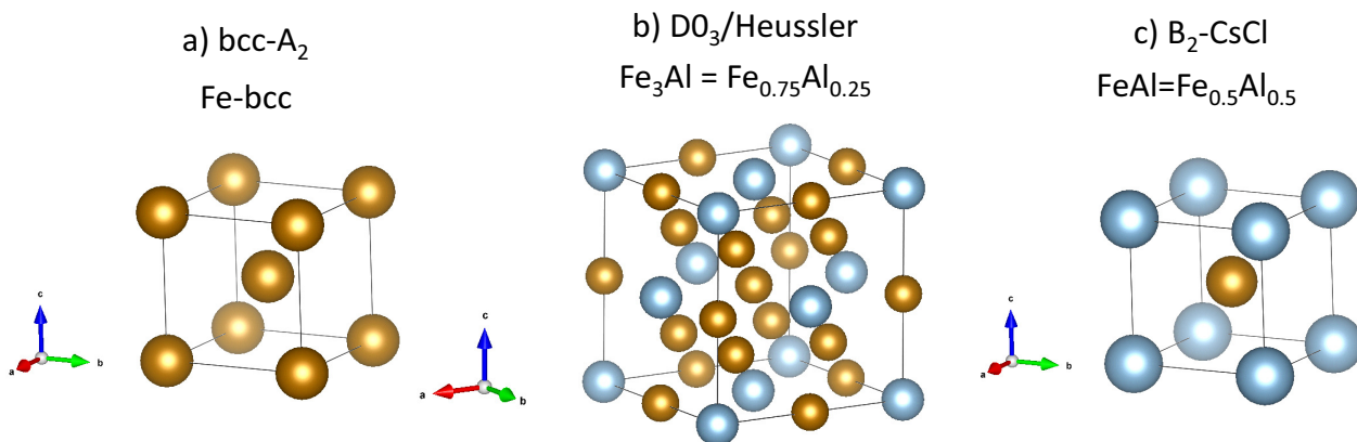
Figure 3.2: Ball models of the main atomic structure of iron rich \text{Fe}_{1-x}\text{Al}_x intermetallics. Fe atoms are in brown and Al atoms in light blue.
