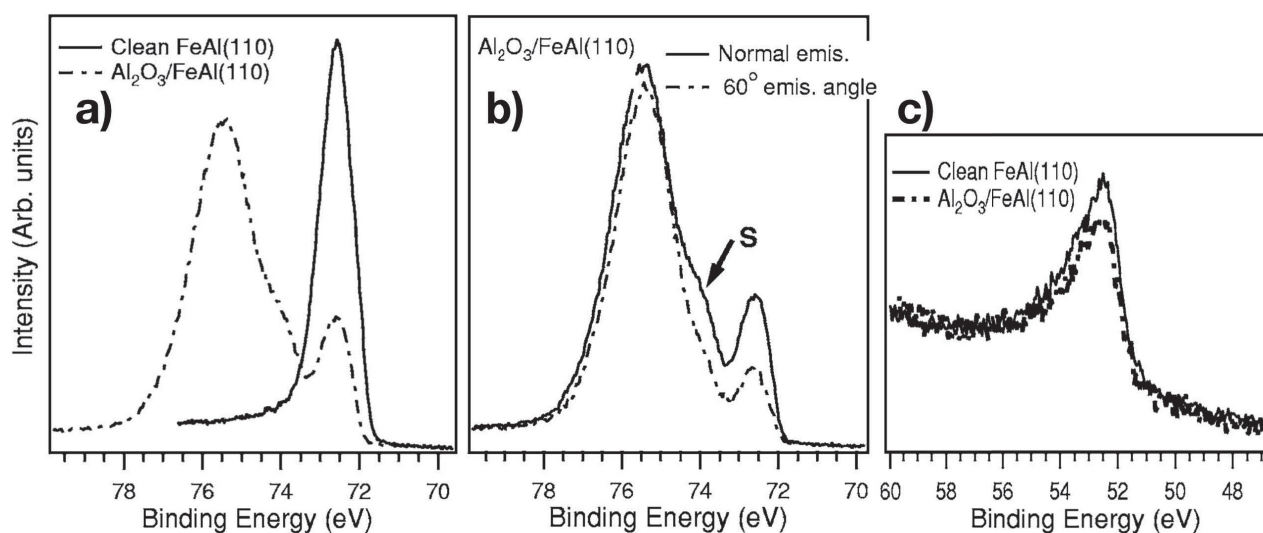
Figure 3.35: Al 2p core level spectra of Fe_{0.53}Al_{0.47}(110) surface. a) Comparison of clean and oxidised surfaces at normal emission; b) Spectra of the oxidised surface at normal ( 0^\circ ) and grazing ( 60^\circ ) emission, revealing a weak shoulder assigned to the existence of interfacial Al atoms; c) Comparison of Fe 3p spectra of clean and oxidised surfaces showing the lack of chemical shift. The photon energy is 150 eV. From Ref. [99].
