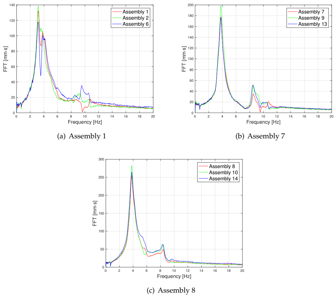
FIGURE 3.26: Frequency response of displacements in symmetry (Total flowering)
