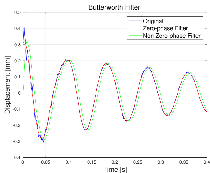
FIGURE 2.13: Comparison of zero-phase filtering and non-zero filtering
