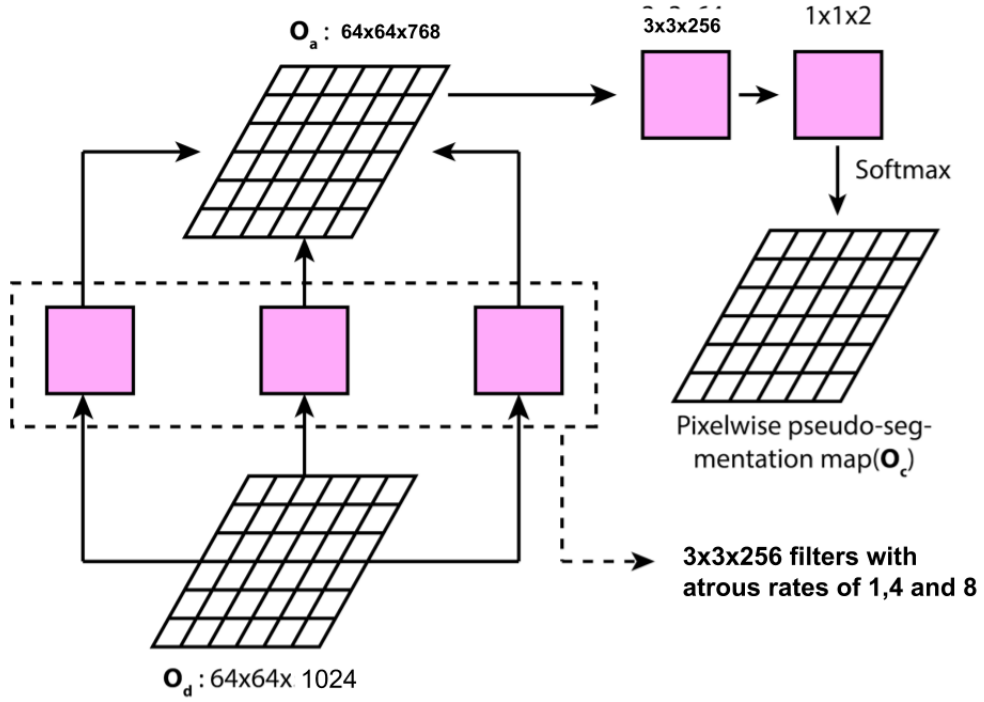
Figure 5.12: Semantic Segmentation module of the proposed system.
