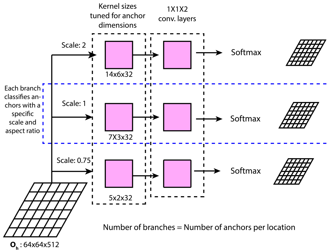
Figure 6.5: The anchor selection layer. For illustration it is assumed that all anchors have been generated by a base anchor of size 64 \times 64 and have an aspect ratio of 0.41 ( width/height ). The anchor at scale 1 then corresponds to a box of size \sim 100 \times 41 . For a feature stride of 16, a kernel of size 7 \times 3 will cover the corresponding area of this box in the feature map. For other scale values, the kernel size can be similarly defined.
