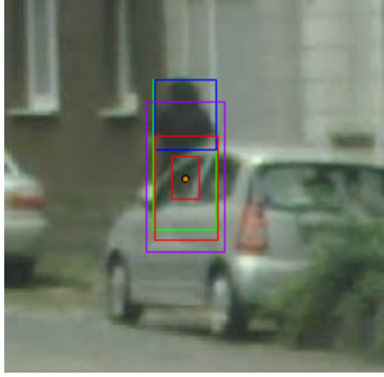
Figure 6.4: An occluded pedestrian with full-body bounding box ( green ) and visible bounding box ( blue ). Red anchors are confocal with the magenta anchor. The red anchors do not overlap well with both the full-body and visible bounding box, while the magenta anchor has sufficient overlap with both.
