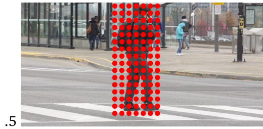
Figure 5.9: Normal Convolution
