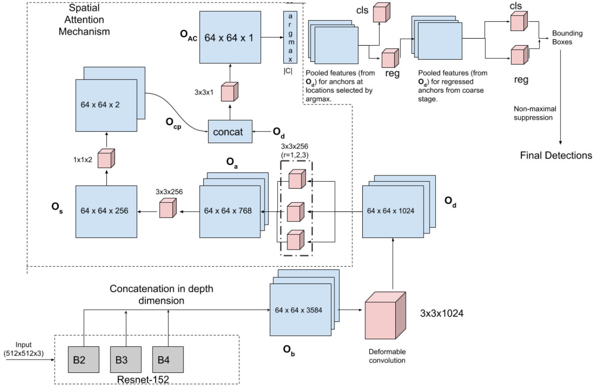
Figure 5.5: Block diagram of the proposed approach.
