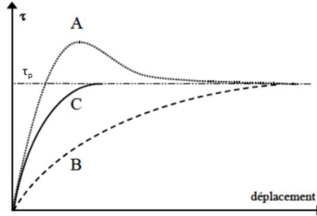
Figure 14: Curves of the shear depending on the consolidation stress. A: Over-consolidated, B: Sub-consolidated, C: Consolidated in critical state [14]
