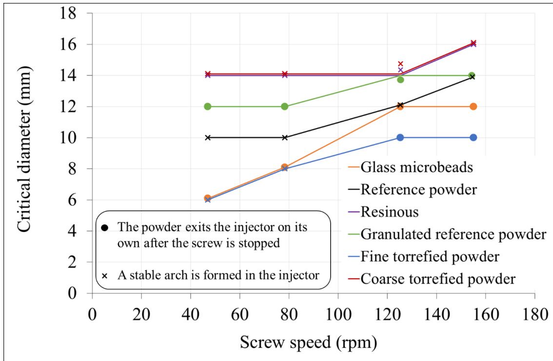
Figure 102: Accumulation critical diameter as a function of the screw speed.
