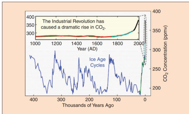
Figure 1: Evolution of the CO 2 atmospheric concentration [2].
