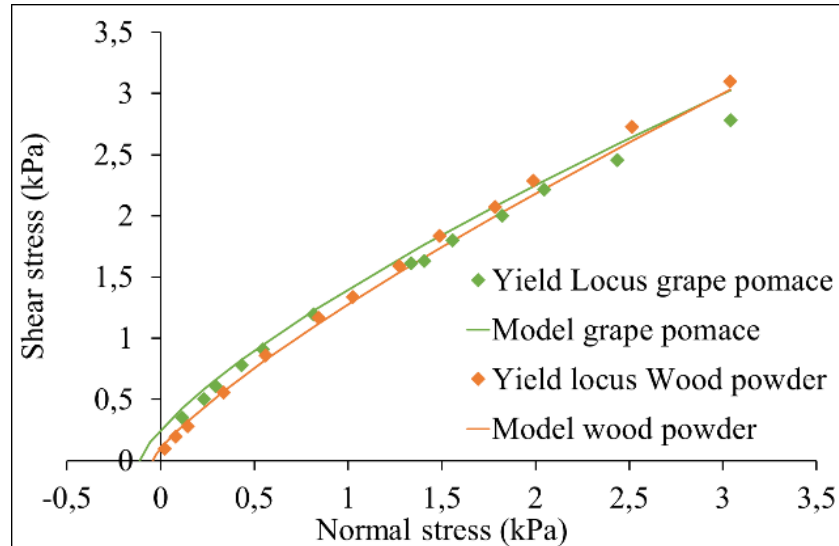
Figure 61: Yield locus at 3 kPa preconsolidation and corresponding model for two biomasses
