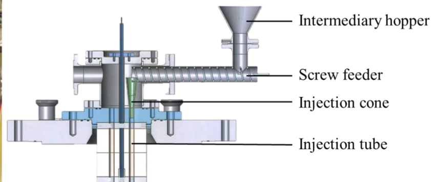
Figure 86: Left, picture of the shaftless screw feeder (axial view). Right, section of the reactor showing the bottom part of the injection system (side view).
