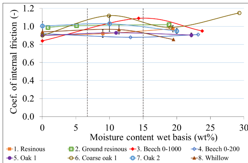
Figure 67: Evolution of the coefficient of internal friction with moisture content for the eight powders
