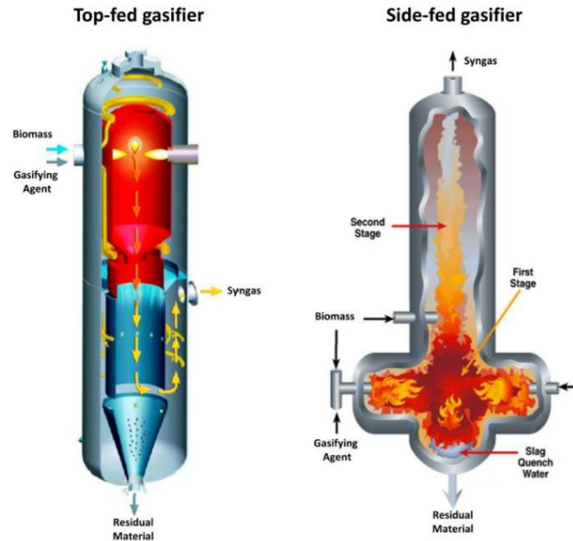
Figure 27: Schematics of entrained flow reactors.[60].
