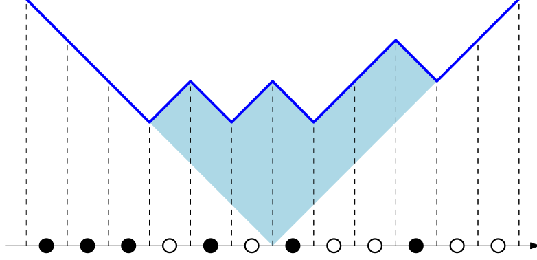
Figure 4.3 – The correspondence between Maya diagram and partitions. Here we consider the partition \lambda = (4, 2, 1) , whose parts give the displacements of the particles ( \bullet ) with respect to their “ground state”. The parts of the conjugate partition \lambda' = (3, 2, 1, 1) give the displacements of the holes ( \circ ).
