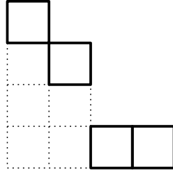
Figure 0.5 – The skew Young diagram of shape (4, 2, 2, 1)/(2, 2, 1) , shown in French convention. It is a horizontal strip since no two cells are in the same column.
