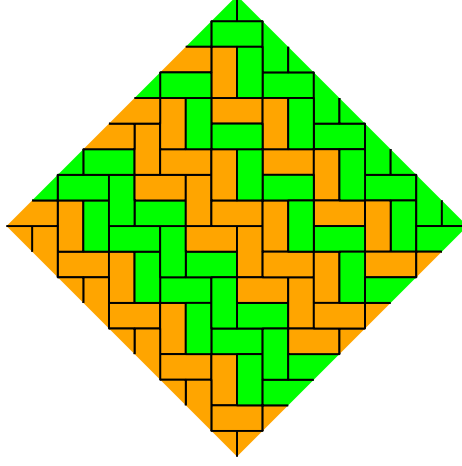
Figure 4.4 – The periodic steep tiling corresponding to the constant sequence of partitions equal to (3, 2, 2) .
