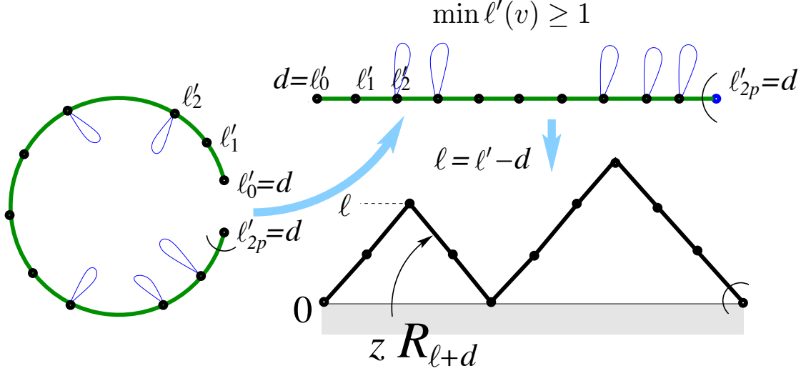
Figure 1.9 – The decomposition of the mobile associated with a map with a boundary counted by W_d . The sequence of labels around the special unlabeled vertex (coming from the root face) is coded by a Dyck path, whose down-steps correspond to the subtrees of the mobile. The global contribution of all possible subtrees for a down-step from height \ell is zR_{\ell+d} . Notice the similarity with Figure 1.7.
