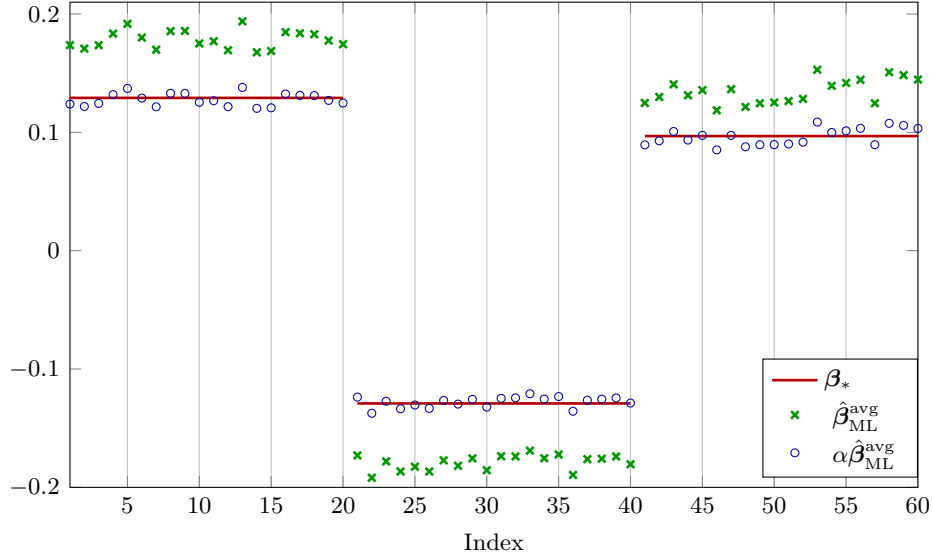
Figure 6.2: Comparison of the maximum likelihood estimate \hat{\beta}_{ML} (averaged over 500 realizations), the true parameter \beta_* and the rescaled classifier \alpha\hat{\beta}_{ML} defined in Theorem 6.3.1 with \mu = [\mathbf{1}_{p/3}, -\mathbf{1}_{p/3}, \frac{3}{4}\mathbf{1}_{p/3}]/\sqrt{p} , \mathbf{C} = 2\mathbf{I}_p , for p = 60 and n = 300 .
