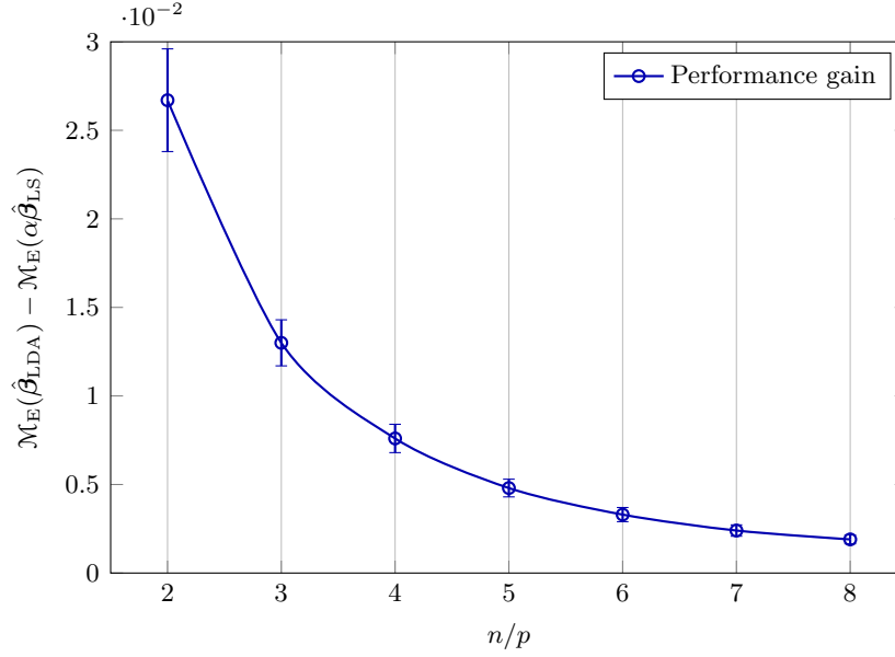
Figure 6.7: Performance gain \mathcal{M}_E(\hat{\beta}_{LDA}) - \mathcal{M}_E(\alpha \hat{\beta}_{LS}) with a width of \pm 1 standard deviation (generated from 500 trials) for \boldsymbol{\mu} = [1, \mathbf{0}_{p-1}] , \mathbf{C} = \mathbf{I}_p and p = 256 .
