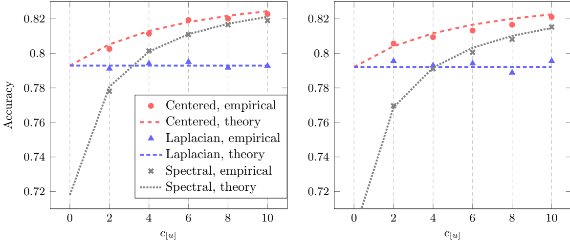
Figure 4.2: Empirical and theoretical accuracy as a function of c_{[u]} with c_{[l]} = 2 , \rho_1 = \rho_2 , p = 100 , -\mu_1 = \mu_2 = [-1, 0, \dots, 0]^T , \mathbf{C} = \mathbf{I}_p (left) or \{\mathbf{C}\}_{i,j} = .1^{|i-j|} (right). Graph constructed with w_{ij} = e^{-\|\mathbf{x}_i - \mathbf{x}_j\|^2/p} . Averaged over 50000/n_{[u]} iterations.
