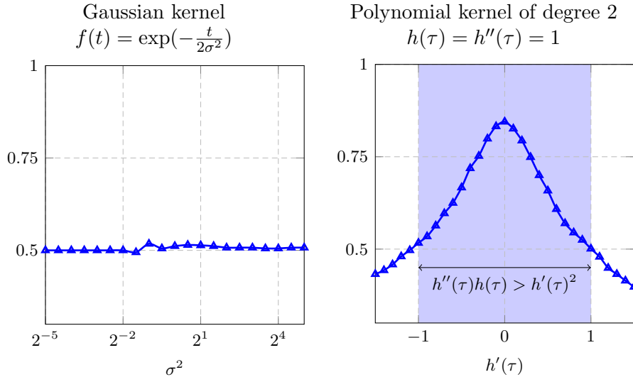
Figure 3.4: Empirical accuracy for 2-class Gaussian data with \mu_1 = \mu_2 , \mathbf{C}_1 = I_p and \mathbf{C}_2 = (1 + \frac{3}{\sqrt{p}})I_p , n = 1024 , p = 784 , n_l/n = 1/16 , n_{[u]1} = n_{[u]2} , n_{[l]1} = n_{[l]2} , \gamma = -1 .
