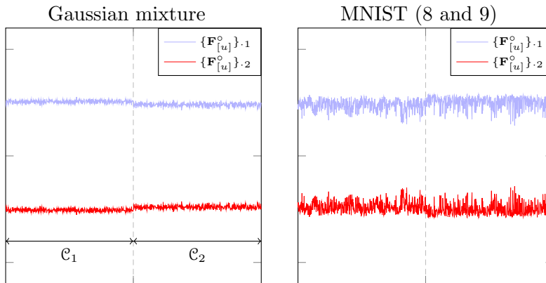
Figure 3.1: \{\mathbf{F}_{[u]}^\circ\}_{\cdot 1} and \{\mathbf{F}_{[u]}^\circ\}_{\cdot 2} for 2-class data, n = 1024 , p = 784 , n_l/n = 1/16 , n_{[l]1} = n_{[l]2} , n_{[l]1} = 3n_{[l]2} , \gamma = -1 , Gaussian kernel.
