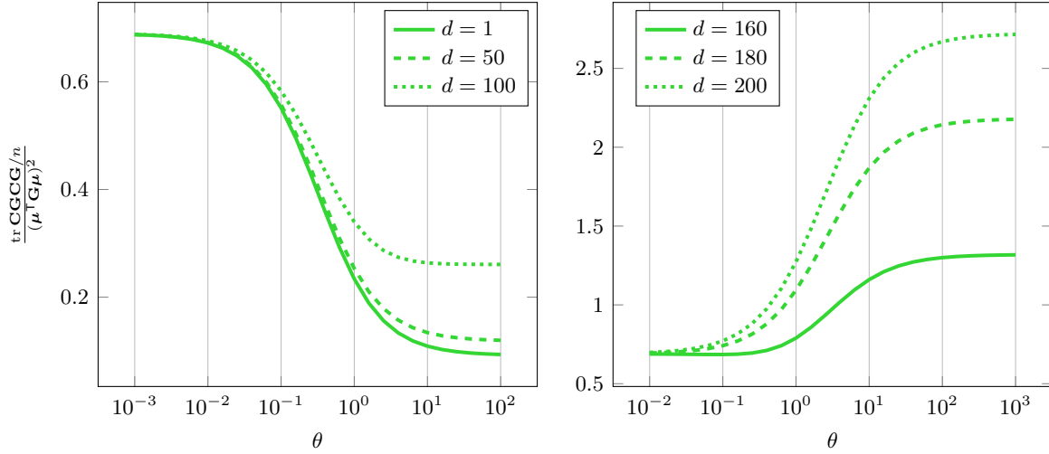
Figure 5.5: \frac{\text{tr } \mathbf{C} \mathbf{G} \mathbf{C} \mathbf{G} / n}{(\boldsymbol{\mu}^\top \mathbf{G} \boldsymbol{\mu})^2} as a function of \theta with n = 400 , p = 200 , \mathbf{C} = \{.4^{|i-j|}\}_{i,j=1}^p , and \boldsymbol{\mu} = \mathbf{v}_d where \mathbf{v}_d is the normalized eigenvector of \mathbf{C} associated with its d -th smallest eigenvalue.
