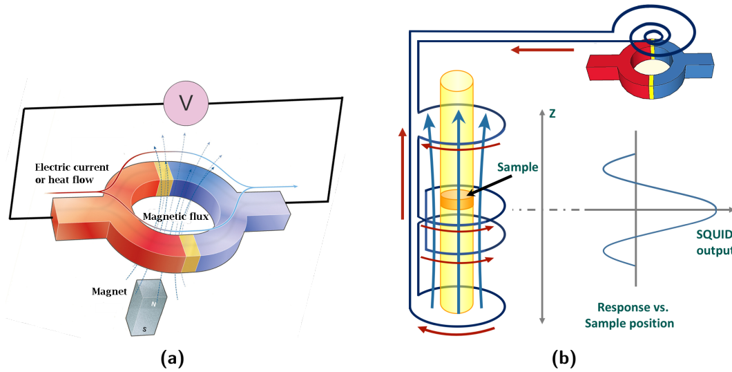
Figure 2.3. (a) A DC SQUID contains two Josephson junctions, the red and blue colors indicate two superconductors while the yellow one indicates the insulator (Image adapted from [81]). (b) A VSM SQUID circuit combines the detection coils. Here, the DC SQUID unit plays the role of current - voltage converter.
