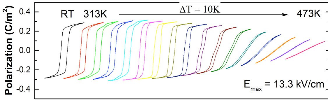
Figure 4.3. The polarization as a function of electric field at various temperatures in the PMN-PT substrate. The P(E) curves are measured at a maximum E -field of 13.3\text{ kV/cm} from room temperature to 473\text{ K} with a step of 10\text{ K} .
