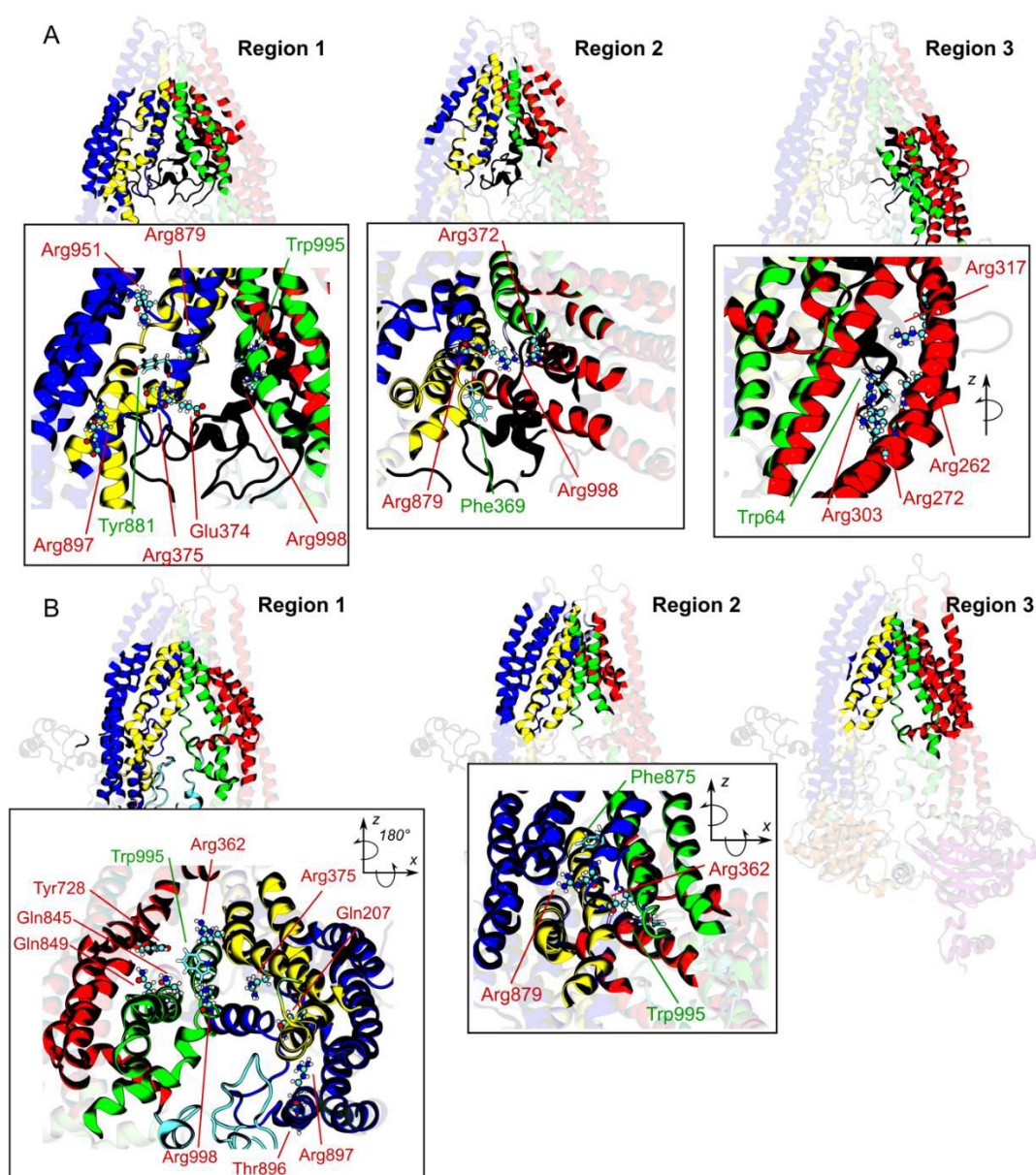
Fig. 1. Binding regions and residues of importance for the modes of binding to MRP4 in A) L_0 -in and B) L_0 -out conformations. Protein secondary structures are colored according to the topology (see Fig. S3 for a detailed definition). Residues of importance involved in H-bonding are depicted in ball and sticks and the corresponding labels are in red. Residues of importance engaged in \pi - \pi stacking interactions are in licorice and labels are in green. Residues of importance of region 3 in MRP4 L_0 -out are not showed owing to a too high overlap with region 1.
