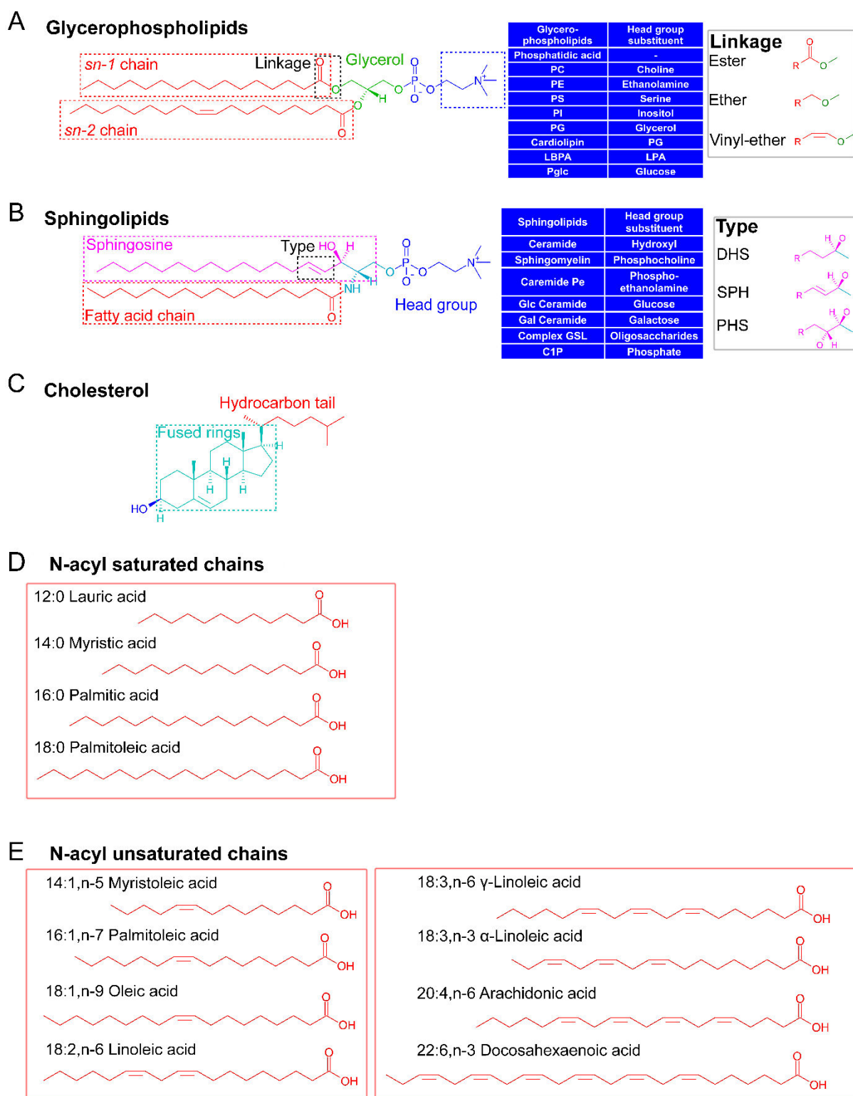
Figure 2: (A) Representation of a characteristic glycerophospholipid, the head group substituents and the linkage between glycerol and fatty chain. (B) Representation of a characteristic sphingolipid, the head group substituent and the different types in the sphingoid base backbone. (C) Representation of a typical sterol, i.e. , cholesterol. (D), (E) N-acyl chains with various length and unsaturation, and position of the double bond. The key is of the form (XX: Y, n-Z), with XX, Y, and Z the number of carbons, double bonds and position of the first double bond from the omega end, respectively. This key describes also the two fatty acyl chains with the form (XX: Y, n-Z): (XX: Y, n-Z). C1P: ceramide-1-phosphate, Complex GSL:
