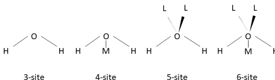
Figure 6: Schematic representation of the different water rigid models.
