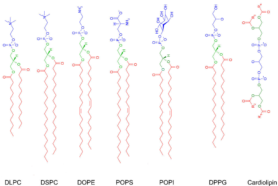
Figure 5: Chemical structures of representative lipids.
