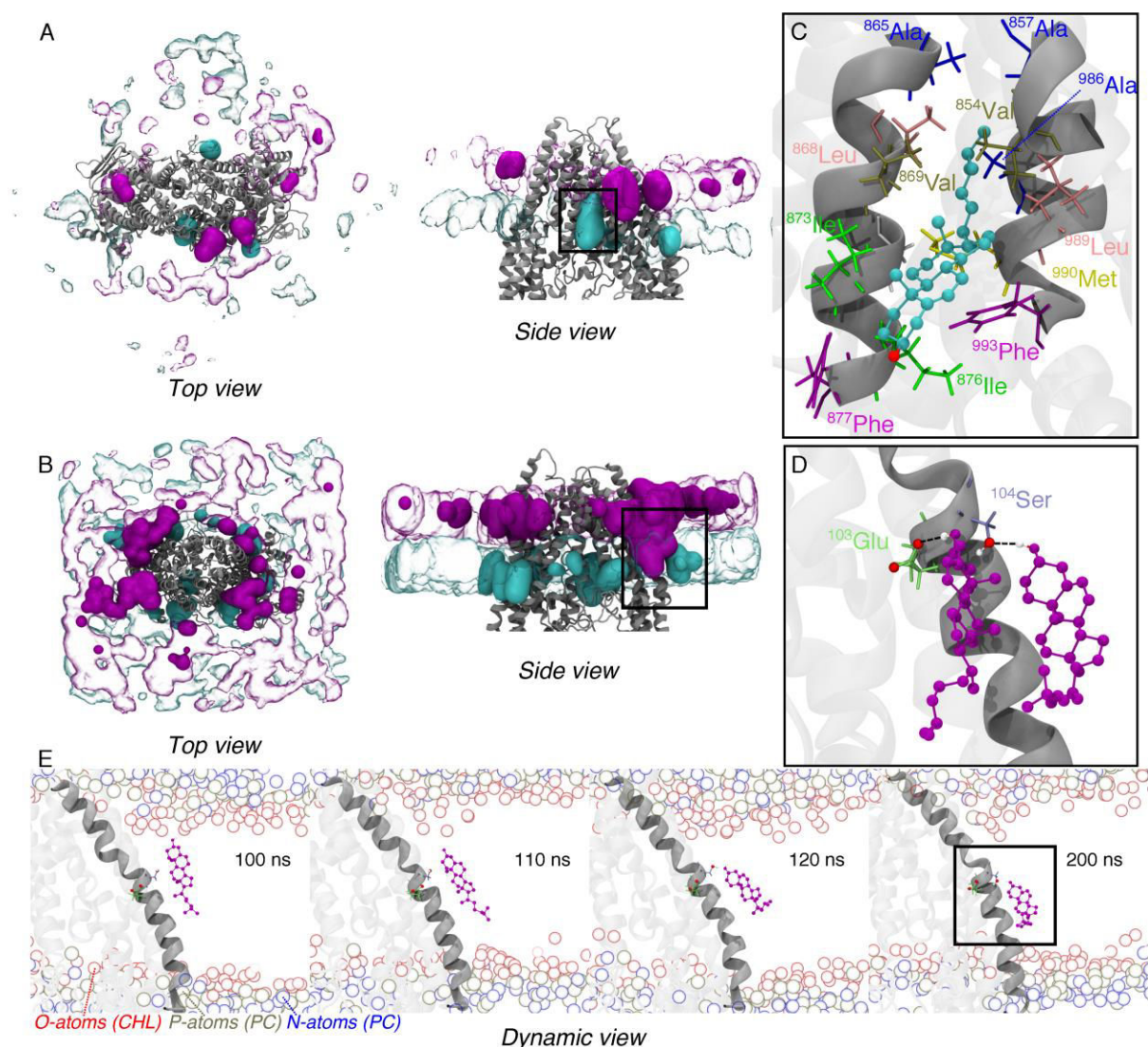
Fig. 3. Top and side views of cholesterol distributions around the exporter embedded in: A) (3:1) POPC:Chol, and B) (1:1) POPC:Chol in bilayer mixtures. The respective specific TMH-Chol interactions are zoomed in panels C) and D). E) Dynamic view of hydrogen bond-driven Chol flip-flop. Upper and lower leaflets are depicted in purple and cyan, respectively.
