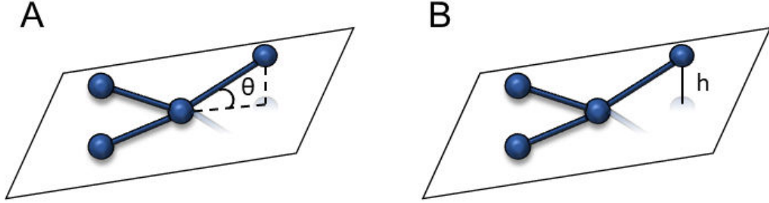
Figure 3: Representation of the out-of-plane torsions adapted from Molecular Modelling. Principles and Applications, by A.R. Leach, 2001.
