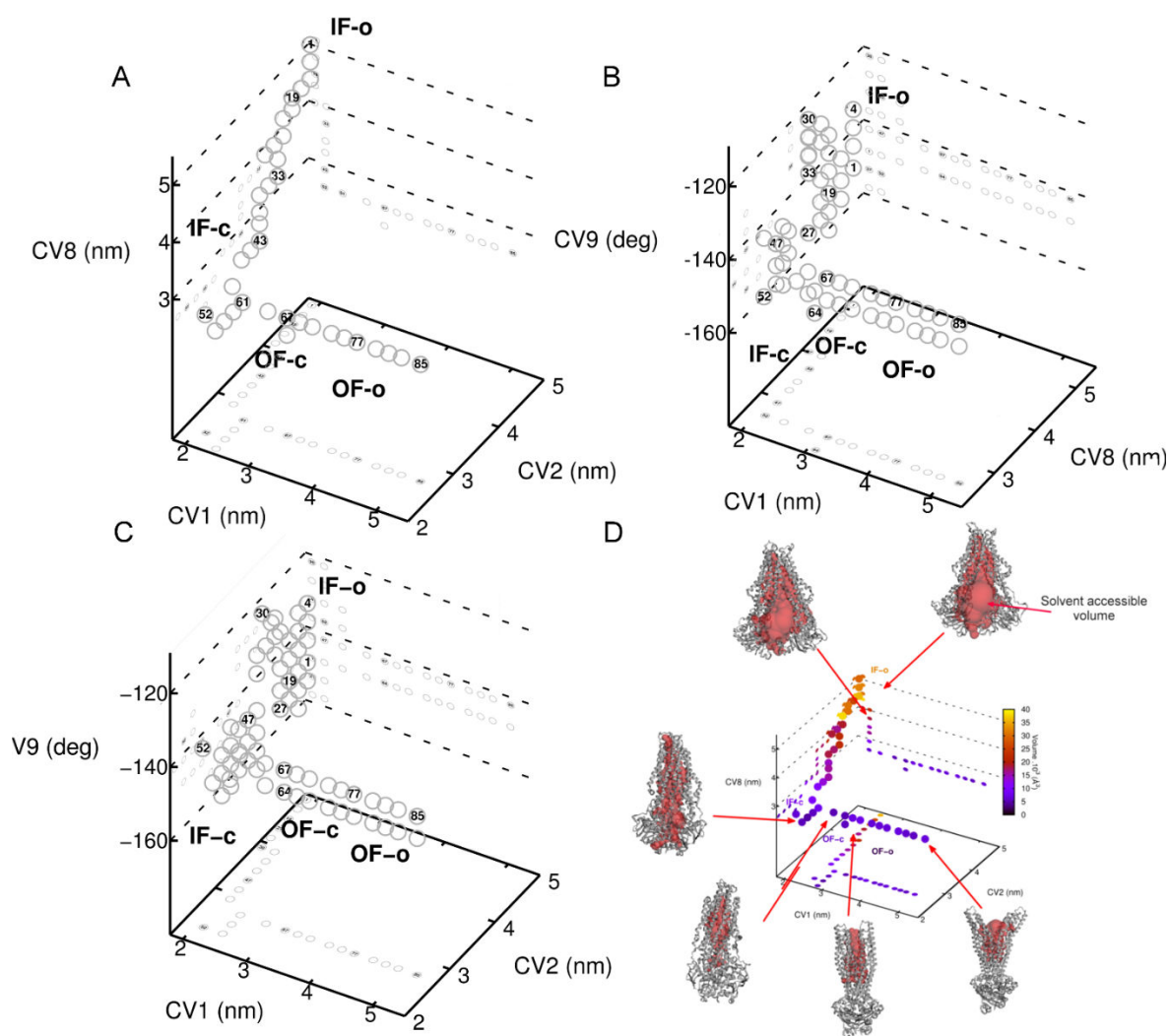
Figure 8: Evolution of A) CV1, CV2, CV8, B) CV1, CV8, CV9, C) CV1, CV2, CV9 along the IF ↔ OF path. D) evolution of CV1, CV2, CV8 along the evolution of the chamber volume.
